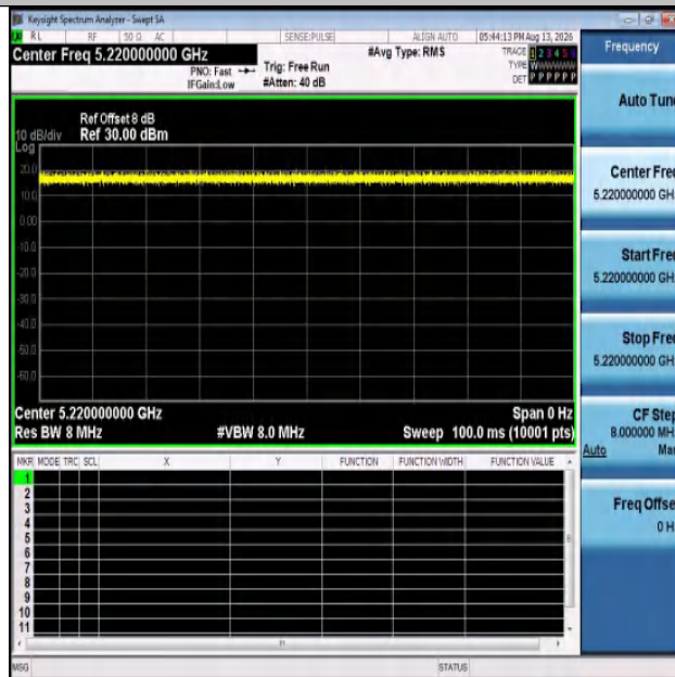
NTNV-11AC20MIMO-Ant2-5220
