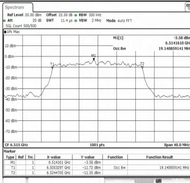
11AX20MIMO-Ant1-6515-PASS
