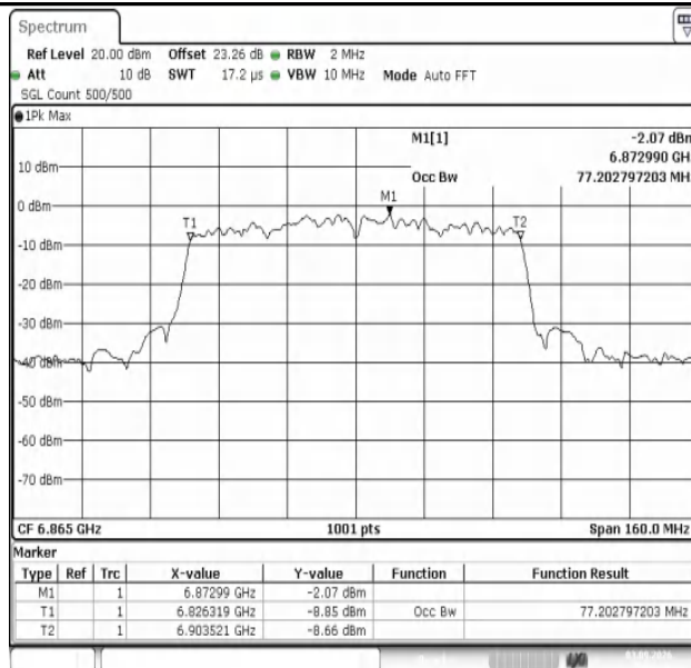
11AX80MIMO-Ant1-6865-PASS
