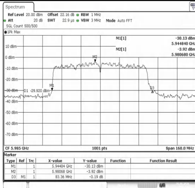
11AX80MIMO-Ant1-5985
