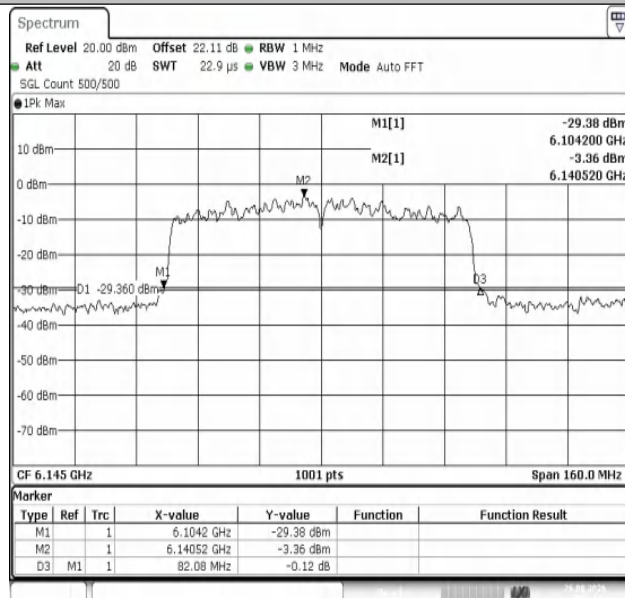
11AX80MIMO-Ant1-6145
