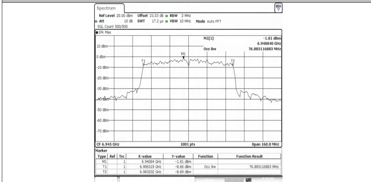
11AX80MIMO-Ant1-6945-PASS
