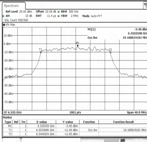
11AX20MIMO-Ant1-6535-PASS
