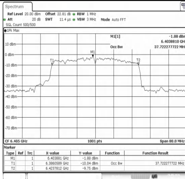
11AX40MIMO-Ant1-6405-PASS
