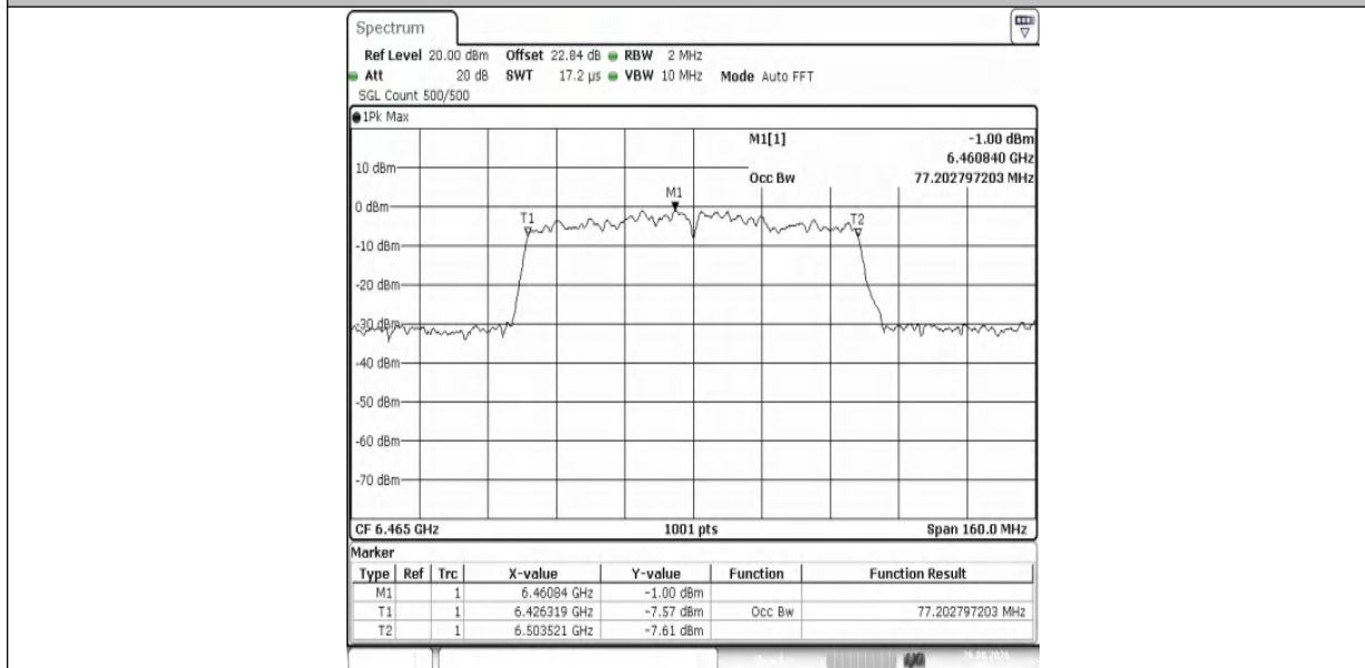
11AX80MIMO-Ant2-6465-PASS
