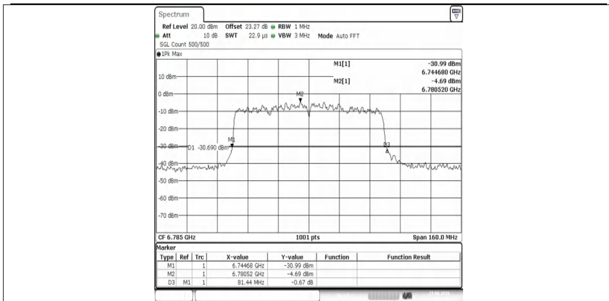
11AX80MIMO-Ant1-6785
