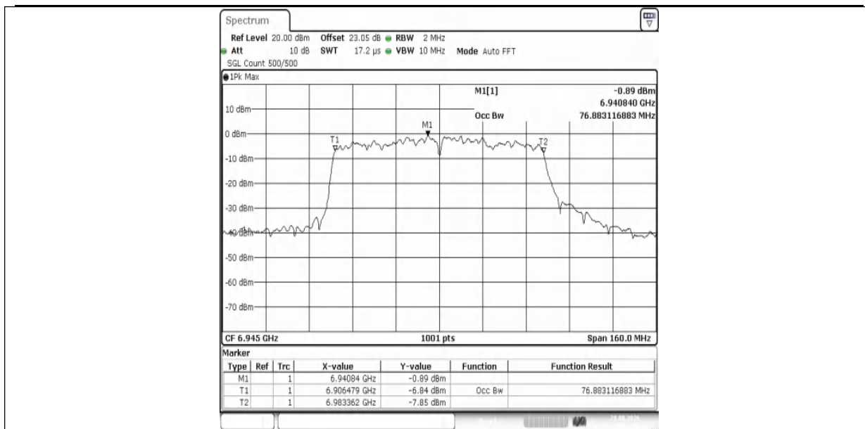
11AX80MIMO-Ant1-6945-PASS
