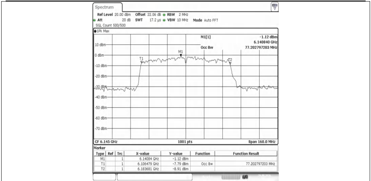
11AX80MIMO-Ant1-6145-PASS
