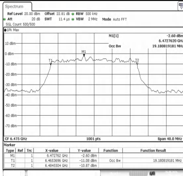
11AX20MIMO-Ant1-6475-PASS
