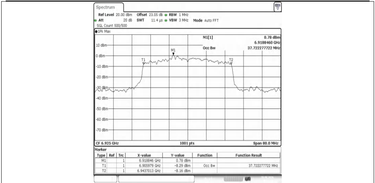
11AX40MIMO-Ant1-6925-PASS
