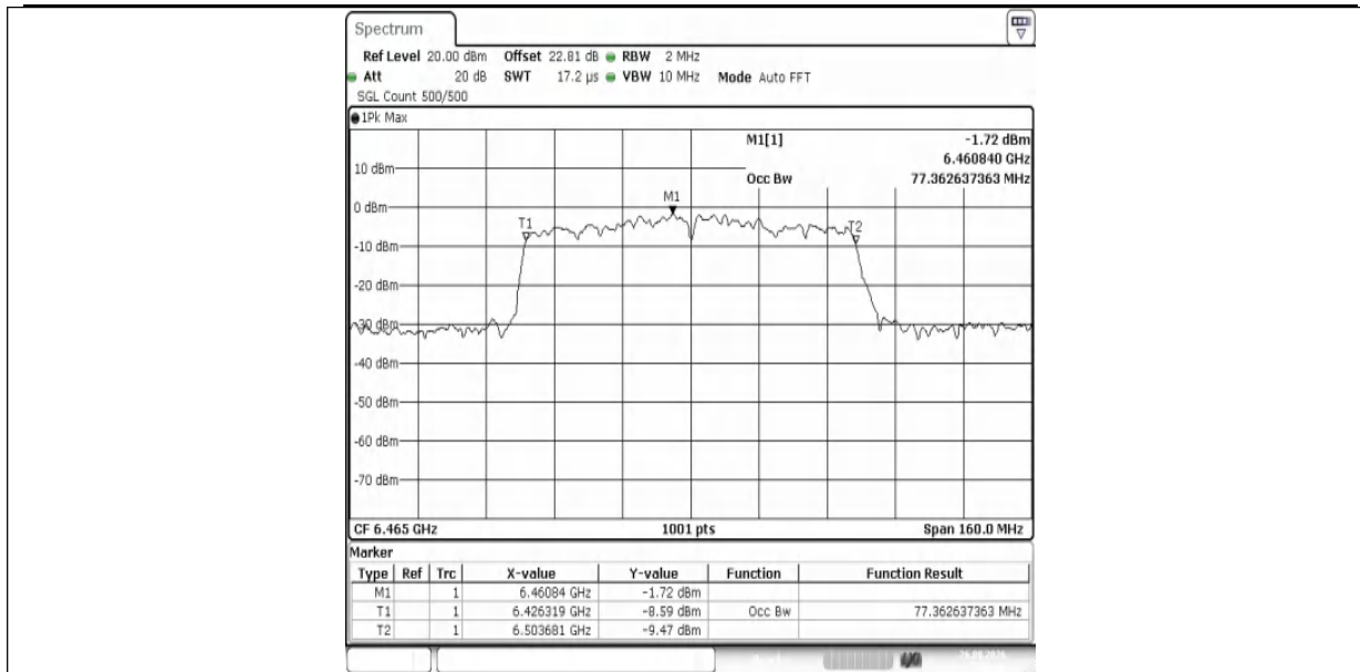
11AX80MIMO-Ant1-6465-PASS
