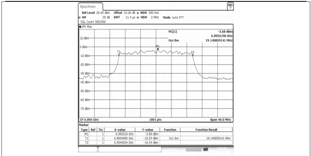
11AX20MIMO-Ant1-6895-PASS
