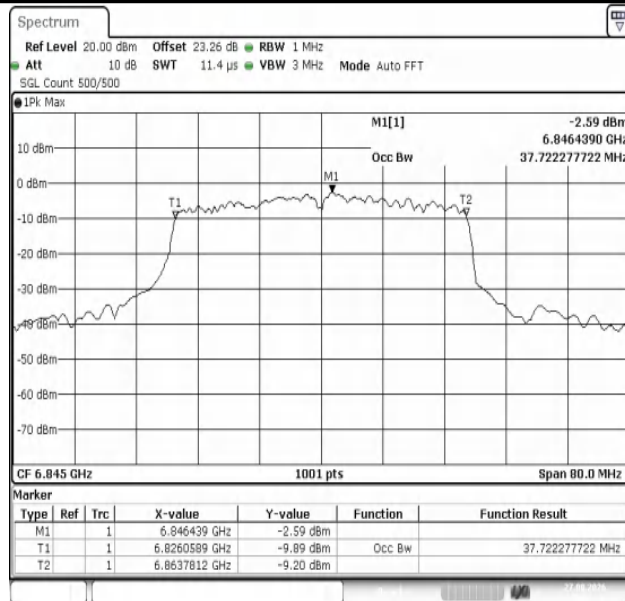
11AX40MIMO-Ant1-6845-PASS
