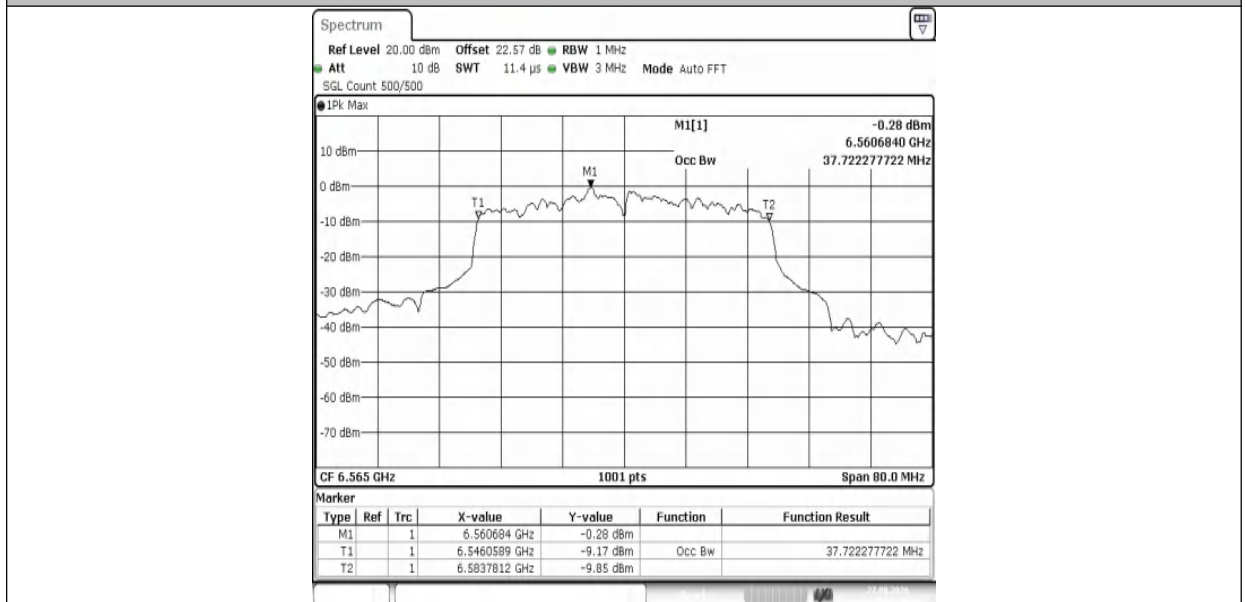
11AX40MIMO-Ant1-6565-PASS
