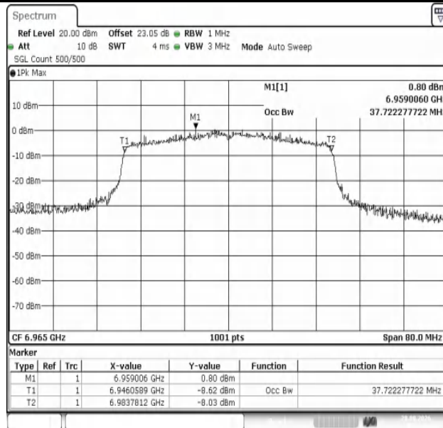
11AX40MIMO-Ant1-6965-PASS
