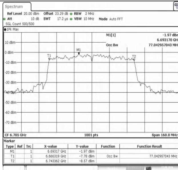
11AX80MIMO-Ant1-6705-PASS
