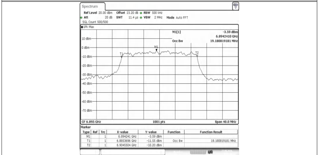
11AX20MIMO-Ant2-6895-PASS
