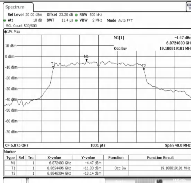
11AX20MIMO-Ant1-6875-PASS
