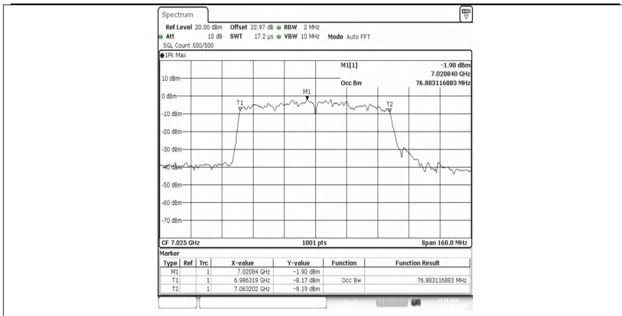
11AX80MIMO-Ant1-7025-PASS
