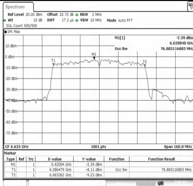
11AX80MIMO-Ant1-6625-PASS
