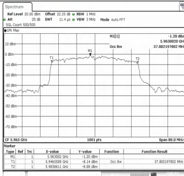
11AX40MIMO-Ant1-5965-PASS
