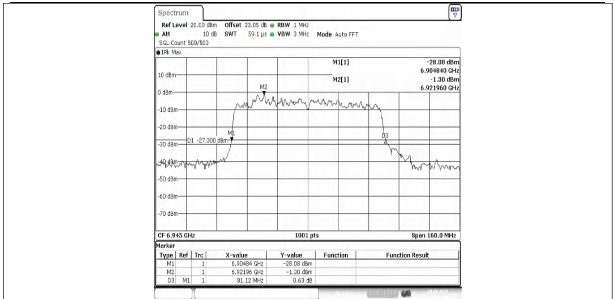
11AX80MIMO-Ant1-6945
