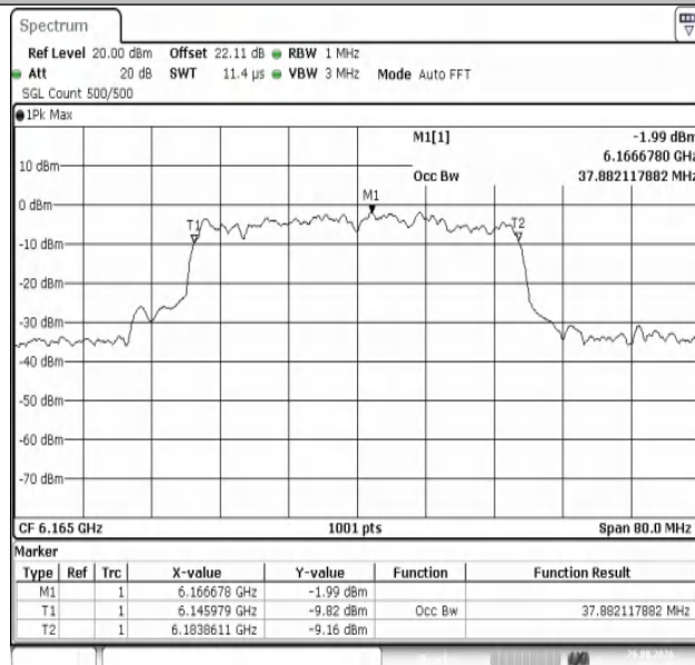
11AX40MIMO-Ant1-6165-PASS
