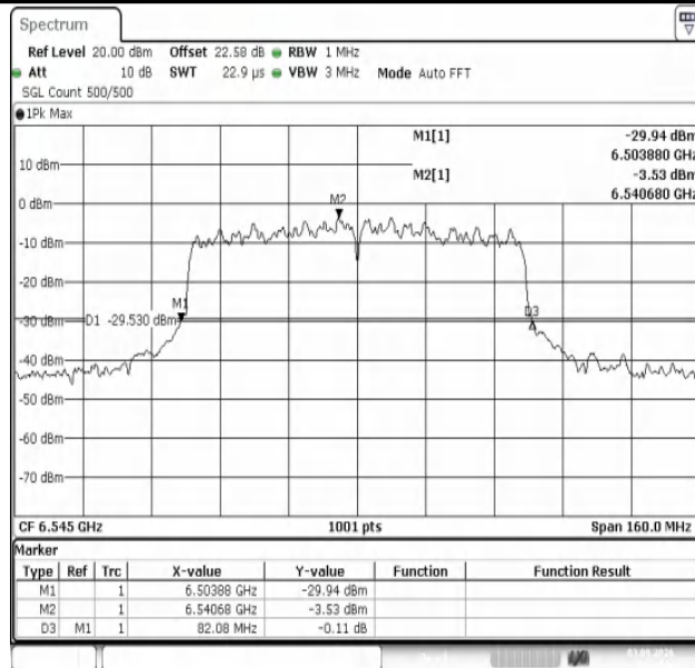
11AX80MIMO-Ant1-6545
