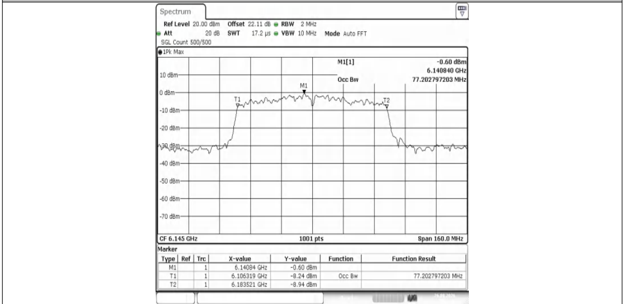
11AX80MIMO-Ant2-6145-PASS
