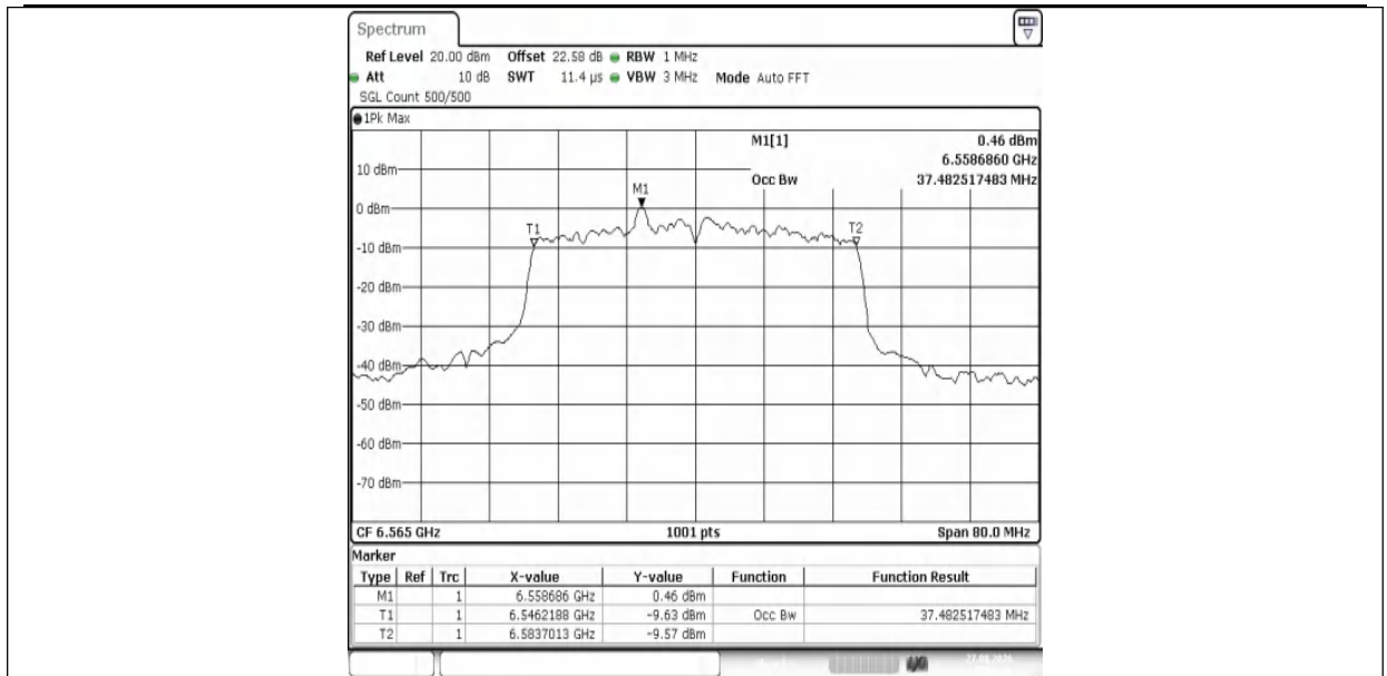
11AX40MIMO-Ant1-6565-PASS
