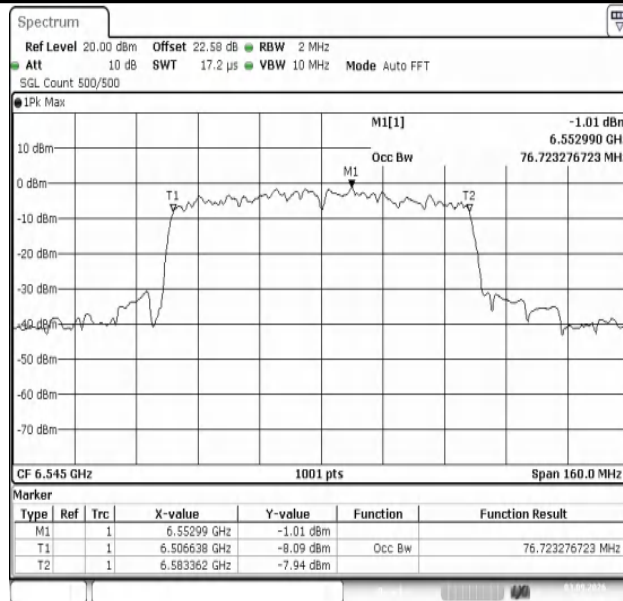
11AX80MIMO-Ant1-6545-PASS
