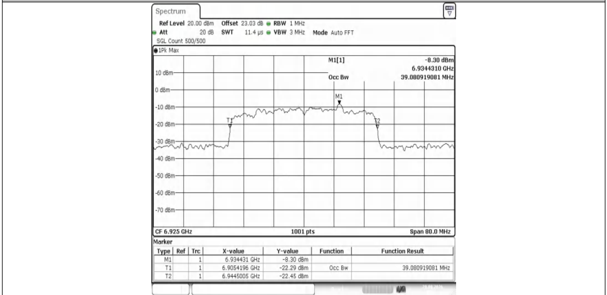
11AX40MIMO-Ant2-6925-PASS
