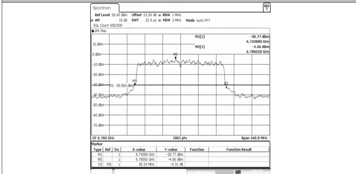
11AX80MIMO-Ant1-6785
