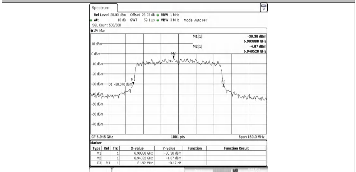
11AX80MIMO-Ant1-6945
