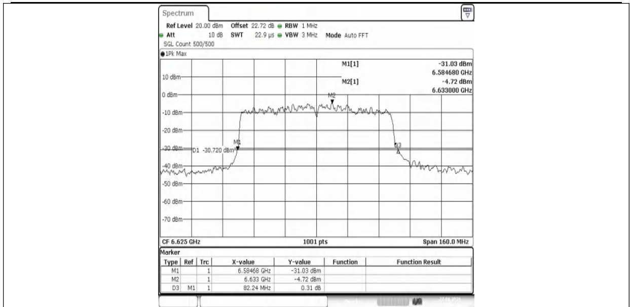
11AX80MIMO-Ant1-6625
