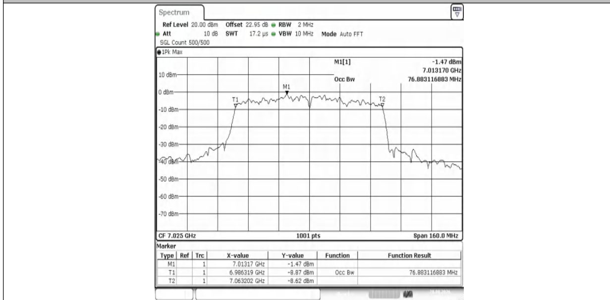
11AX80MIMO-Ant2-7025-PASS
