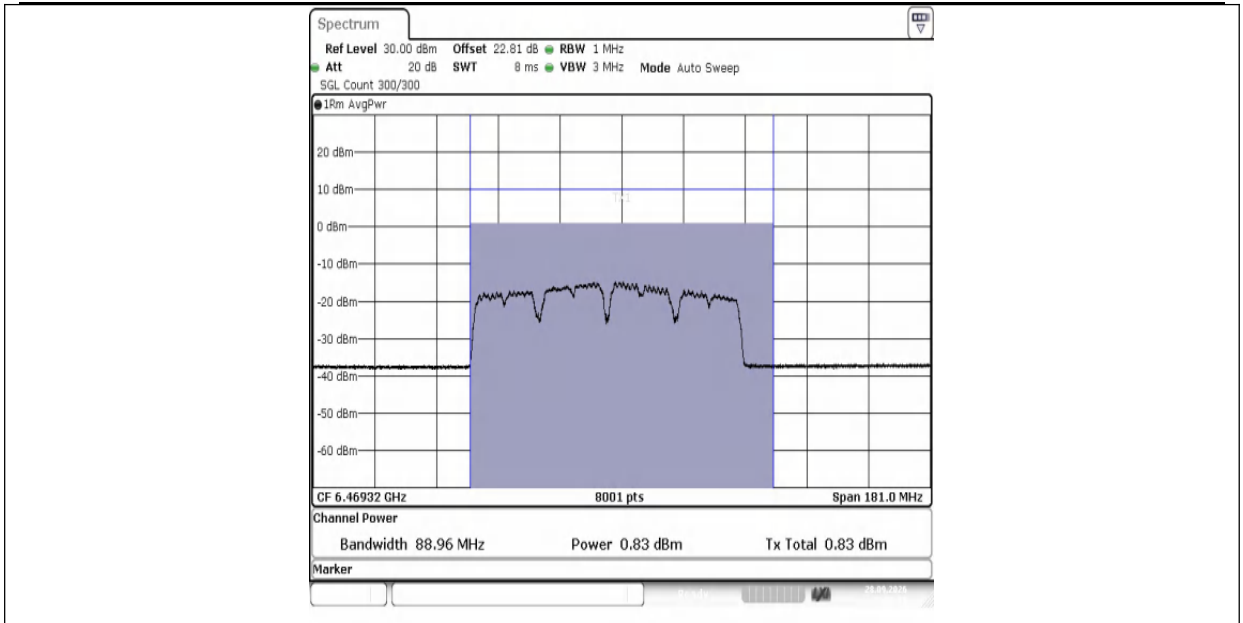
11AX80MIMO-Ant1-6465-PASS
