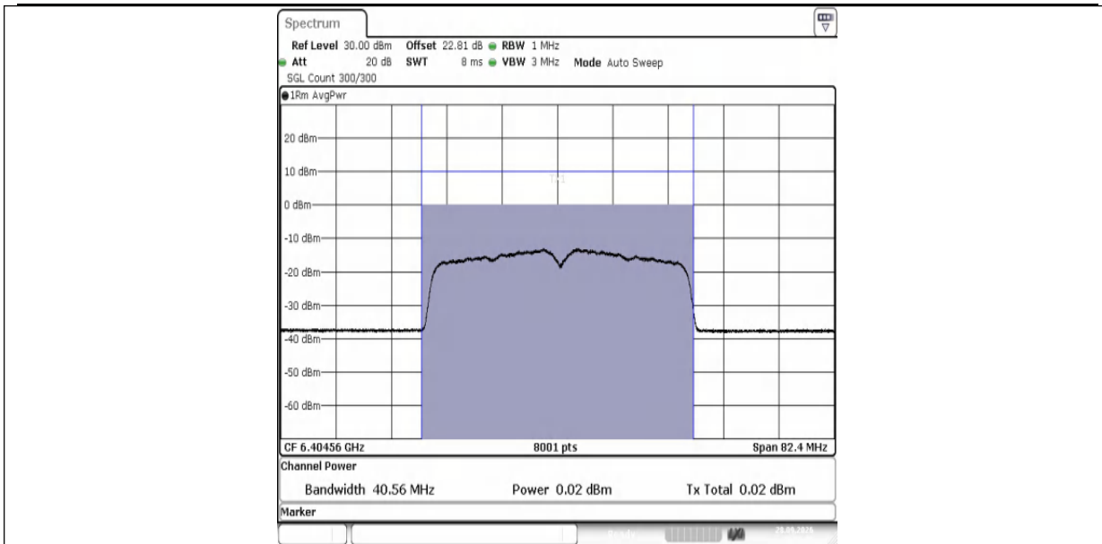
11AX40MIMO-Ant1-6405-PASS
