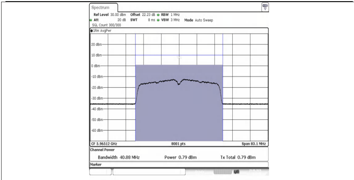
11AX40MIMO-Ant1-5965-PASS
