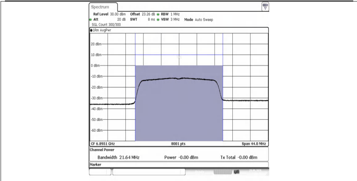
11AX20MIMO-Ant1-6895-PASS
