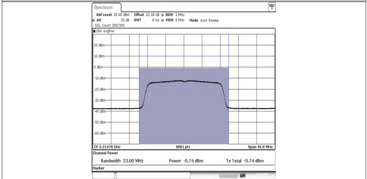
11AX20MIMO-Ant1-6515-PASS
