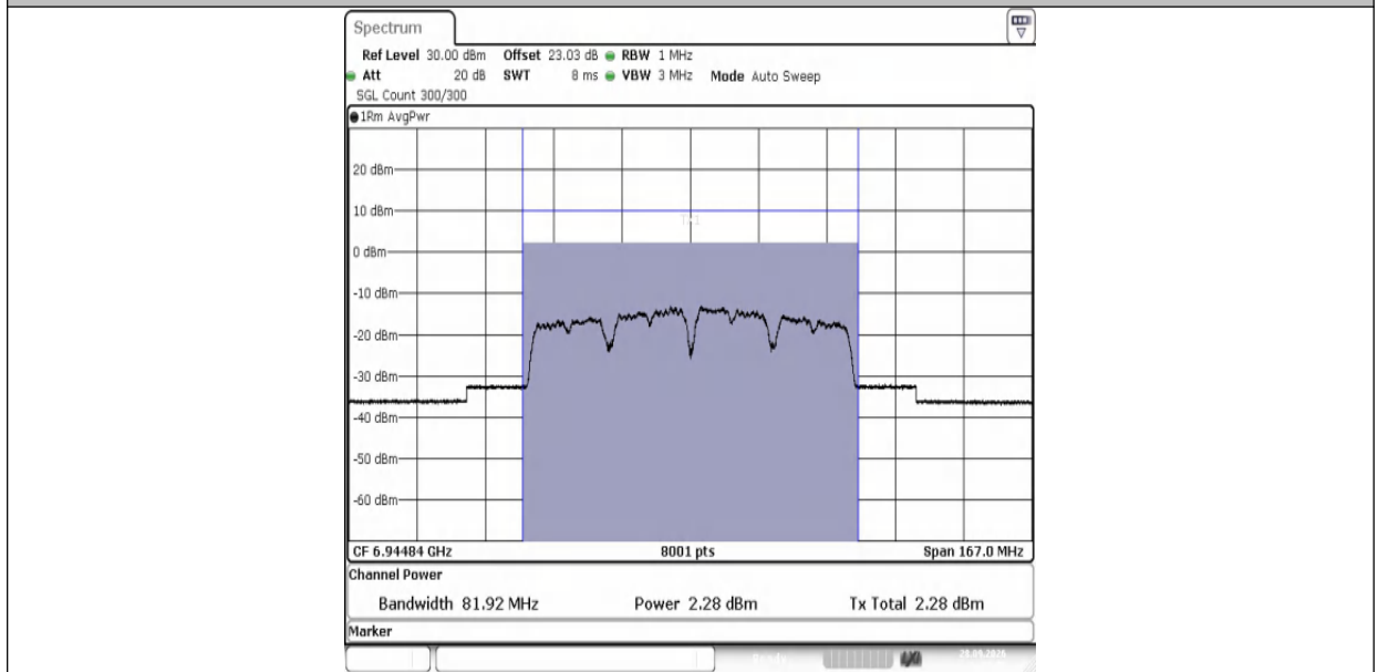
11AX80MIMO-Ant2-6945-PASS
