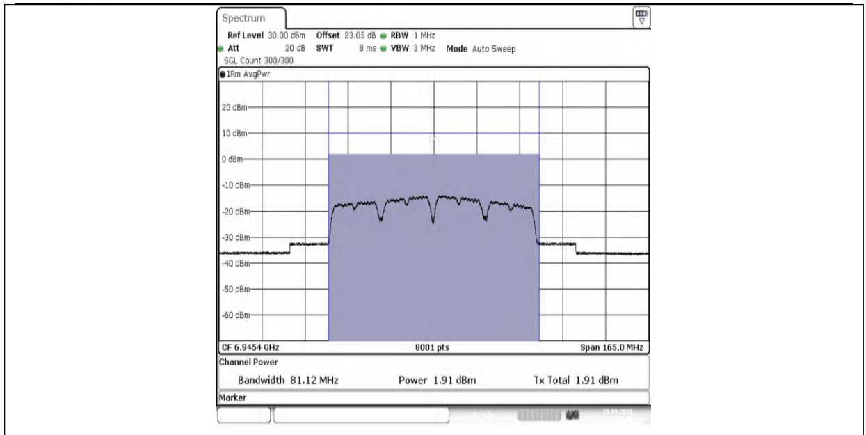
11AX80MIMO-Ant1-6945-PASS
