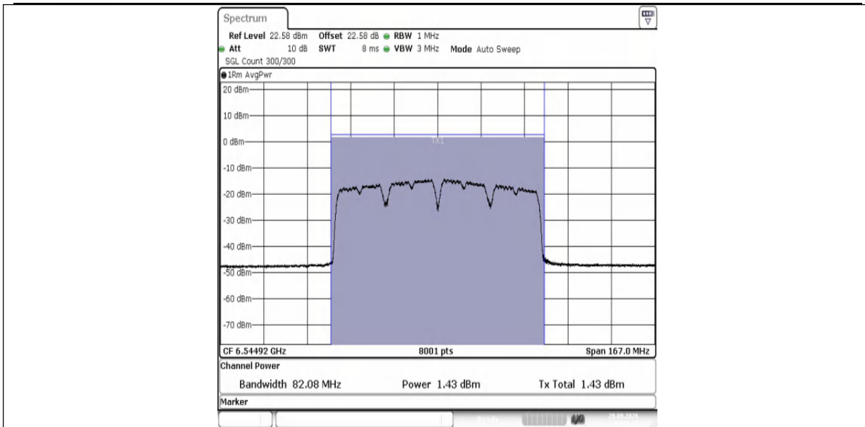
11AX80MIMO-Ant1-6545-PASS
