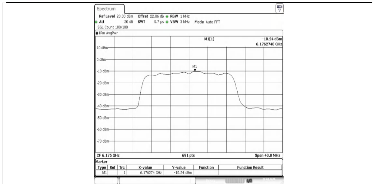
11AX20MIMO-Ant1-6175-PASS
