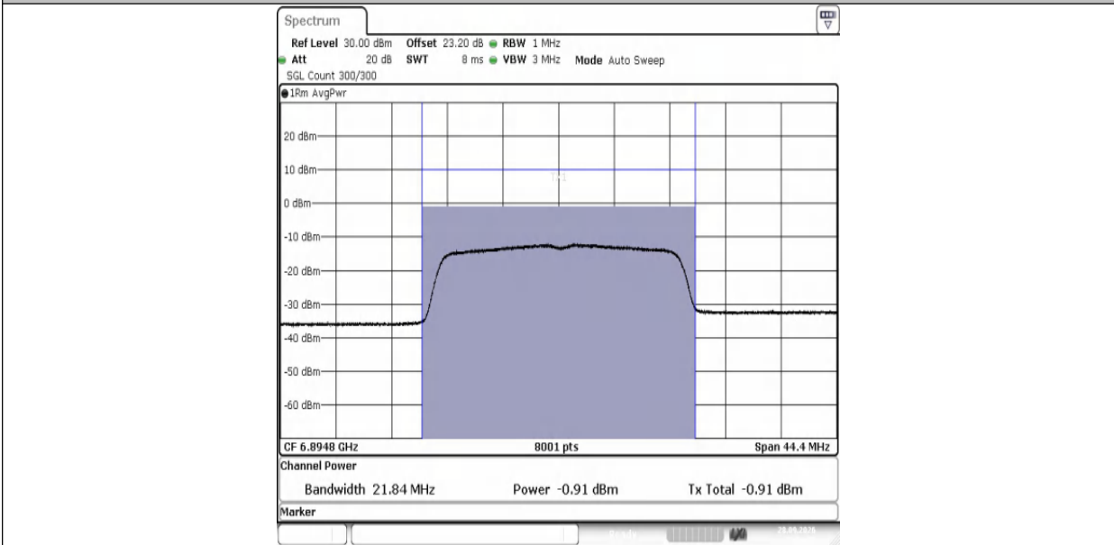
11AX20MIMO-Ant2-6895-PASS
