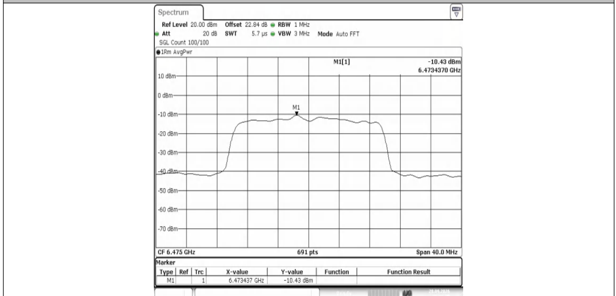
11AX20MIMO-Ant1-6475-PASS
