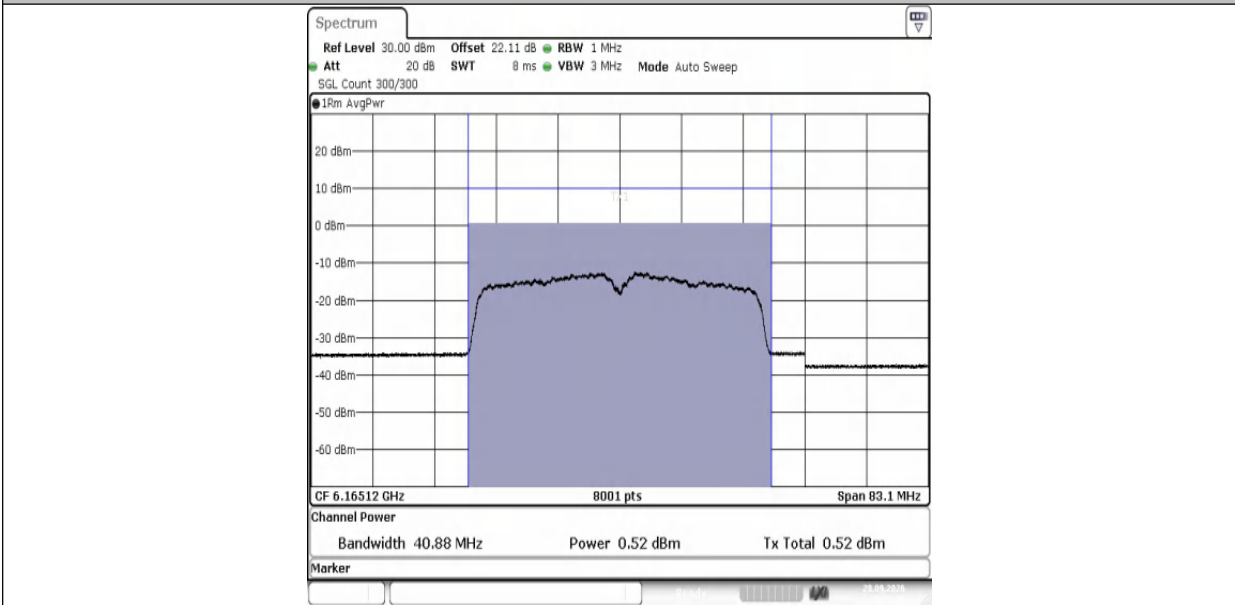
11AX40MIMO-Ant2-6165-PASS
