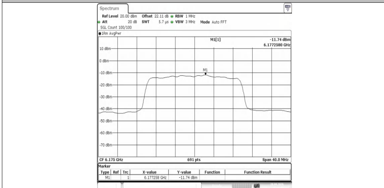
11AX20MIMO-Ant1-6175-PASS
