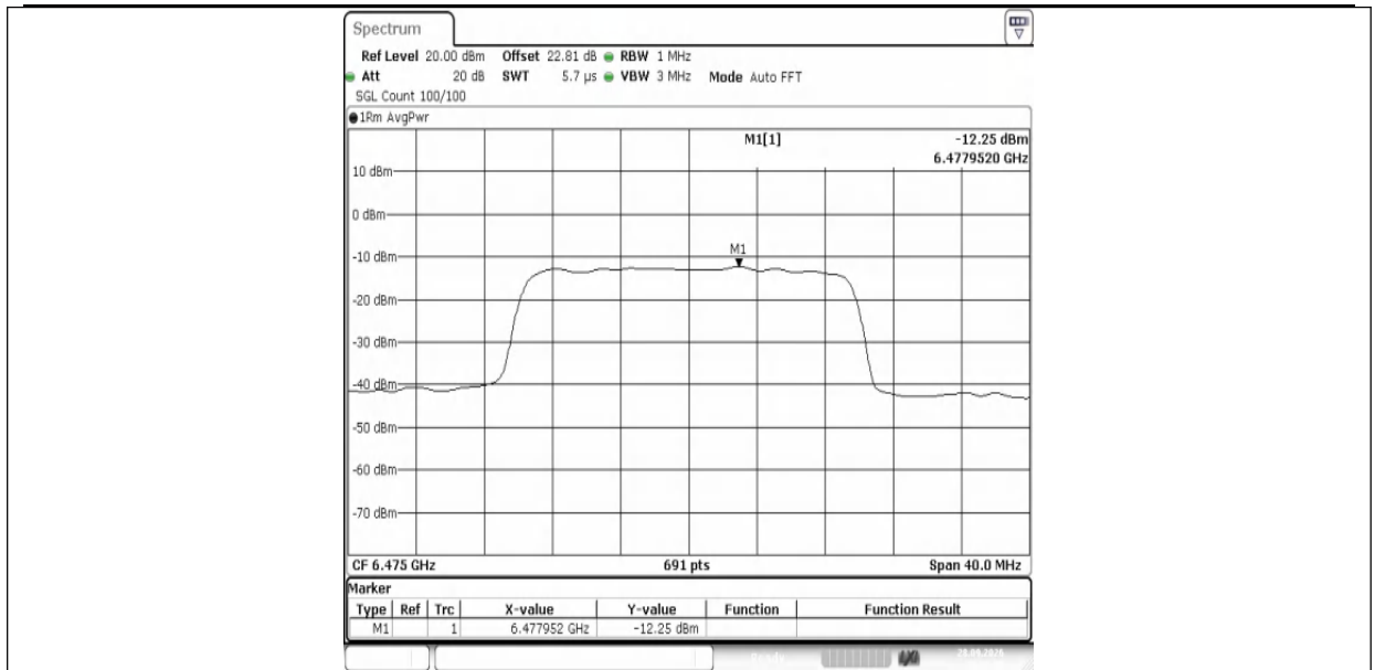
11AX20MIMO-Ant1-6475-PASS
