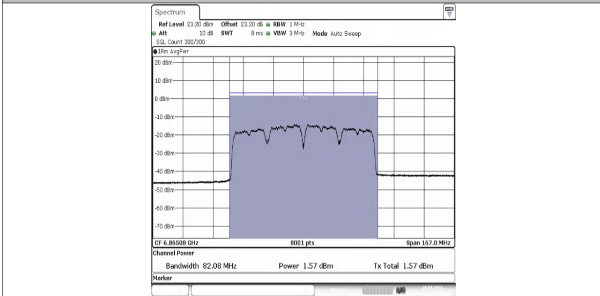
11AX80MIMO-Ant2-6865-PASS
