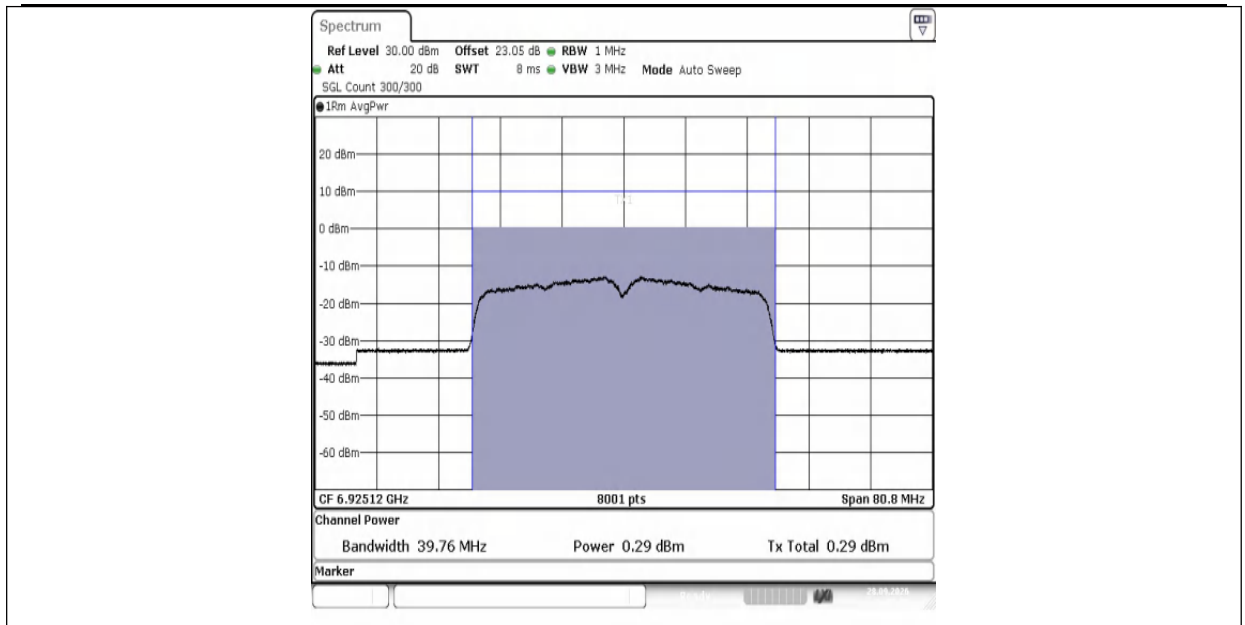
11AX40MIMO-Ant1-6925-PASS
