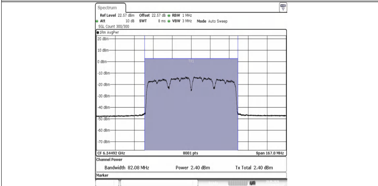
11AX80MIMO-Ant2-6545-PASS
