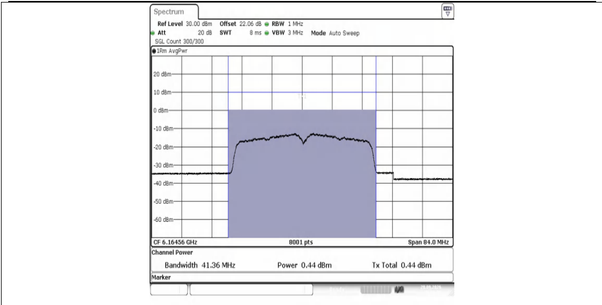
11AX40MIMO-Ant1-6165-PASS
