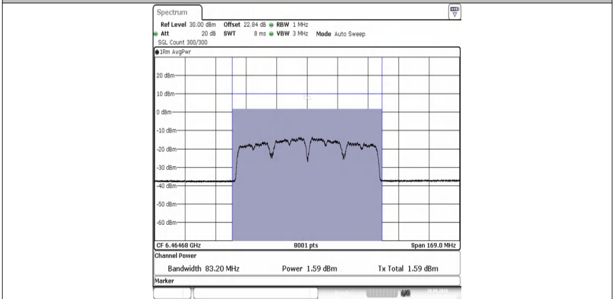
11AX80MIMO-Ant2-6465-PASS
