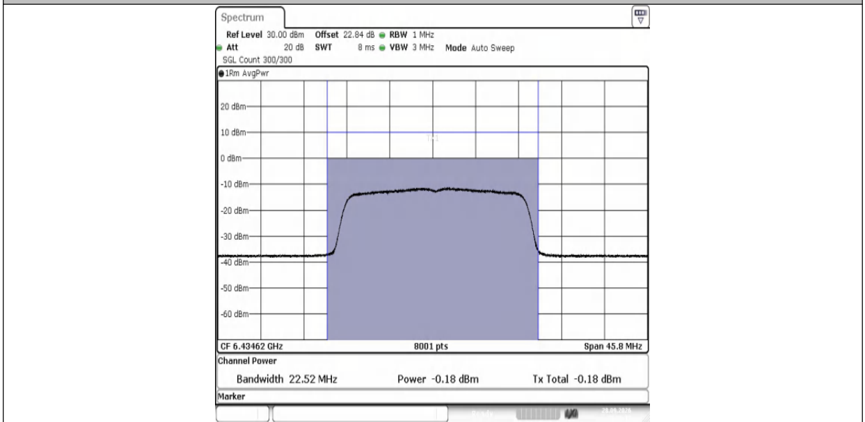
11AX20MIMO-Ant1-6435-PASS
