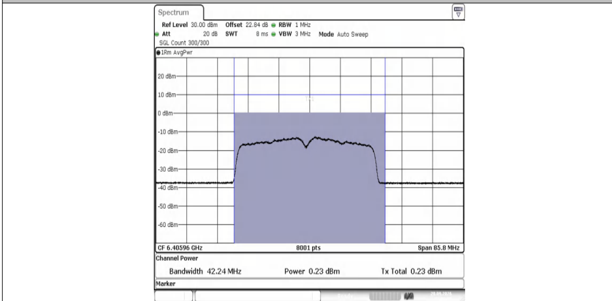
11AX40MIMO-Ant2-6405-PASS
