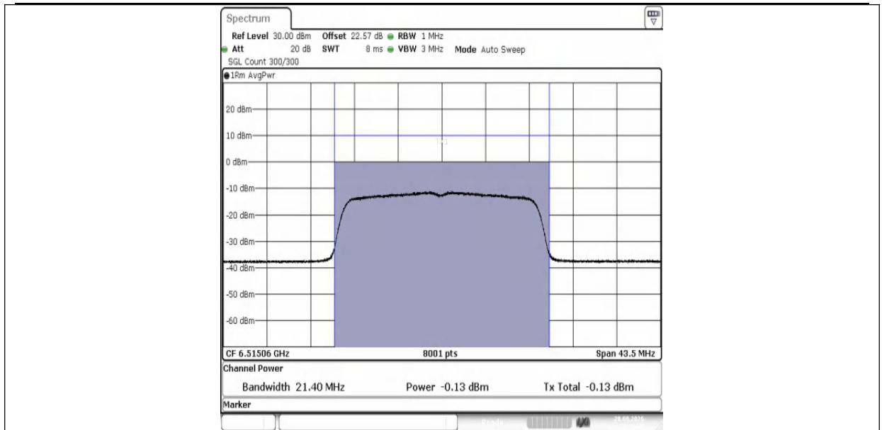
11AX20MIMO-Ant2-6515-PASS
