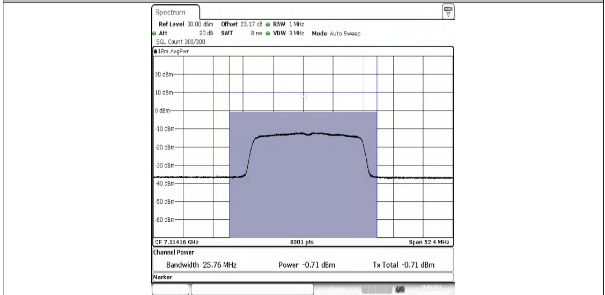
11AX20MIMO-Ant2-7115-PASS
