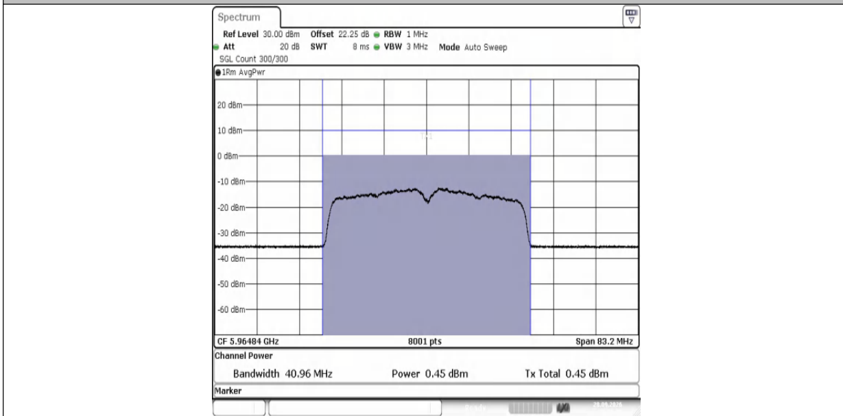
11AX40MIMO-Ant2-5965-PASS
