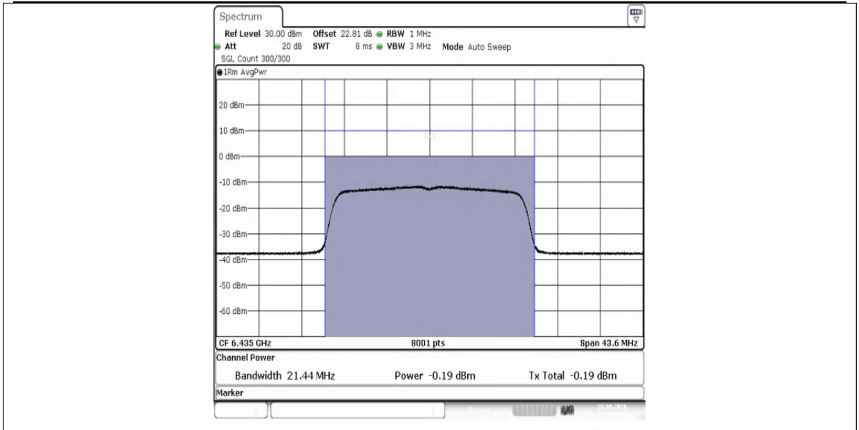
11AX20MIMO-Ant1-6435-PASS
