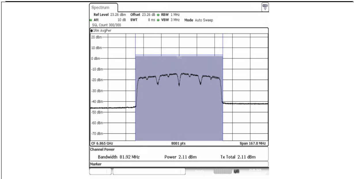
11AX80MIMO-Ant1-6865-PASS
