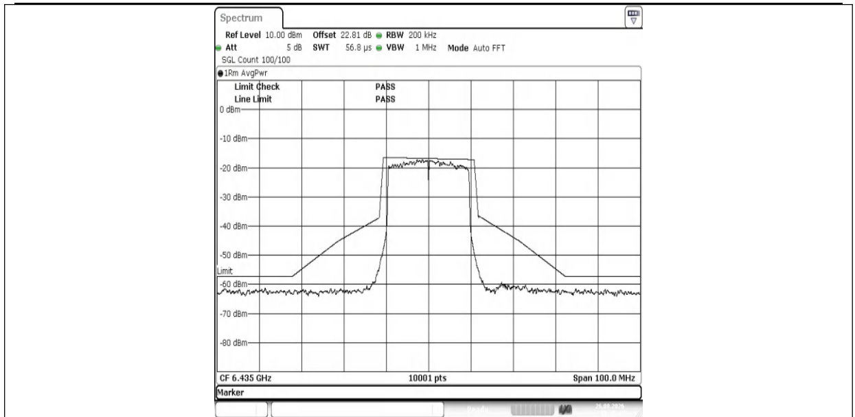
NTNV-11AX20MIMO-Ant1-6435-PASS
