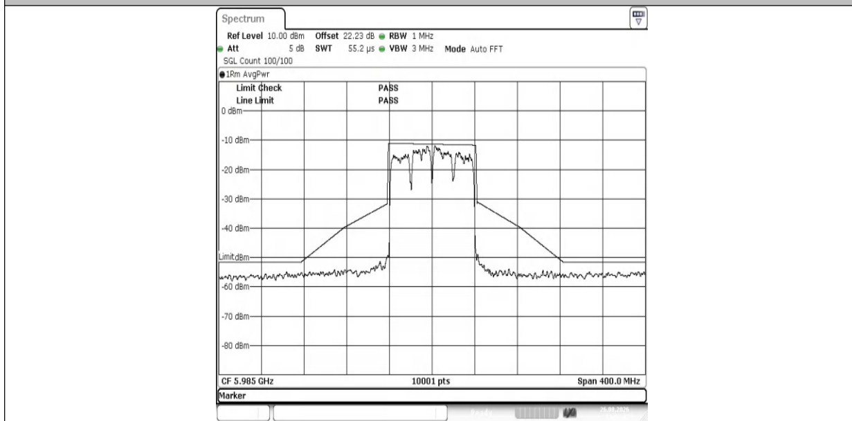
NTNV-11AX80MIMO-Ant2-5985-PASS
