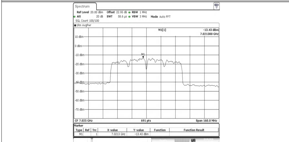
11AX80MIMO-Ant1-7025-PASS
