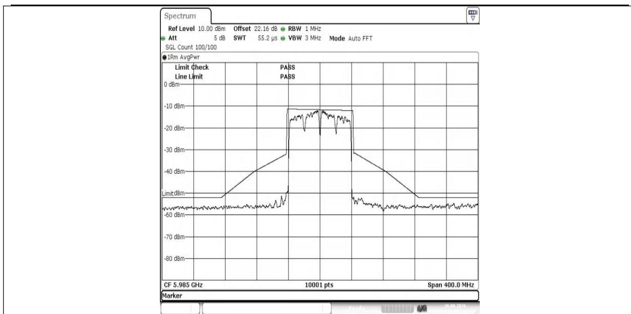
NTNV-11AX80MIMO-Ant1-5985-PASS
