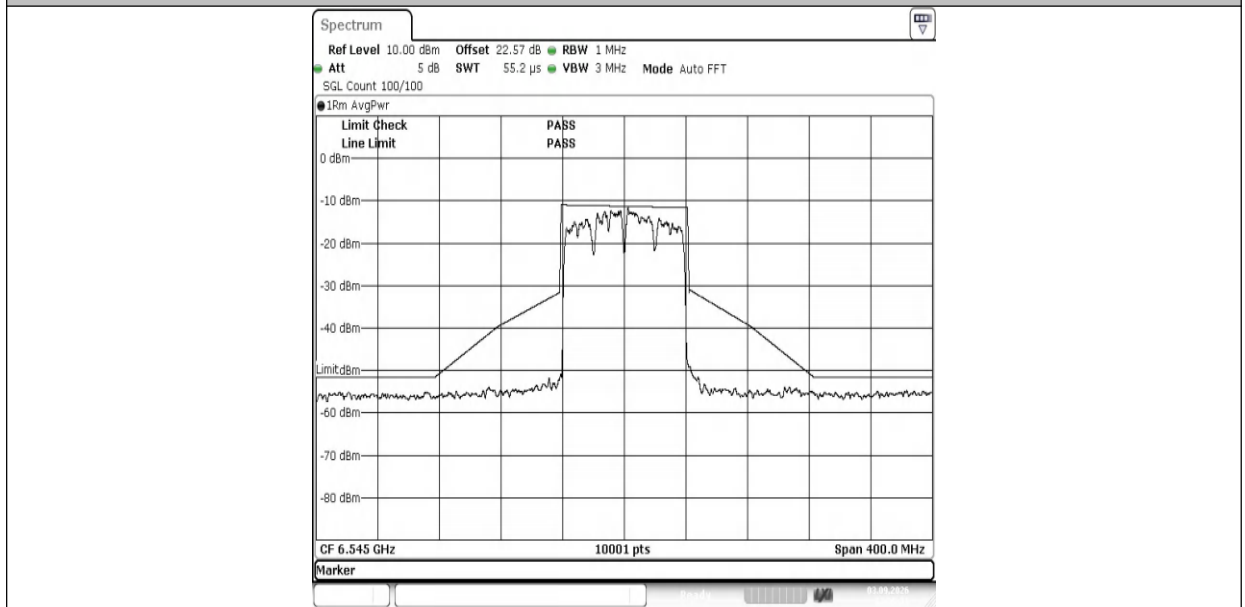
NTNV-11AX80MIMO-Ant2-6545-PASS
