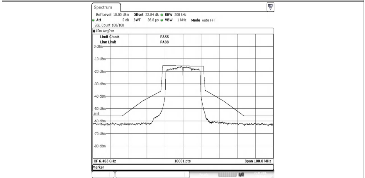
NTNV-11AX20MIMO-Ant2-6435-PASS
