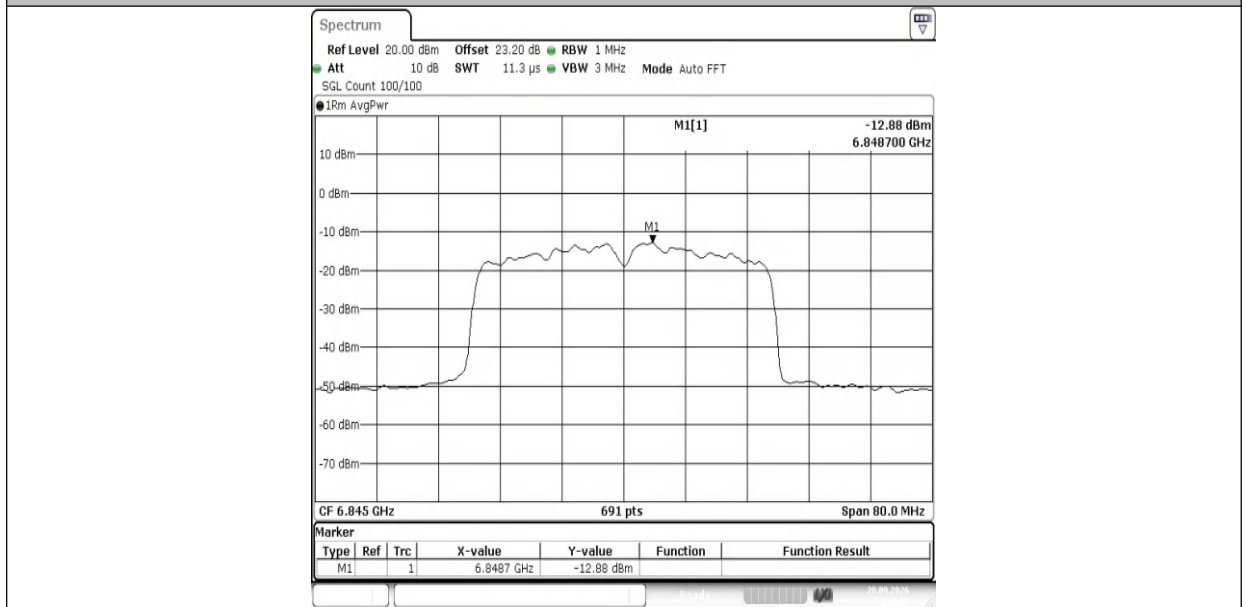
11AX40MIMO-Ant2-6845-PASS
