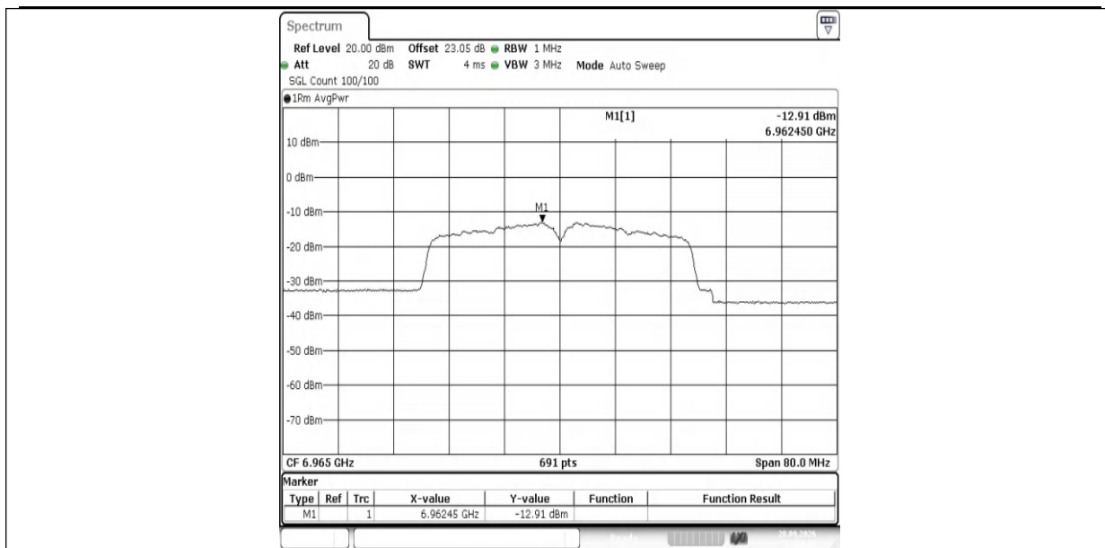
11AX40MIMO-Ant1-6965-PASS
