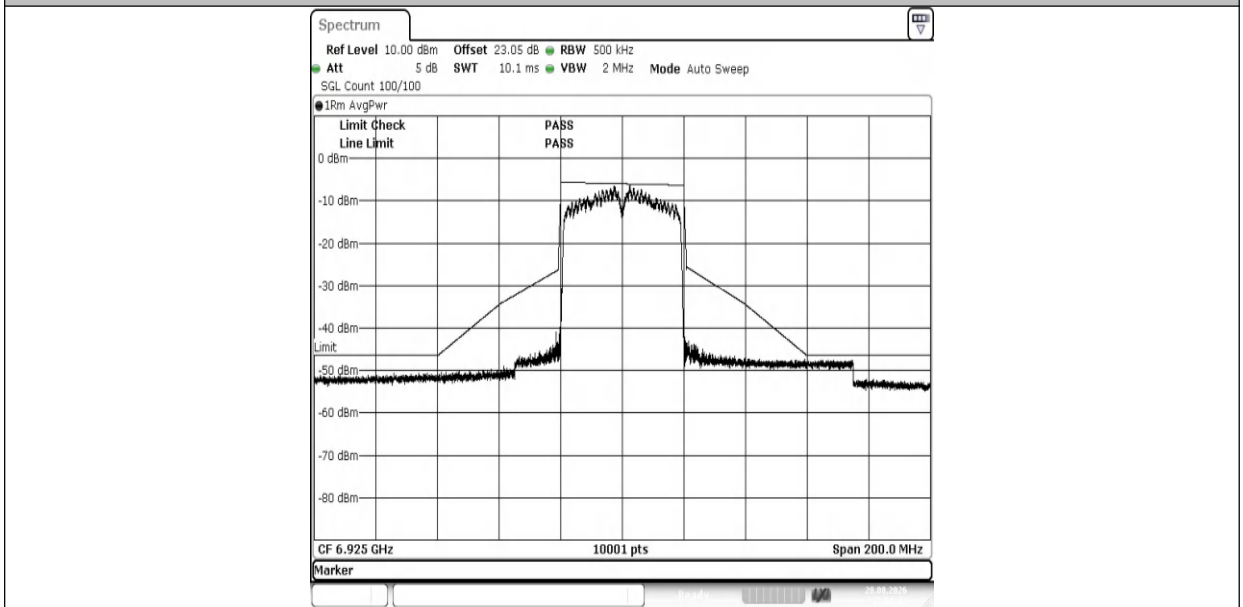
NTNV-11AX40MIMO-Ant1-6925-PASS
