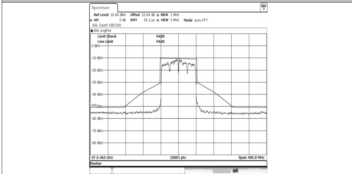
NTNV-11AX80MIMO-Ant2-6465-PASS
