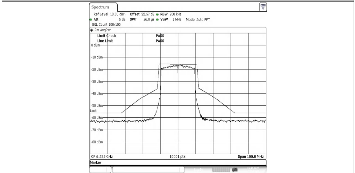
NTNV-11AX20MIMO-Ant2-6535-PASS
