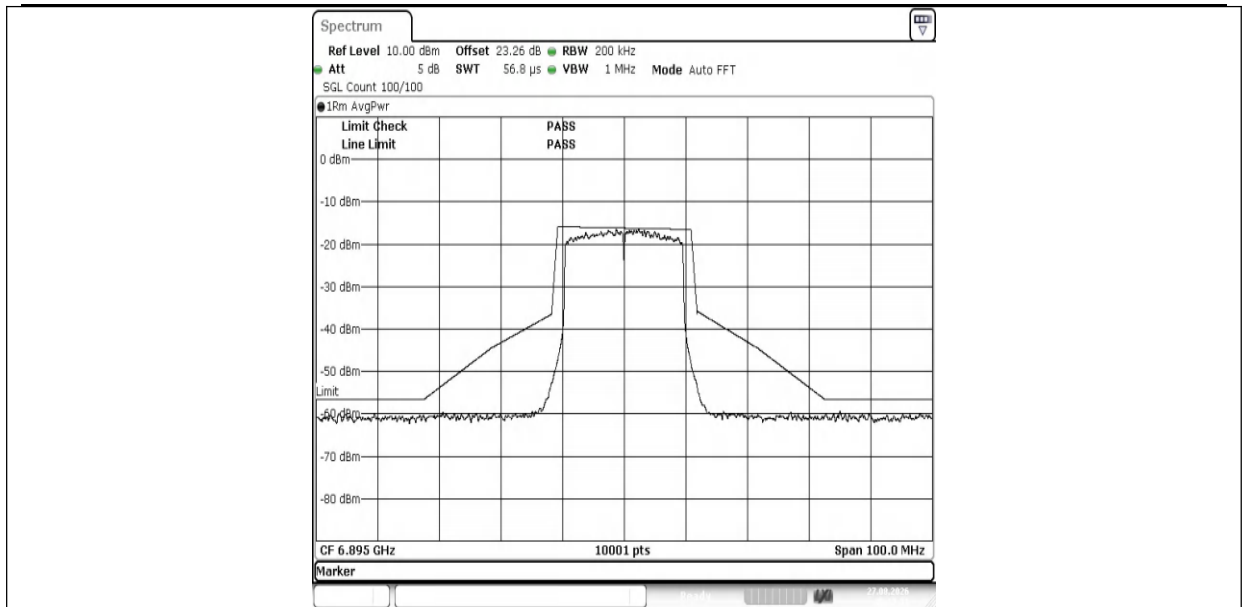
NTNV-11AX20MIMO-Ant1-6895-PASS
