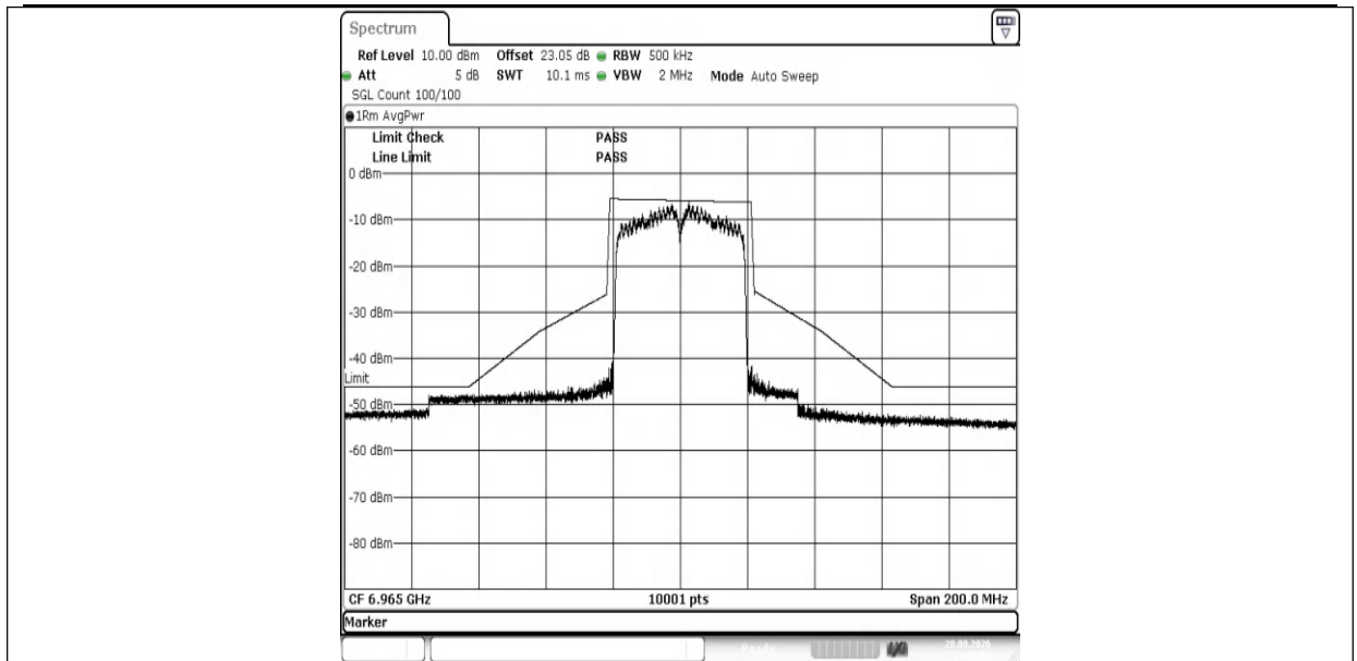
NTNV-11AX40MIMO-Ant1-6965-PASS
