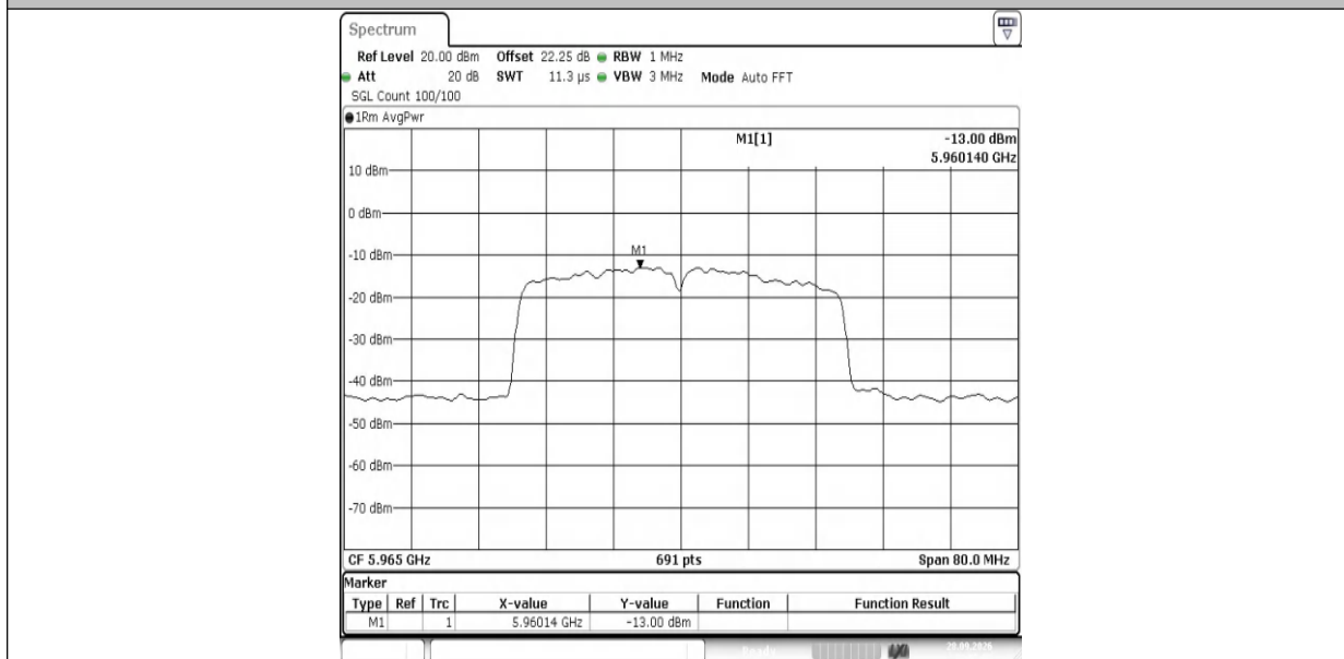
11AX40MIMO-Ant1-5965-PASS
