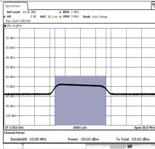
11AX20SISO-Ant1-5955-5955-PASS
