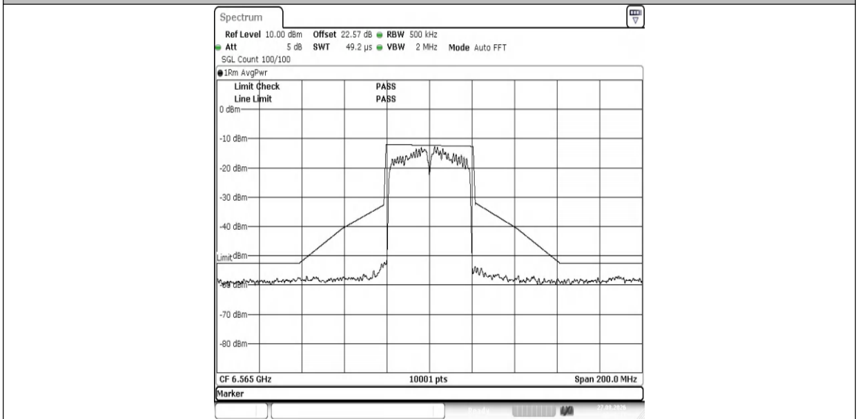
NTNV-11AX40MIMO-Ant2-6565-PASS
