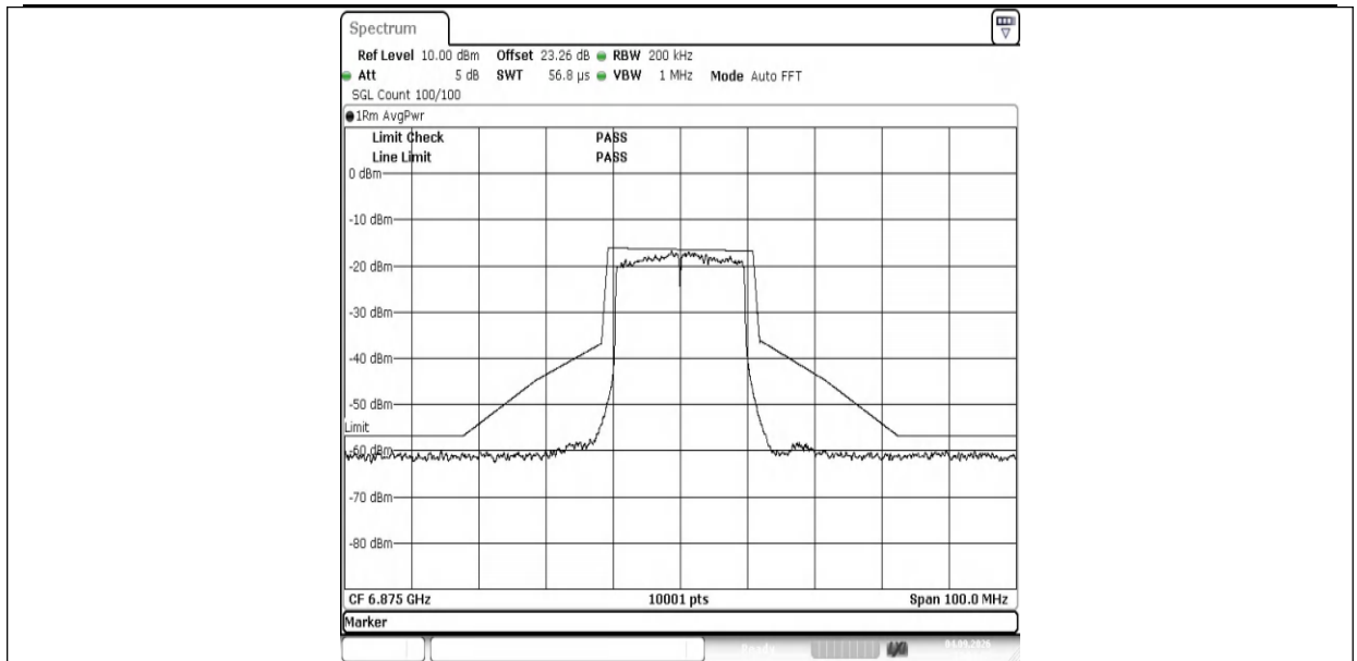
NTNV-11AX20MIMO-Ant1-6875-PASS
