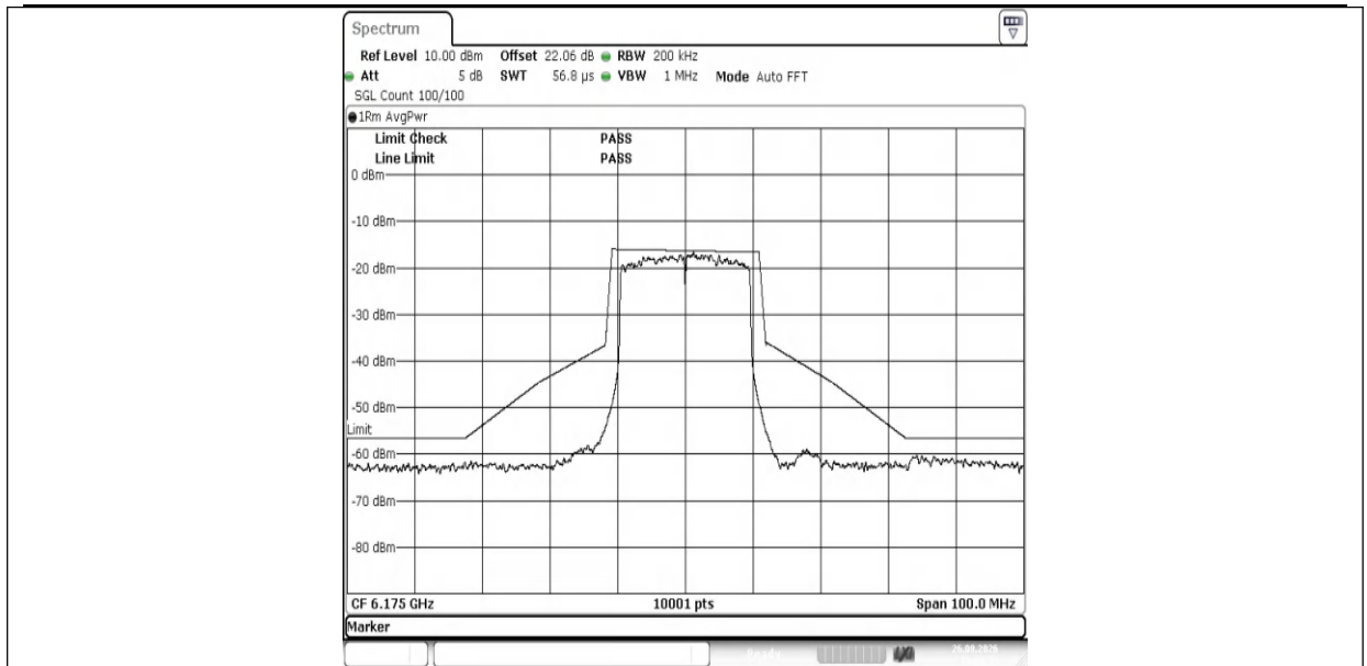
NTNV-11AX20MIMO-Ant1-6175-PASS
