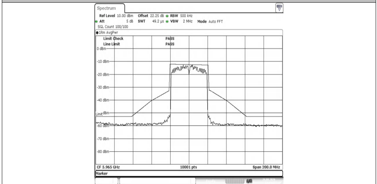
NTNV-11AX40MIMO-Ant1-5965-PASS
