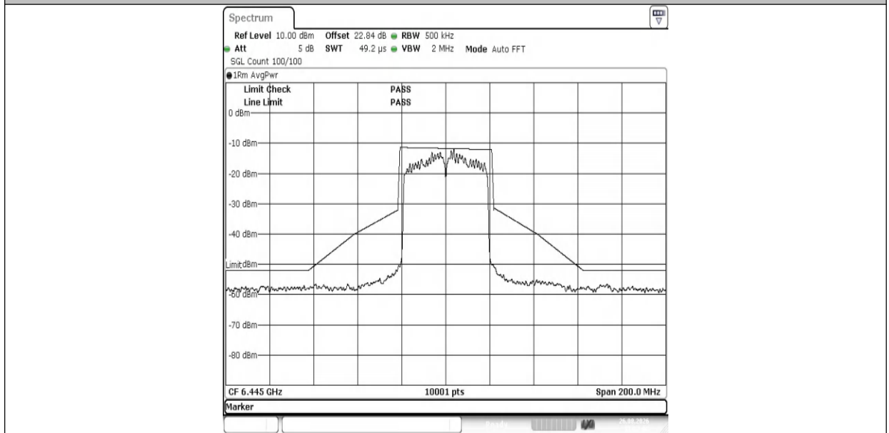
NTNV-11AX40MIMO-Ant2-6445-PASS
