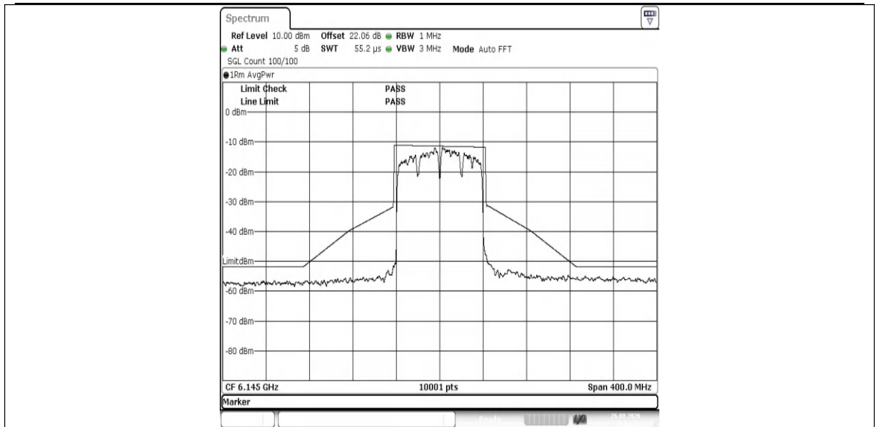
NTNV-11AX80MIMO-Ant1-6145-PASS
