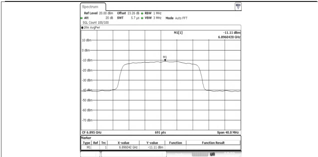
11AX20MIMO-Ant1-6895-PASS
