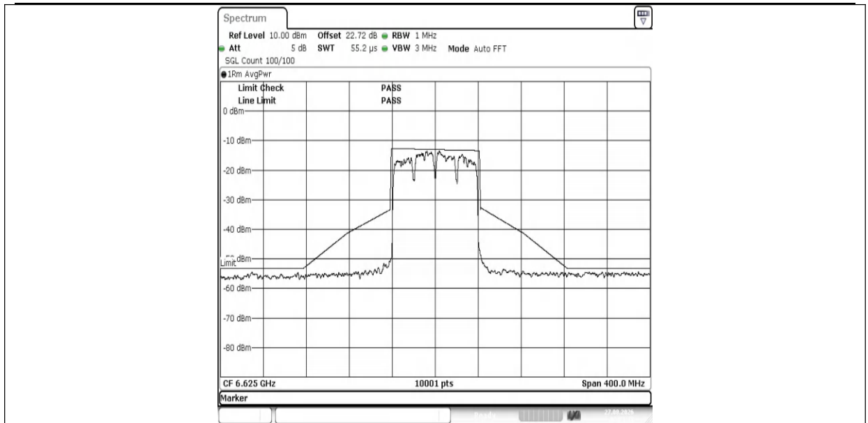
NTNV-11AX80MIMO-Ant1-6625-PASS
