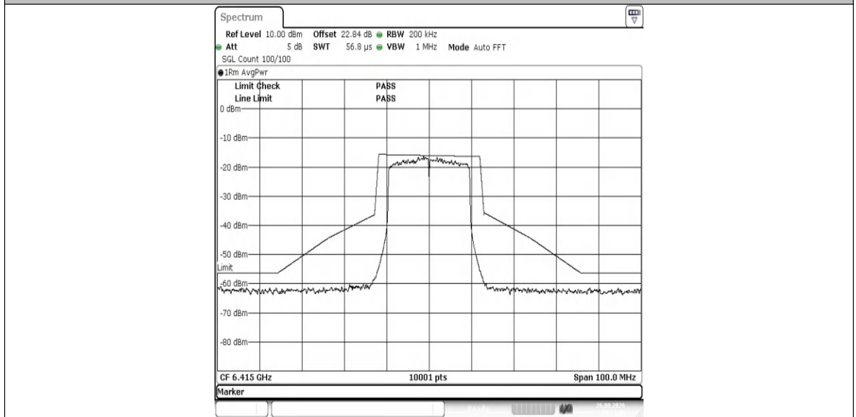
NTNV-11AX20MIMO-Ant1-6415-PASS
