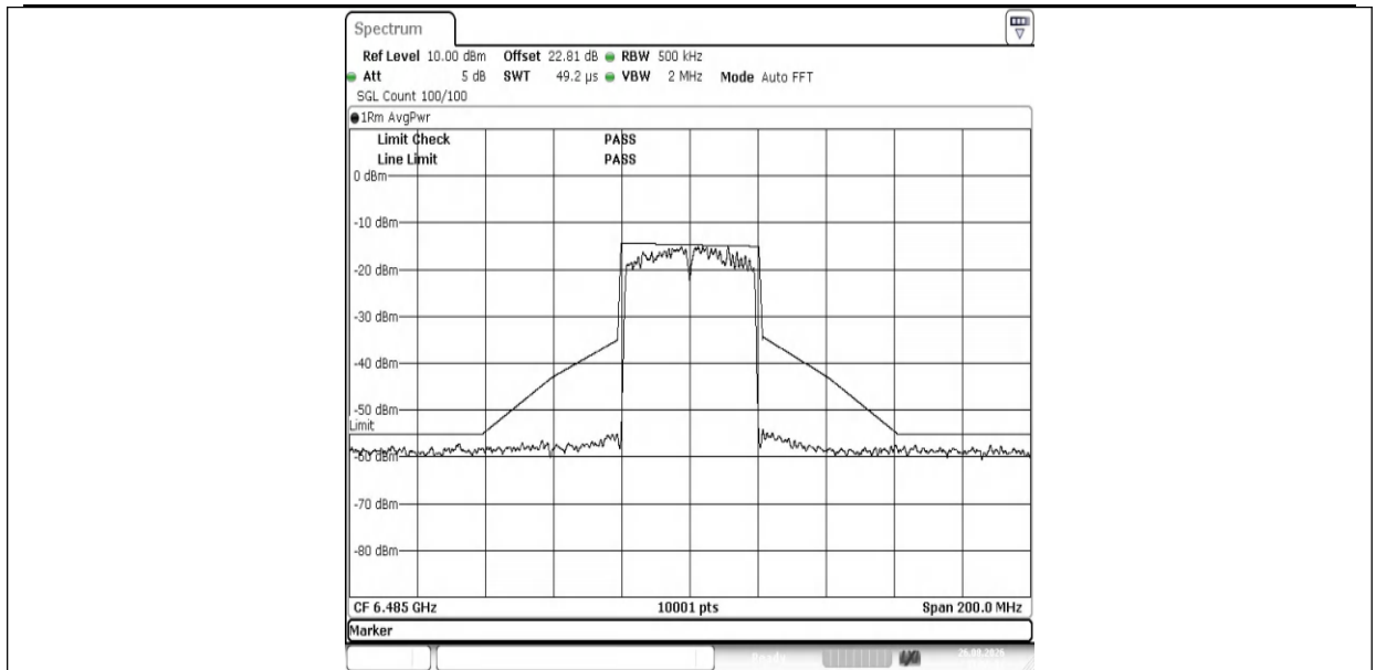
NTNV-11AX40MIMO-Ant1-6485-PASS
