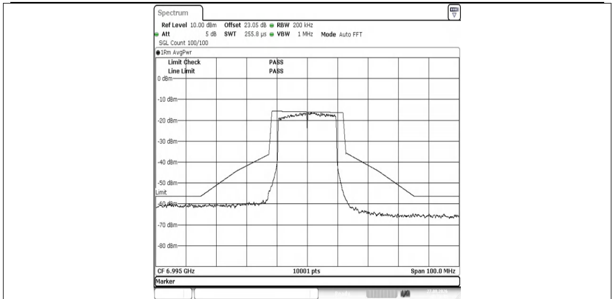
NTNV-11AX20MIMO-Ant1-6995-PASS
