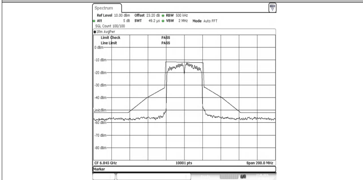
NTNV-11AX40MIMO-Ant2-6845-PASS
