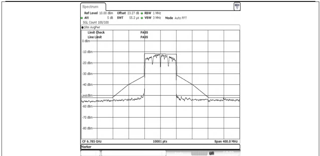
NTNV-11AX80MIMO-Ant1-6785-PASS
