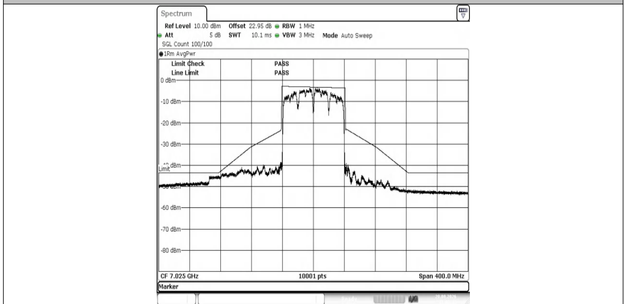
NTNV-11AX80MIMO-Ant1-7025-PASS
