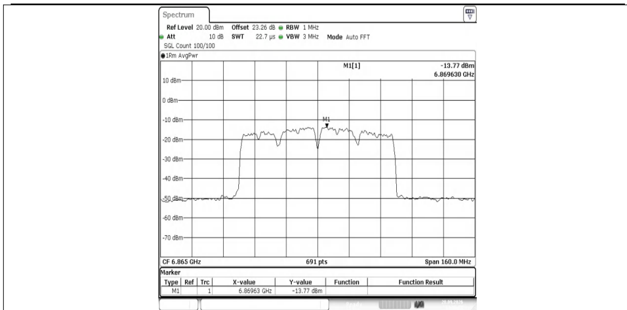
11AX80MIMO-Ant1-6865-PASS
