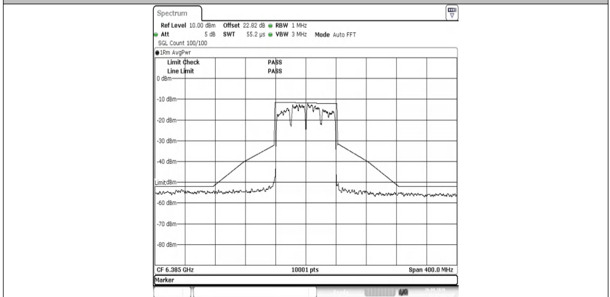
NTNV-11AX80MIMO-Ant1-6385-PASS
