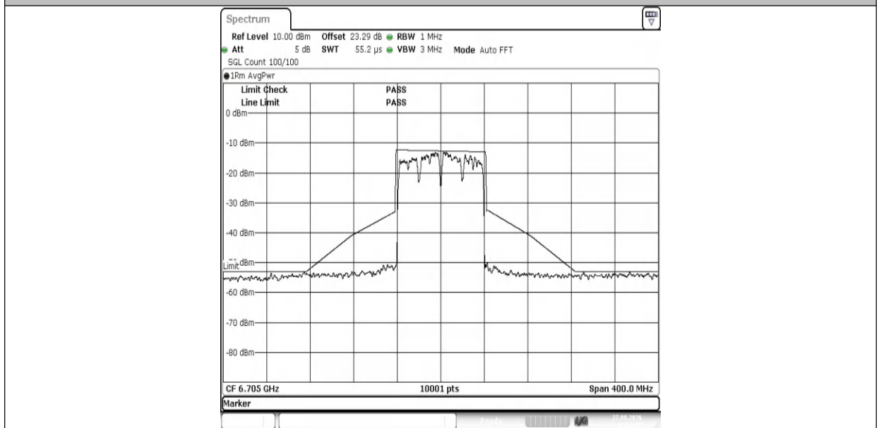
NTNV-11AX80MIMO-Ant1-6705-PASS
