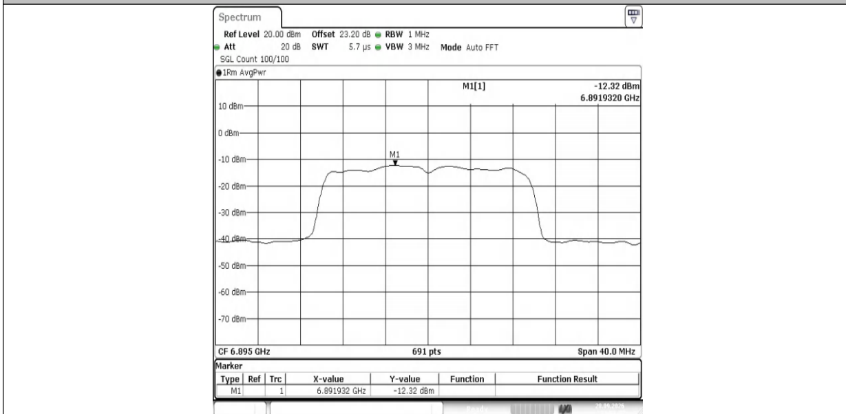
11AX20MIMO-Ant1-6895-PASS
