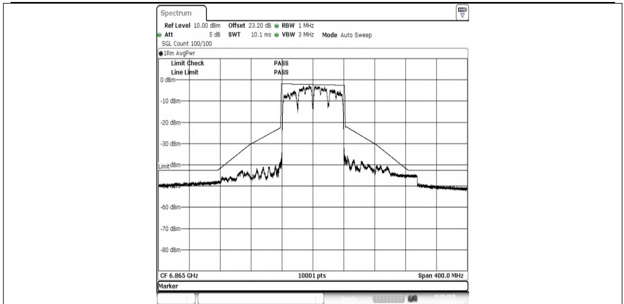
NTNV-11AX80MIMO-Ant2-6865-PASS
