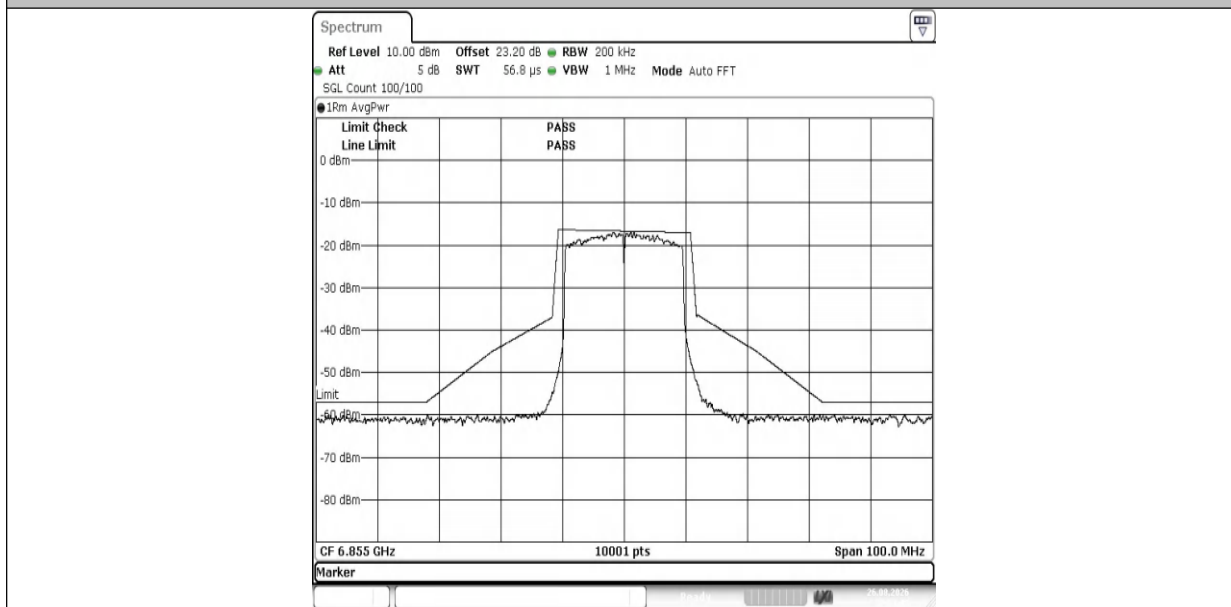
NTNV-11AX20MIMO-Ant2-6855-PASS
