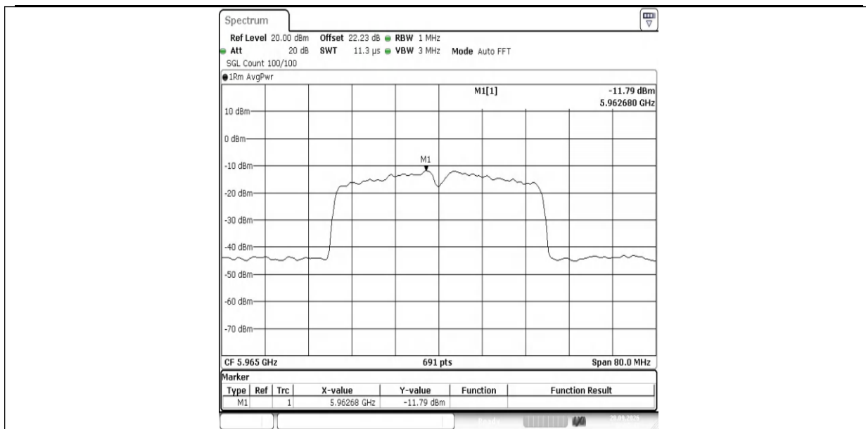
11AX40MIMO-Ant1-5965-PASS
