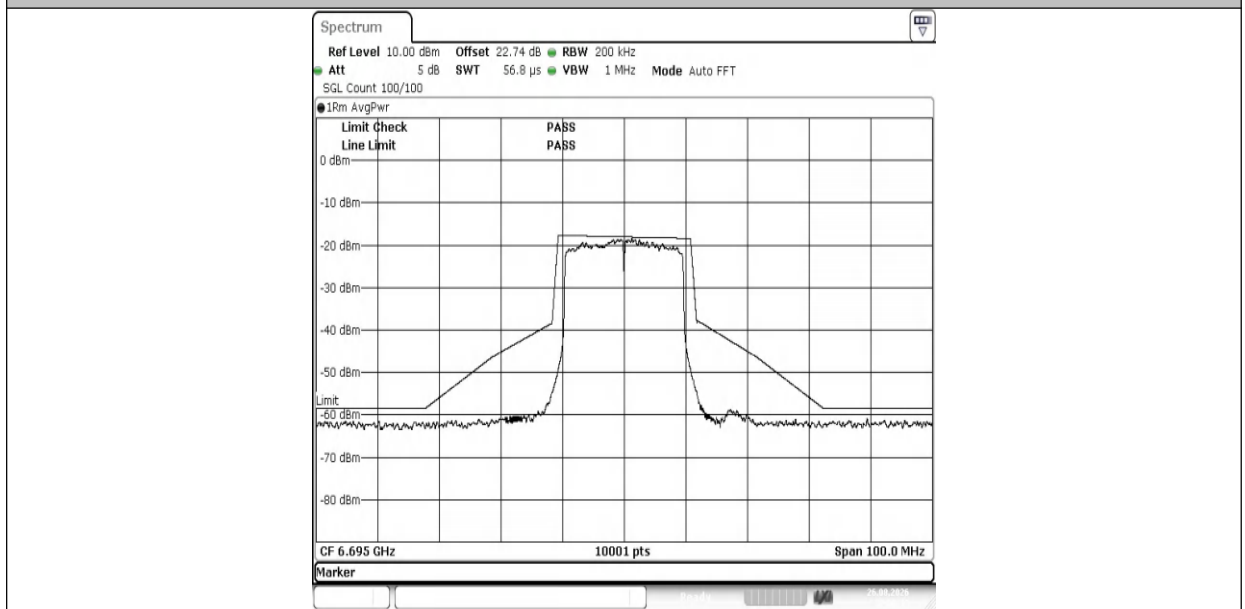
NTNV-11AX20MIMO-Ant1-6695-PASS
