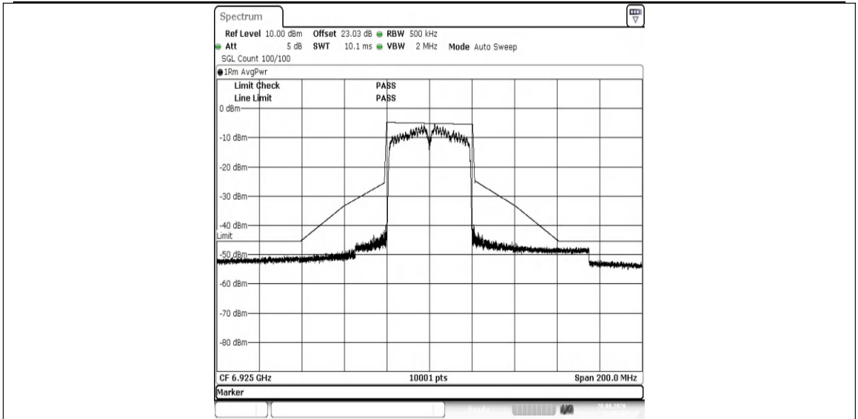
NTNV-11AX40MIMO-Ant2-6925-PASS
