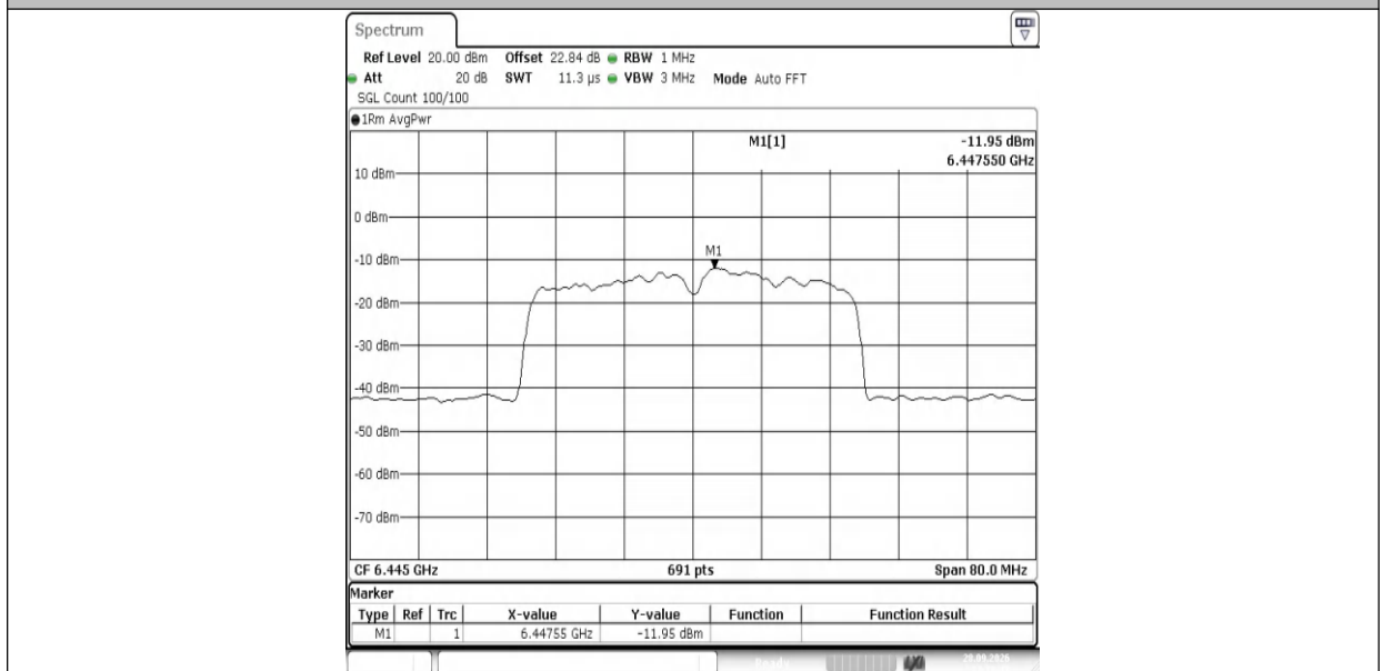
11AX40MIMO-Ant1-6445-PASS
