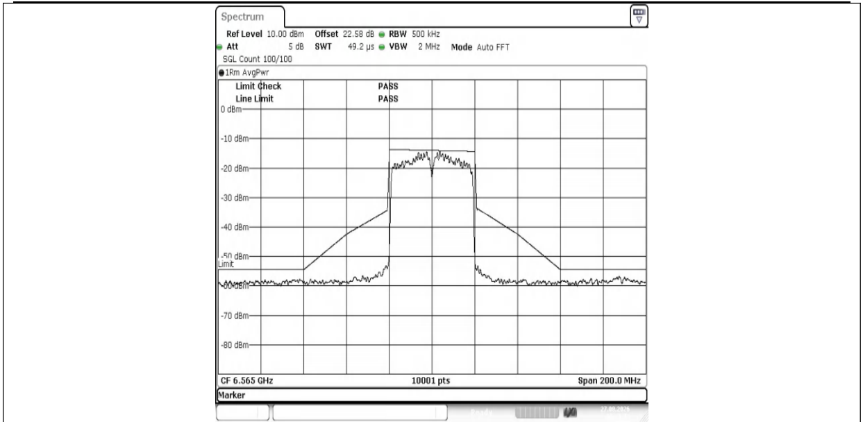
NTNV-11AX40MIMO-Ant1-6565-PASS
