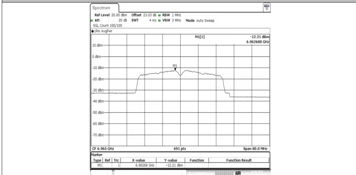
11AX40MIMO-Ant1-6965-PASS
