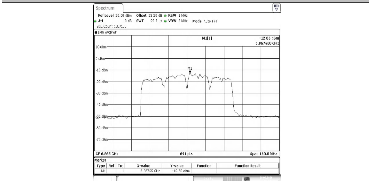
11AX80MIMO-Ant1-6865-PASS
