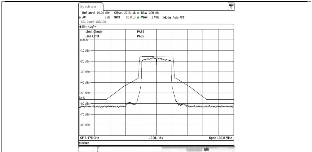
NTNV-11AX20MIMO-Ant1-6475-PASS
