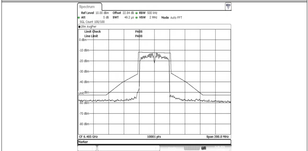
NTNV-11AX40MIMO-Ant1-6405-PASS
