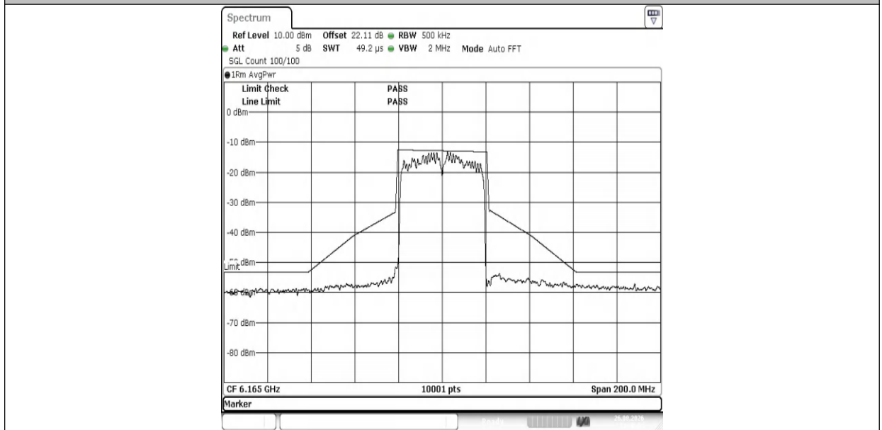
NTNV-11AX40MIMO-Ant2-6165-PASS
