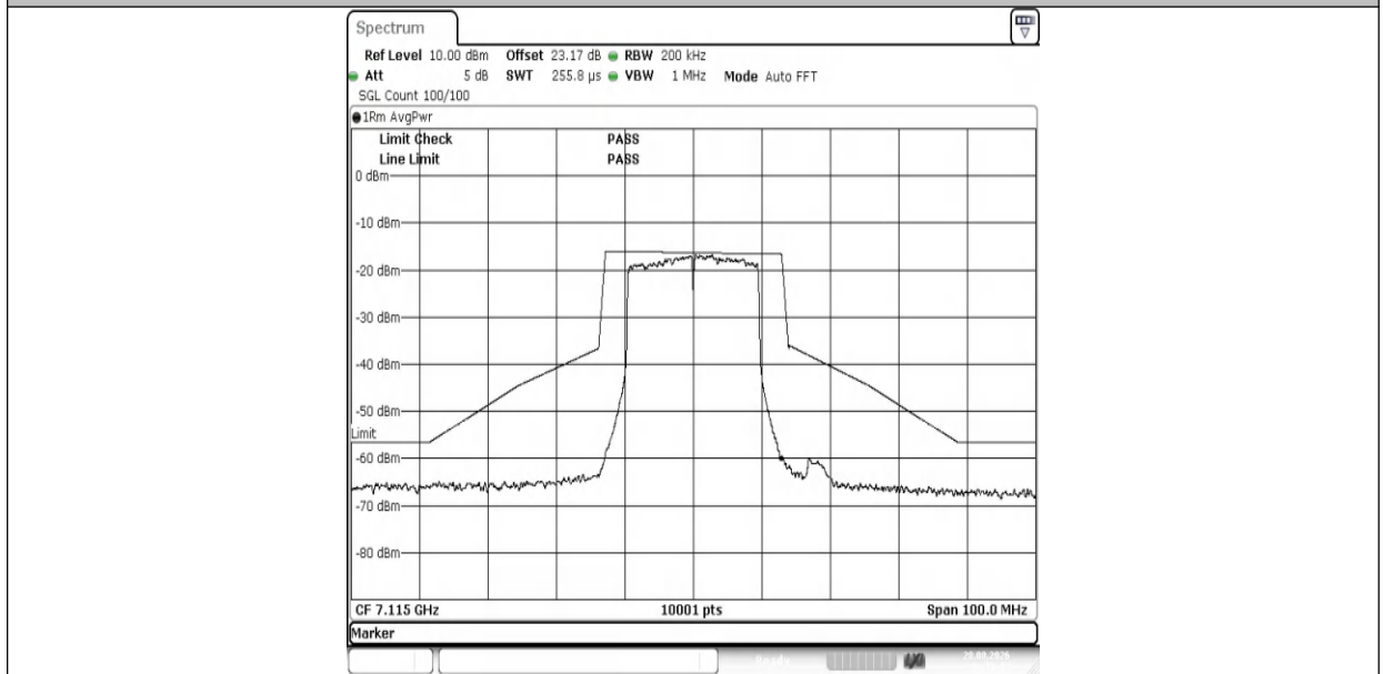
NTNV-11AX20MIMO-Ant2-7115-PASS
