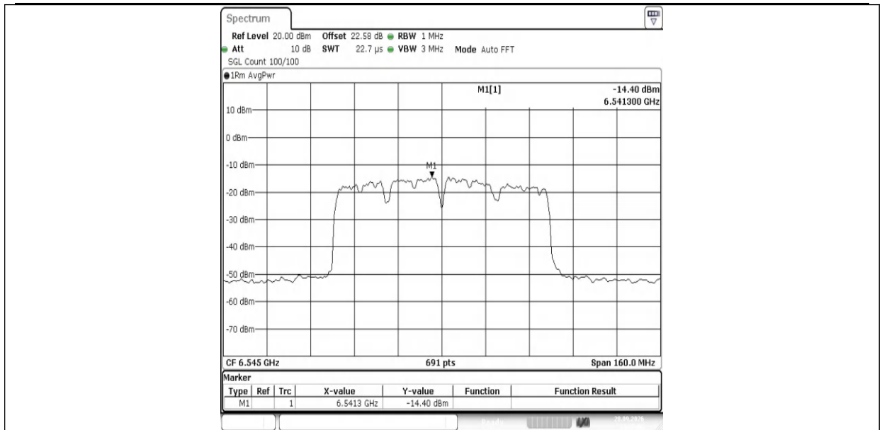
11AX80MIMO-Ant1-6545-PASS
