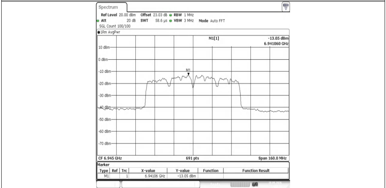
11AX80MIMO-Ant2-6945-PASS
