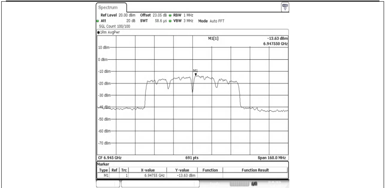
11AX80MIMO-Ant1-6945-PASS
