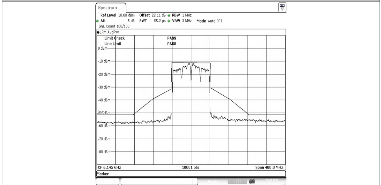
NTNV-11AX80MIMO-Ant2-6145-PASS
