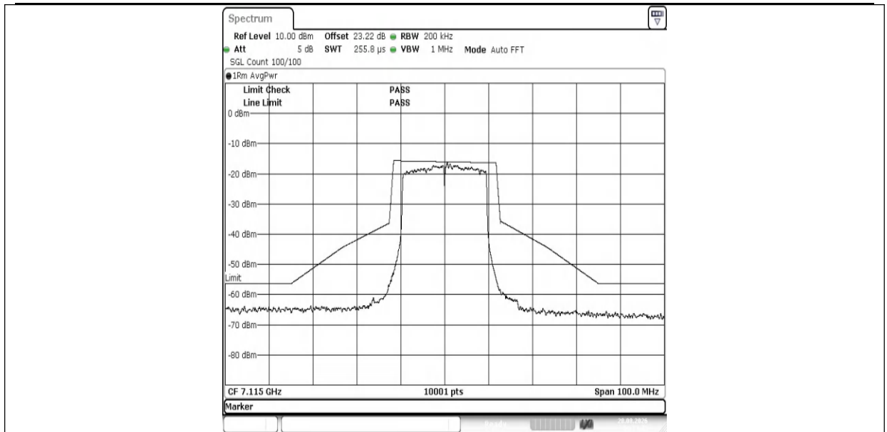
NTNV-11AX20MIMO-Ant1-7115-PASS
