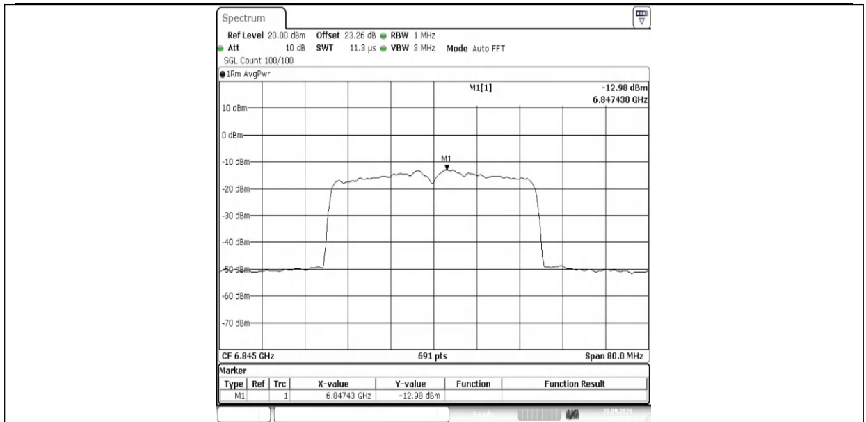
11AX40MIMO-Ant1-6845-PASS
