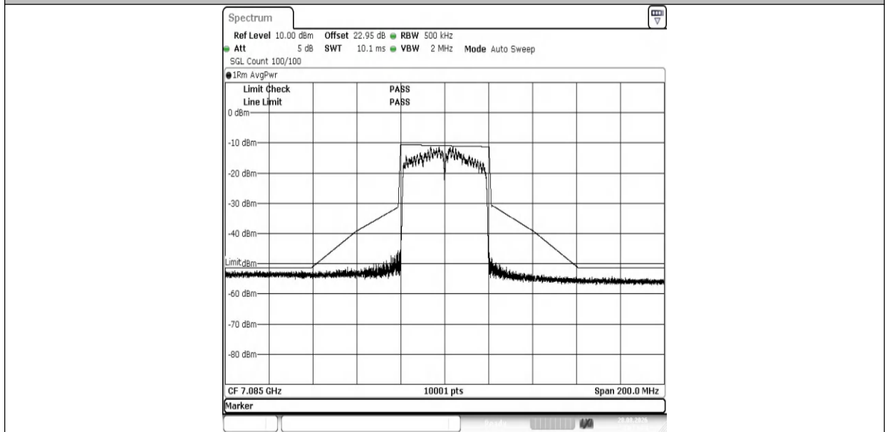
NTNV-11AX40MIMO-Ant2-7085-PASS
