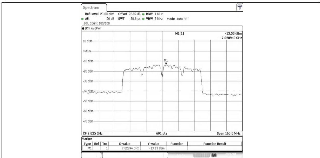
11AX80MIMO-Ant1-7025-PASS
