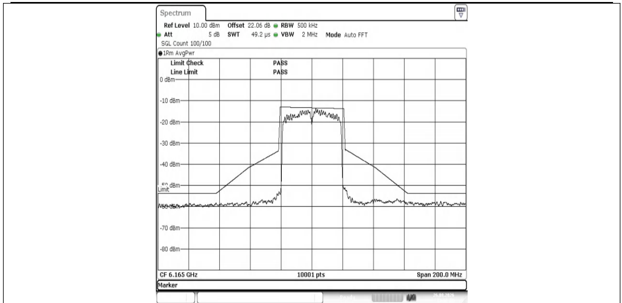
NTNV-11AX40MIMO-Ant1-6165-PASS
