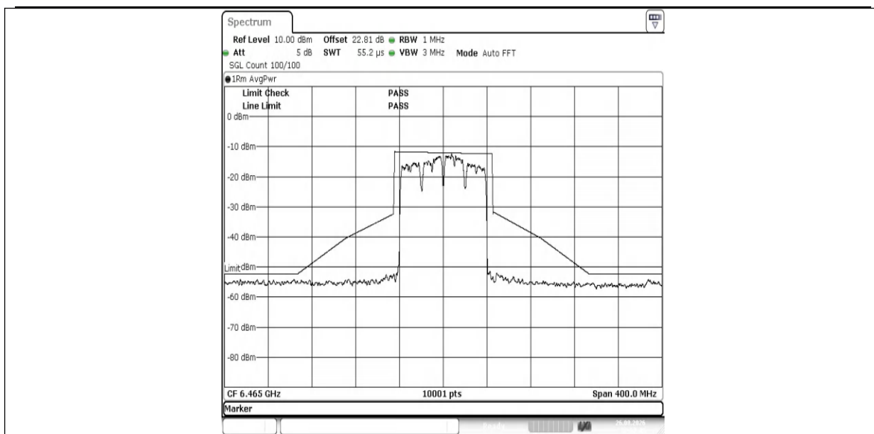
NTNV-11AX80MIMO-Ant1-6465-PASS
