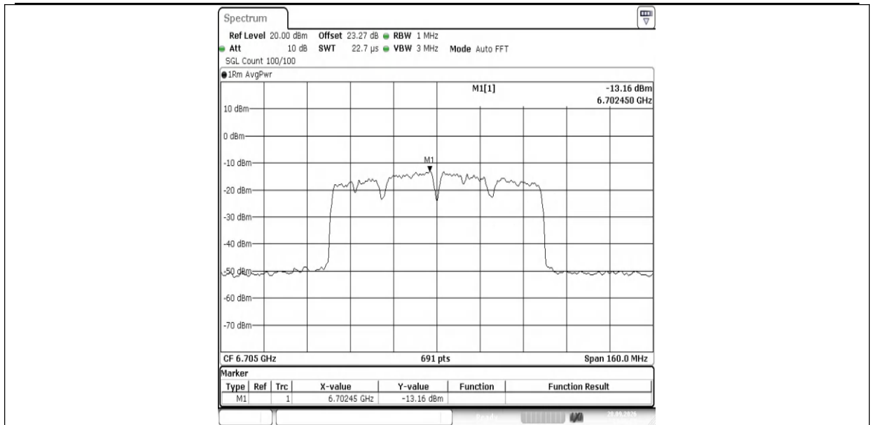
11AX80MIMO-Ant1-6705-PASS
