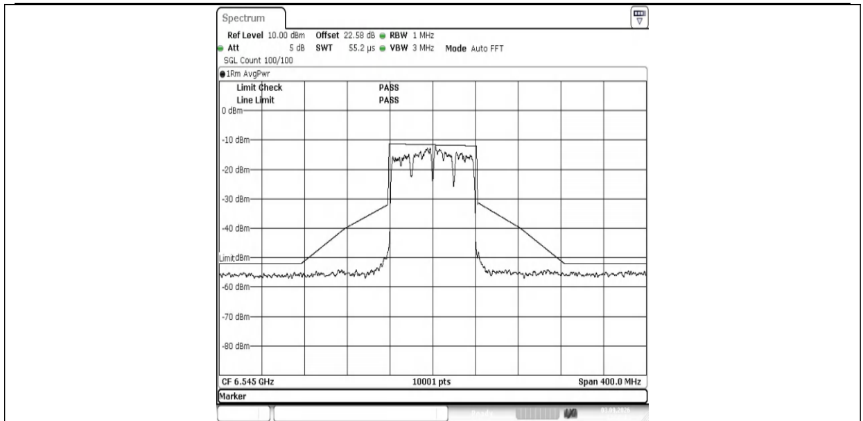
NTNV-11AX80MIMO-Ant1-6545-PASS
