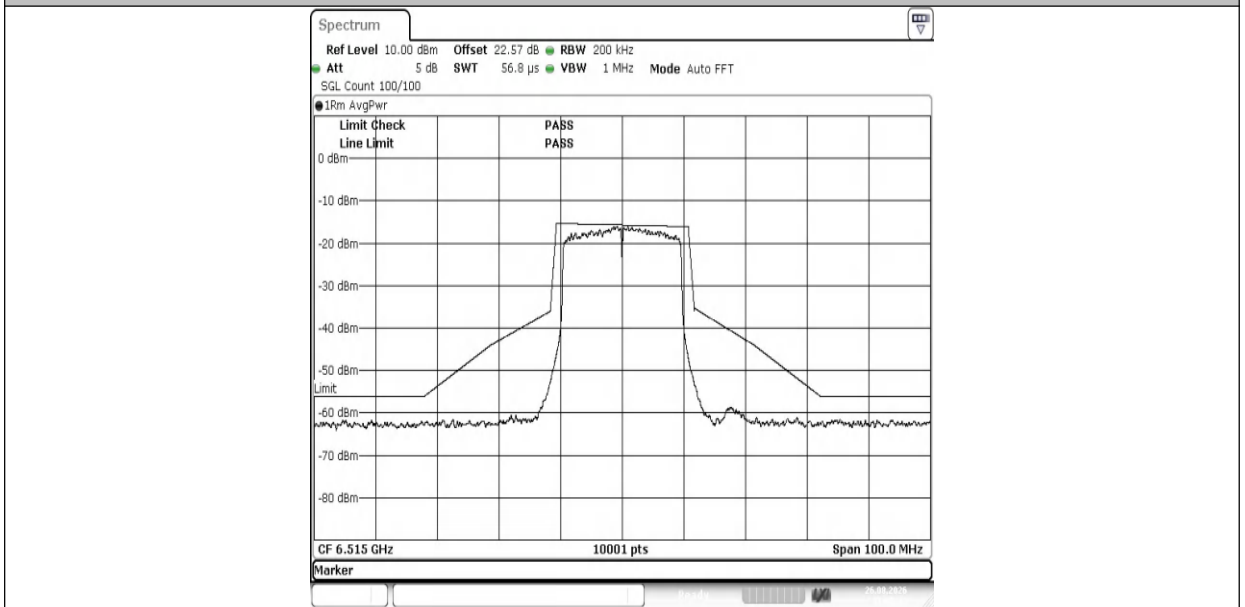
NTNV-11AX20MIMO-Ant2-6515-PASS
