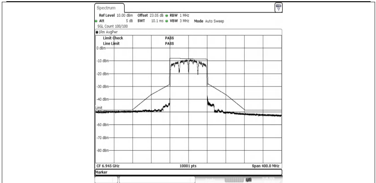
NTNV-11AX80MIMO-Ant1-6945-PASS
