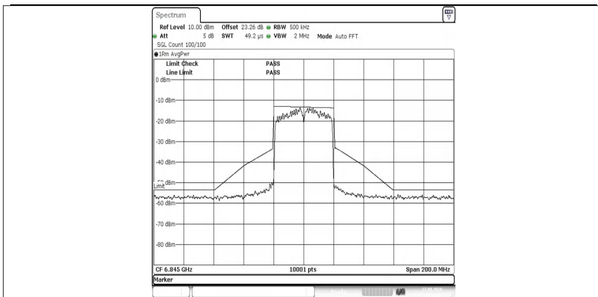
NTNV-11AX40MIMO-Ant1-6845-PASS
