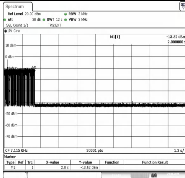
11AX20SISO-Ant1-7115-Center-9-PASS
