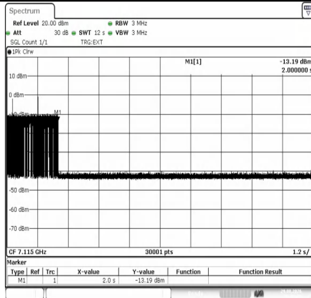
11AX20SISO-Ant1-7115-Center-3-PASS
