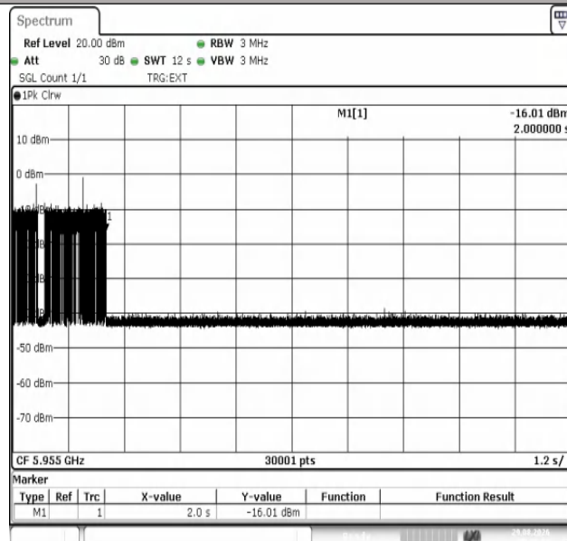
11AX20SISO-Ant1-5955-Center-3-PASS
