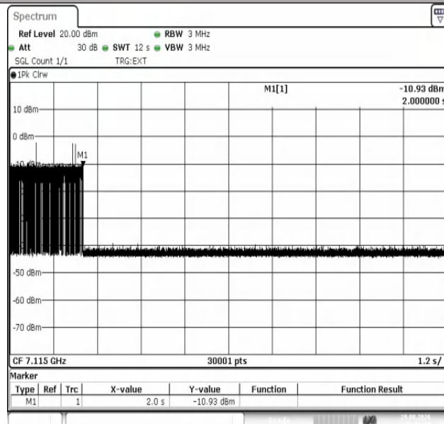
11AX20SISO-Ant1-7115-Center-1-PASS
