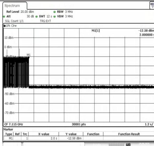
11AX20SISO-Ant1-7115-Center-7-PASS
