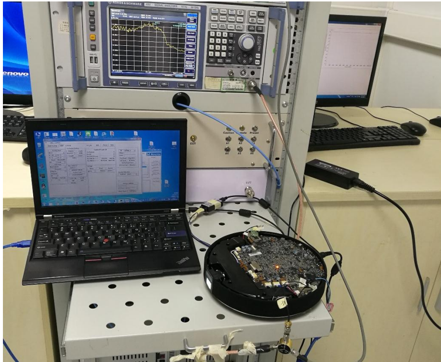
Conducted Test-BT3.0 ANT2
