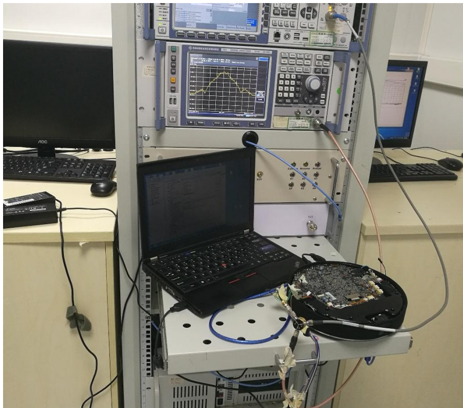
Conducted Test-BT3.0 ANT3
