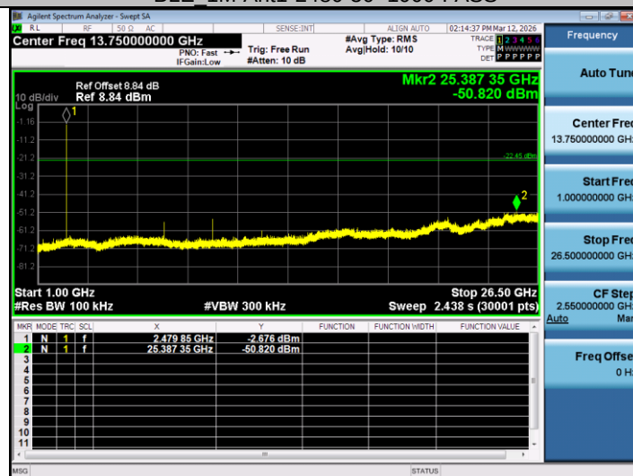
BLE_1M-Ant1-2480-1000~26500-PASS
