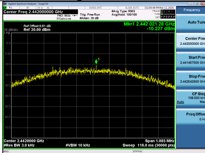
BLE_1M-Ant1-2442-PASS
