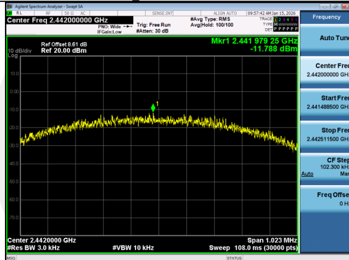
BLE_1M-Ant1-2442-PASS
