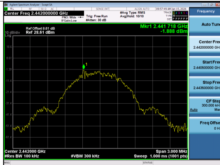
BLE_1M-Ant1-2442-0-Reference-PASS
