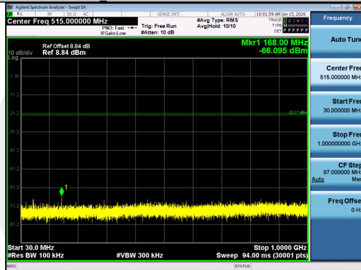
BLE_1M-Ant1-2480-30-1000-PASS
