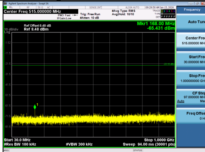
BLE_1M-Ant1-2402-30~1000-PASS
