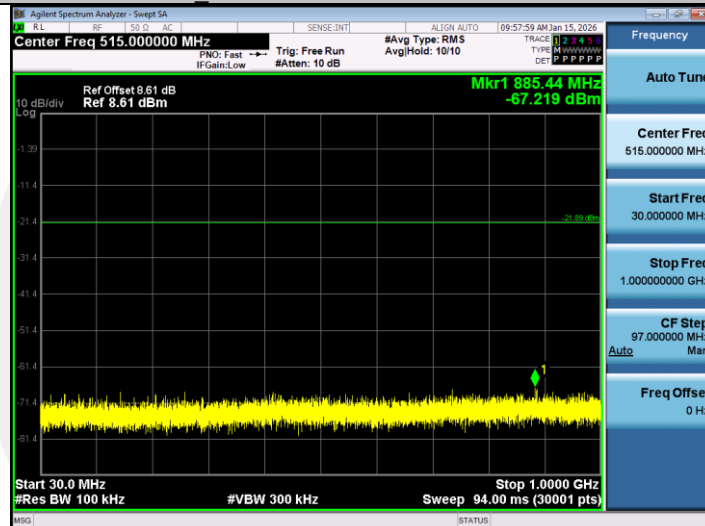
BLE_1M-Ant1-2442-30-1000-PASS
