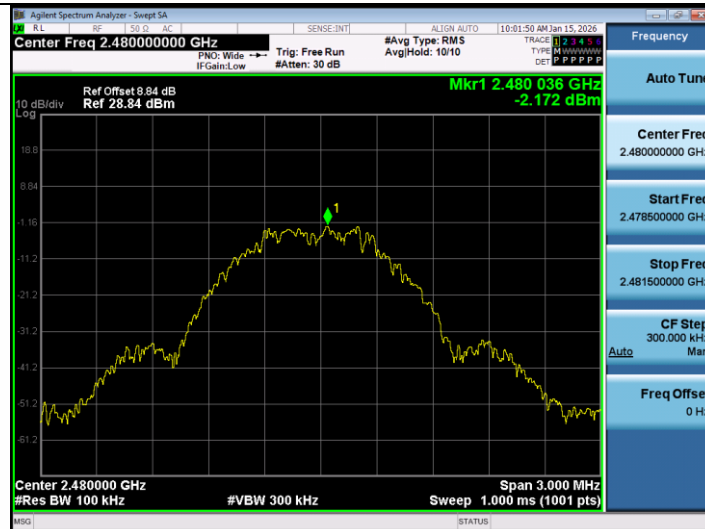
BLE_1M-Ant1-2480-0-Reference-PASS
