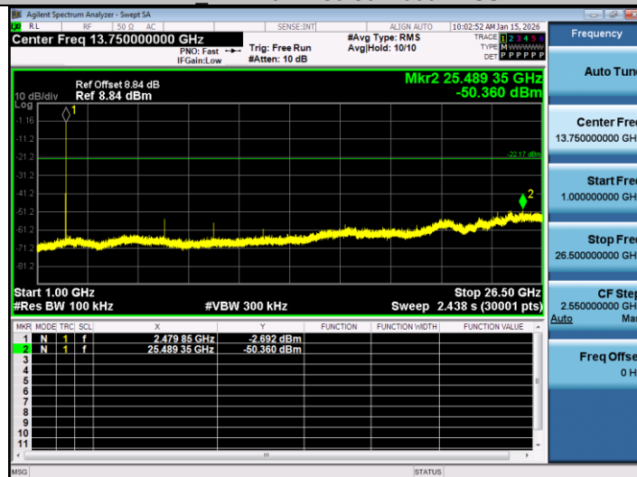
BLE_1M-Ant1-2480-1000-26500-PASS
