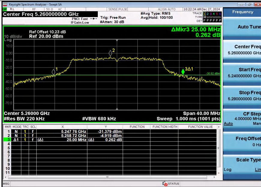
11AC20SISO-Ant1-5260
