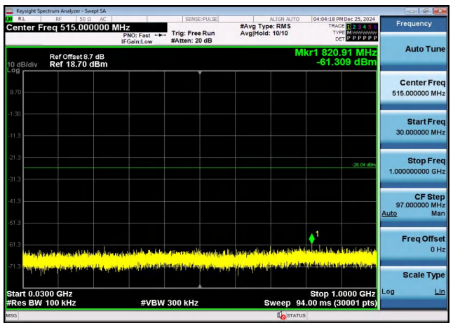
30MHz-1GHz
