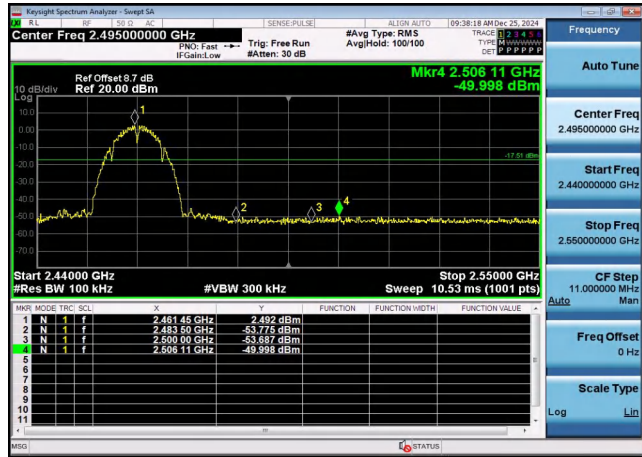
Right bandedge
