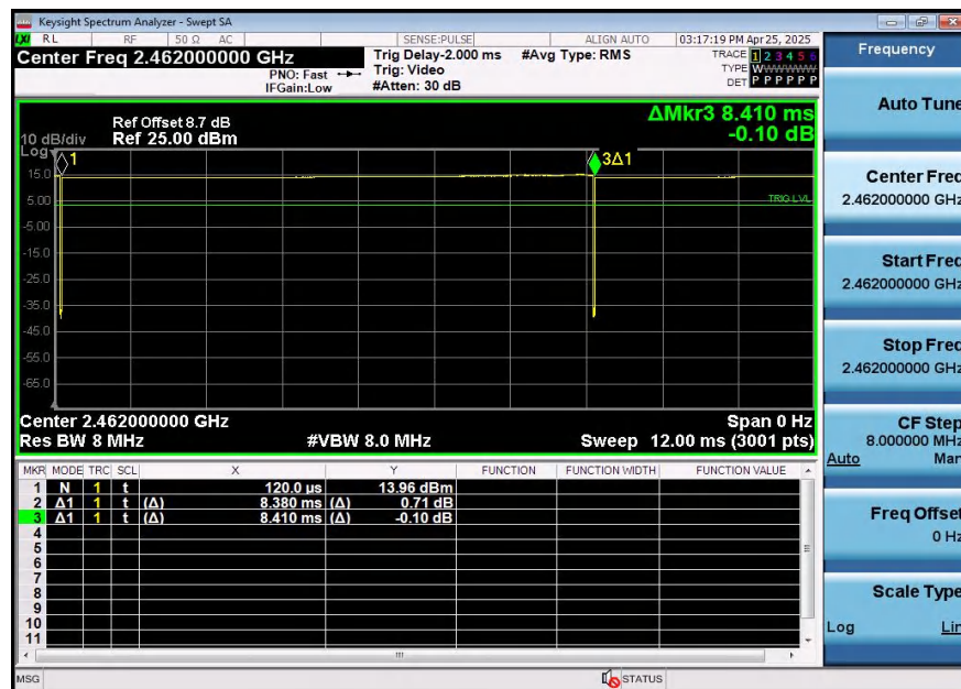
Ant2
