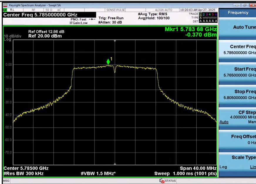
11A-Ant1-5785-PASS
