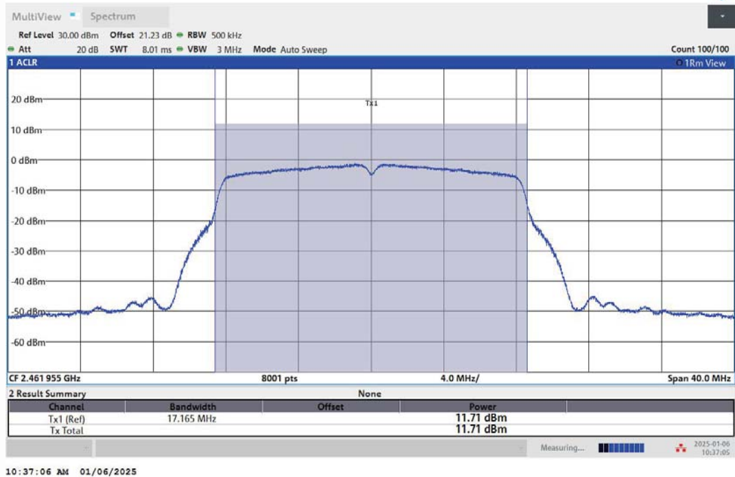
11G-Ant2-2462-PASS
