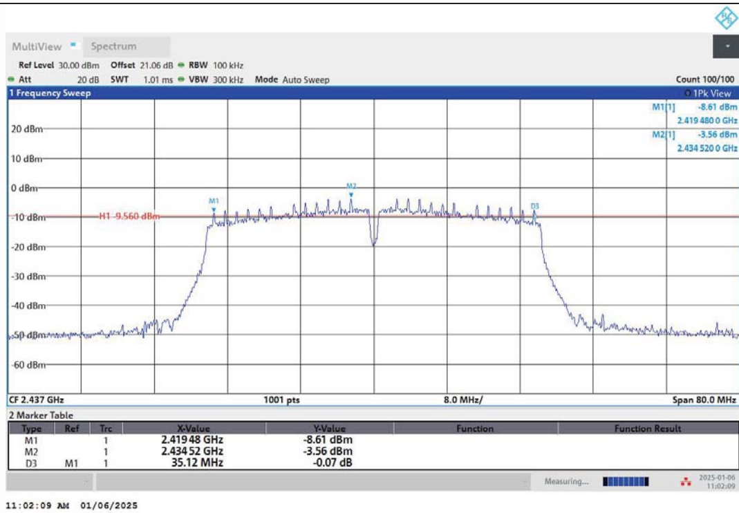
11N40MIMO-Ant1-2437-PASS
