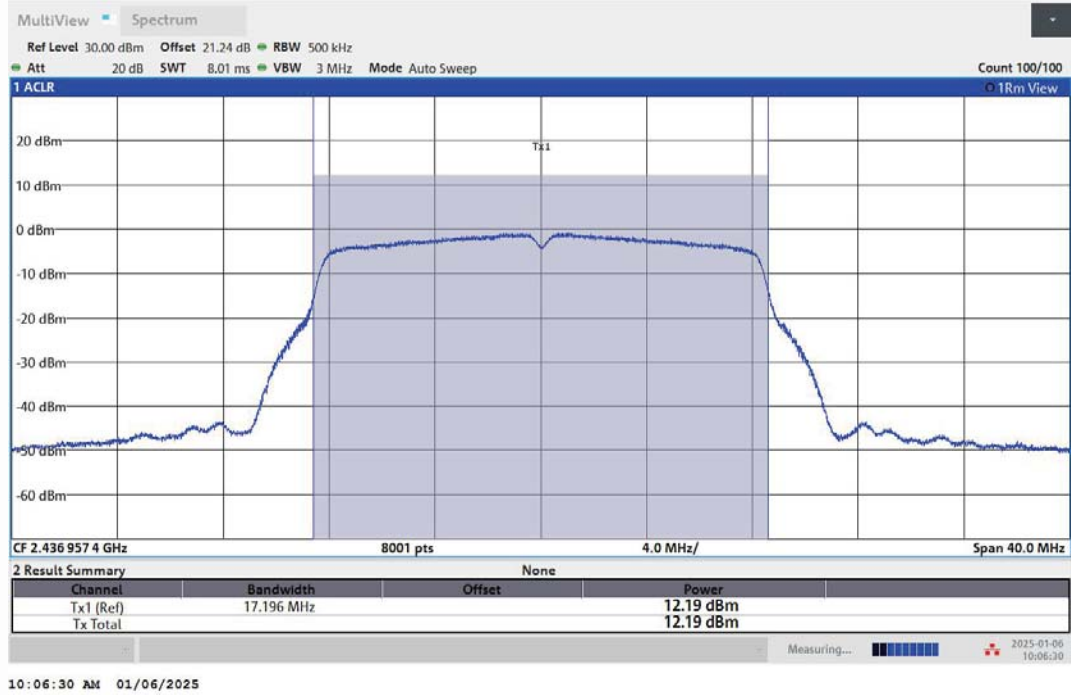
11G-Ant1-2437-PASS
