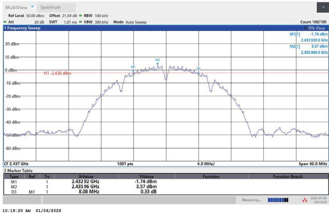
11B-Ant2-2437-PASS
