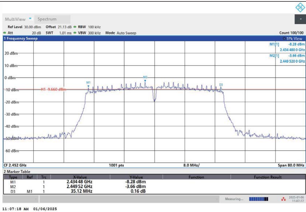
11N40MIMO-Ant1-2452-PASS
