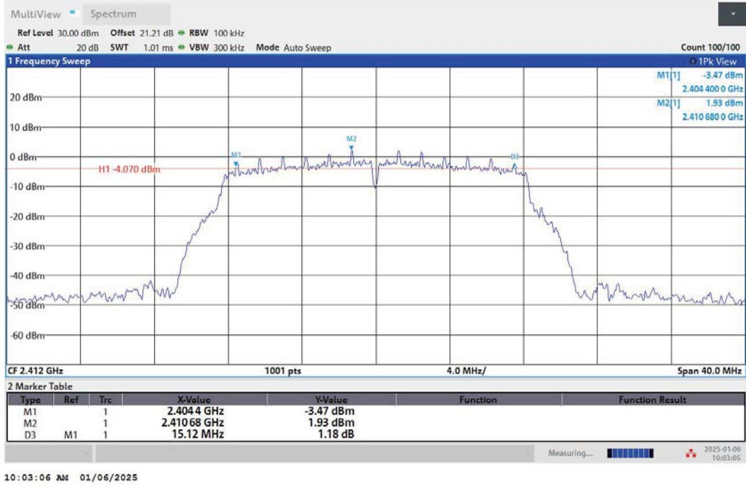
11G-Ant1-2412-PASS
