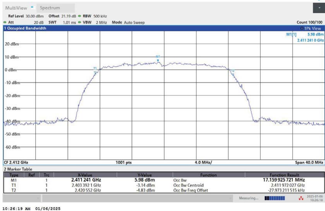
11G-Ant2-2412
