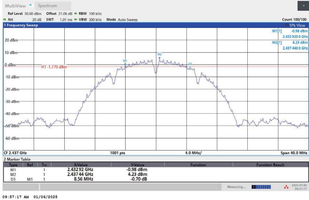
11B-Ant1-2437-PASS
