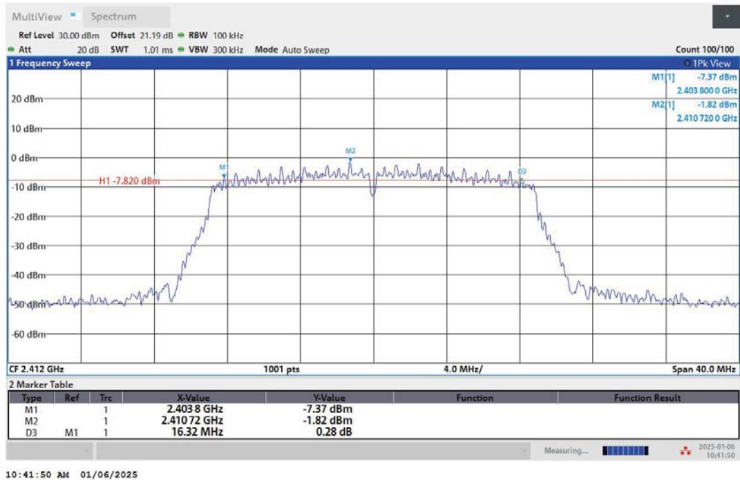
11N20MIMO-Ant2-2412-PASS
