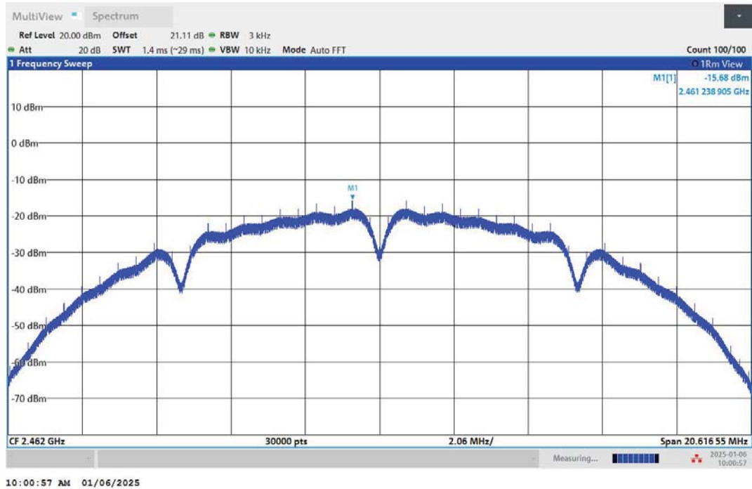
11B-Ant1-2462-PASS
