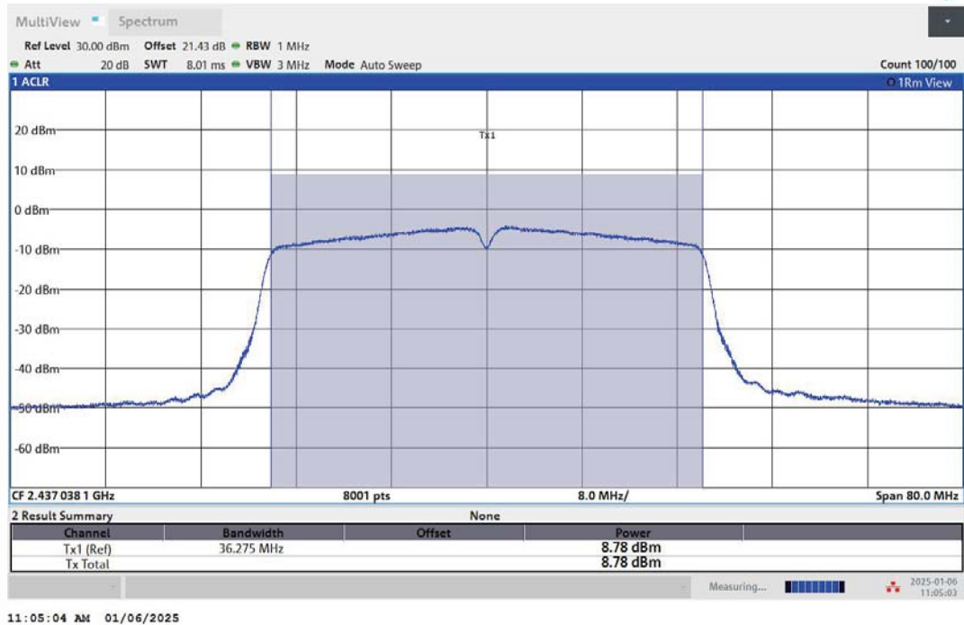
11N40MIMO-Ant2-2437-PASS
