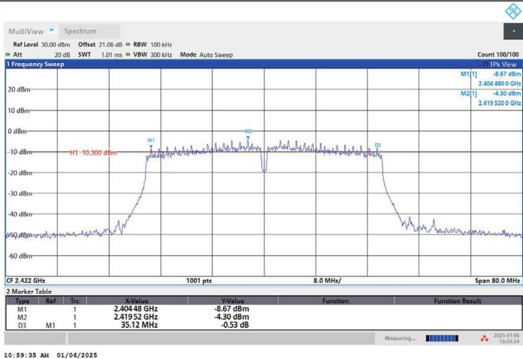
11N40MIMO-Ant2-2422-PASS
