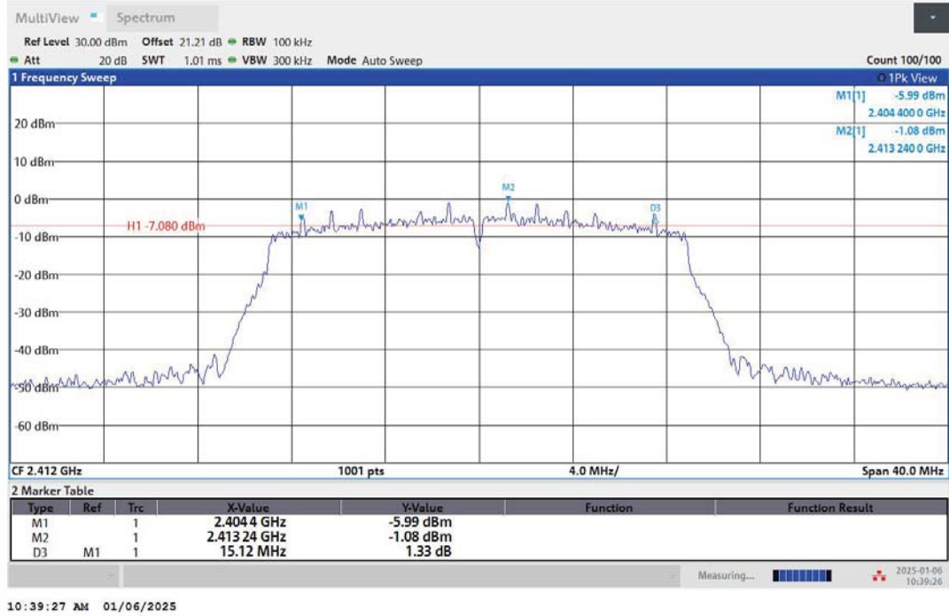
11N20MIMO-Ant1-2412-PASS
