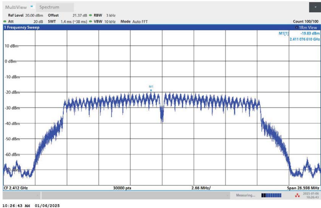
11G-Ant2-2412-PASS
