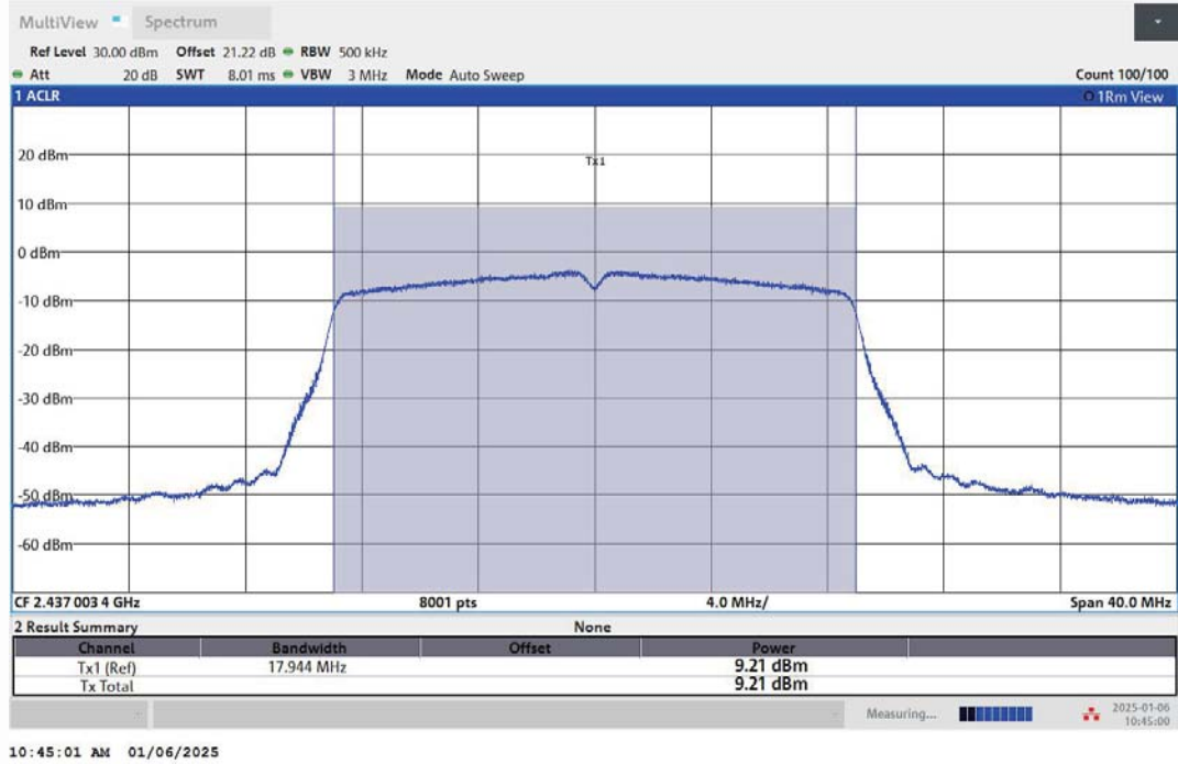
11N20MIMO-Ant1-2437-PASS
