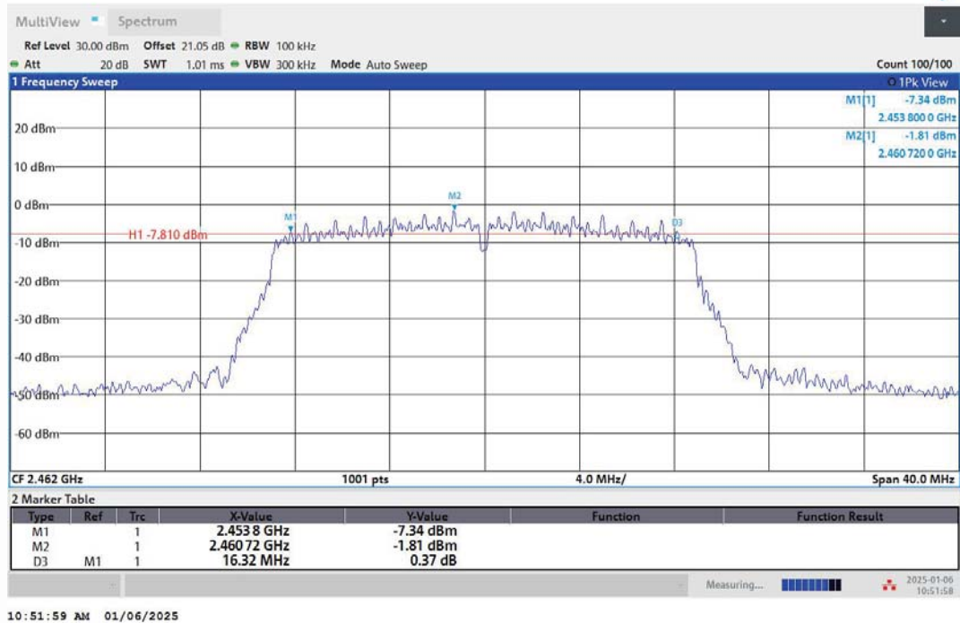
11N20MIMO-Ant2-2462-PASS
