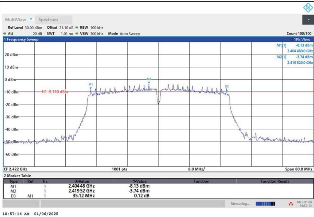
11N40MIMO-Ant1-2422-PASS
