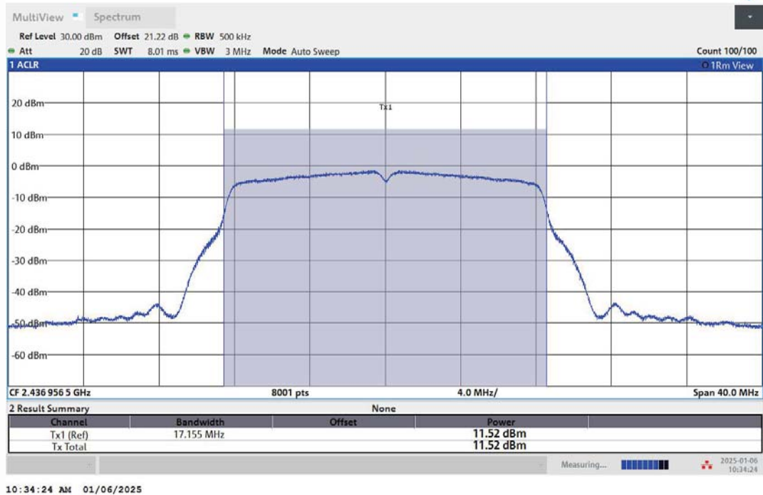
11G-Ant2-2437-PASS
