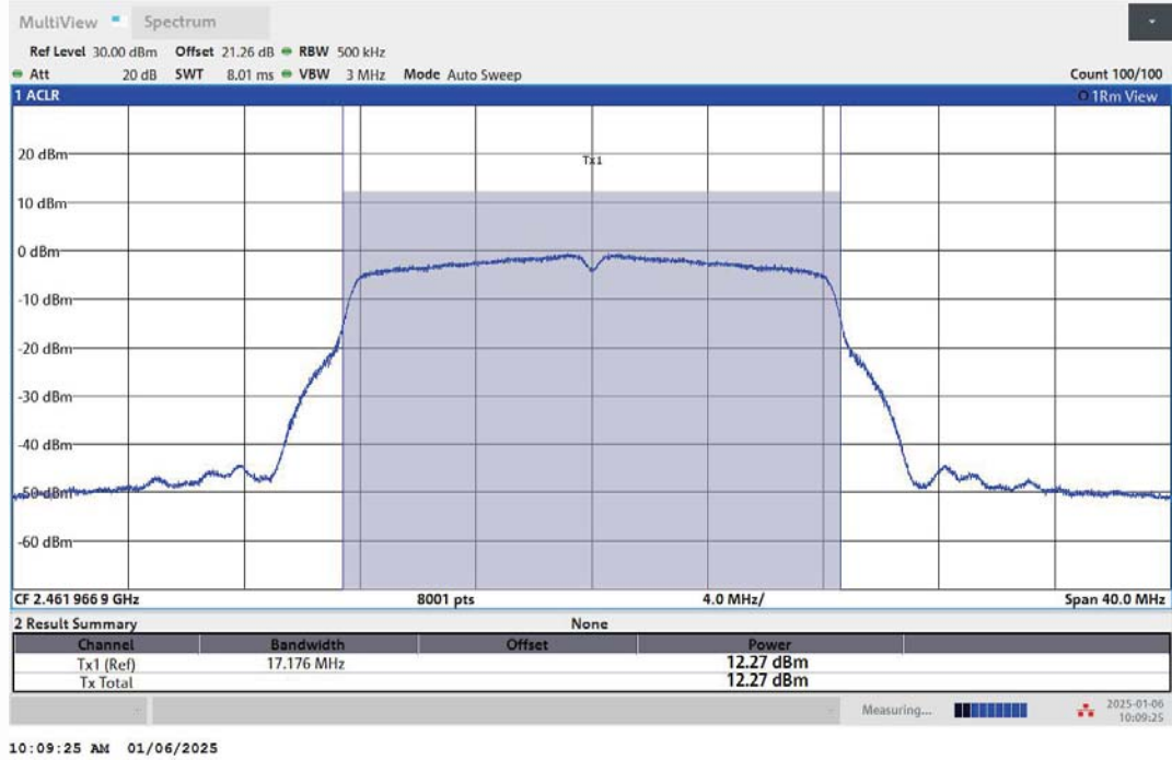
11G-Ant1-2462-PASS
