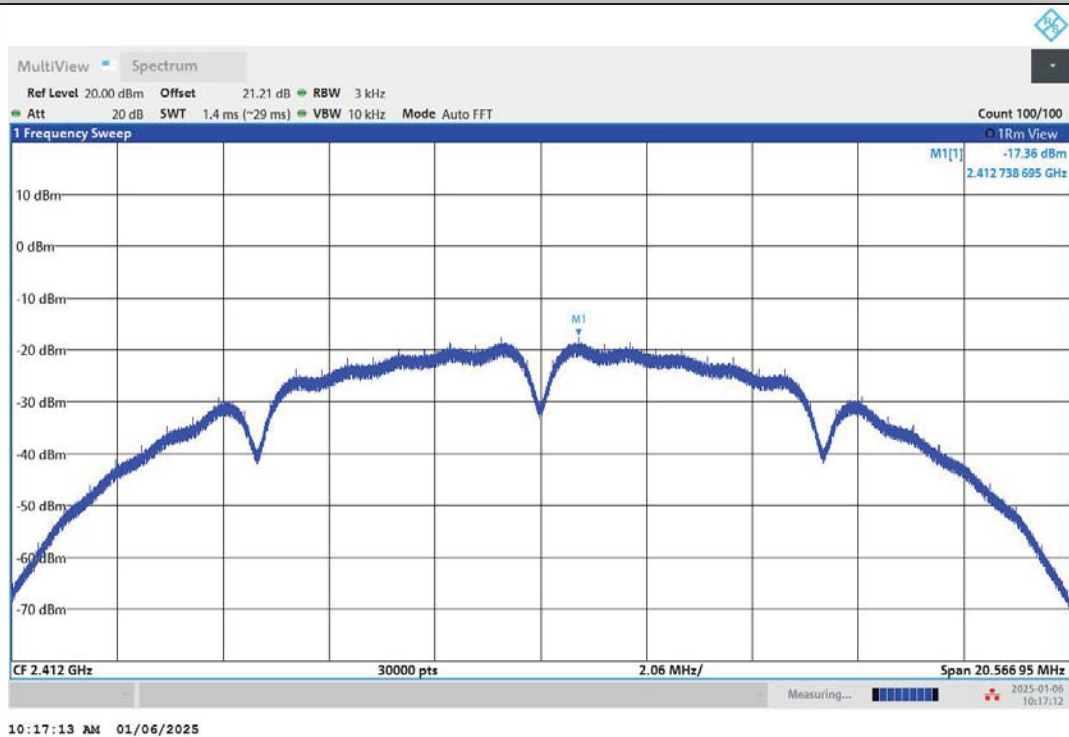
11B-Ant2-2412-PASS
