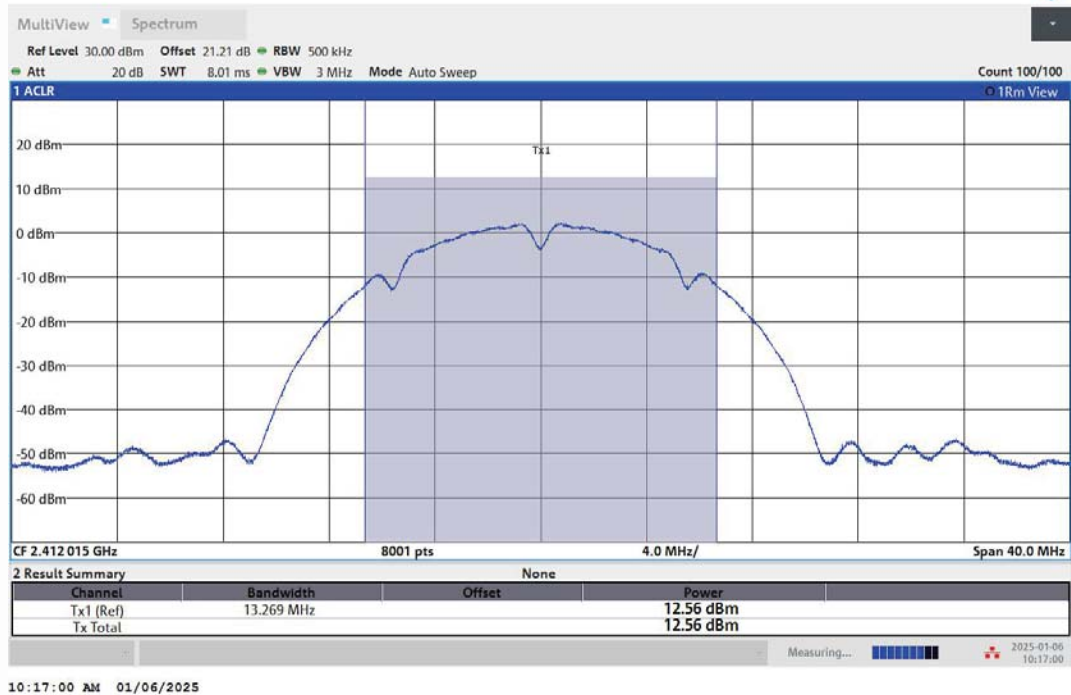
11B-Ant2-2412-PASS
