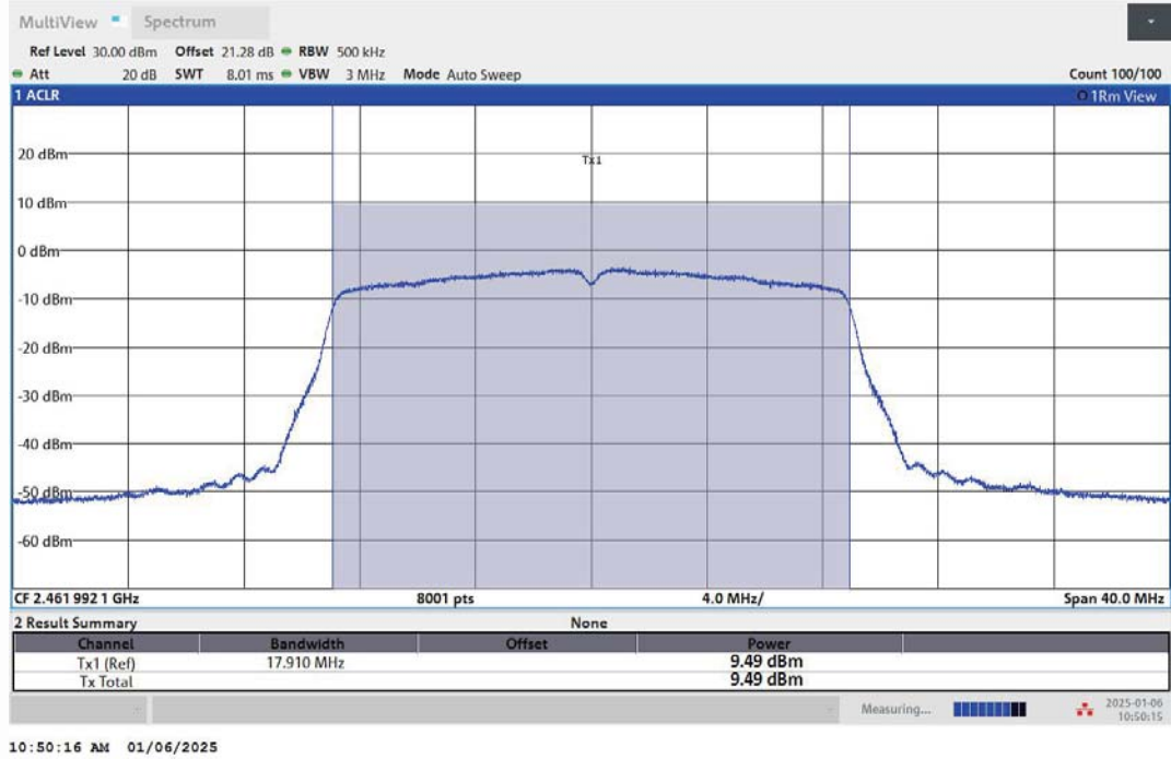
11N20MIMO-Ant1-2462-PASS
