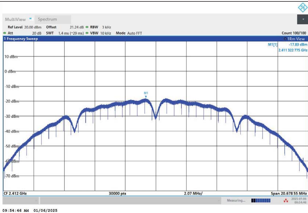
11B-Ant1-2412-PASS
