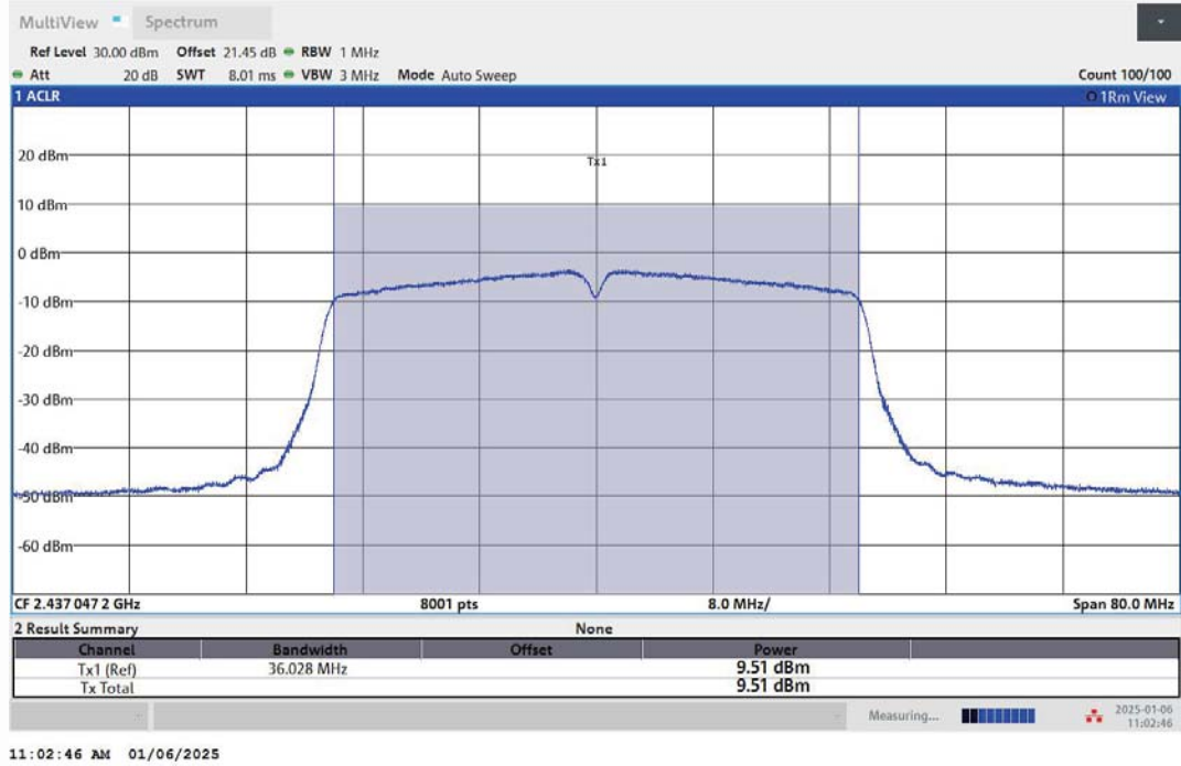
11N40MIMO-Ant1-2437-PASS
