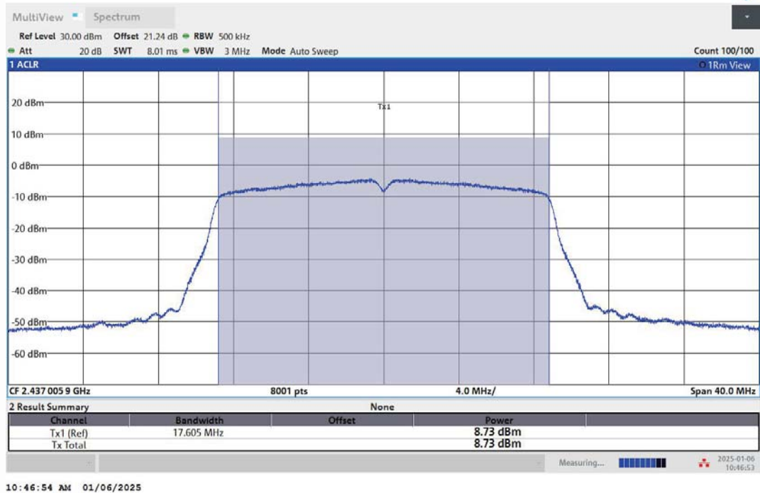
11N20MIMO-Ant2-2437-PASS
