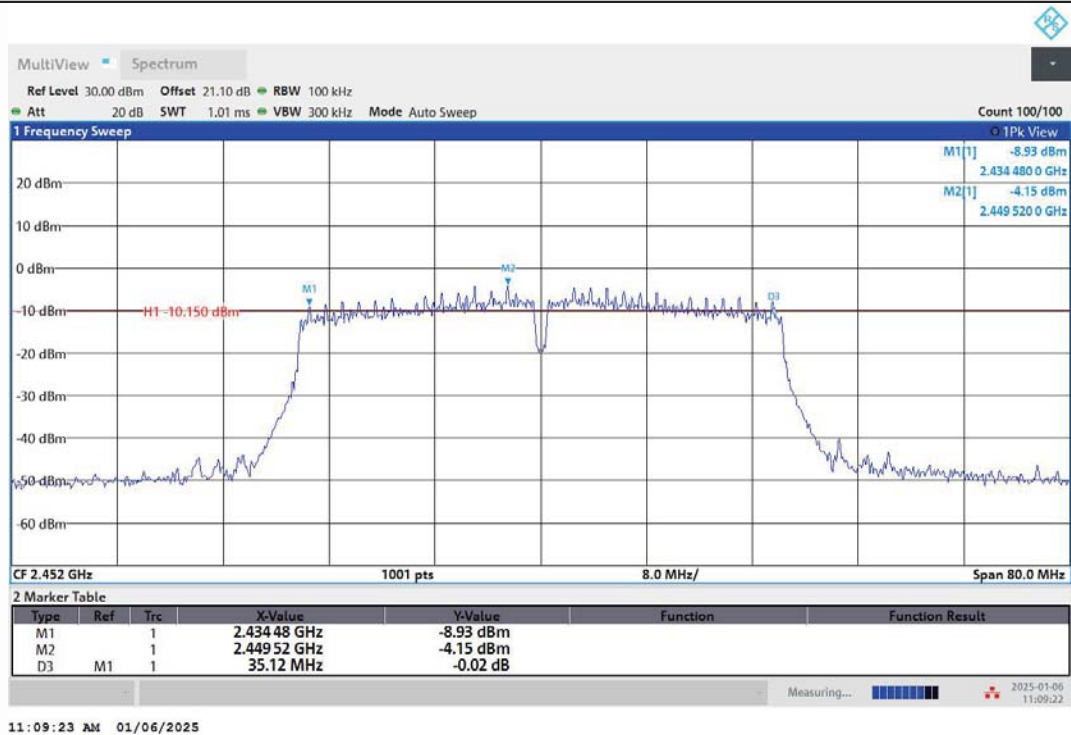
11N40MIMO-Ant2-2452-PASS
