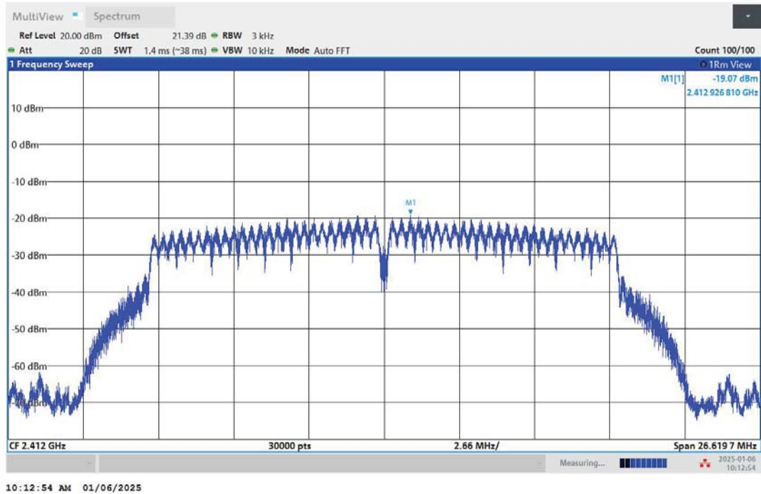
11G-Ant1-2412-PASS
