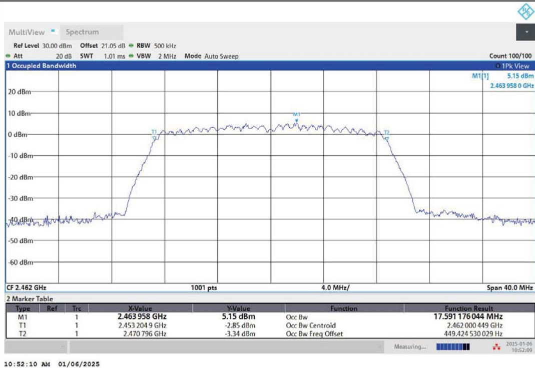
11N20MIMO-Ant2-2462
