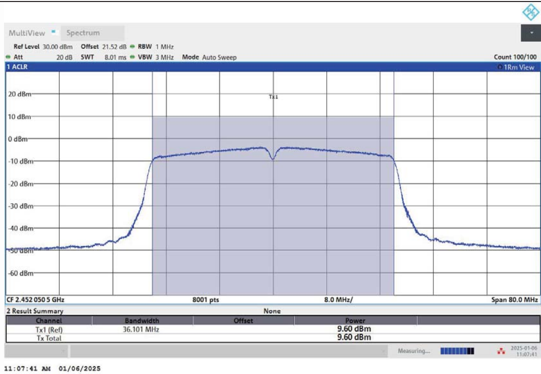
11N40MIMO-Ant1-2452-PASS
