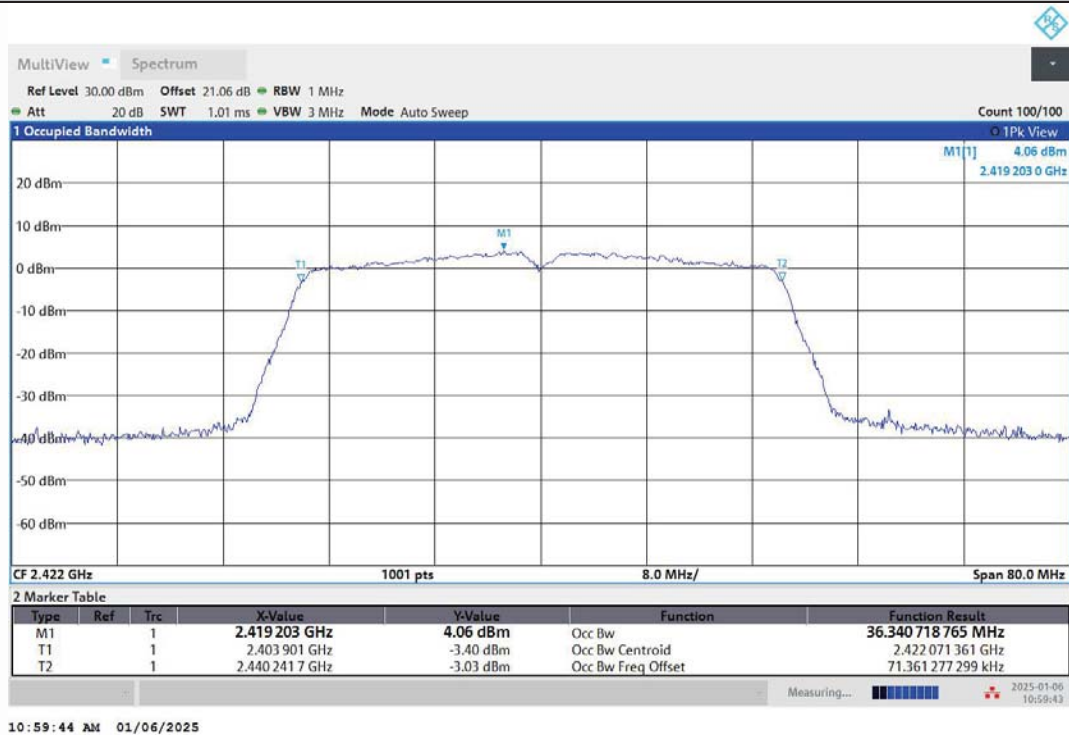
11N40MIMO-Ant2-2422
