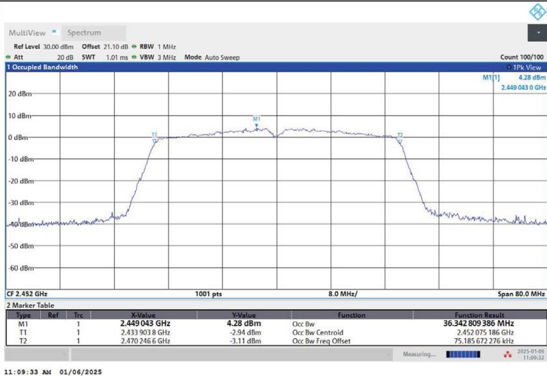
11N40MIMO-Ant2-2452
