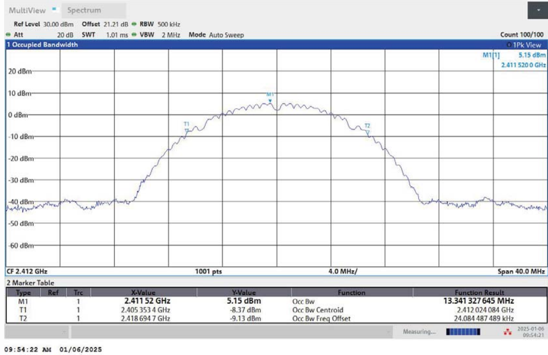
11B-Ant1-2412
