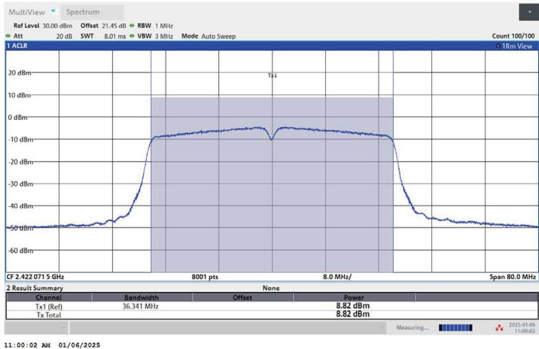
11N40MIMO-Ant2-2422-PASS
