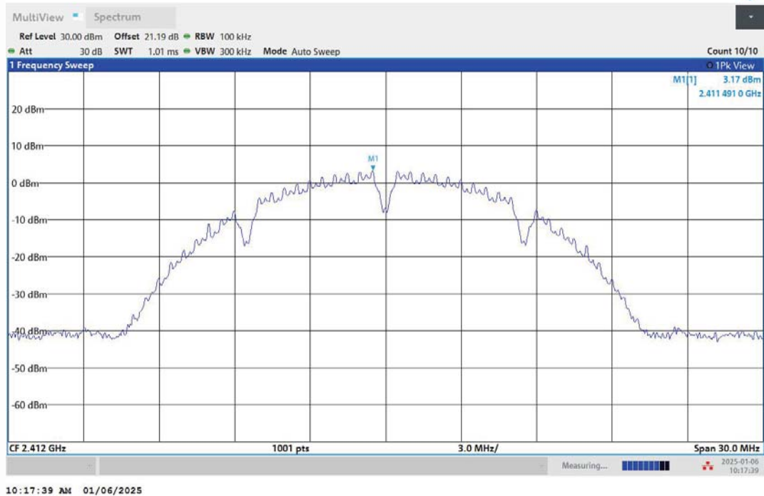
11B-Ant2-2412-0~Reference-PASS
