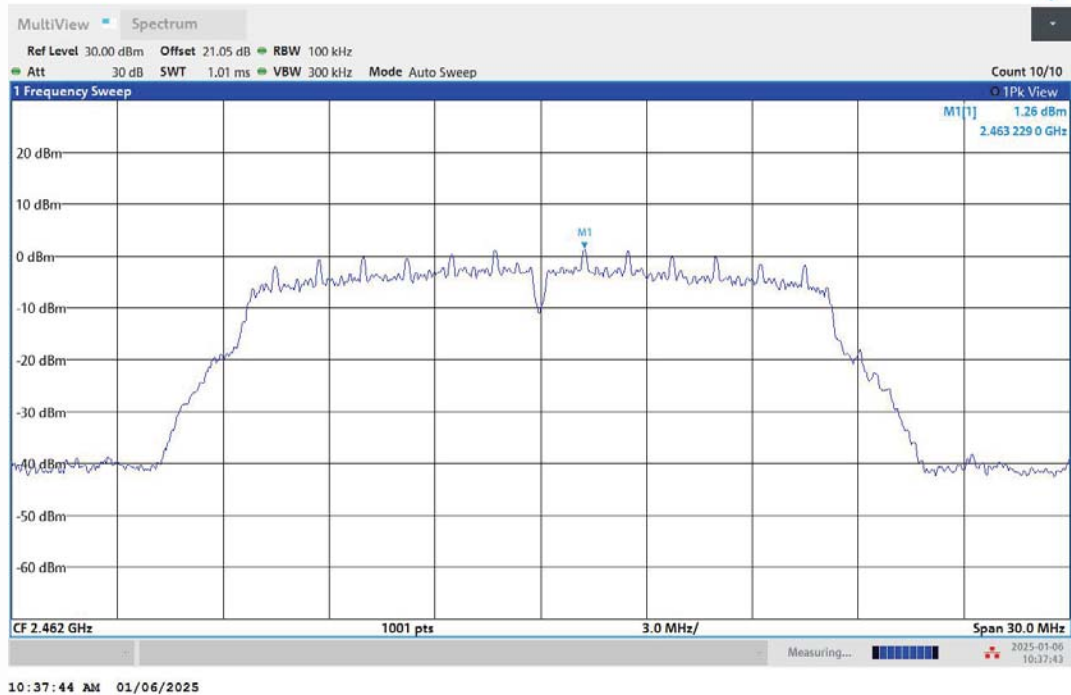
11G-Ant2-2462-0~Reference-PASS
