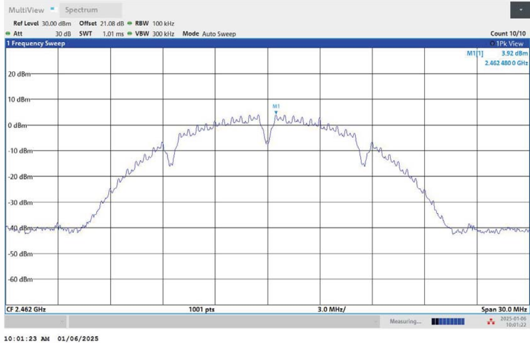
11B-Ant1-2462-0~Reference-PASS
