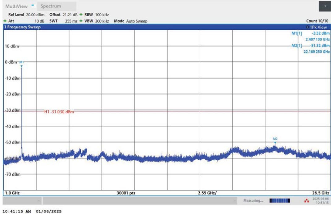
11N20MIMO-Ant1-2412-1000~26500-PASS
