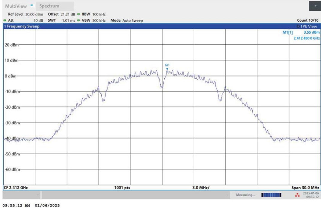
11B-Ant1-2412-0~Reference-PASS
