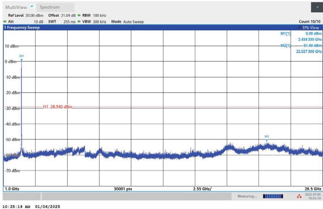
11G-Ant2-2437-1000~26500-PASS
