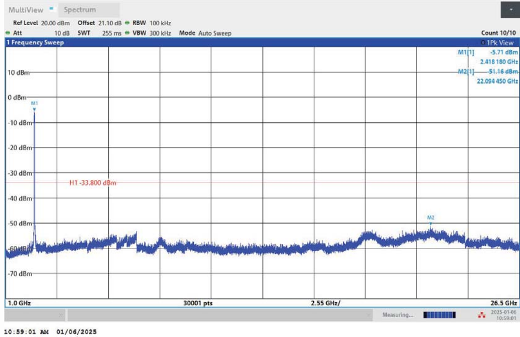
11N40MIMO-Ant1-2422-1000~26500-PASS
