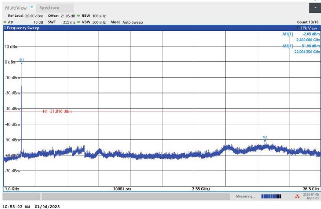
11N20MIMO-Ant2-2462-1000~26500-PASS
