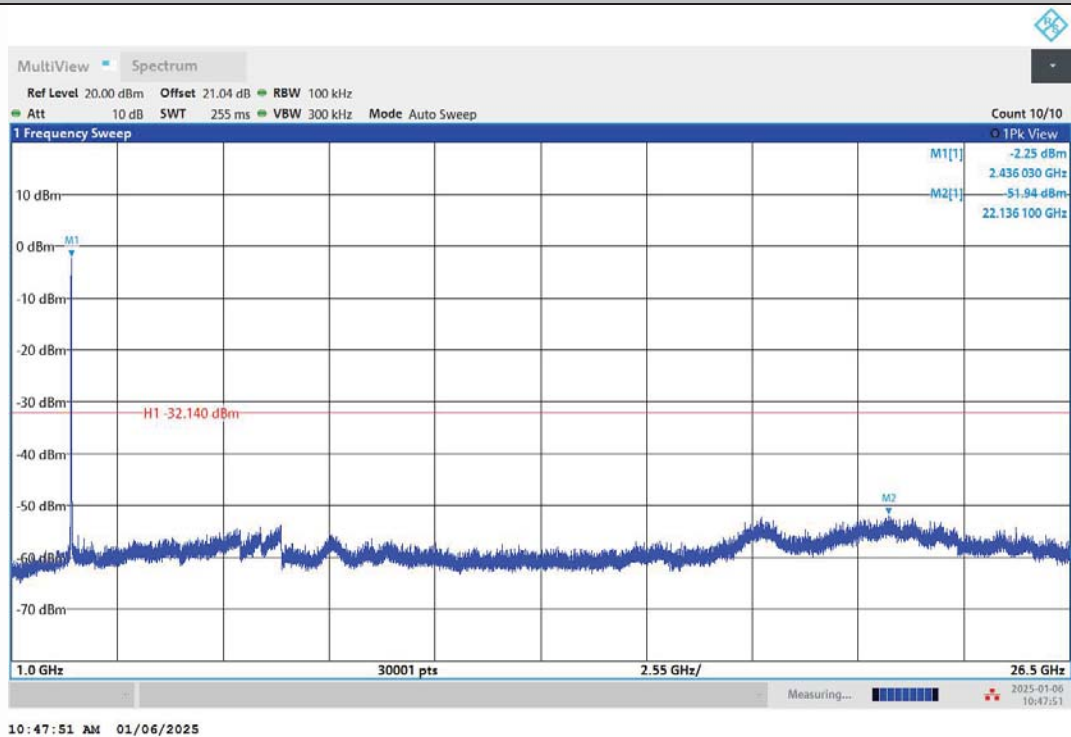
11N20MIMO-Ant2-2437-1000~26500-PASS
