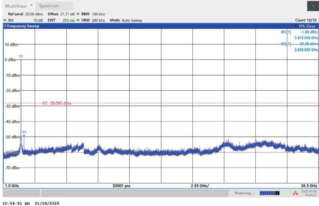
11G-Ant1-2412-1000~26500-PASS
