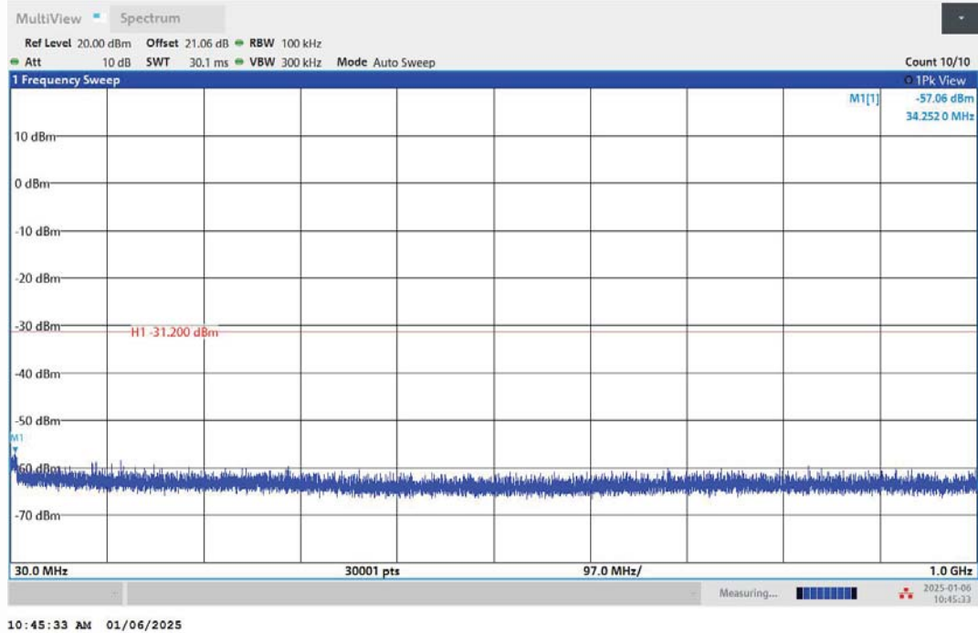
11N20MIMO-Ant1-2437-30~1000-PASS
