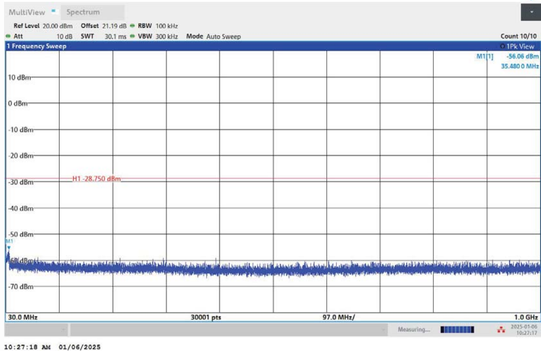
11G-Ant2-2412-30~1000-PASS
