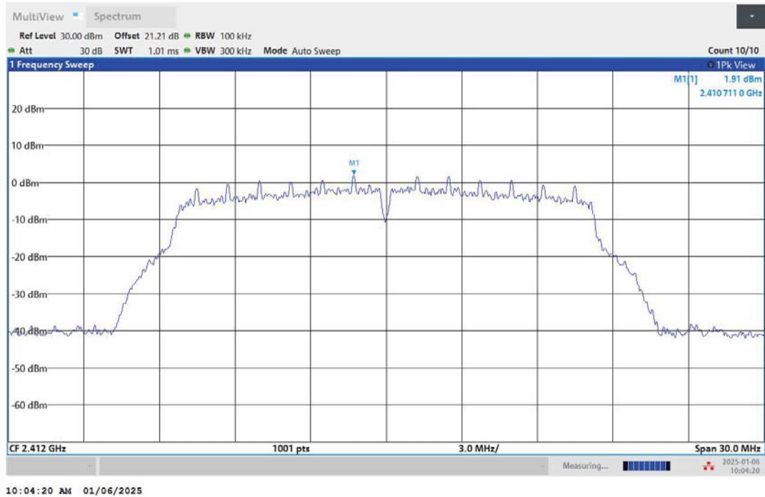
11G-Ant1-2412-0~Reference-PASS
