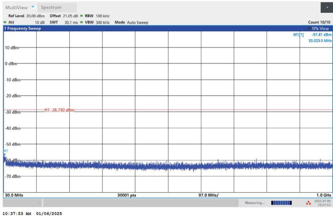
11G-Ant2-2462-30~1000-PASS
