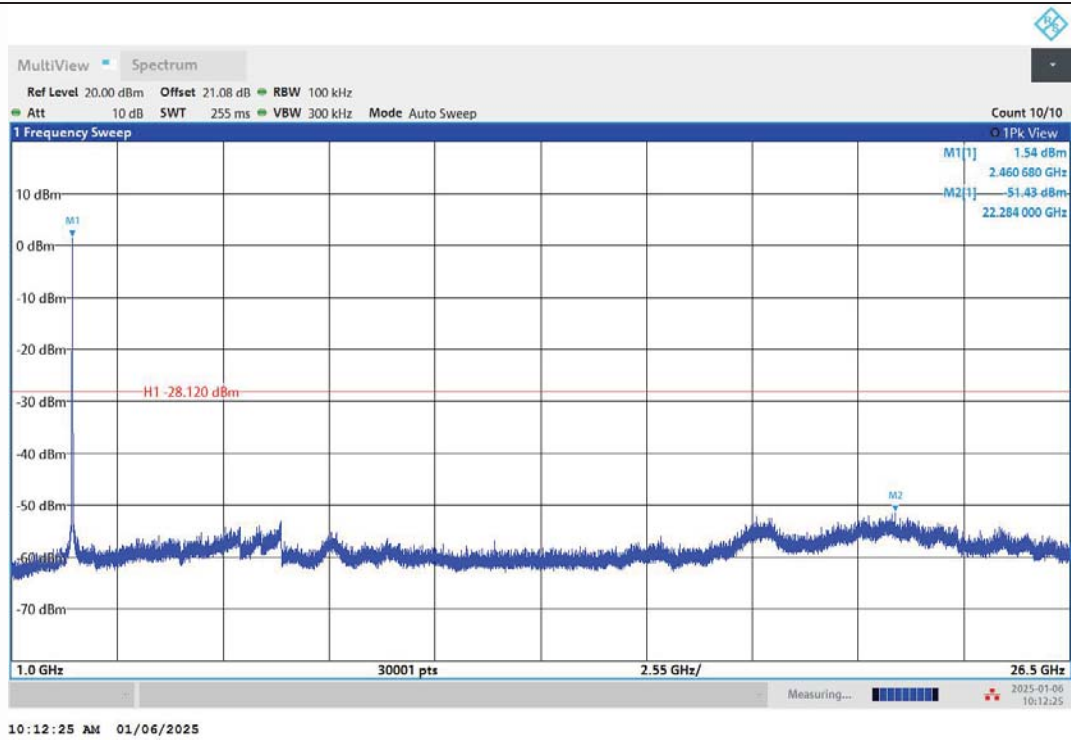
11G-Ant1-2462-1000~26500-PASS
