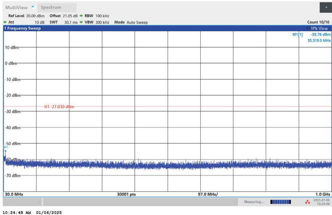
11B-Ant2-2462-30~1000-PASS
