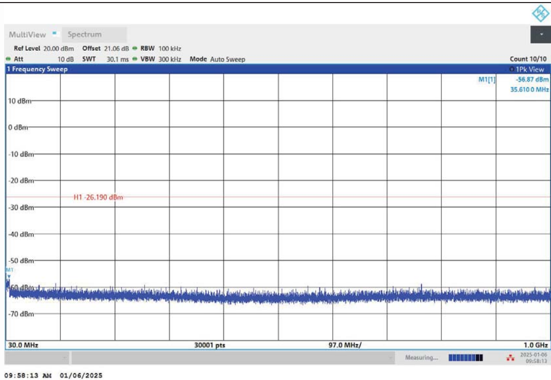
11B-Ant1-2437-30~1000-PASS
