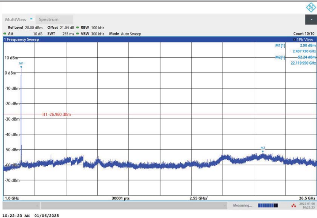
11B-Ant2-2437-1000~26500-PASS
