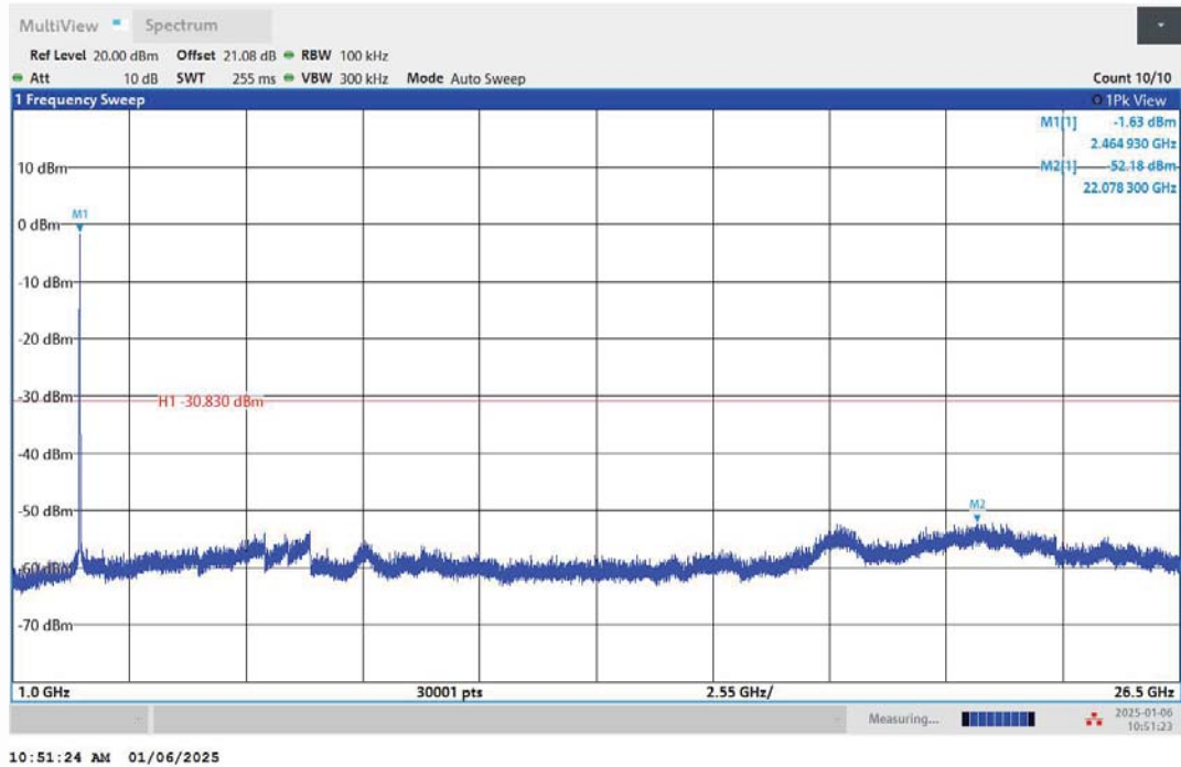
11N20MIMO-Ant1-2462-1000~26500-PASS
