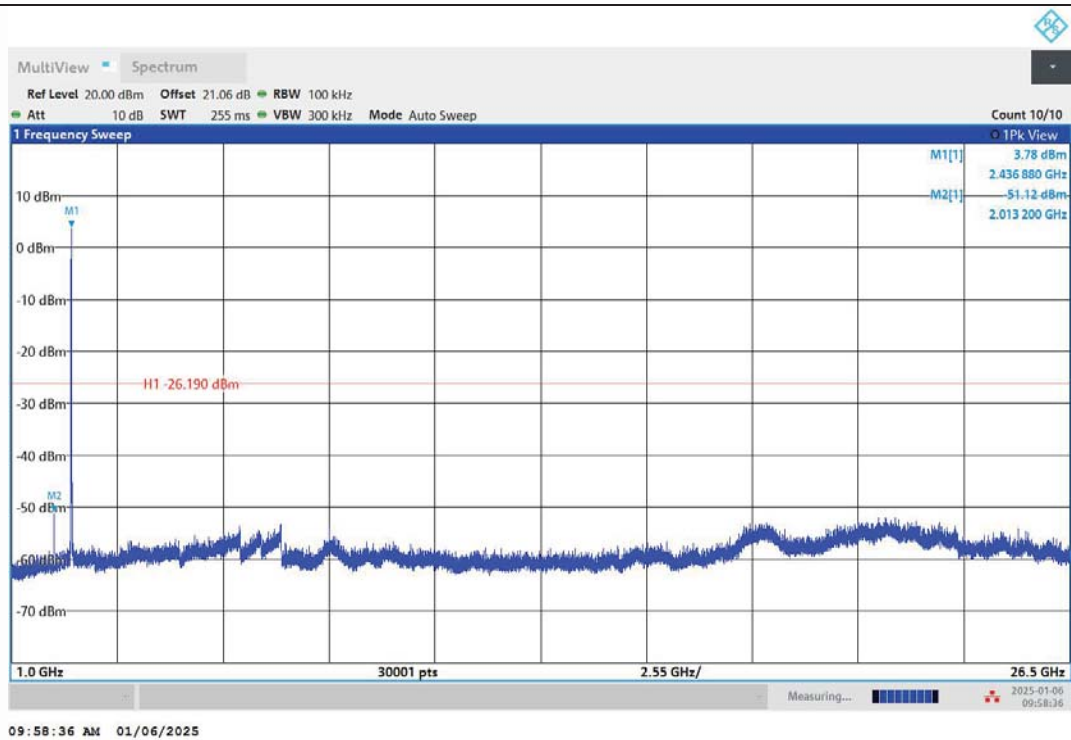
11B-Ant1-2437-1000~26500-PASS
