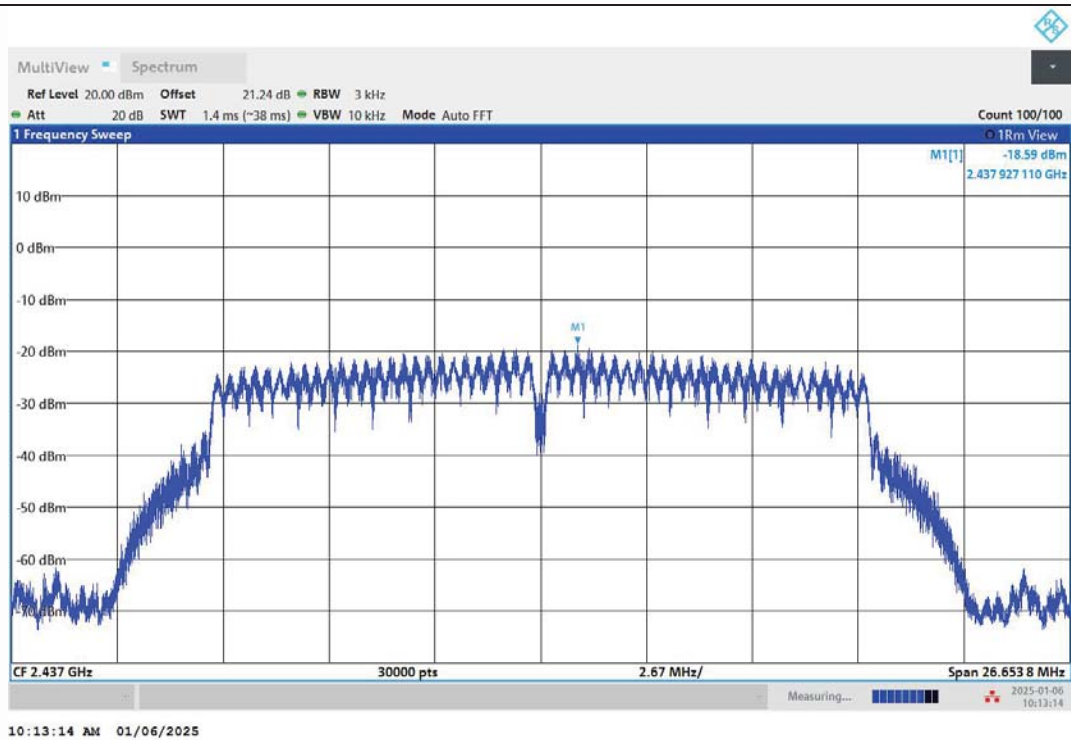
11G-Ant1-2437-PASS
