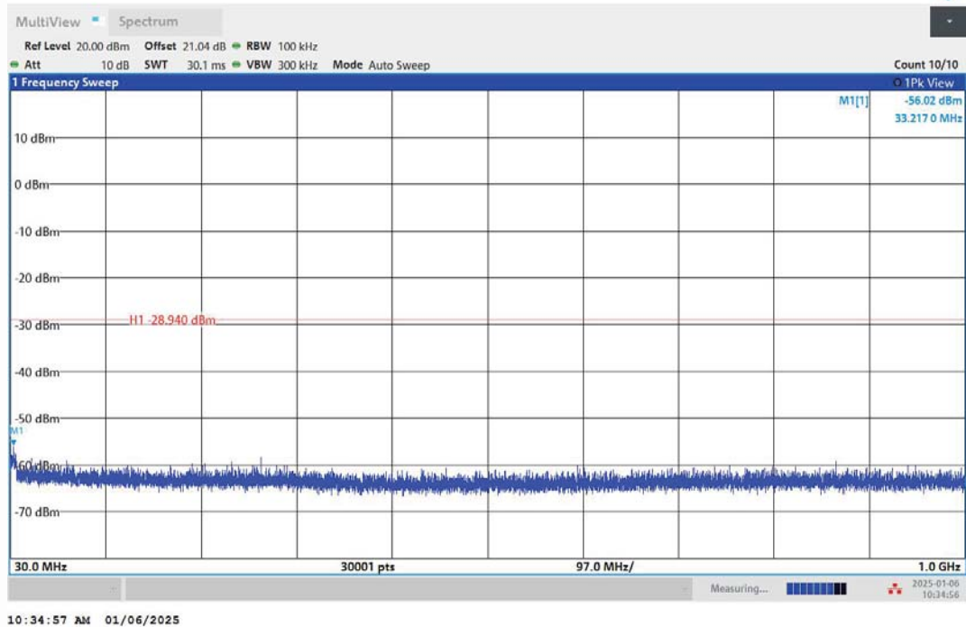
11G-Ant2-2437-30~1000-PASS
