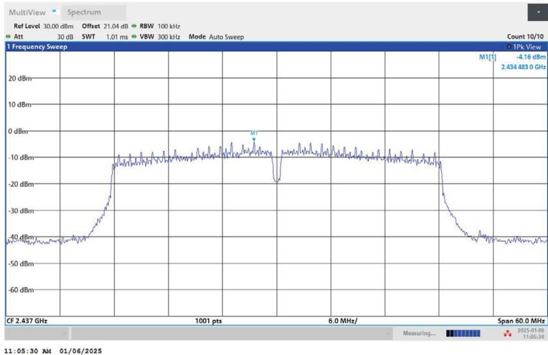
11N40MIMO-Ant2-2437-0~Reference-PASS
