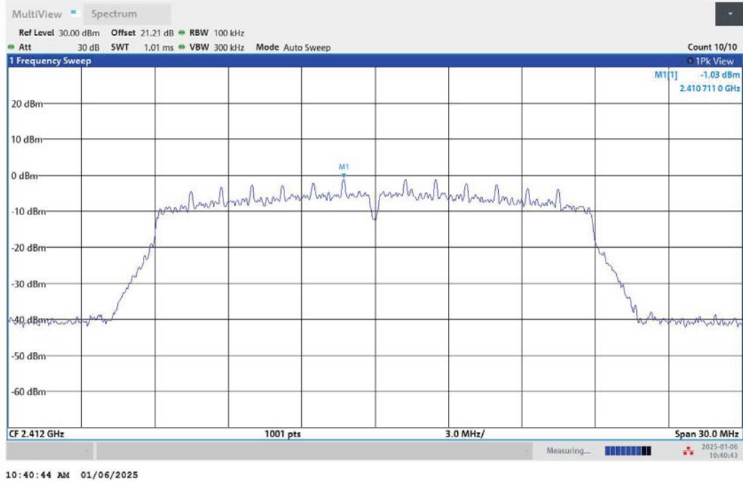
11N20MIMO-Ant1-2412-0~Reference-PASS
