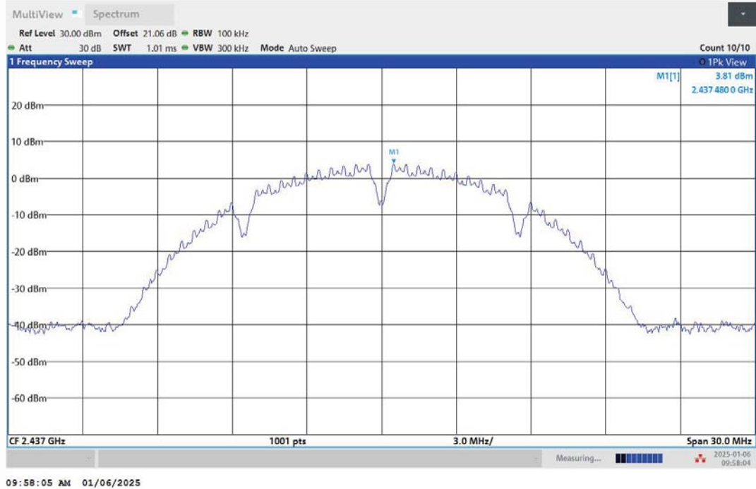
11B-Ant1-2437-0~Reference-PASS
