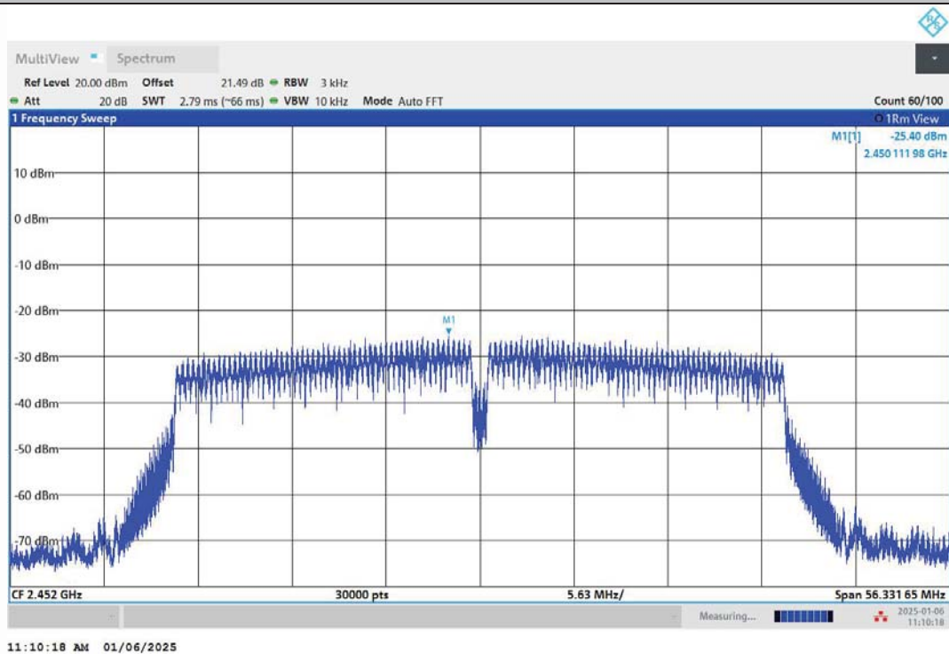
11N40MIMO-Ant2-2452-PASS
