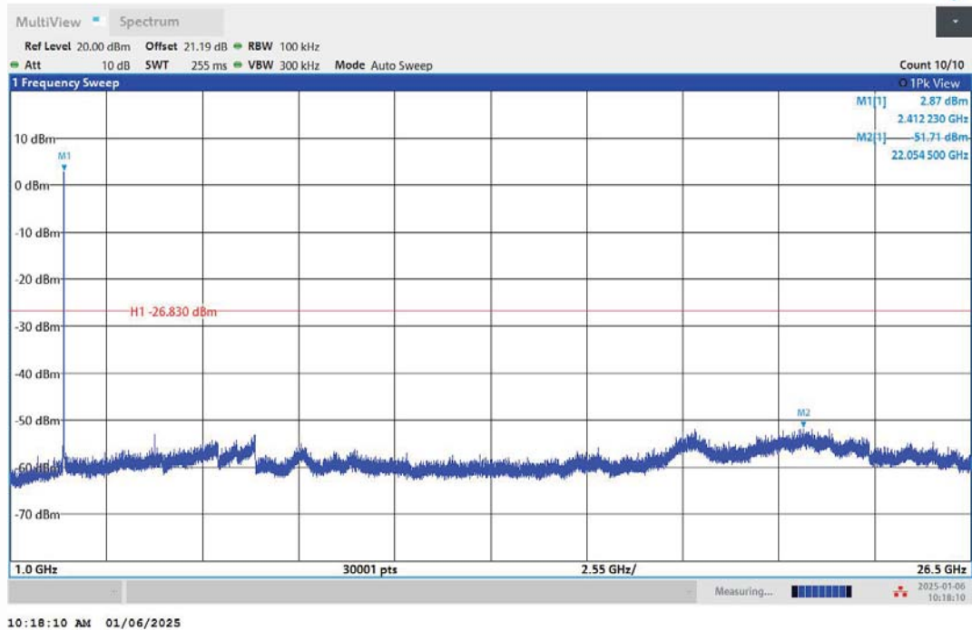
11B-Ant2-2412-1000~26500-PASS
