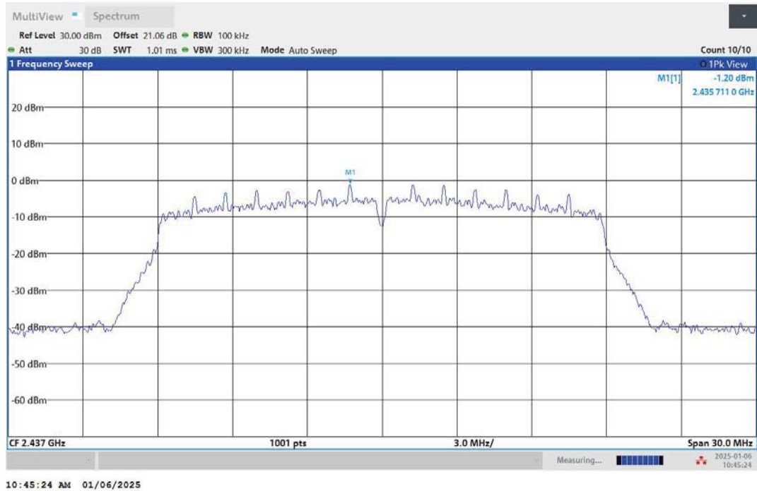
11N20MIMO-Ant1-2437-0~Reference-PASS
