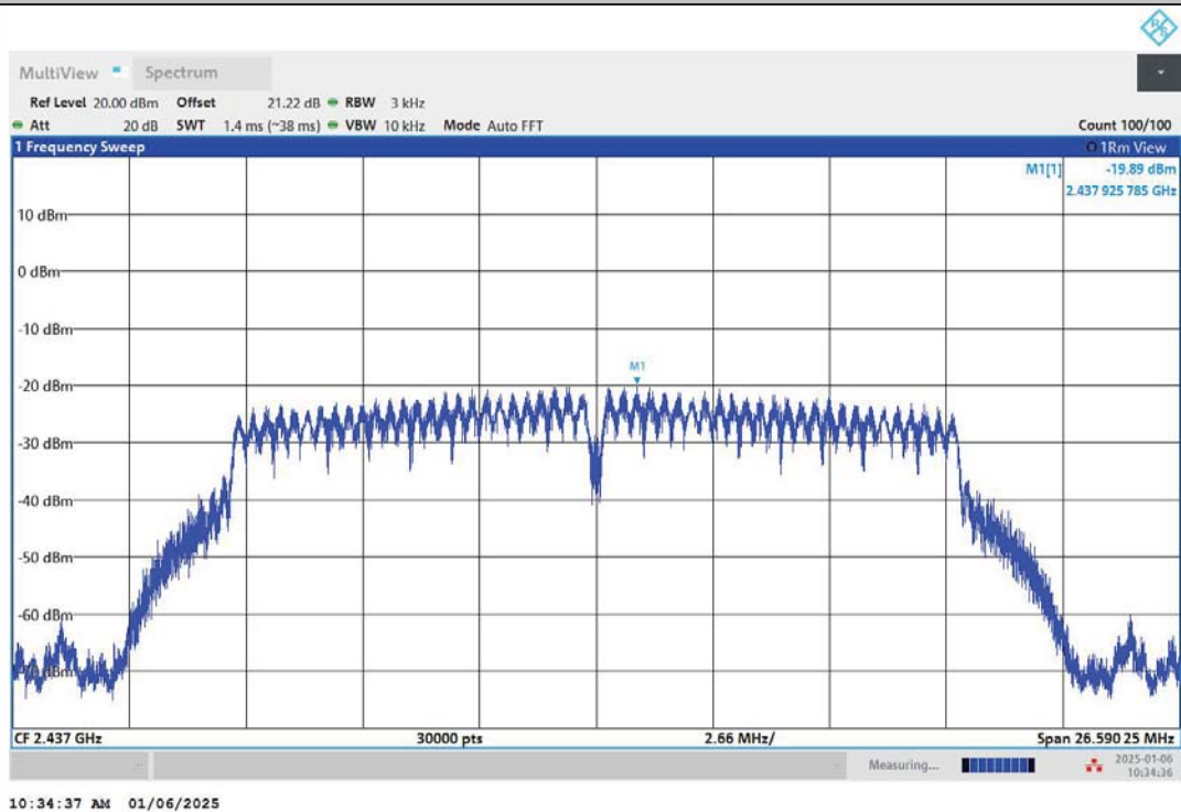
11G-Ant2-2437-PASS
