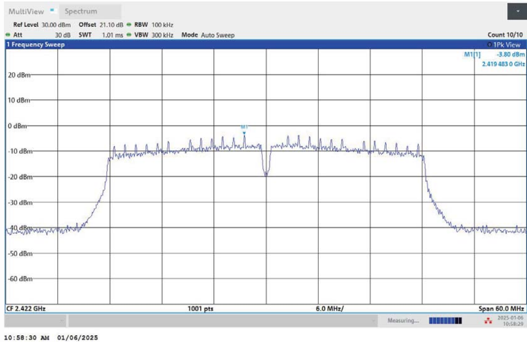
11N40MIMO-Ant1-2422-0~Reference-PASS
