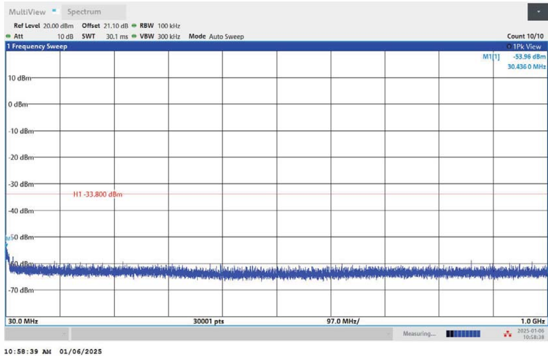
11N40MIMO-Ant1-2422-30~1000-PASS
