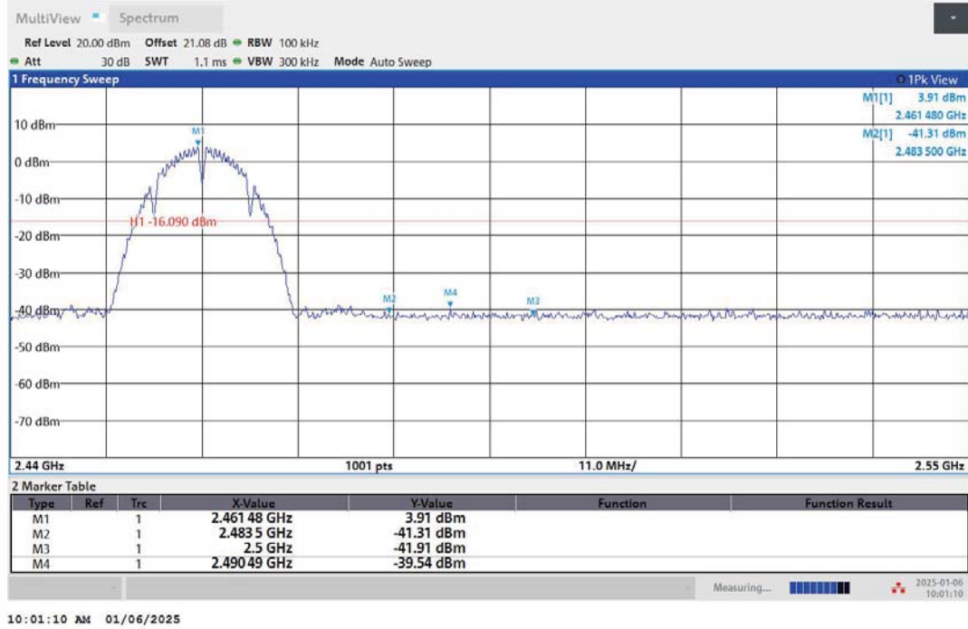
11B-Ant1-2462-PASS
