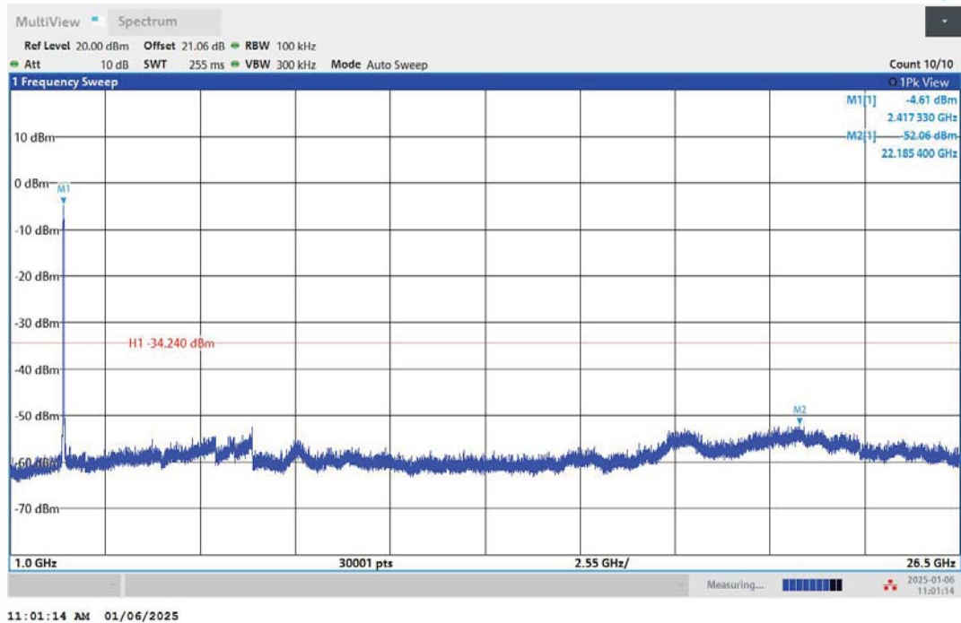
11N40MIMO-Ant2-2422-1000~26500-PASS
