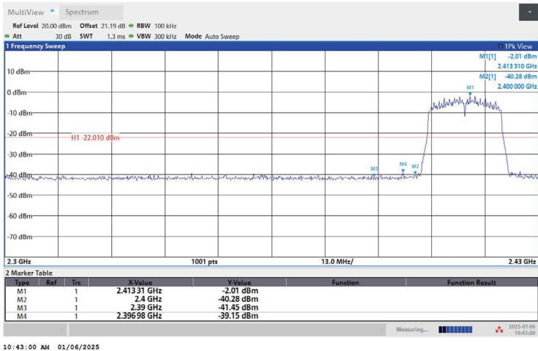
11N20MIMO-Ant2-2412-PASS
