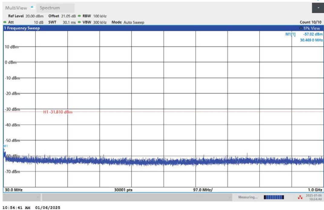
11N20MIMO-Ant2-2462-30~1000-PASS
