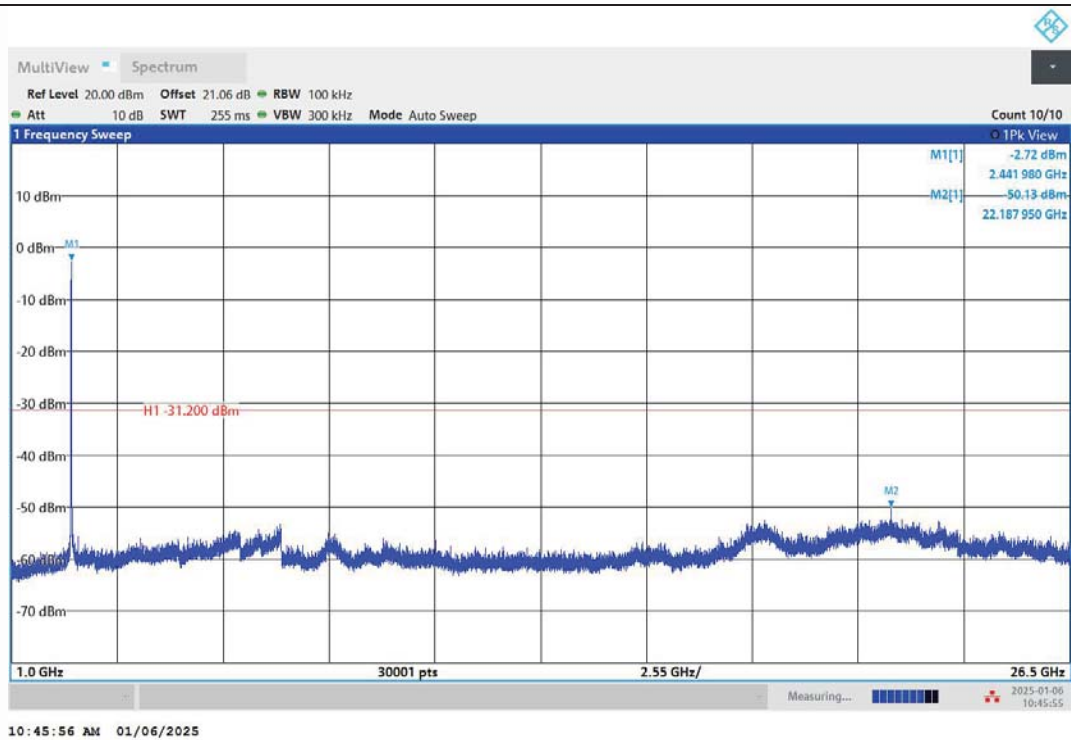
11N20MIMO-Ant1-2437-1000~26500-PASS
