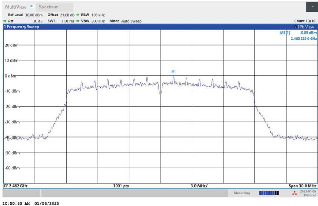
11N20MIMO-Ant1-2462-0~Reference-PASS
