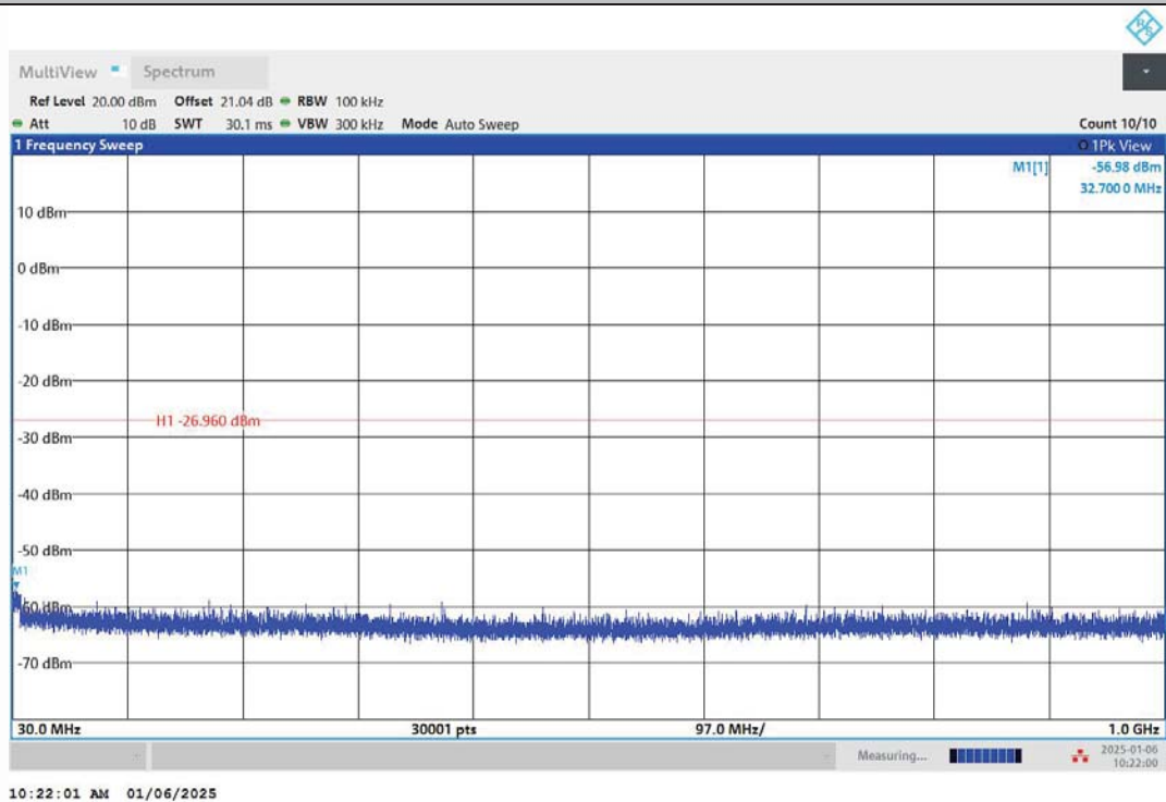
11B-Ant2-2437-30~1000-PASS
