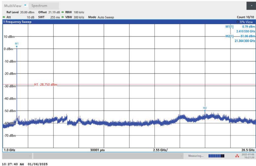
11G-Ant2-2412-1000~26500-PASS
