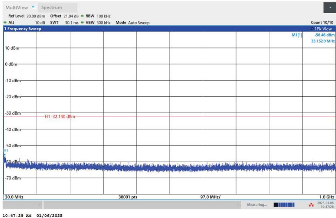
11N20MIMO-Ant2-2437-30~1000-PASS
