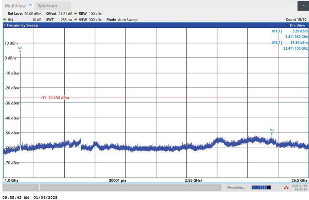
11B-Ant1-2412-1000~26500-PASS
