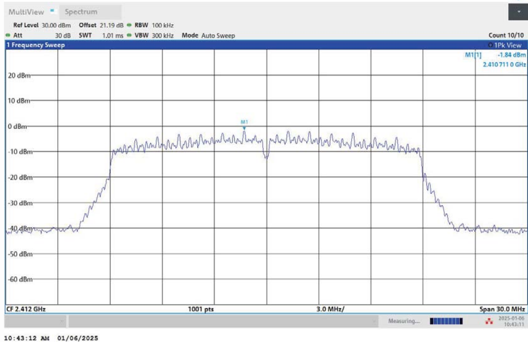
11N20MIMO-Ant2-2412-0~Reference-PASS
