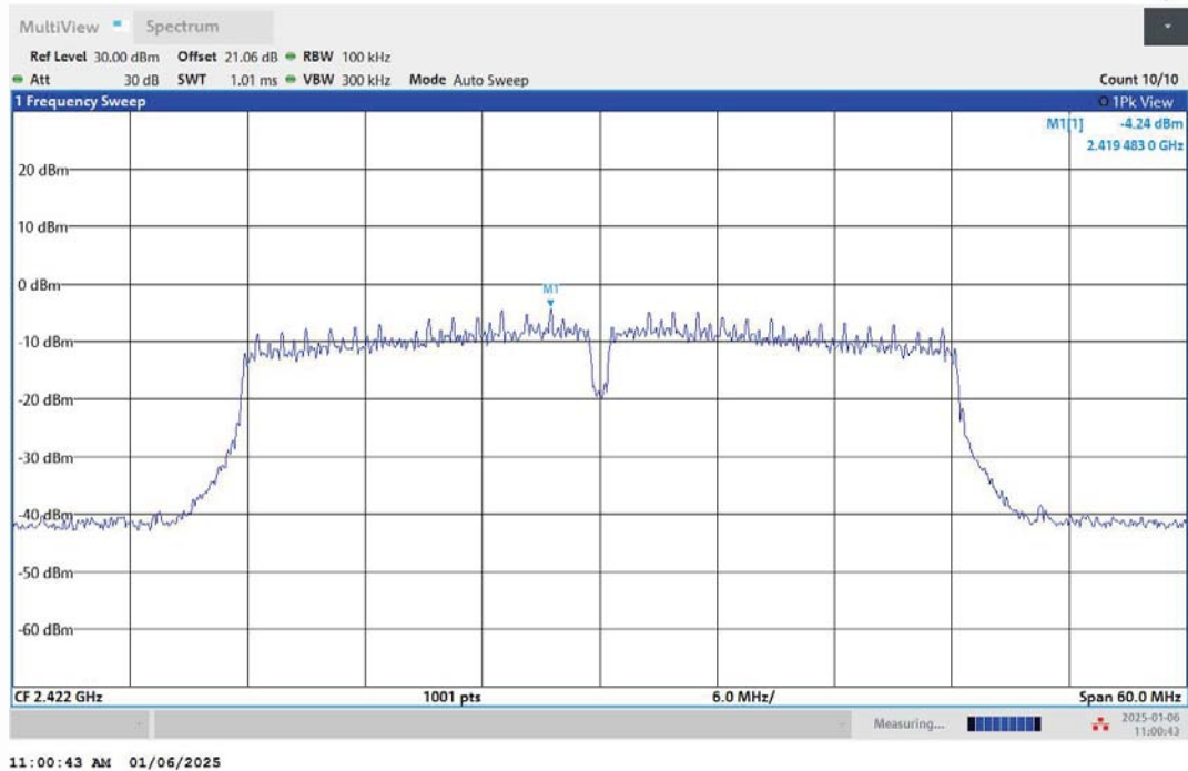
11N40MIMO-Ant2-2422-0~Reference-PASS
