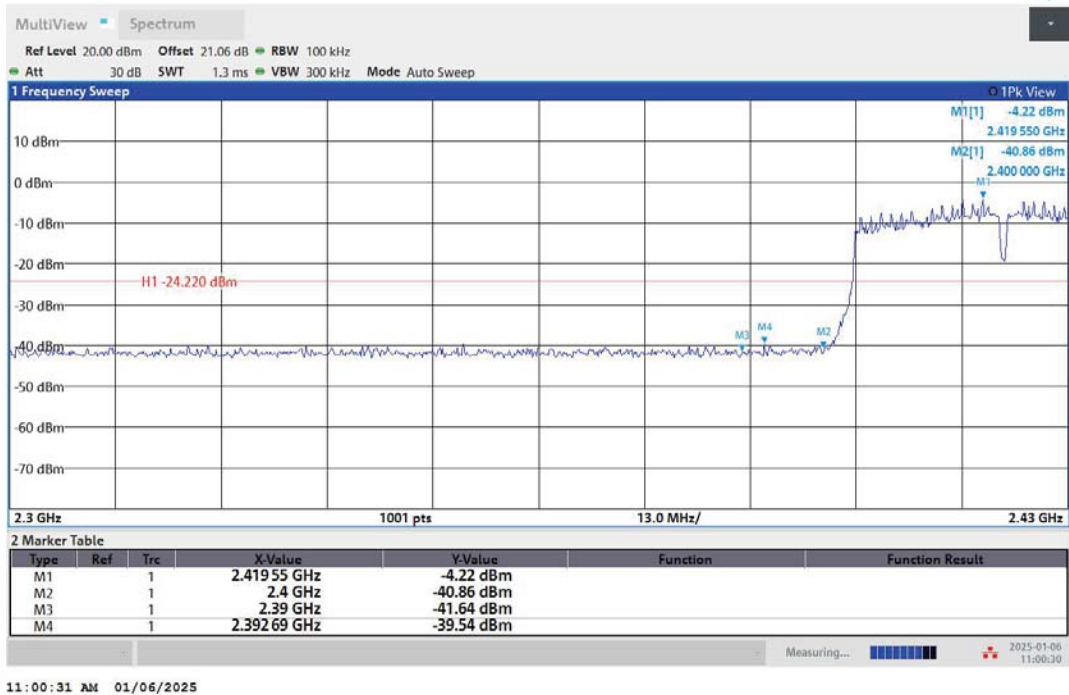
11N40MIMO-Ant2-2422-PASS
