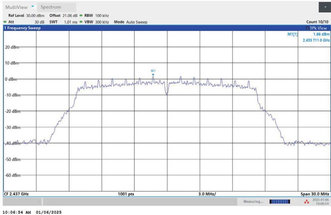
11G-Ant1-2437-0~Reference-PASS
