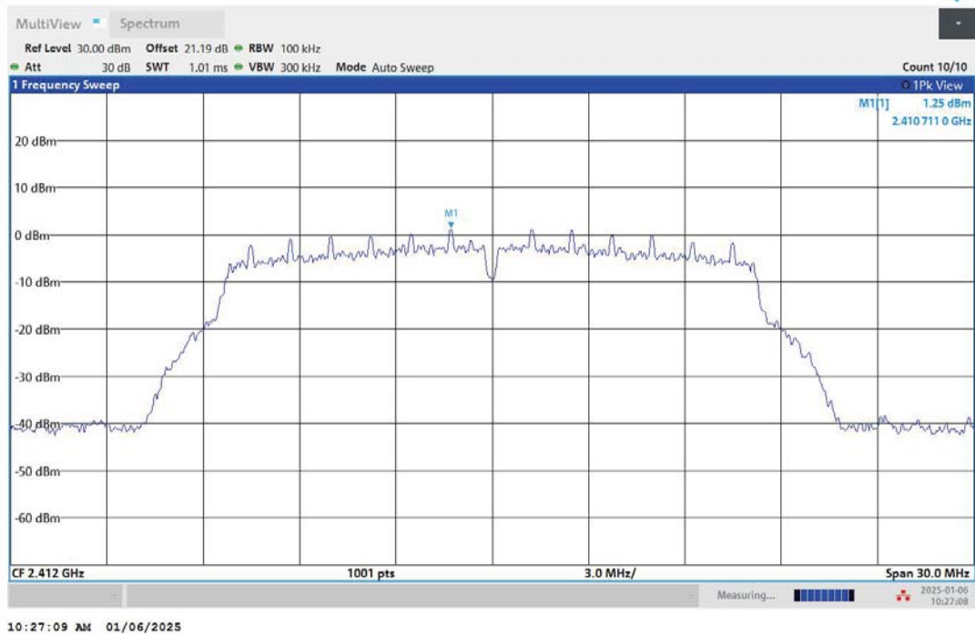
11G-Ant2-2412-0~Reference-PASS
