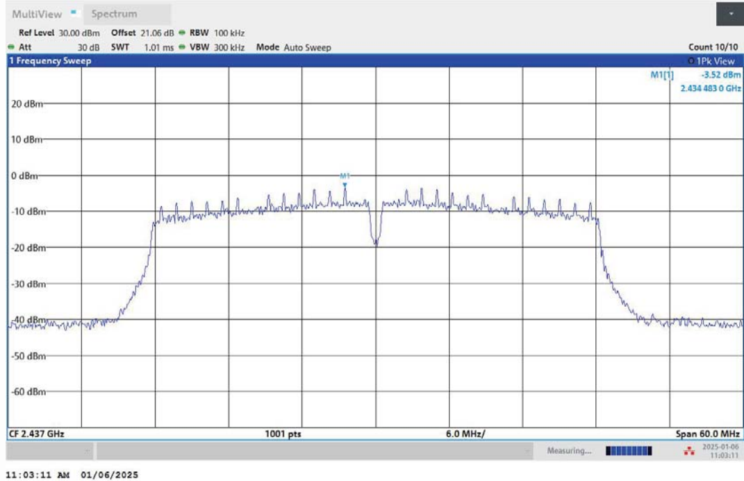
11N40MIMO-Ant1-2437-0~Reference-PASS
