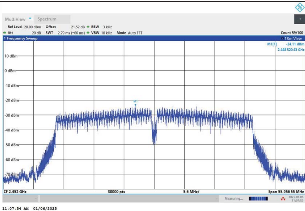
11N40MIMO-Ant1-2452-PASS
