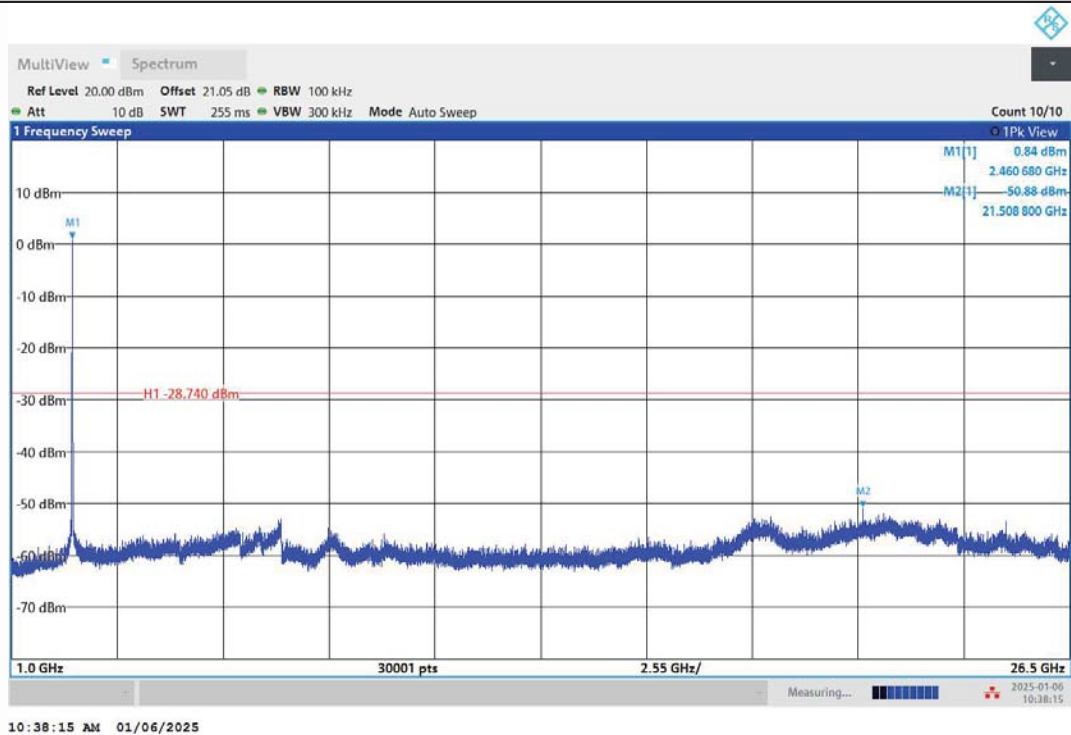
11G-Ant2-2462-1000~26500-PASS
