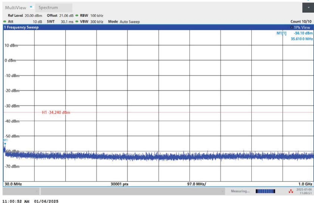
11N40MIMO-Ant2-2422-30~1000-PASS
