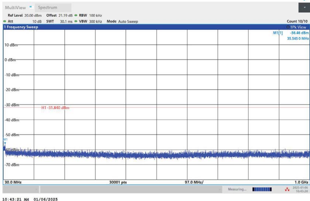
11N20MIMO-Ant2-2412-30~1000-PASS
