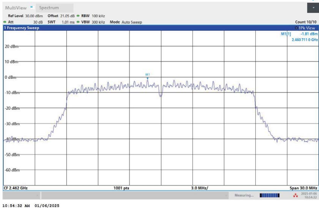
11N20MIMO-Ant2-2462-0~Reference-PASS
