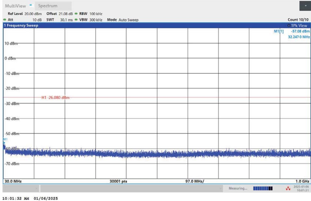
11B-Ant1-2462-30~1000-PASS
