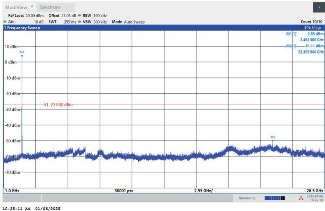
11B-Ant2-2462-1000~26500-PASS
