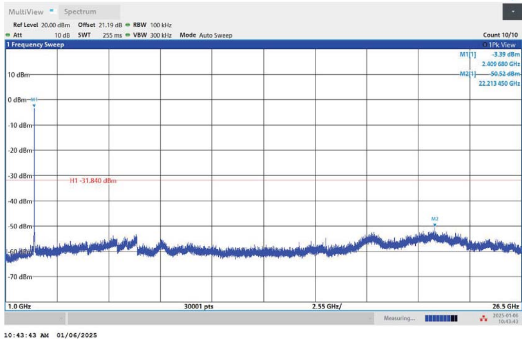
11N20MIMO-Ant2-2412-1000~26500-PASS
