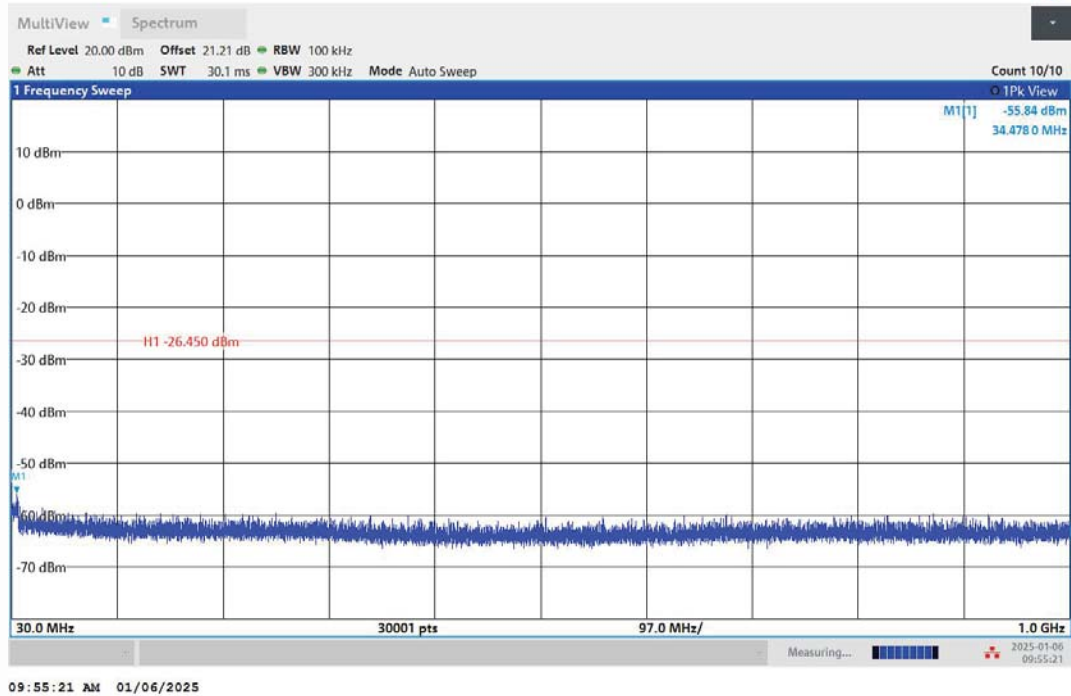
11B-Ant1-2412-30~1000-PASS
