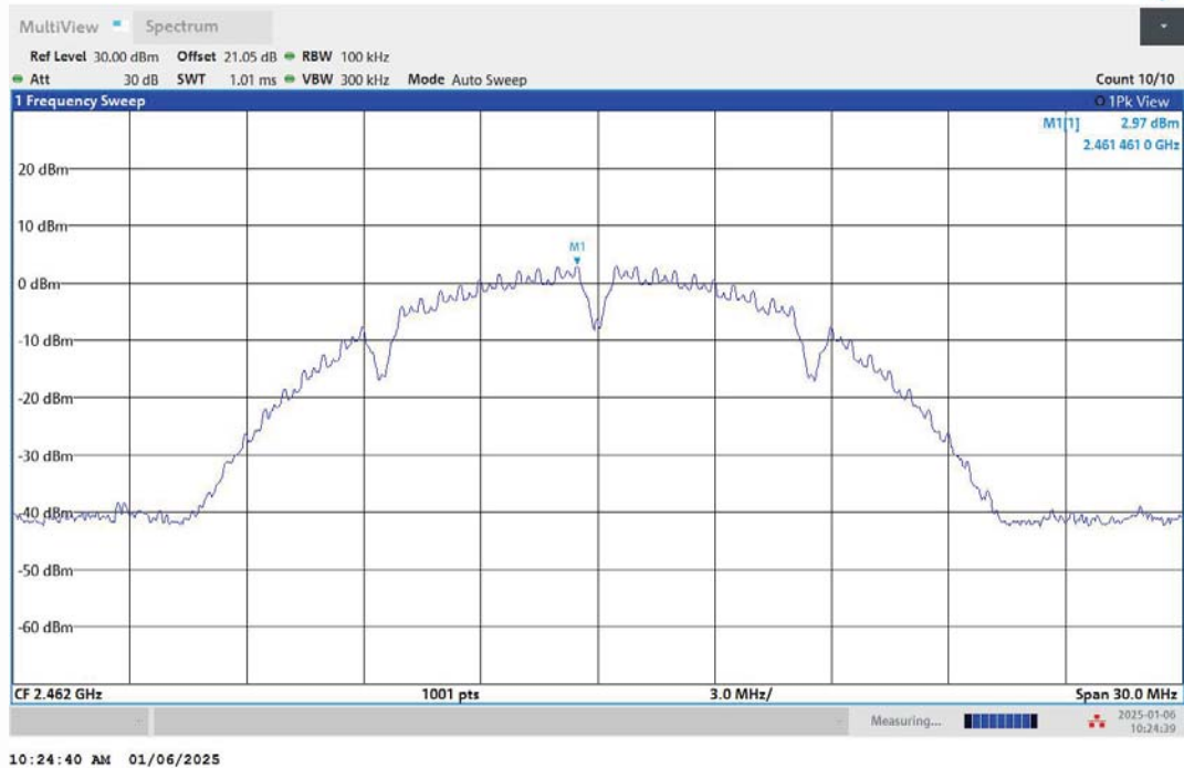
11B-Ant2-2462-0~Reference-PASS
