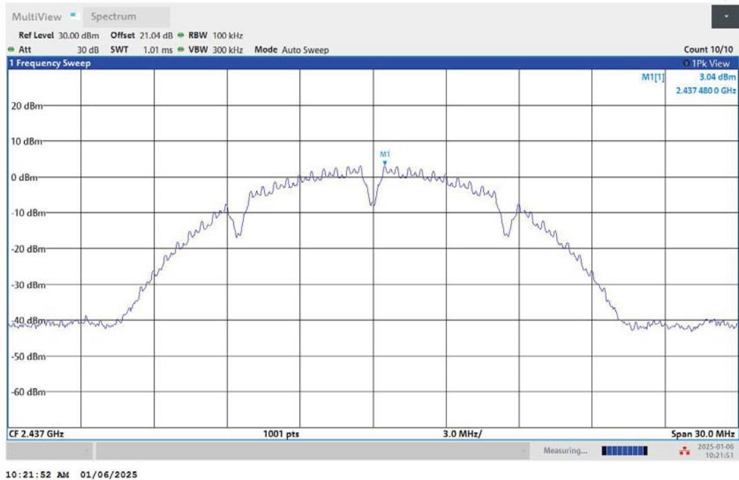
11B-Ant2-2437-0~Reference-PASS
