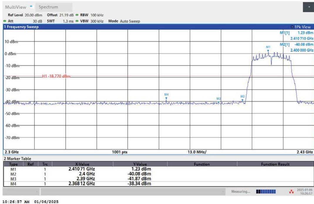
11G-Ant2-2412-PASS
