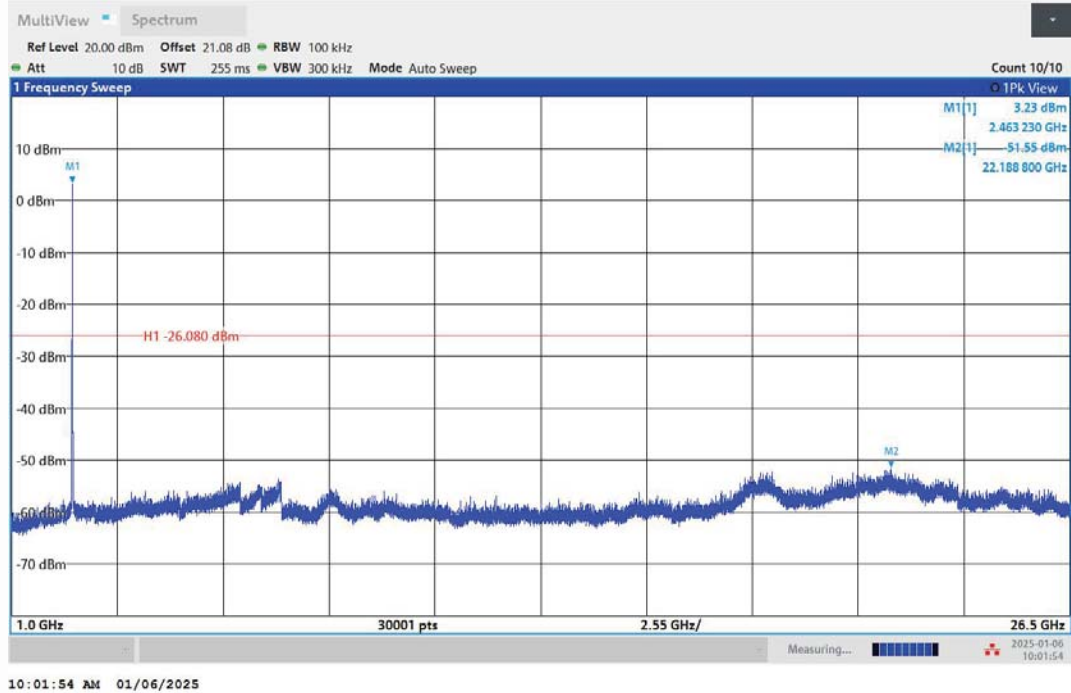
11B-Ant1-2462-1000~26500-PASS
