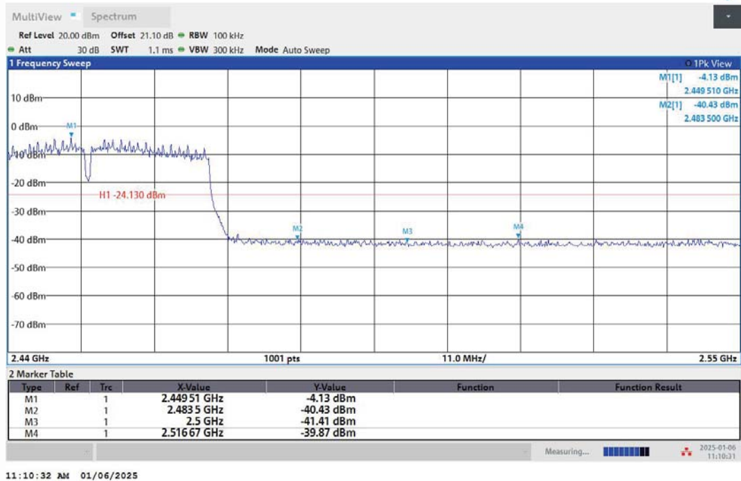
11N40MIMO-Ant2-2452-PASS
