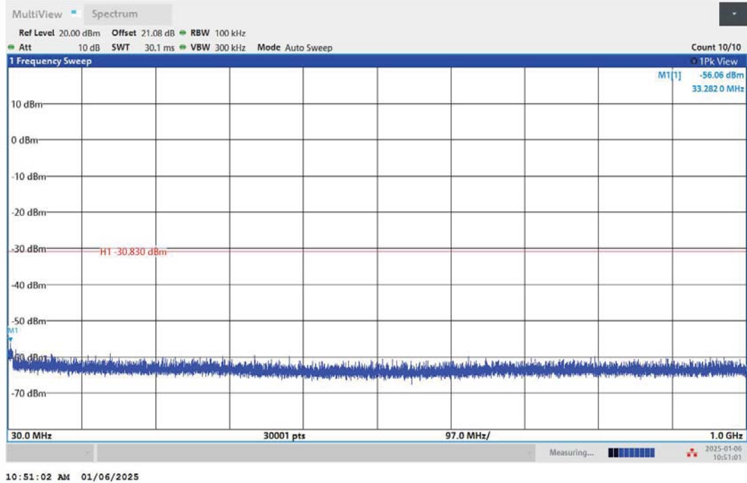
11N20MIMO-Ant1-2462-30~1000-PASS
