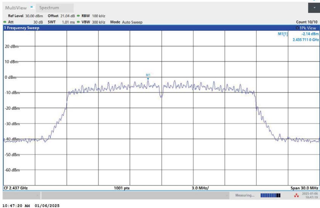
11N20MIMO-Ant2-2437-0~Reference-PASS
