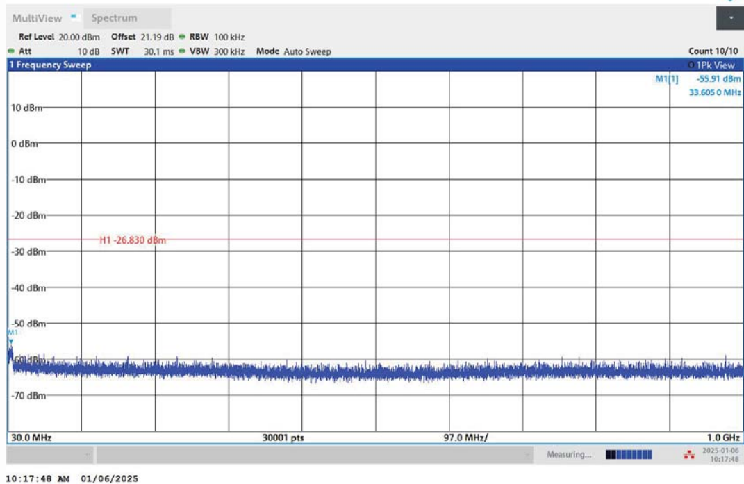
11B-Ant2-2412-30~1000-PASS
