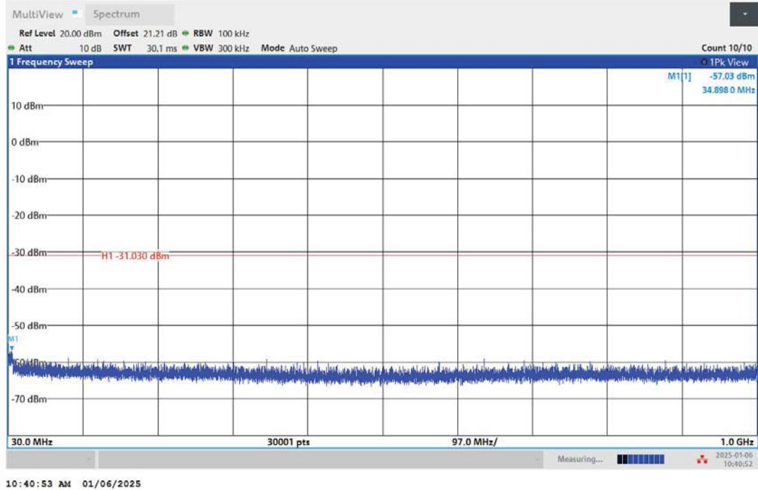
11N20MIMO-Ant1-2412-30~1000-PASS
