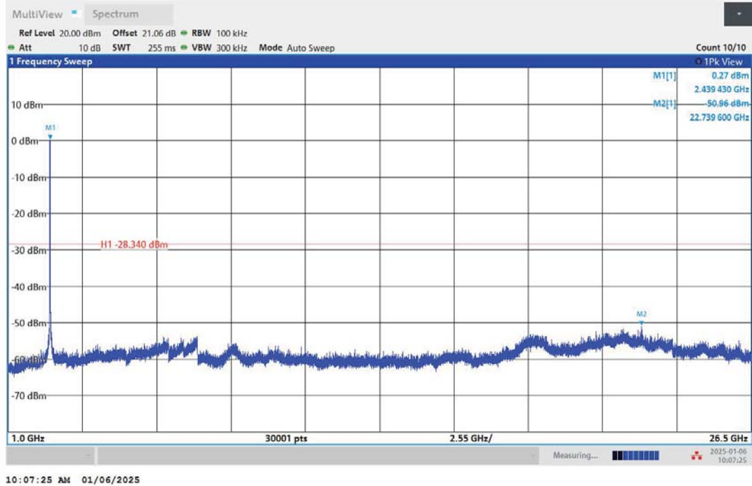
11G-Ant1-2437-1000~26500-PASS
