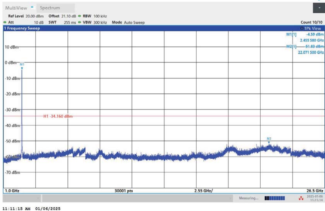
11N40MIMO-Ant2-2452-1000~26500-PASS
