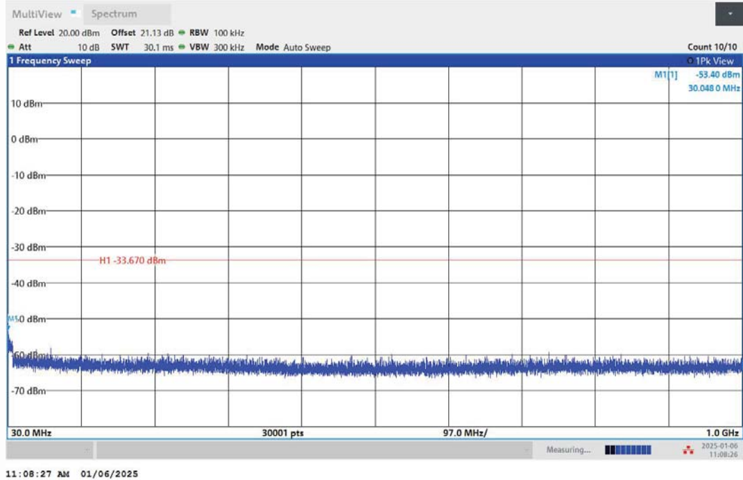
11N40MIMO-Ant1-2452-30~1000-PASS
