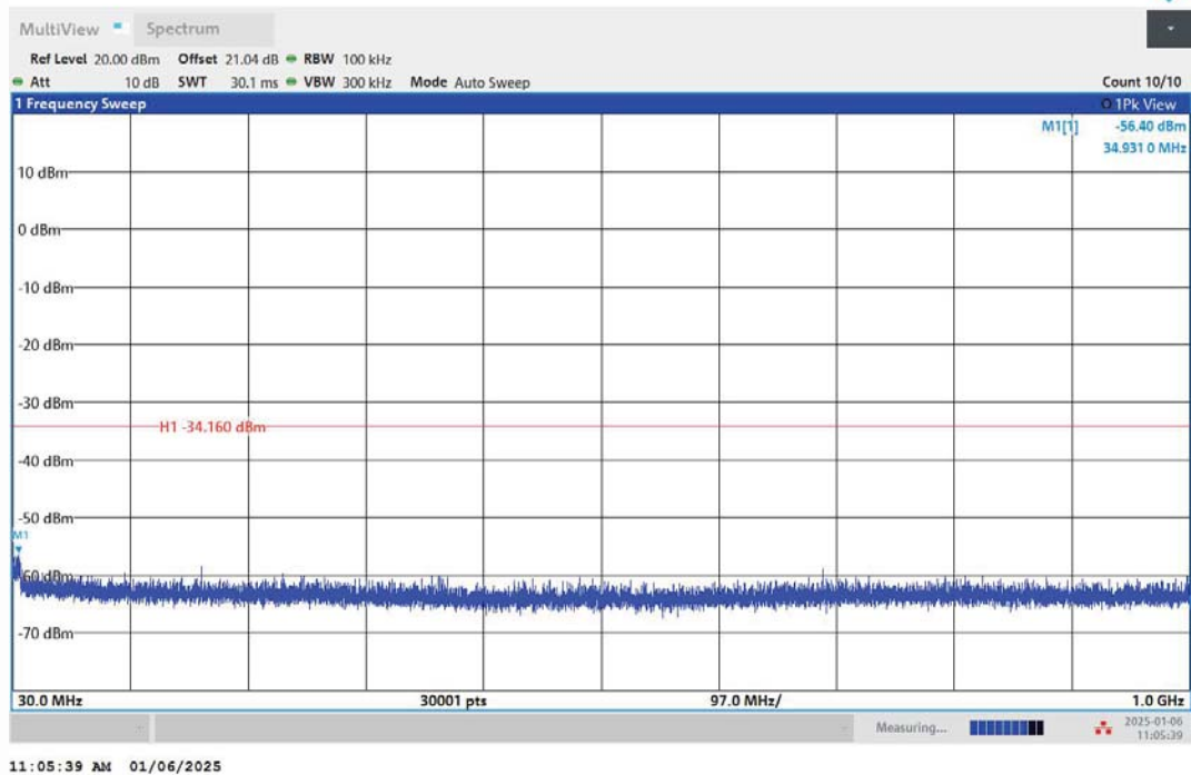
11N40MIMO-Ant2-2437-30~1000-PASS
