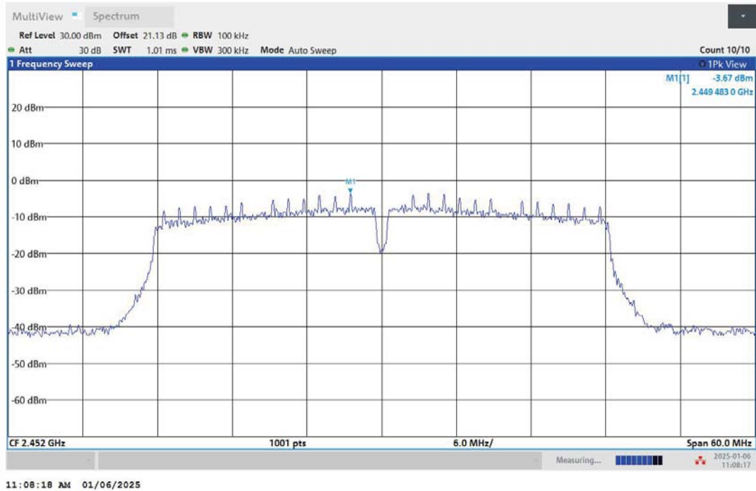
11N40MIMO-Ant1-2452-0~Reference-PASS
