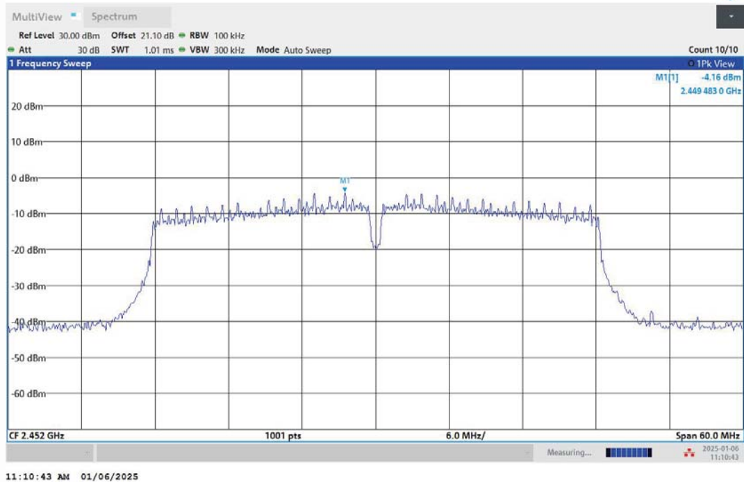
11N40MIMO-Ant2-2452-0~Reference-PASS
