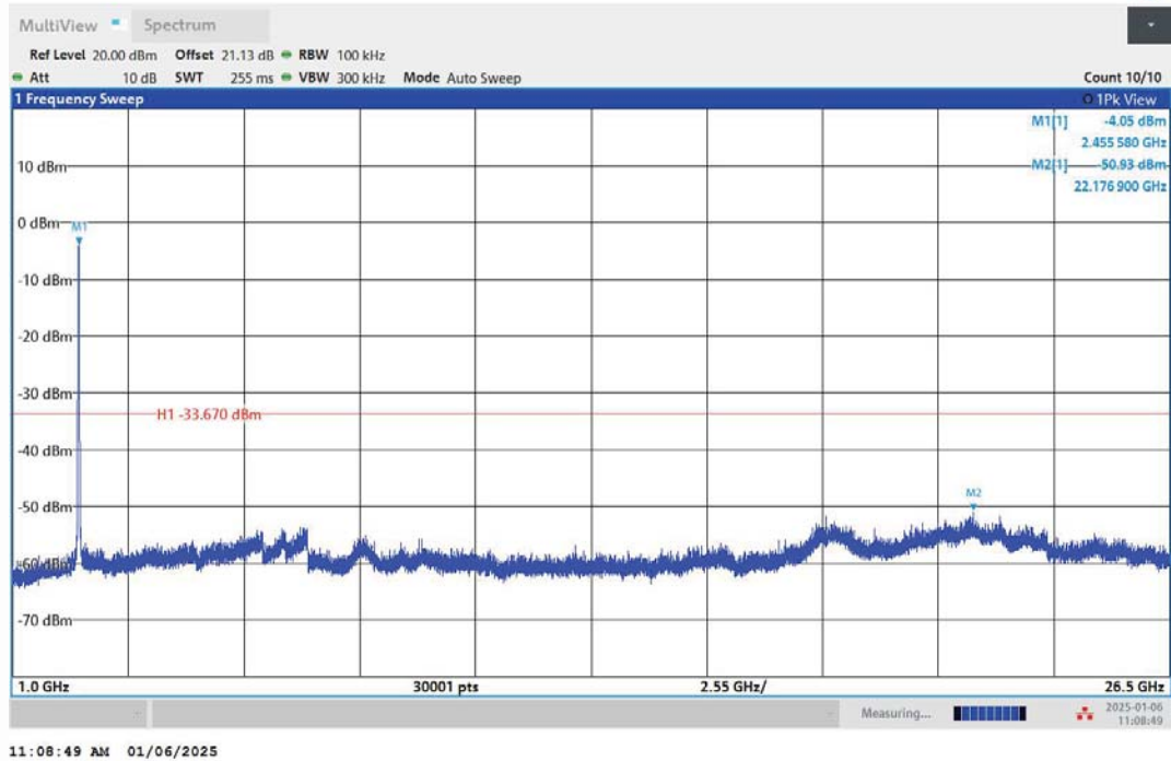
11N40MIMO-Ant1-2452-1000~26500-PASS
