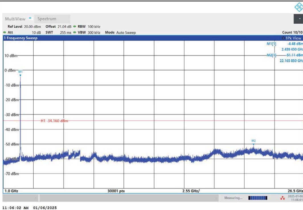
11N40MIMO-Ant2-2437-1000~26500-PASS
