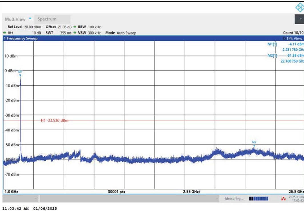
11N40MIMO-Ant1-2437-1000~26500-PASS
