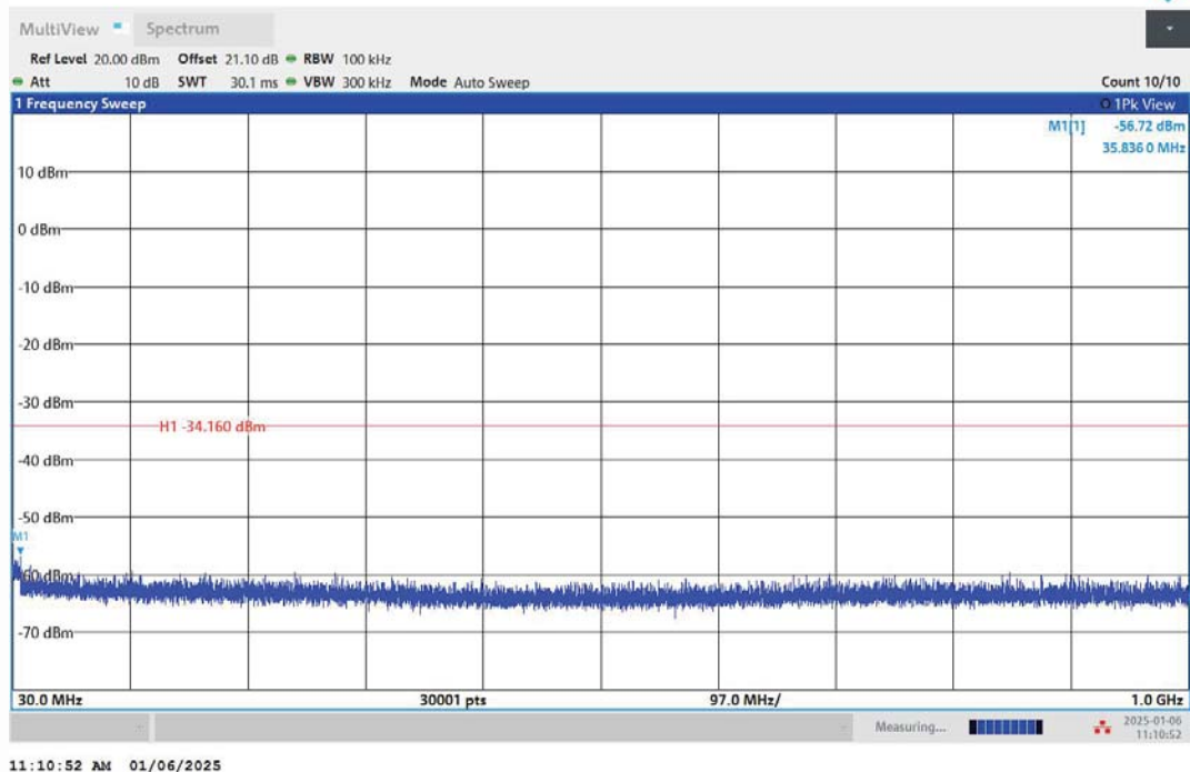
11N40MIMO-Ant2-2452-30~1000-PASS
