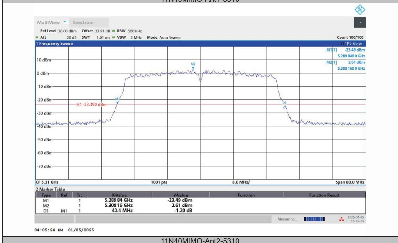
11N40MIMO-Ant2-5310
