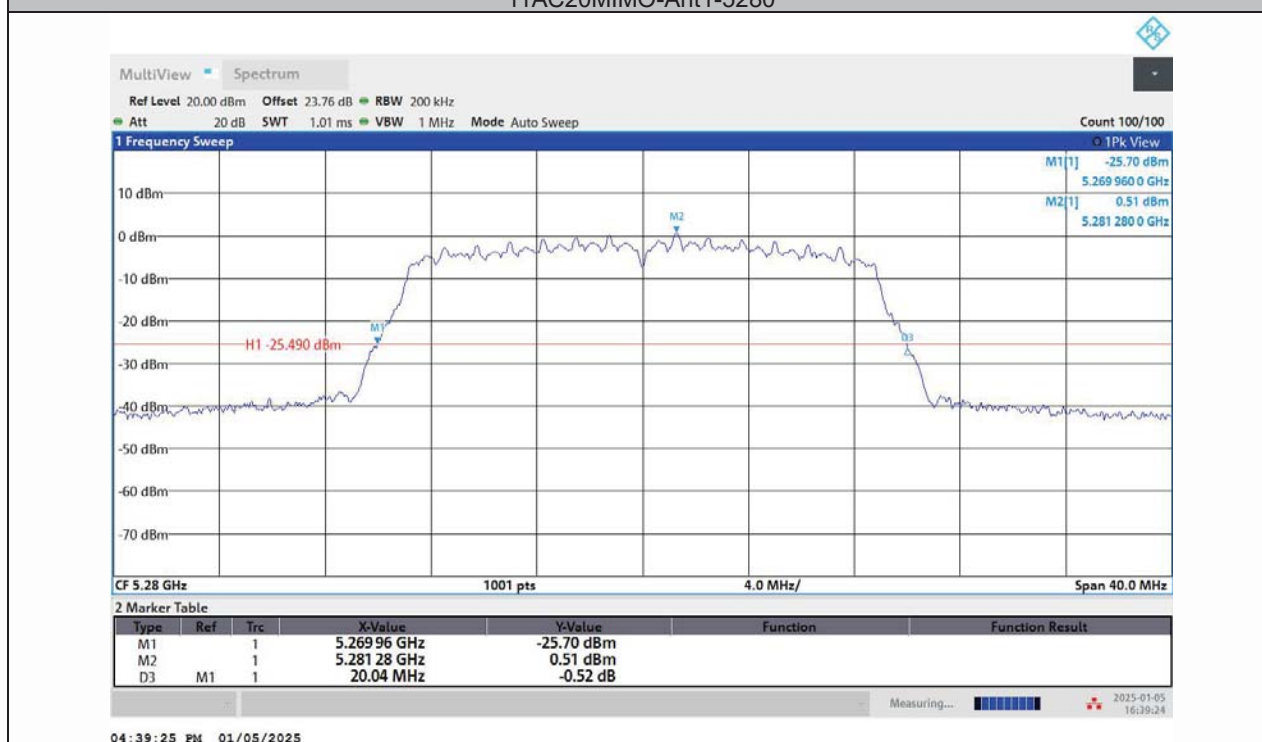
11AC20MIMO-Ant2-5280
