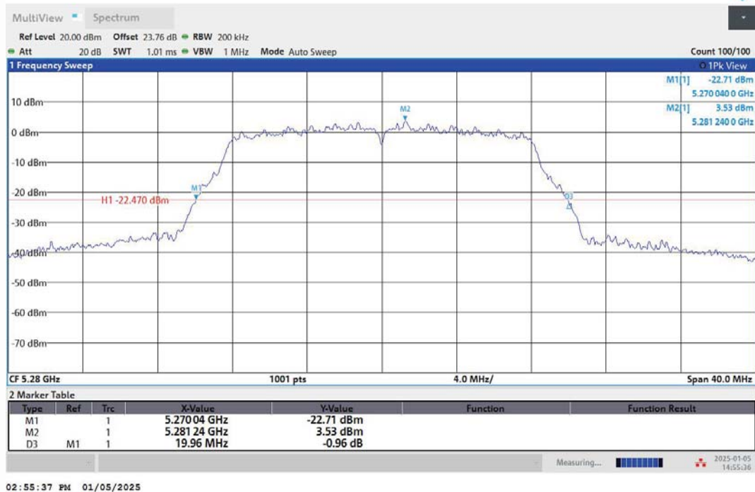
11A-Ant2-5280
