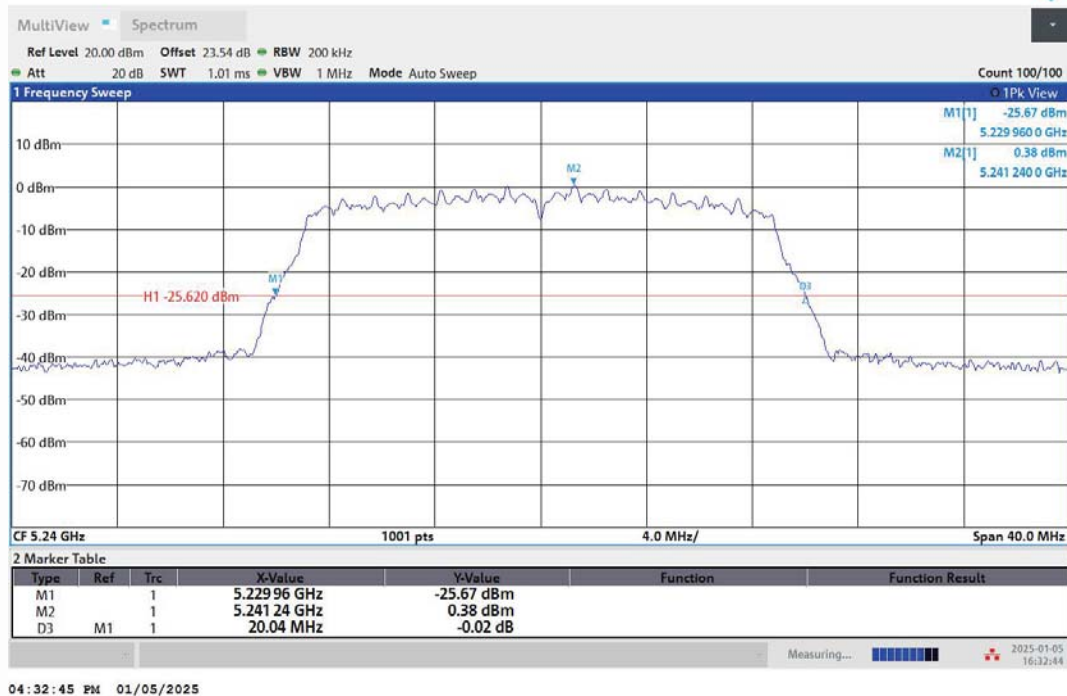
11AC20MIMO-Ant2-5240
