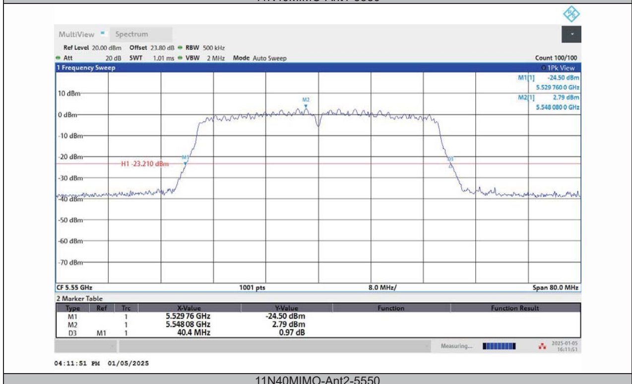
11N40MIMO-Ant2-5550
