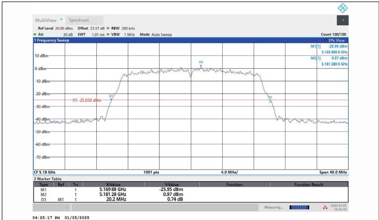
11AC20MIMO-Ant1-5180
