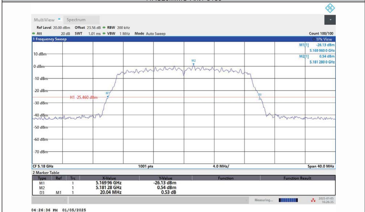
11AC20MIMO-Ant2-5180
