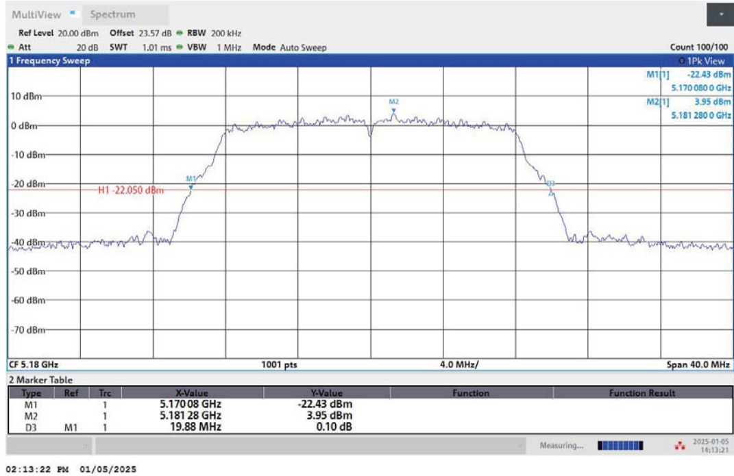
11A-Ant1-5180
