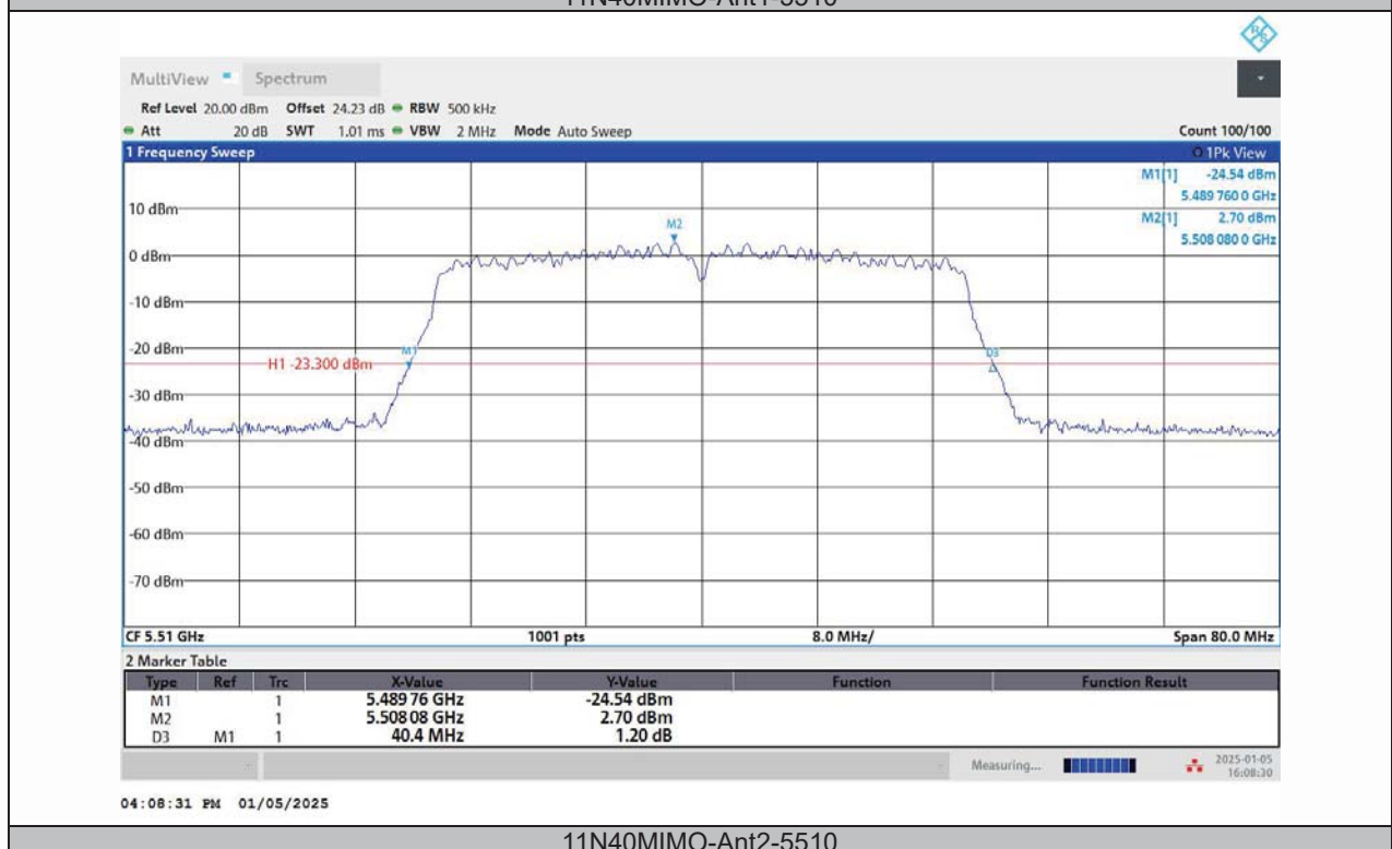
11N40MIMO-Ant2-5510
