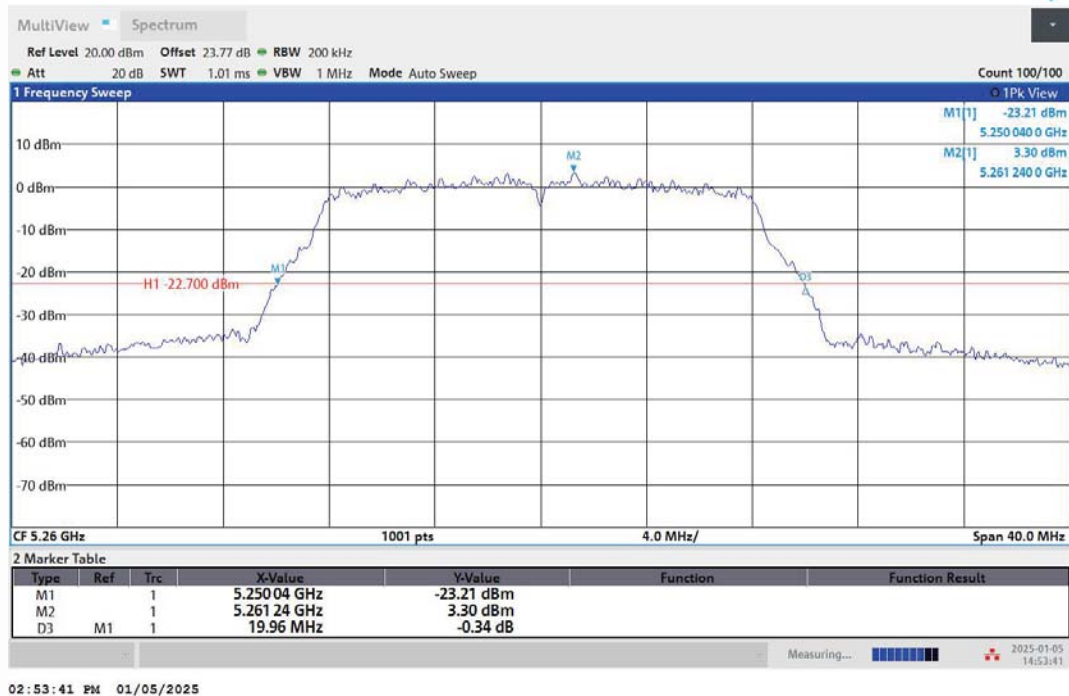
11A-Ant2-5260
