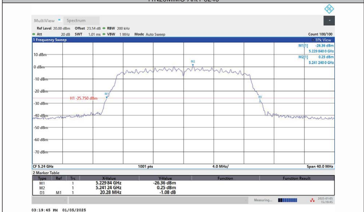
11N20MIMO-Ant2-5240
