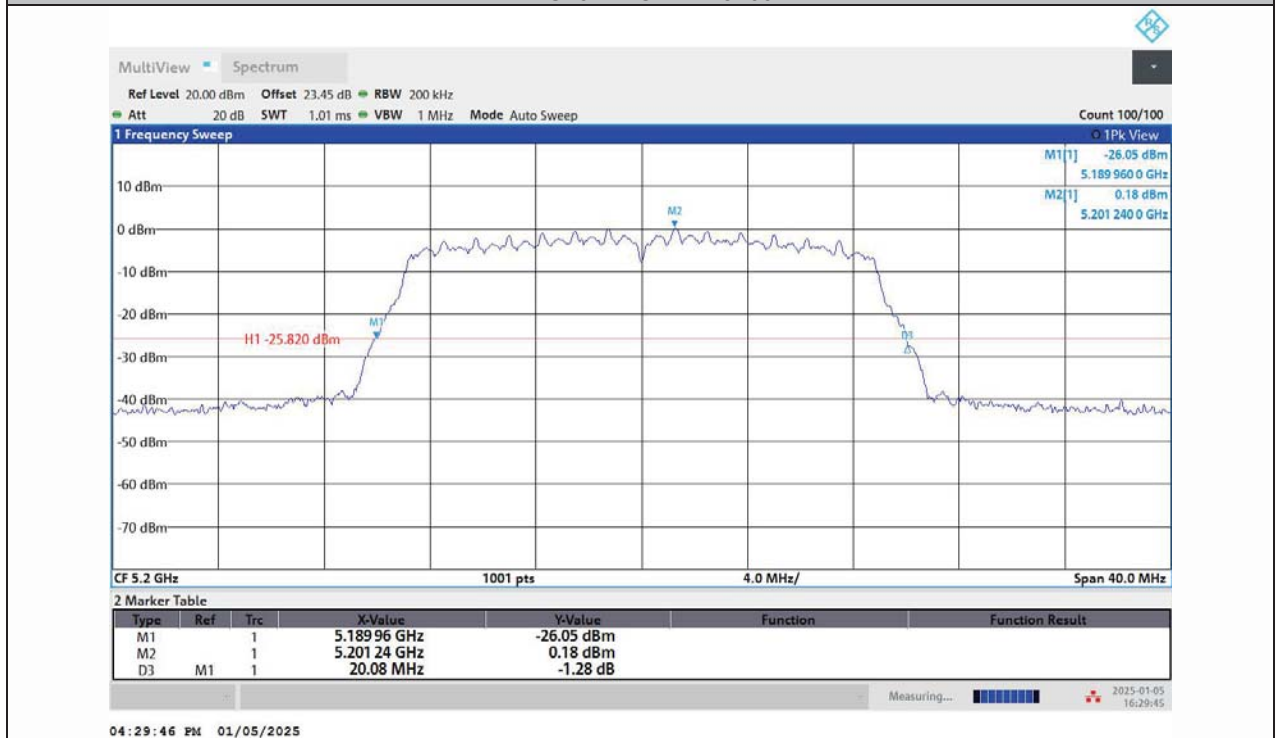
11AC20MIMO-Ant2-5200
