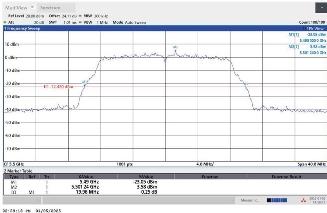
11A-Ant2-5500
