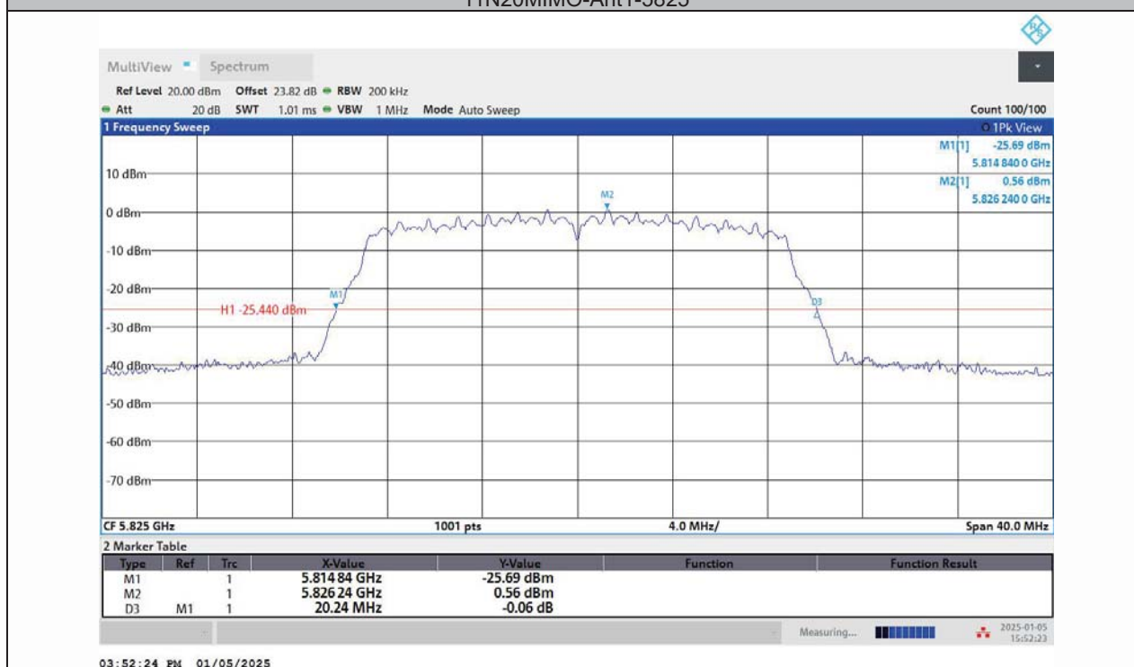
11N20MIMO-Ant2-5825
