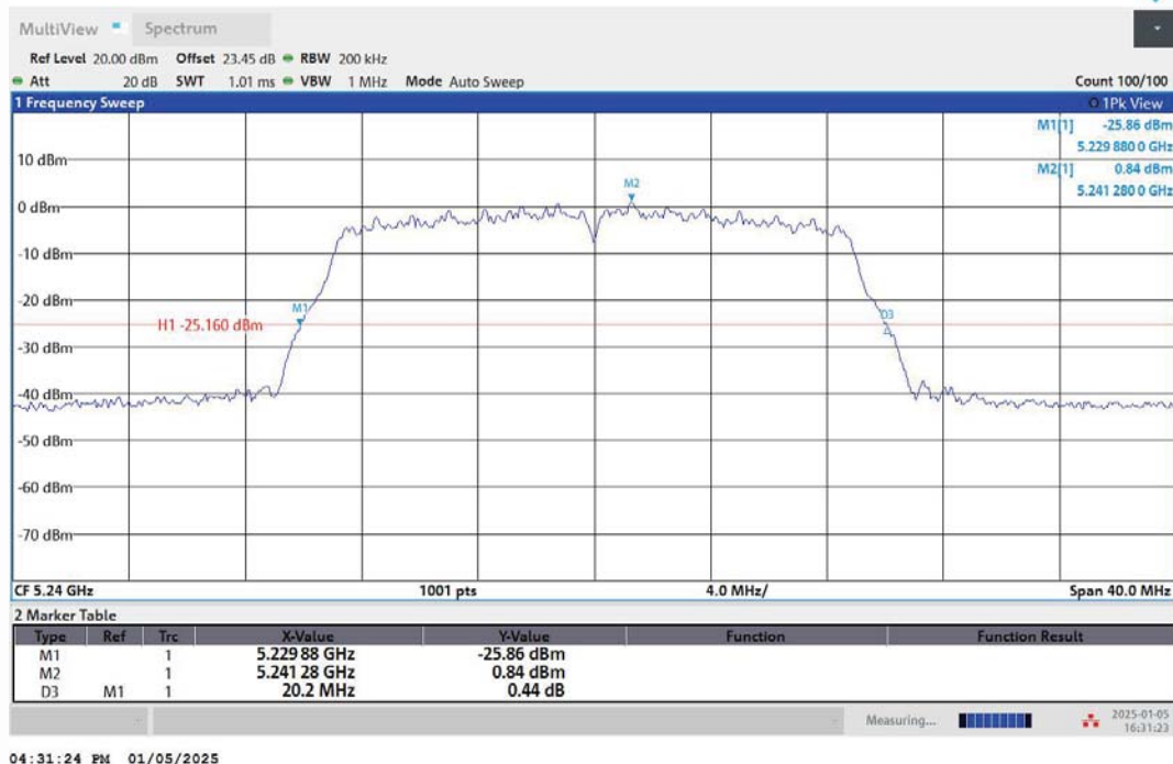
11AC20MIMO-Ant1-5240
