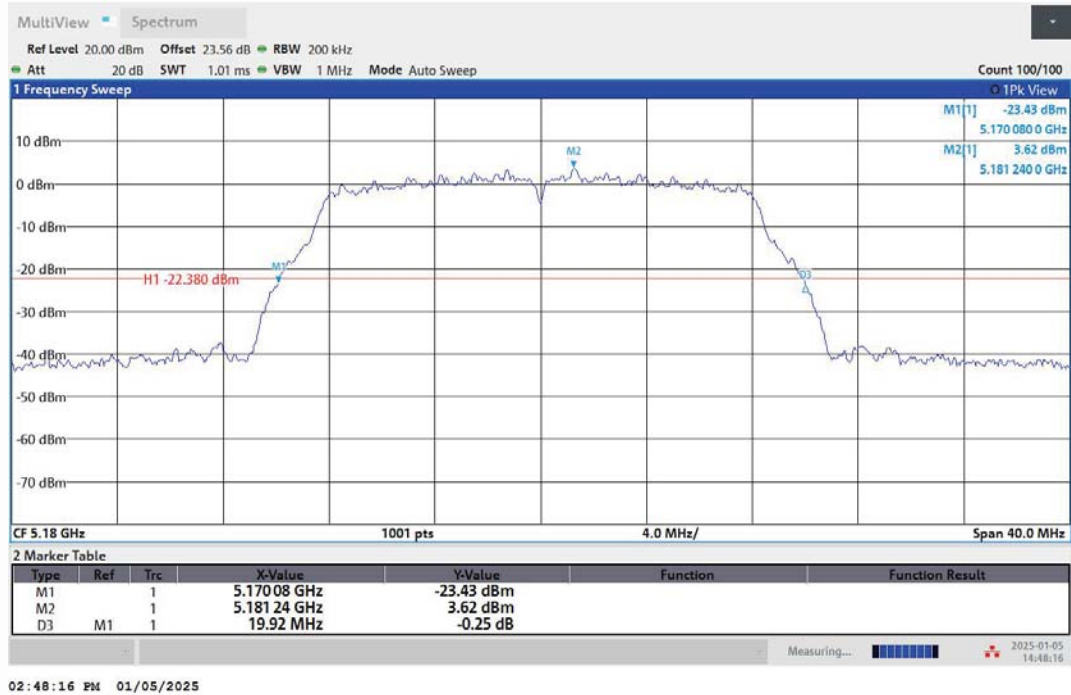
11A-Ant2-5180
