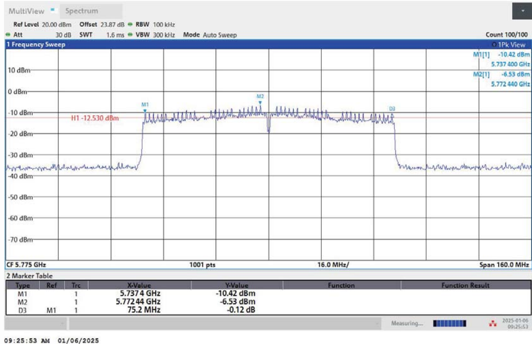
11AC80MIMO-Ant2-5775-PASS
