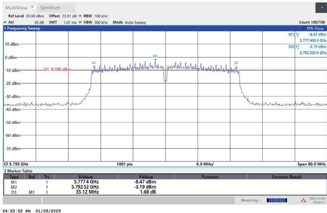
11N40MIMO-Ant2-5795-PASS
