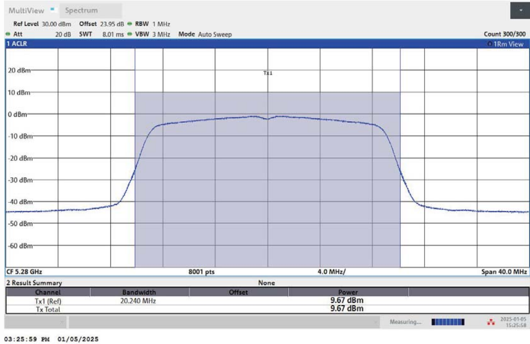
11N20MIMO-Ant1-5280-PASS
