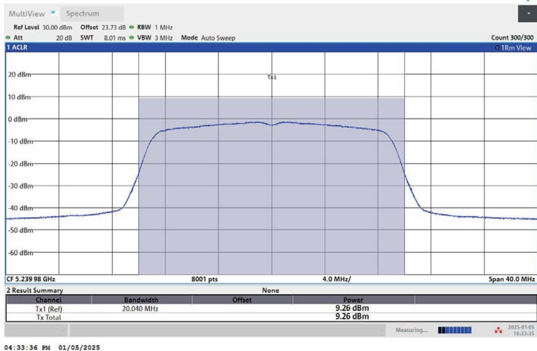
11AC20MIMO-Ant2-5240-PASS
