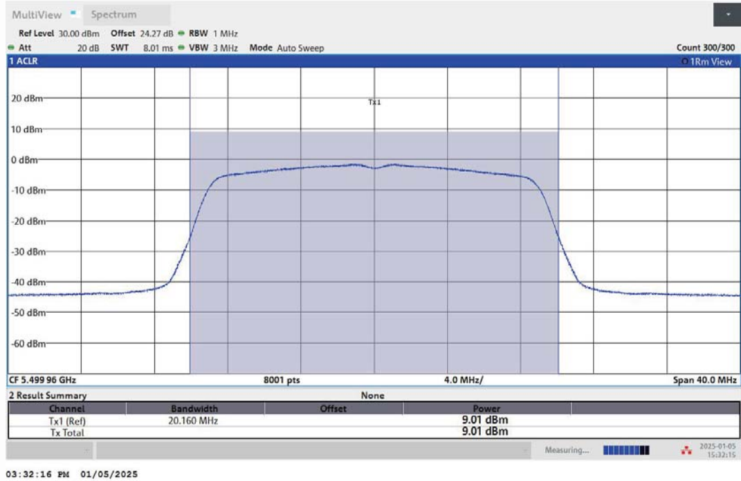
11N20MIMO-Ant1-5500-PASS
