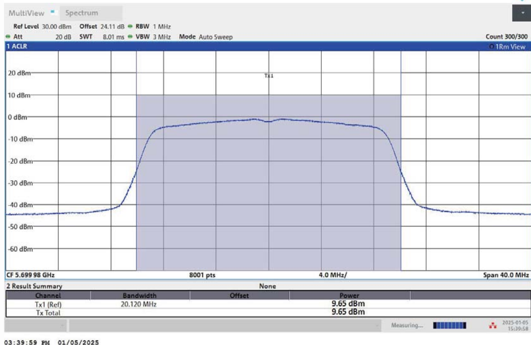
11N20MIMO-Ant1-5700-PASS
