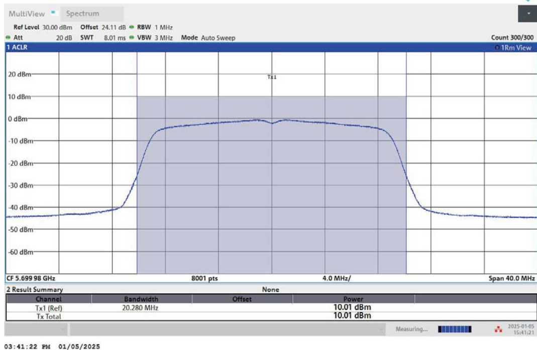
11N20MIMO-Ant2-5700-PASS
