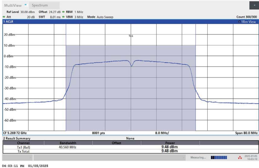
11N40MIMO-Ant2-5270-PASS
