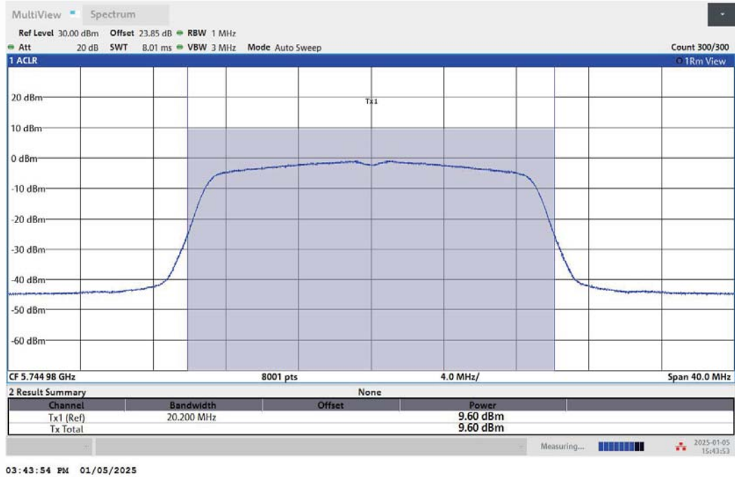
11N20MIMO-Ant1-5745-PASS
