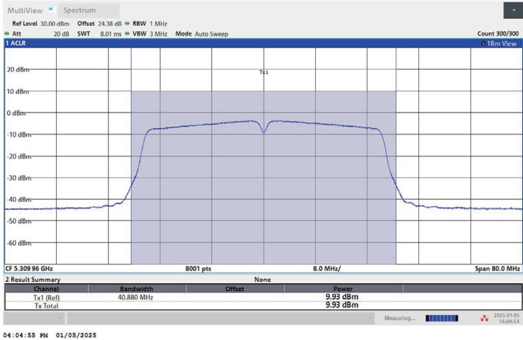
11N40MIMO-Ant1-5310-PASS
