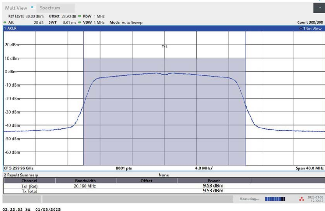
11N20MIMO-Ant1-5260-PASS
