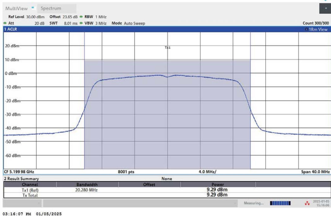
11N20MIMO-Ant2-5200-PASS
