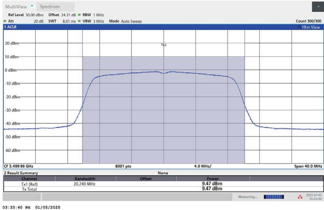
11N20MIMO-Ant2-5500-PASS
