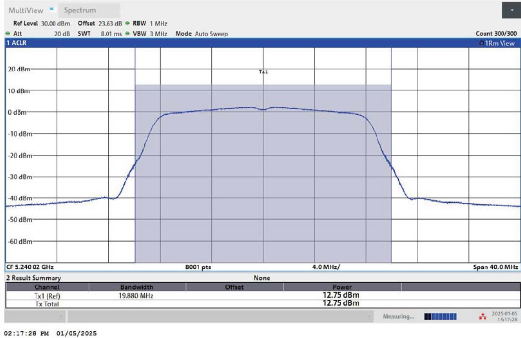
11A-Ant1-5240-PASS
