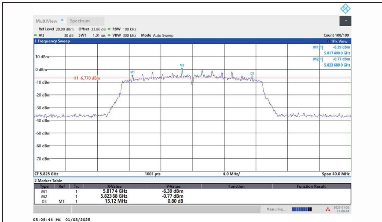
11AC20MIMO-Ant1-5825-PASS
