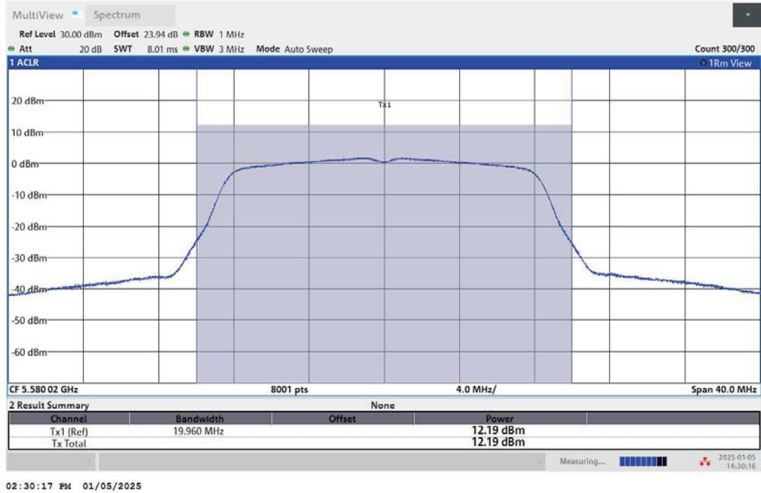
11A-Ant1-5580-PASS
