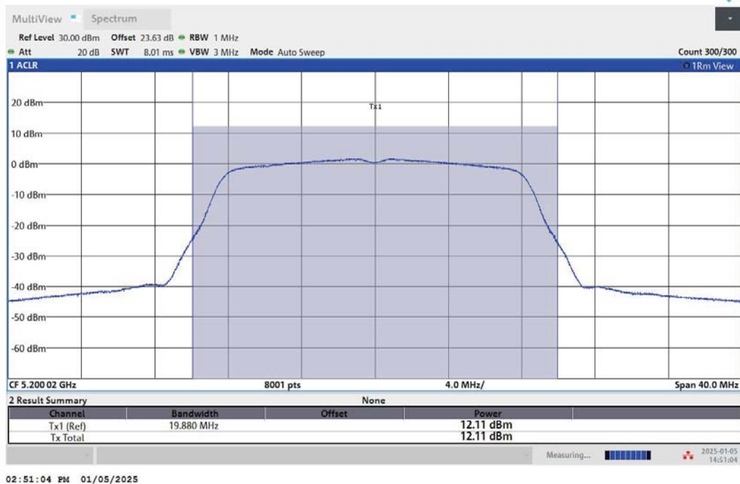
11A-Ant2-5200-PASS
