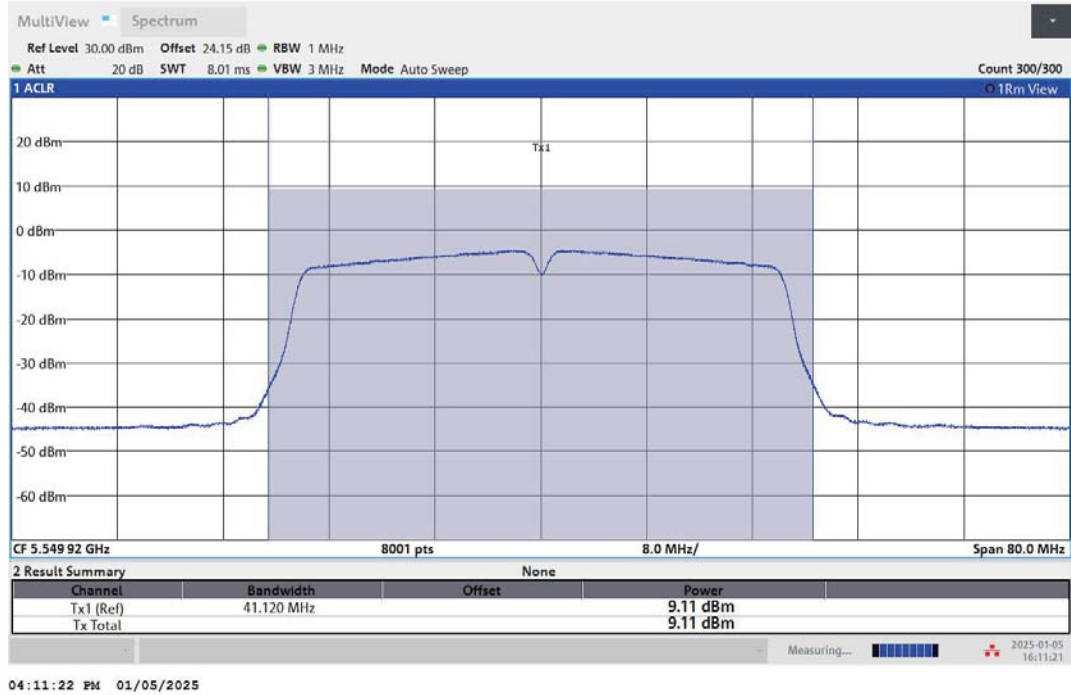
11N40MIMO-Ant1-5550-PASS
