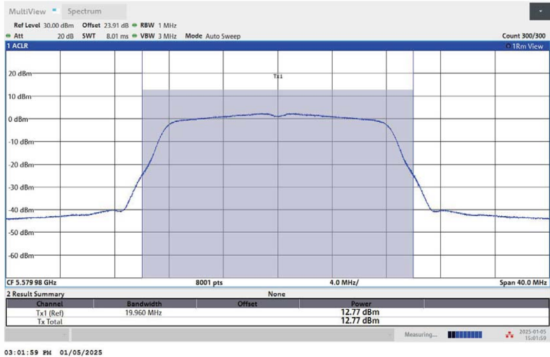
11A-Ant2-5580-PASS
