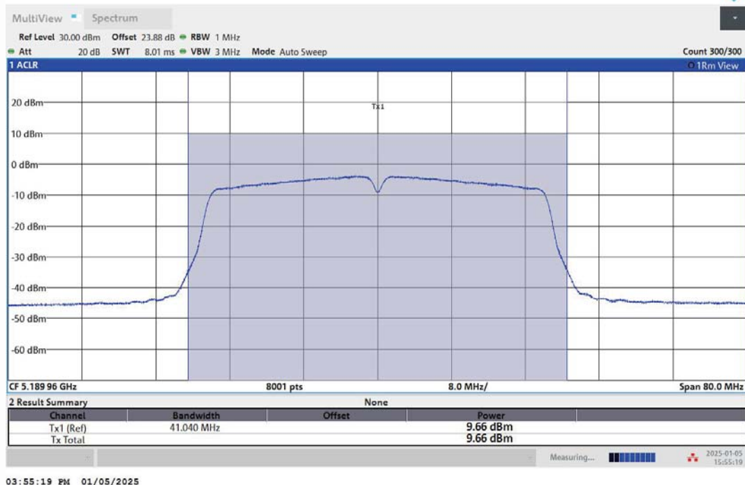
11N40MIMO-Ant1-5190-PASS
