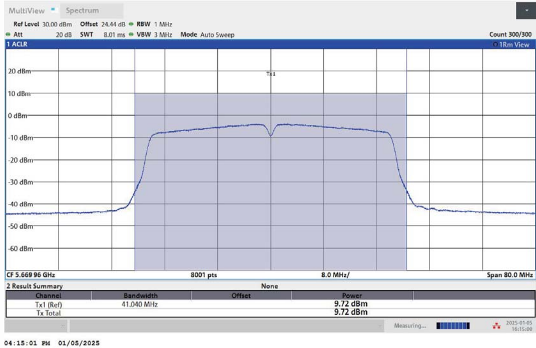
11N40MIMO-Ant1-5670-PASS
