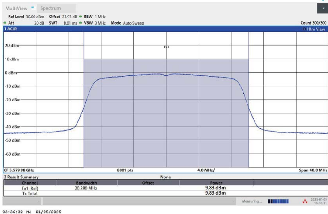
11N20MIMO-Ant2-5580-PASS
