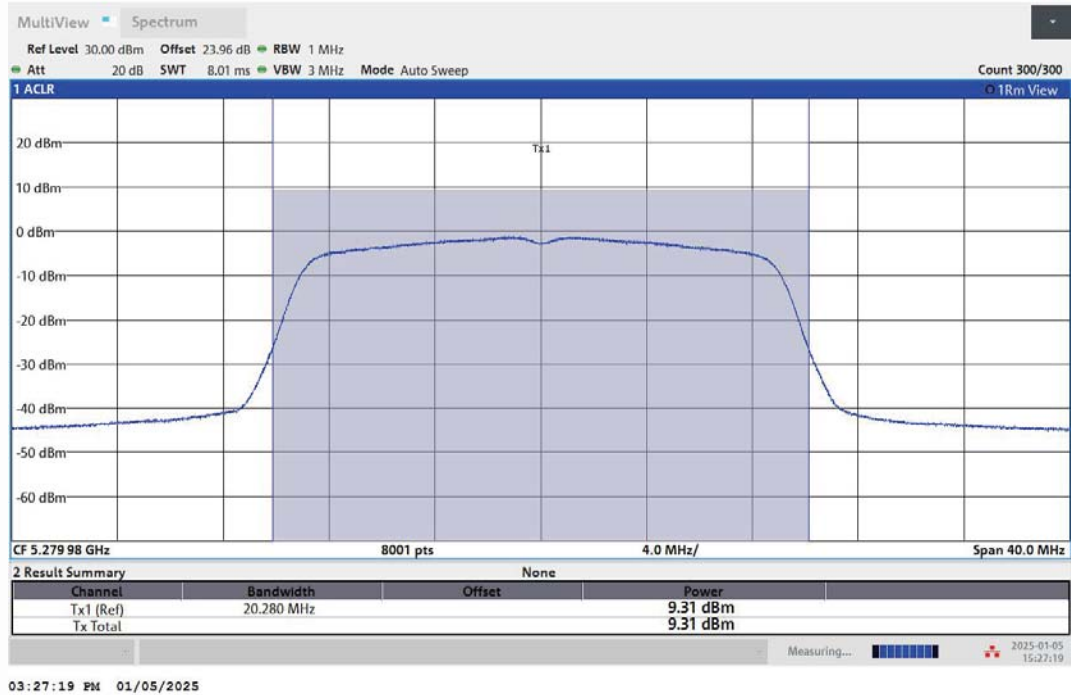
11N20MIMO-Ant2-5280-PASS
