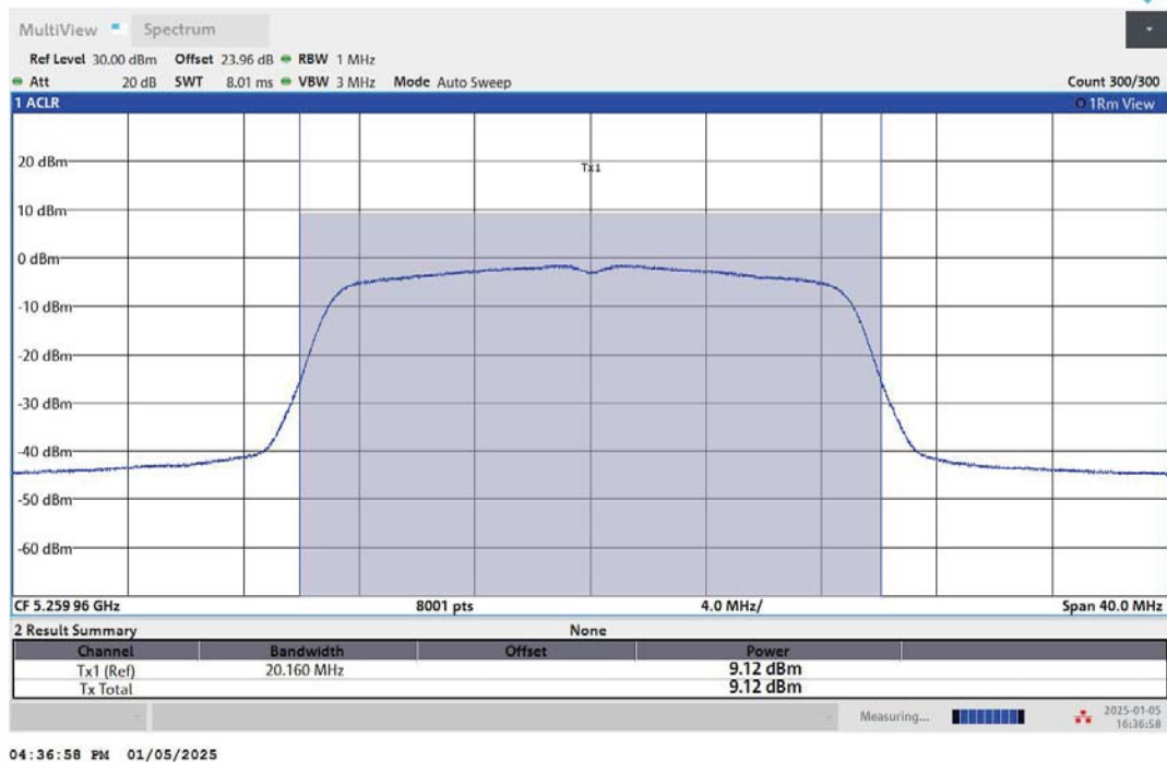
11AC20MIMO-Ant2-5260-PASS
