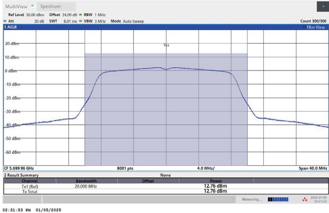
11A-Ant1-5700-PASS
