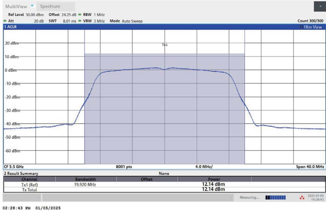
11A-Ant1-5500-PASS
