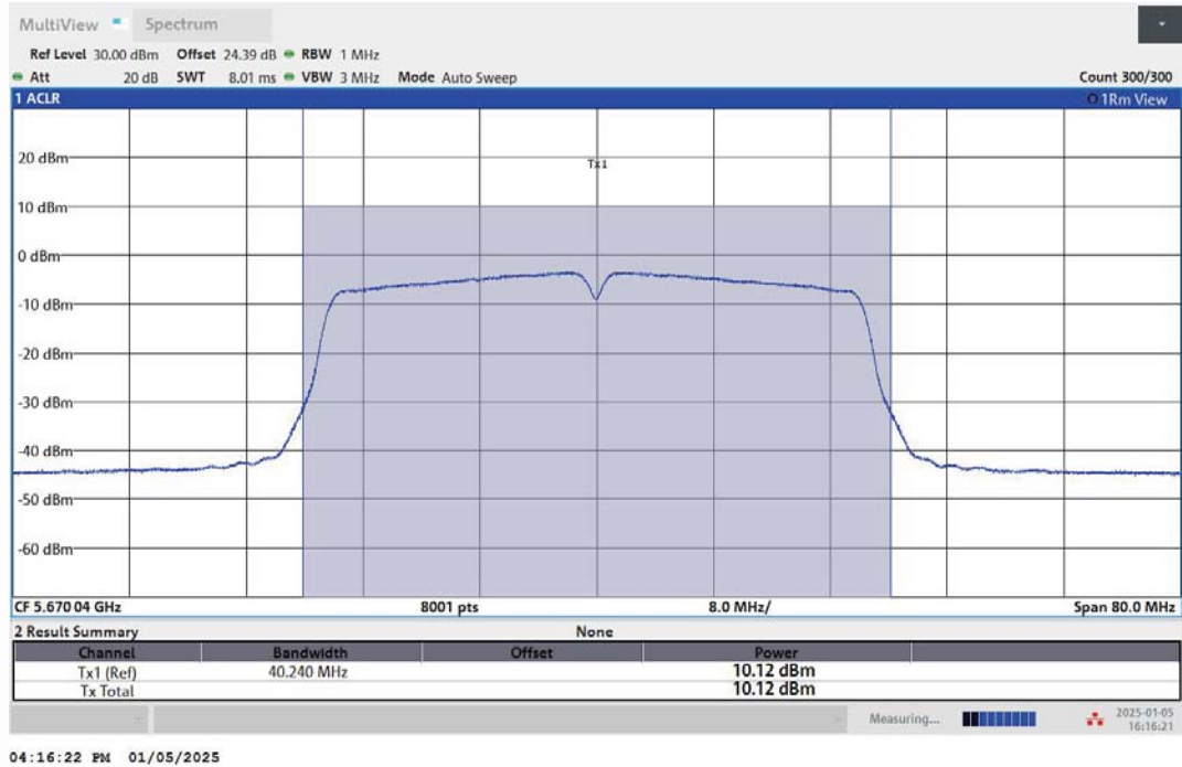
11N40MIMO-Ant2-5670-PASS
