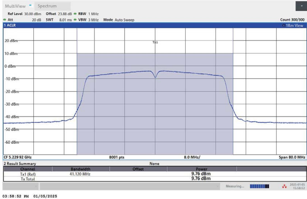
11N40MIMO-Ant1-5230-PASS
