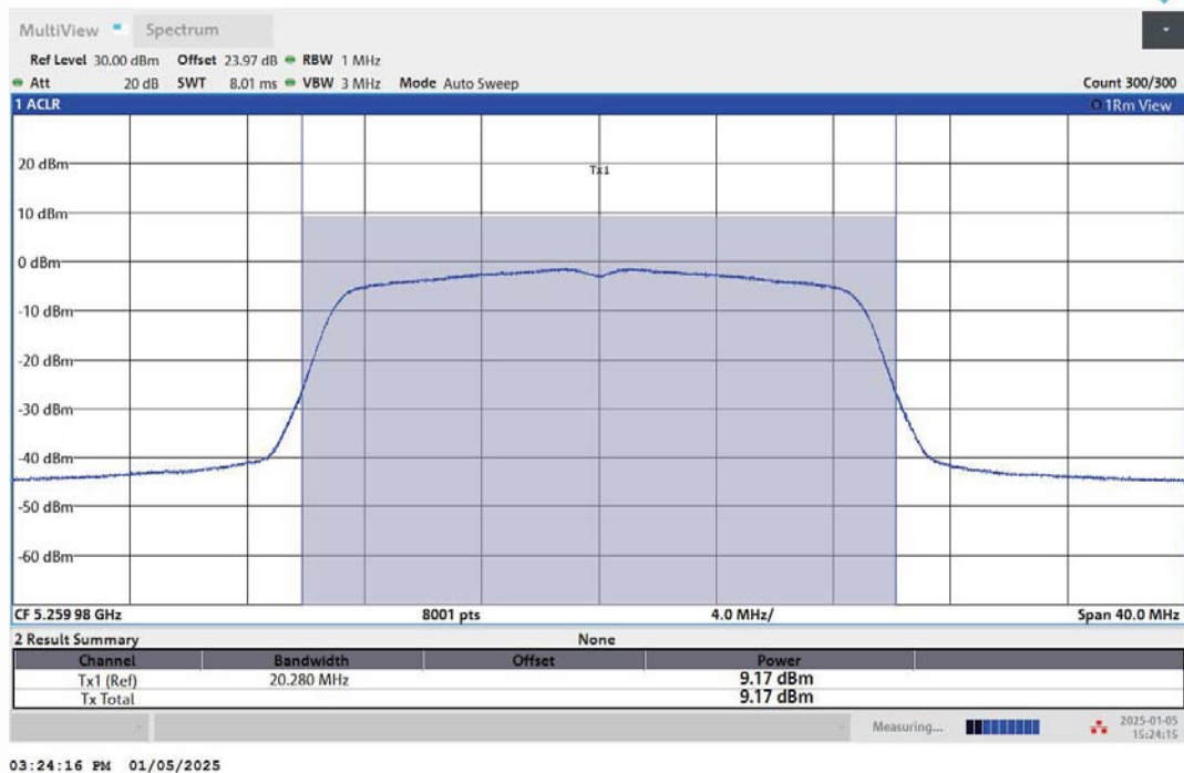
11N20MIMO-Ant2-5260-PASS
