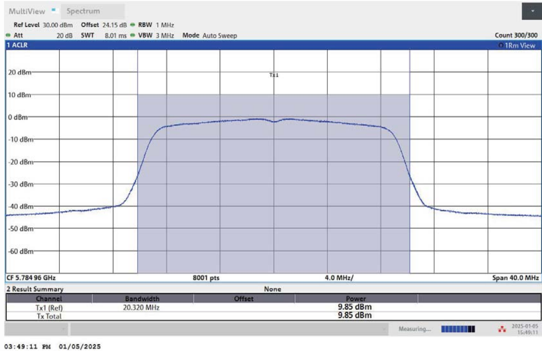
11N20MIMO-Ant2-5785-PASS
