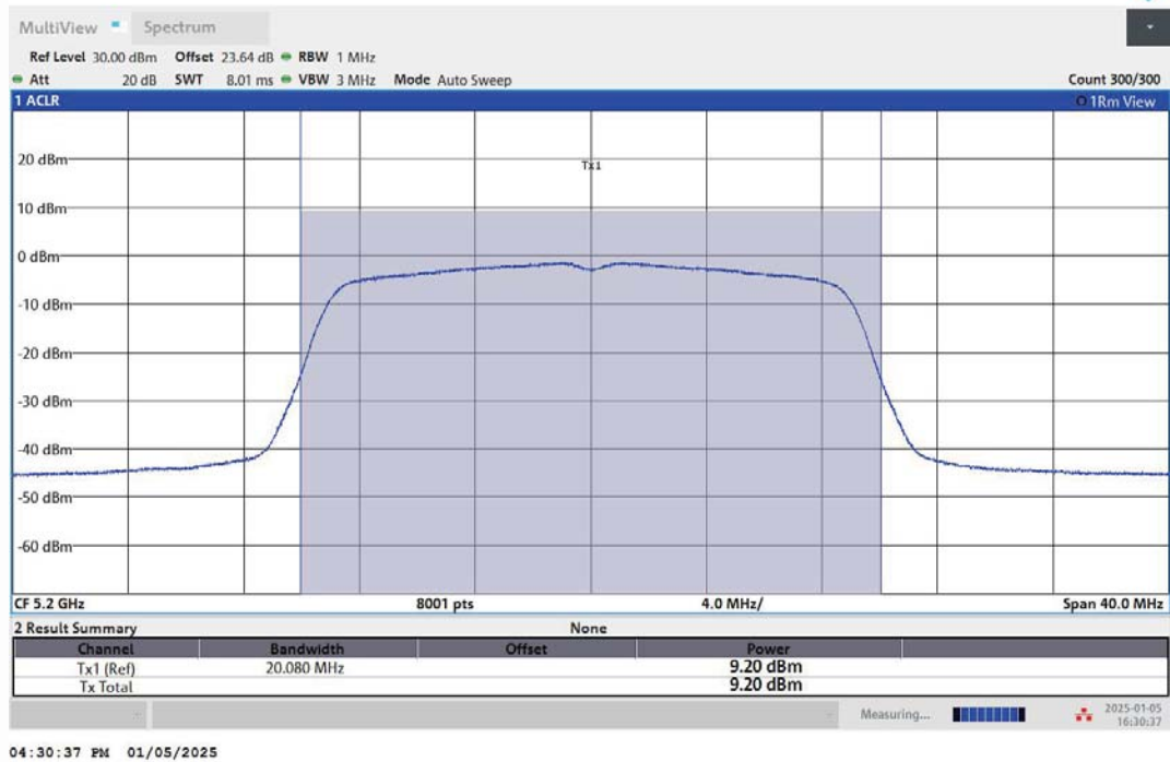
11AC20MIMO-Ant2-5200-PASS
