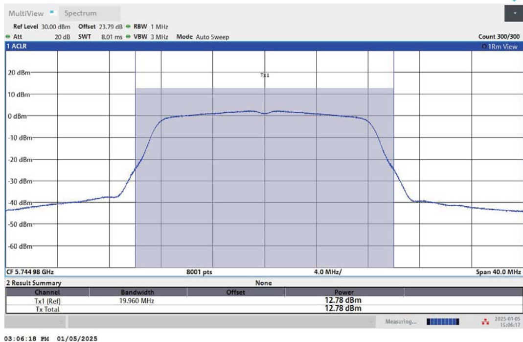
11A-Ant2-5745-PASS
