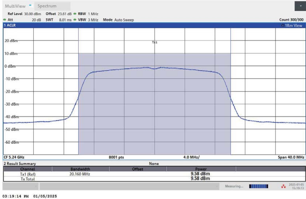
11N20MIMO-Ant1-5240-PASS
