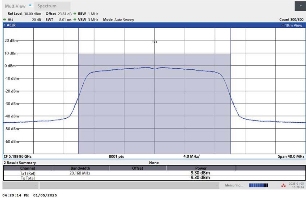
11AC20MIMO-Ant1-5200-PASS
