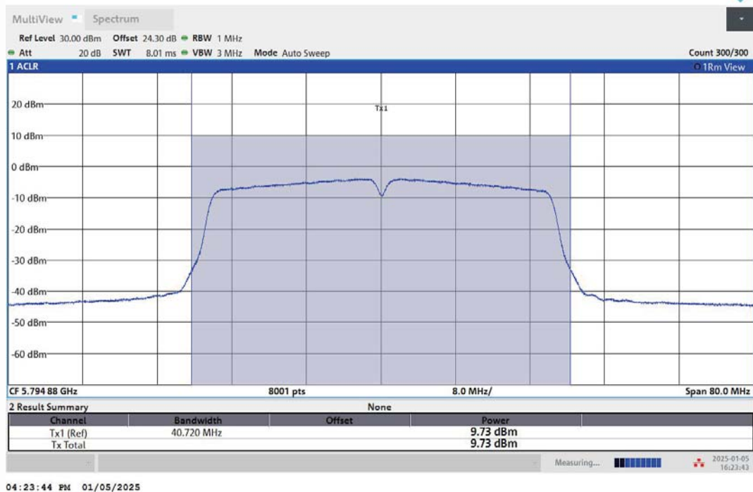
11N40MIMO-Ant2-5795-PASS
