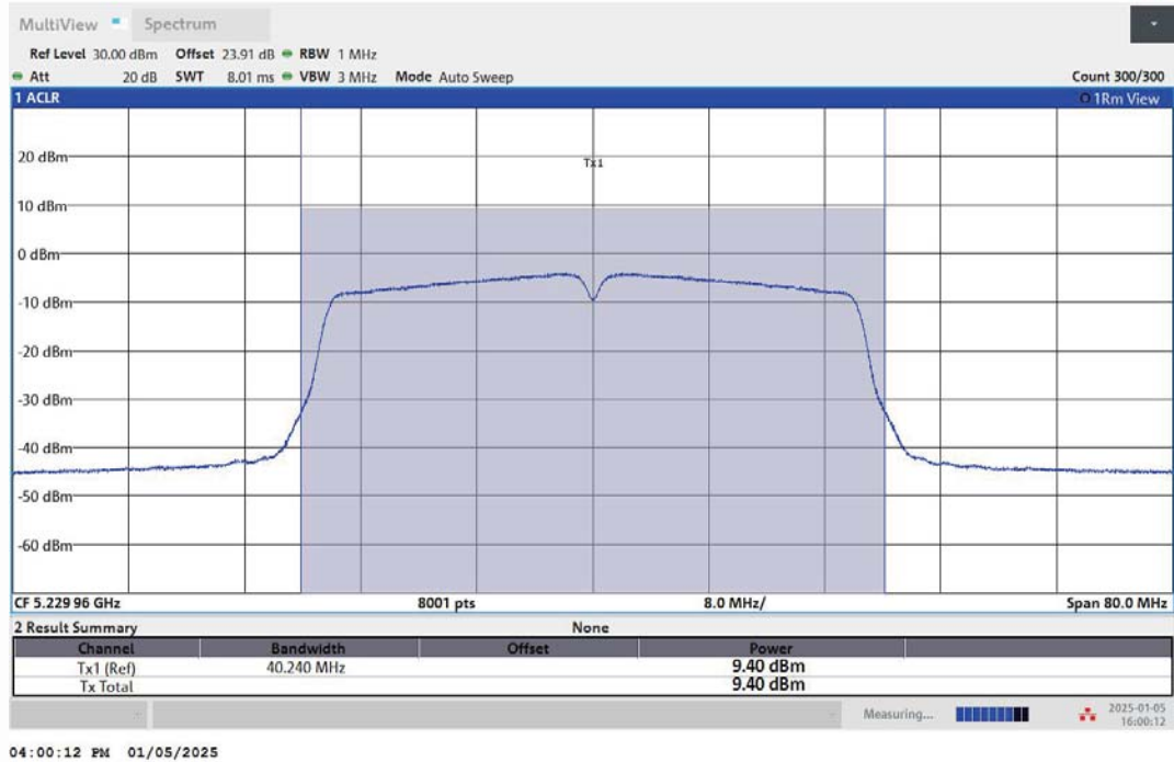
11N40MIMO-Ant2-5230-PASS
