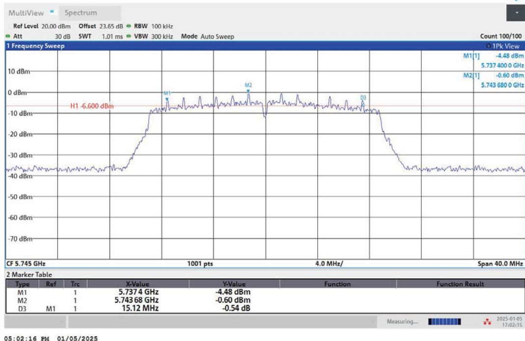
11AC20MIMO-Ant1-5745-PASS
