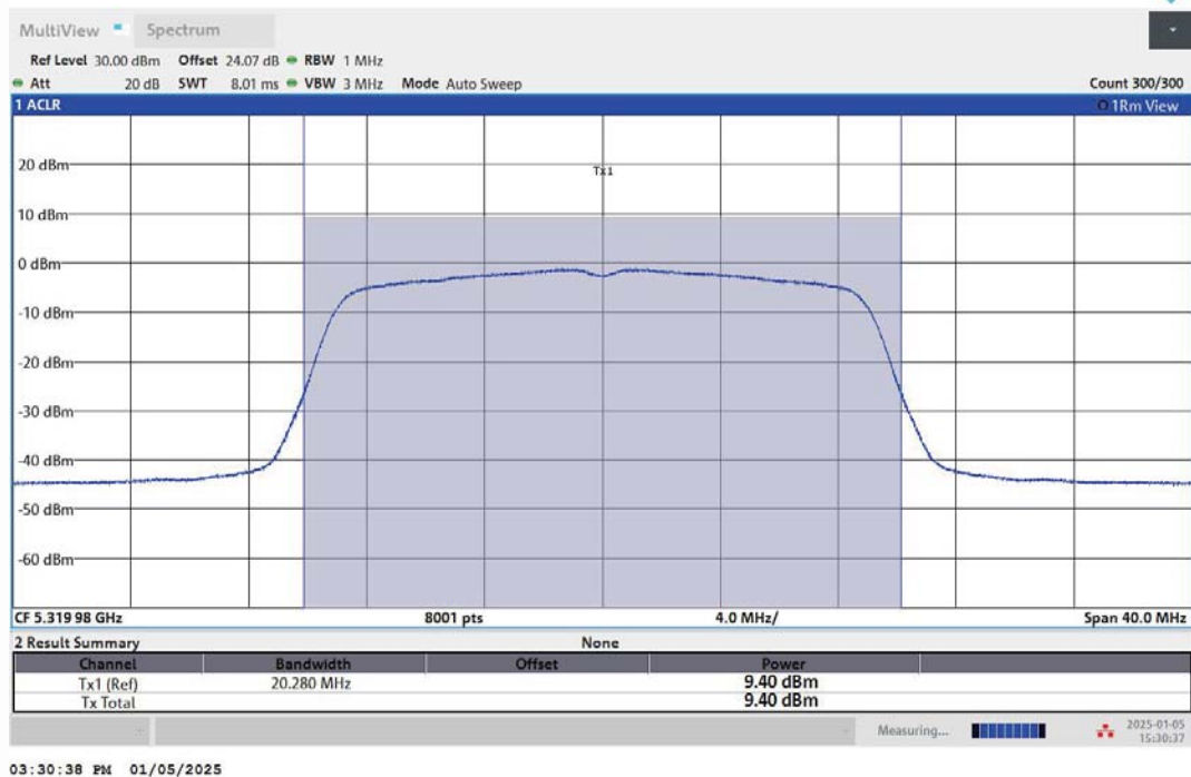
11N20MIMO-Ant2-5320-PASS
