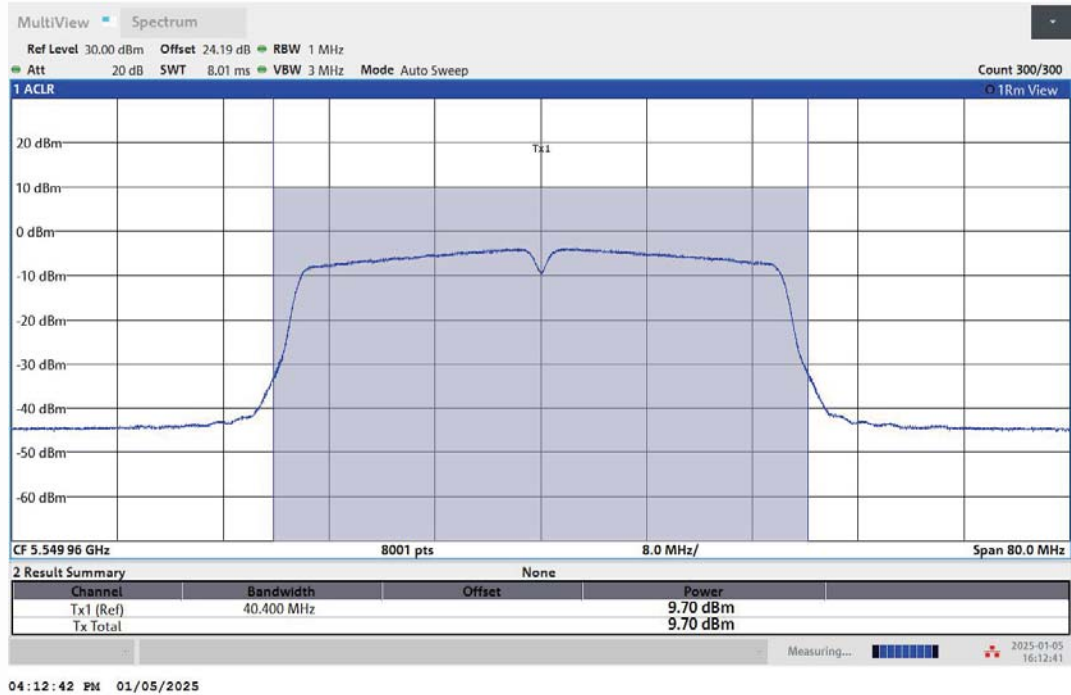
11N40MIMO-Ant2-5550-PASS
