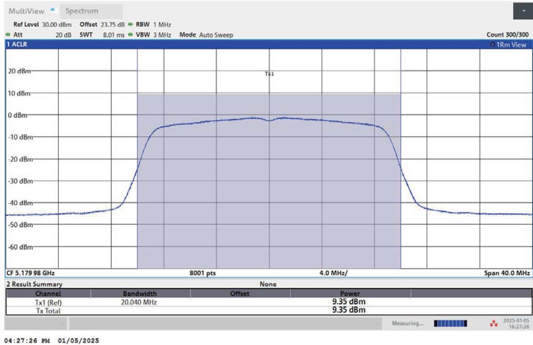
11AC20MIMO-Ant2-5180-PASS
