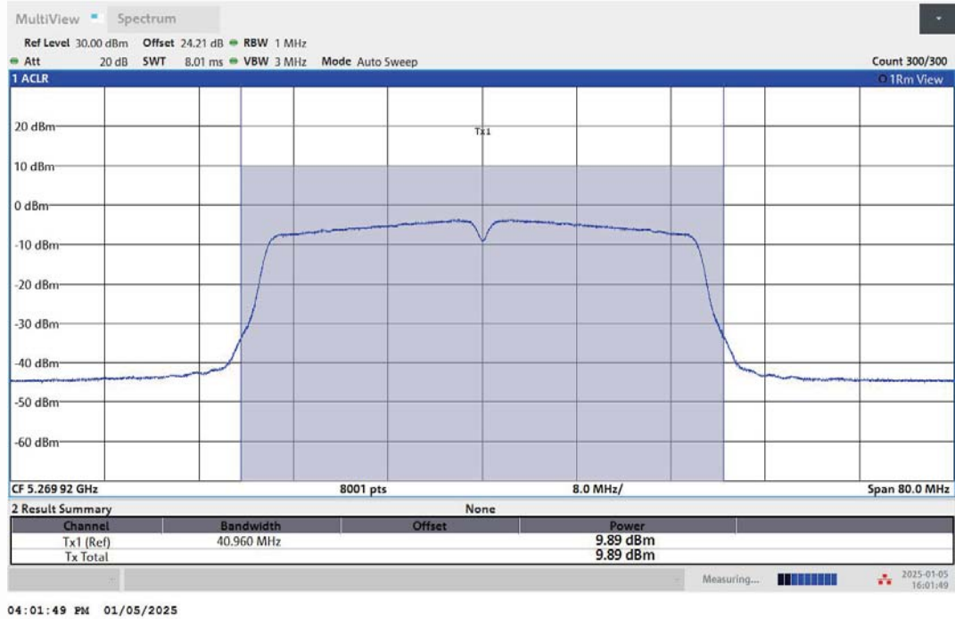
11N40MIMO-Ant1-5270-PASS
