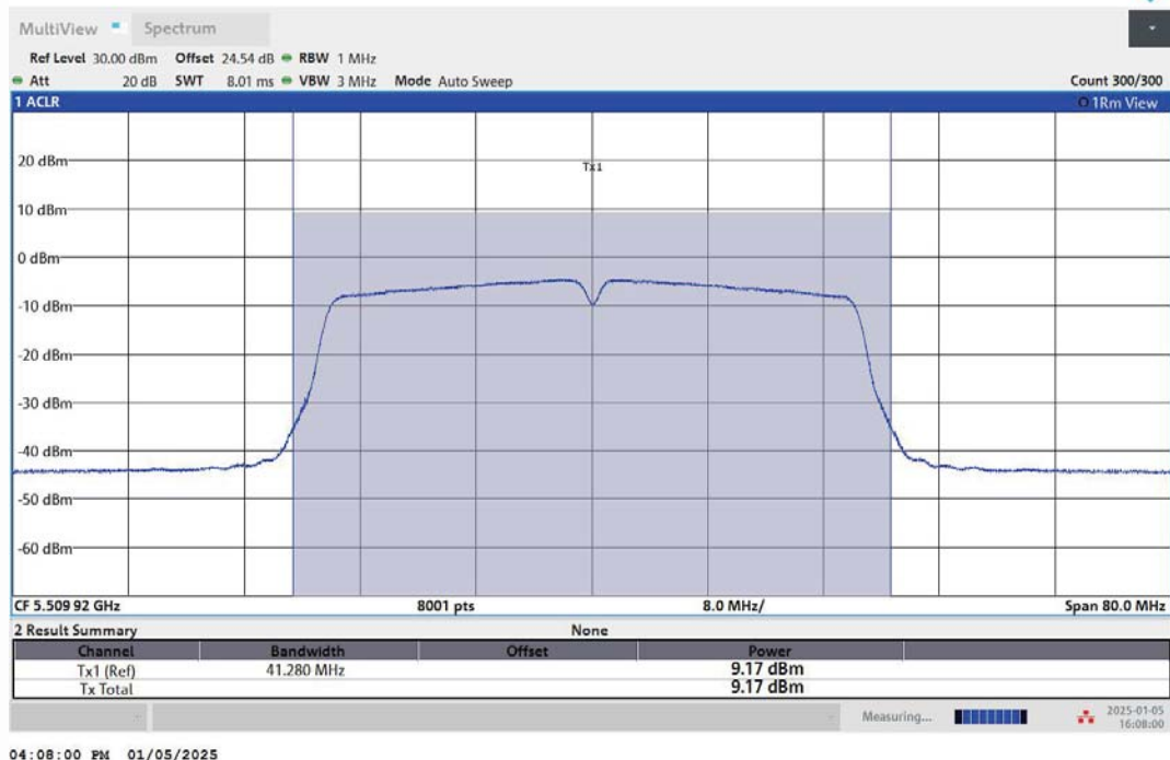
11N40MIMO-Ant1-5510-PASS
