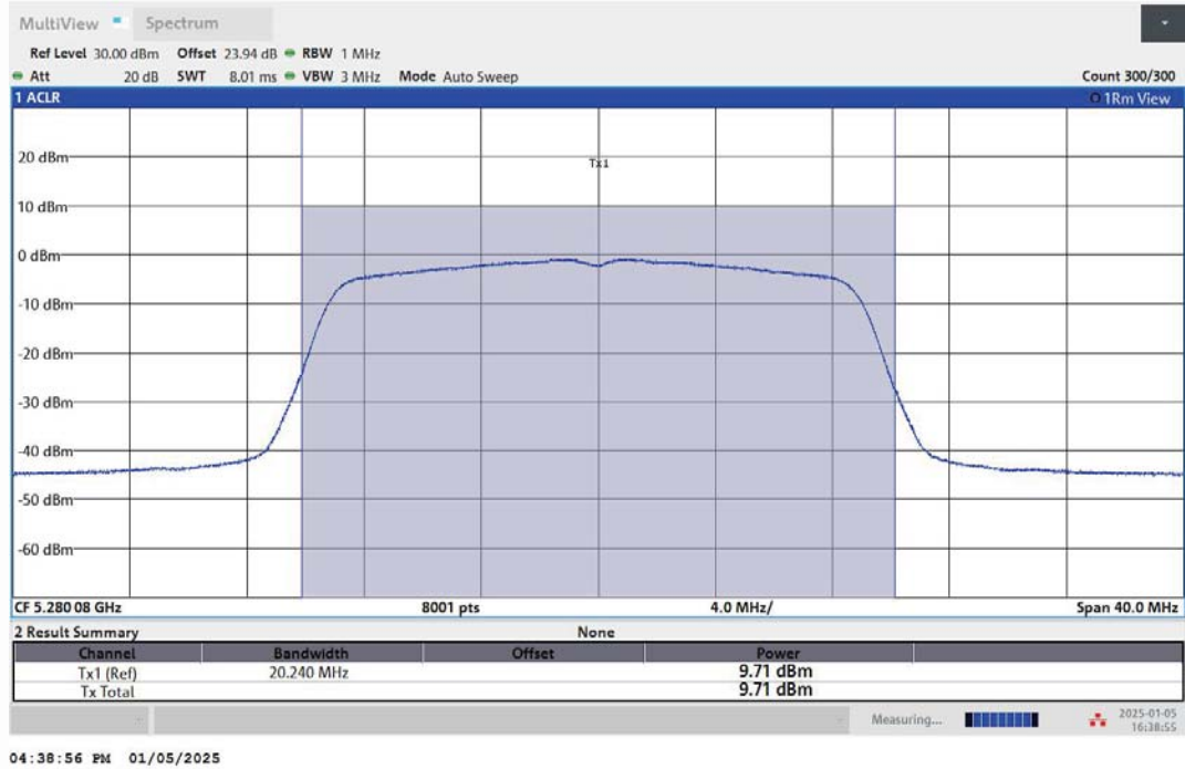
11AC20MIMO-Ant1-5280-PASS
