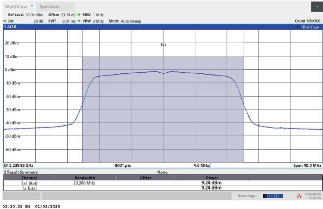
11N20MIMO-Ant2-5240-PASS
