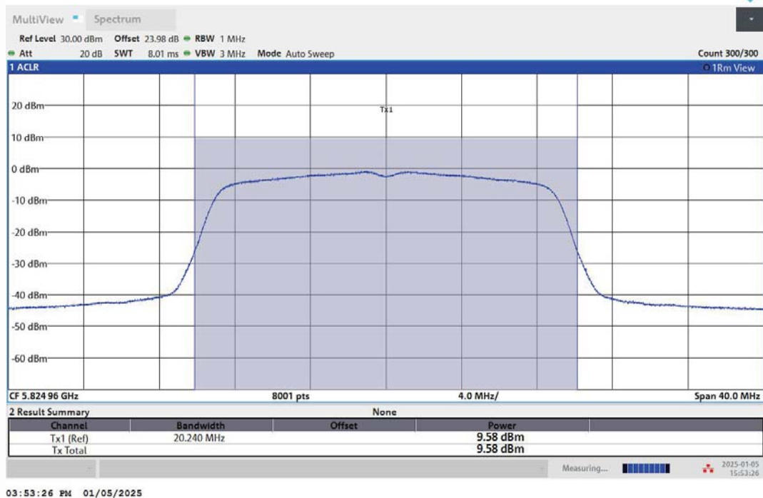
11N20MIMO-Ant2-5825-PASS
