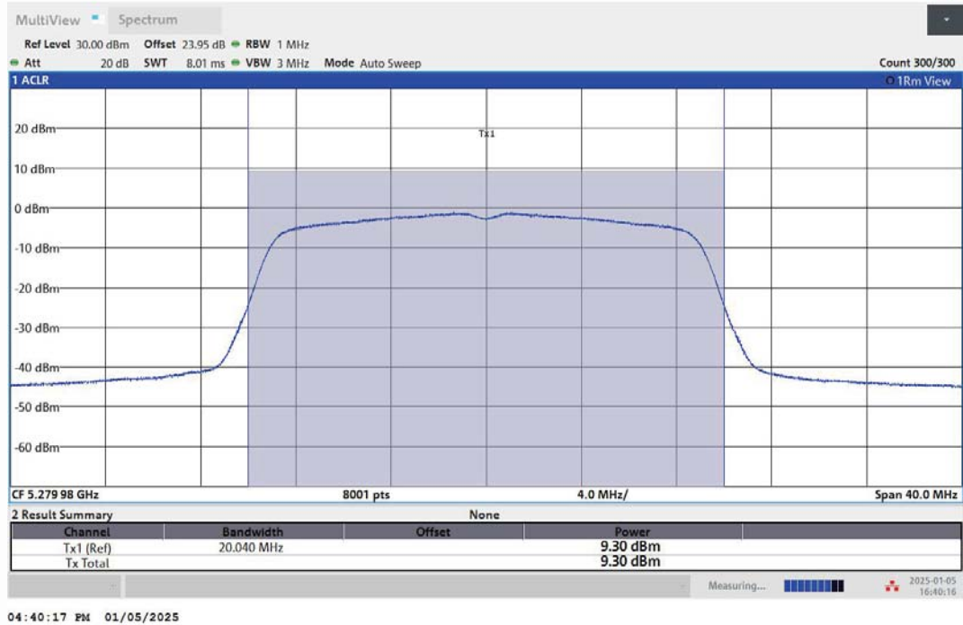
11AC20MIMO-Ant2-5280-PASS
