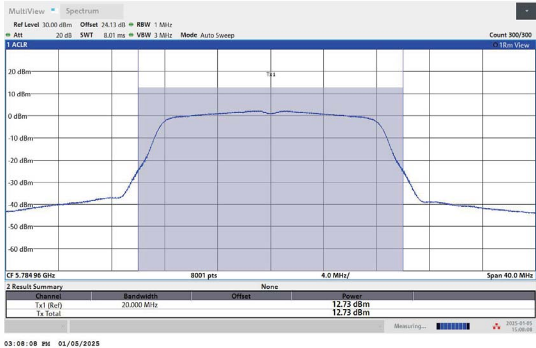
11A-Ant2-5785-PASS
