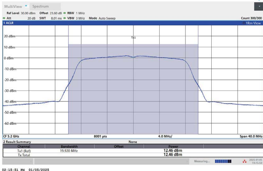
11A-Ant1-5200-PASS
