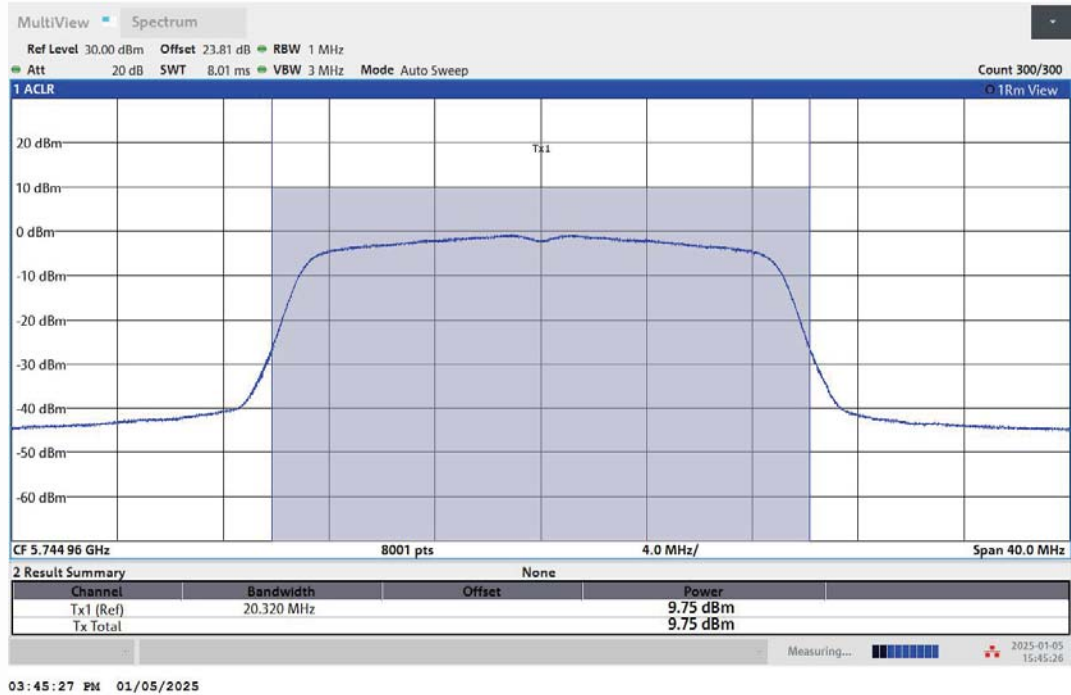
11N20MIMO-Ant2-5745-PASS
