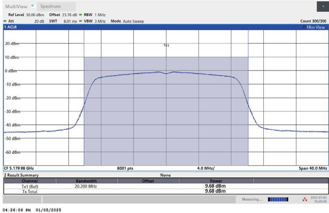
11AC20MIMO-Ant1-5180-PASS
