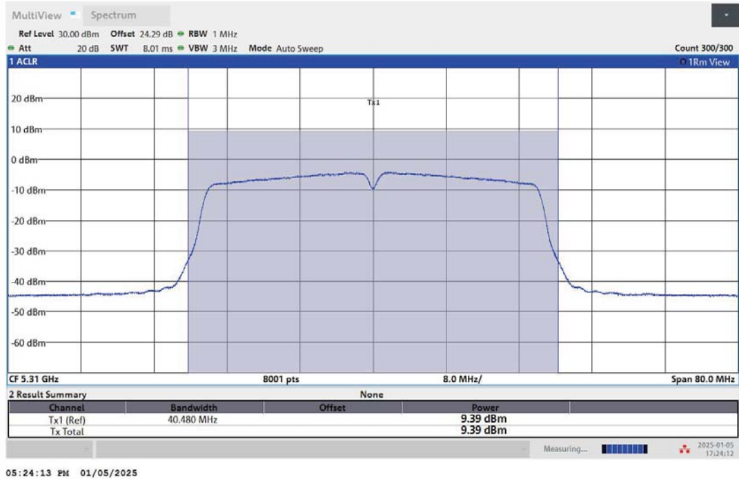
11AC40MIMO-Ant2-5310-PASS
