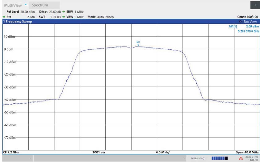
11A-Ant1-5200-PASS
