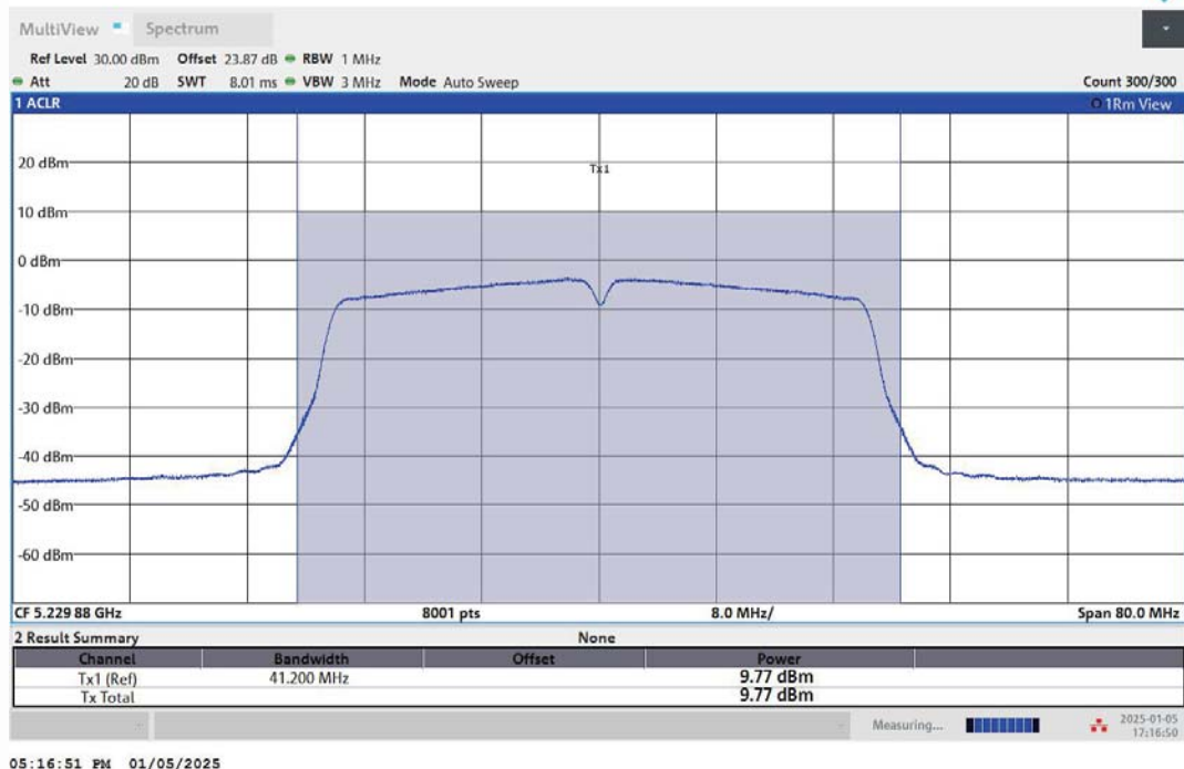
11AC40MIMO-Ant1-5230-PASS
