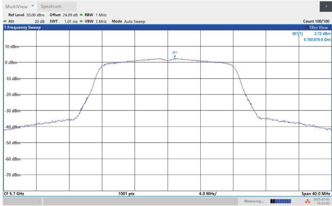
11A-Ant1-5700-PASS
