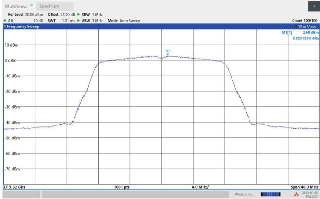
11A-Ant1-5320-PASS
