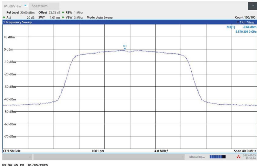
11N20MIMO-Ant2-5580-PASS
