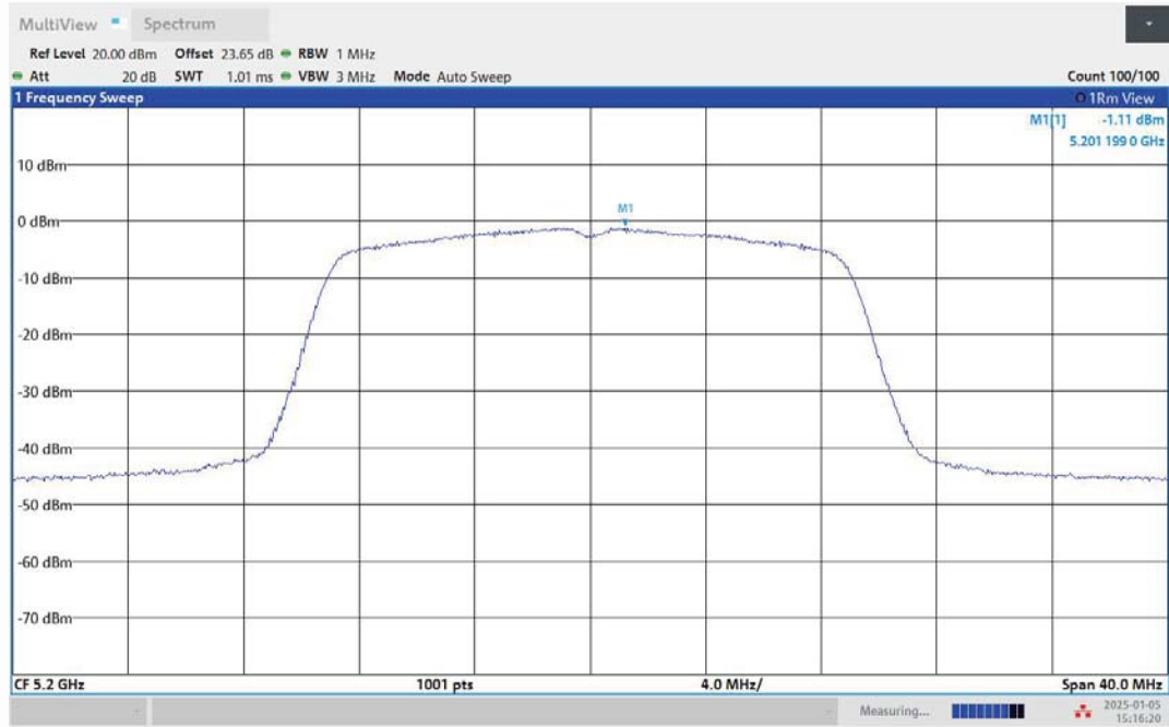
11N20MIMO-Ant2-5200-PASS
