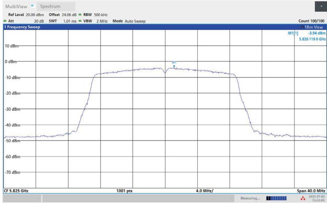
11N20MIMO-Ant1-5825-PASS
