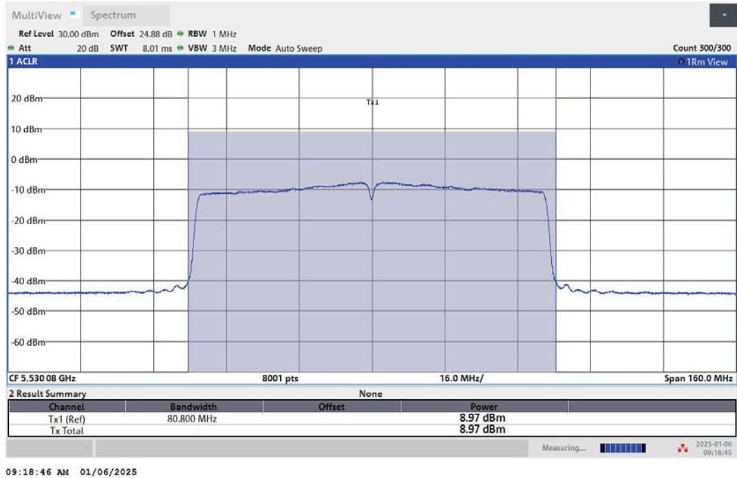
11AC80MIMO-Ant2-5530-PASS
