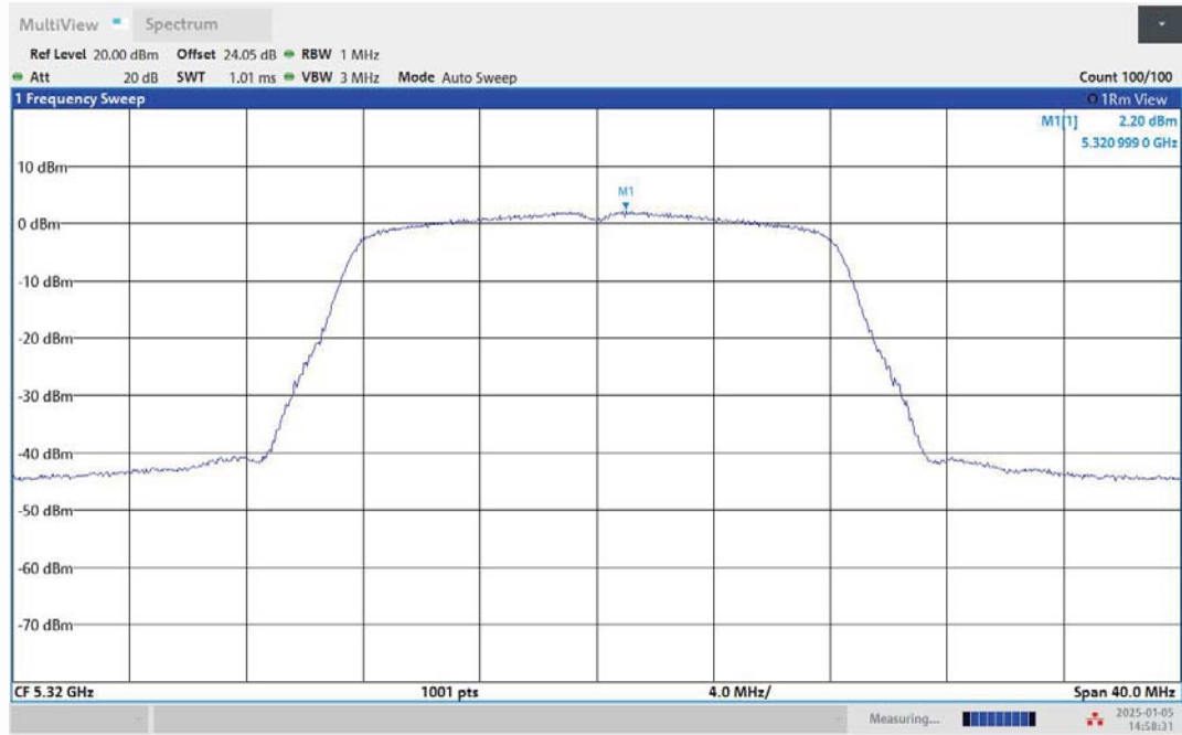
11A-Ant2-5320-PASS
