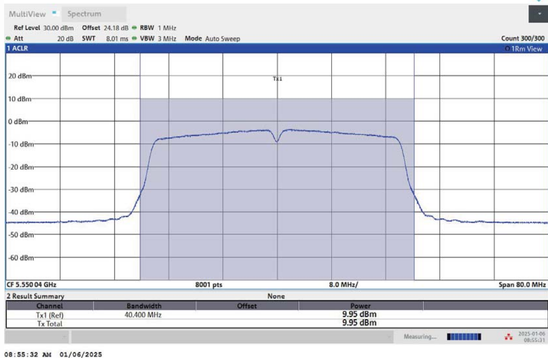
11AC40MIMO-Ant2-5550-PASS
