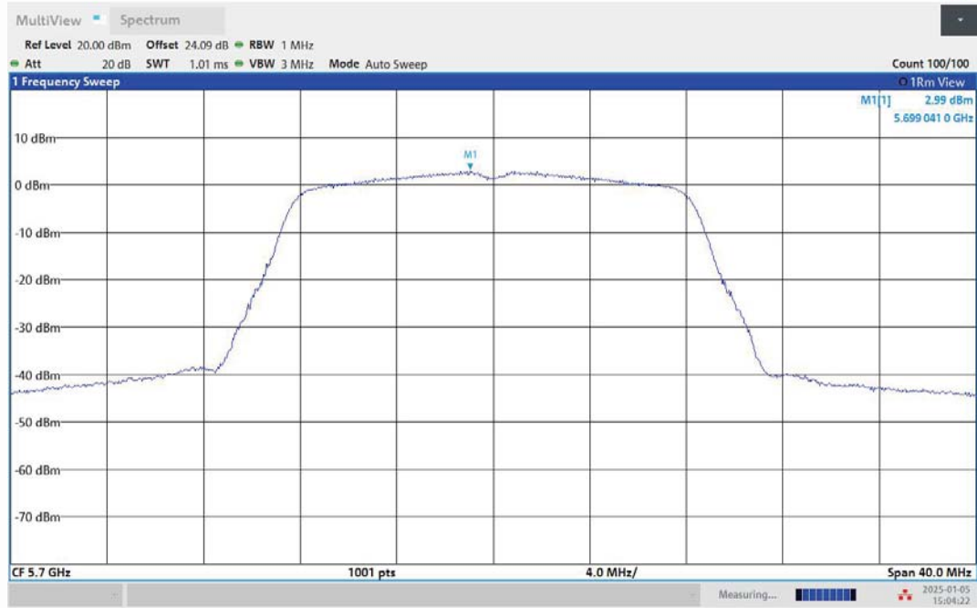
11A-Ant2-5700-PASS
