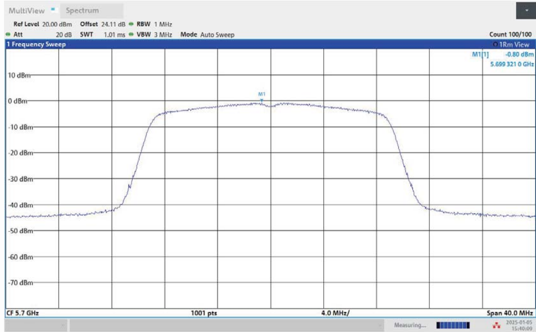
11N20MIMO-Ant1-5700-PASS
