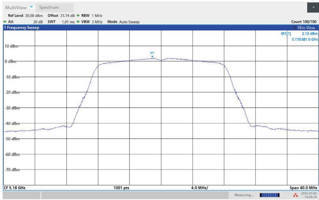
11A-Ant2-5180-PASS
