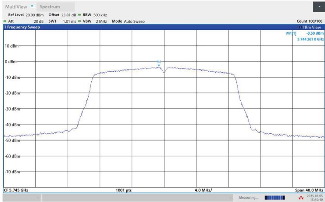
11N20MIMO-Ant2-5745-PASS
