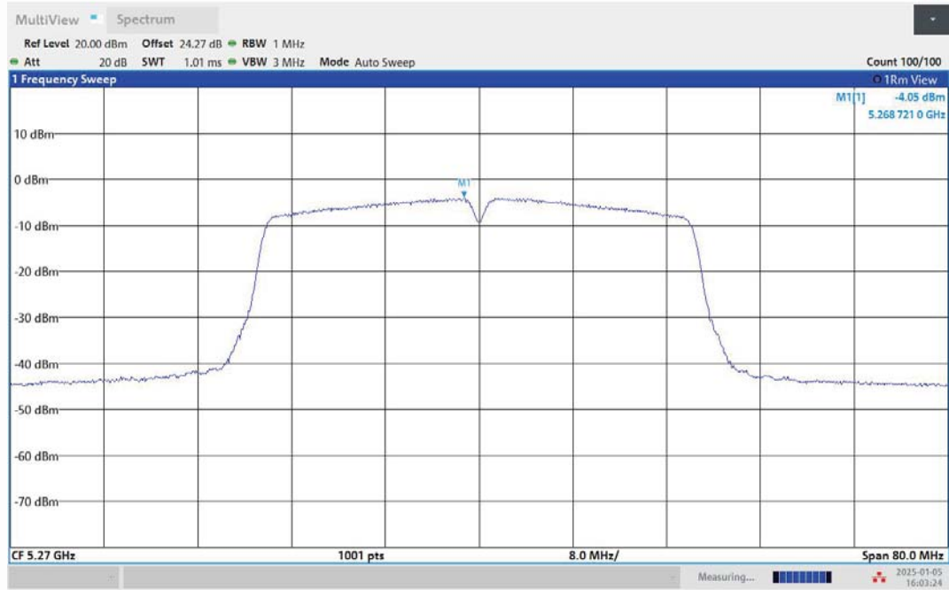
11N40MIMO-Ant2-5270-PASS
