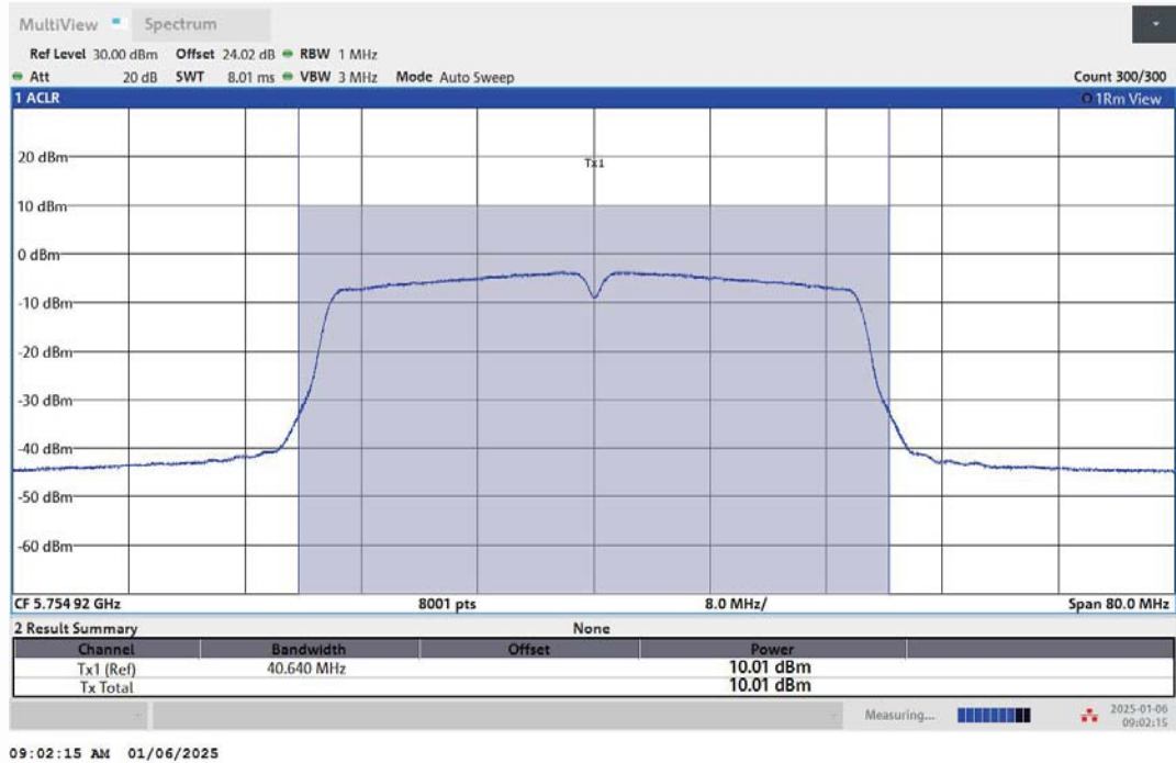
11AC40MIMO-Ant2-5755-PASS
