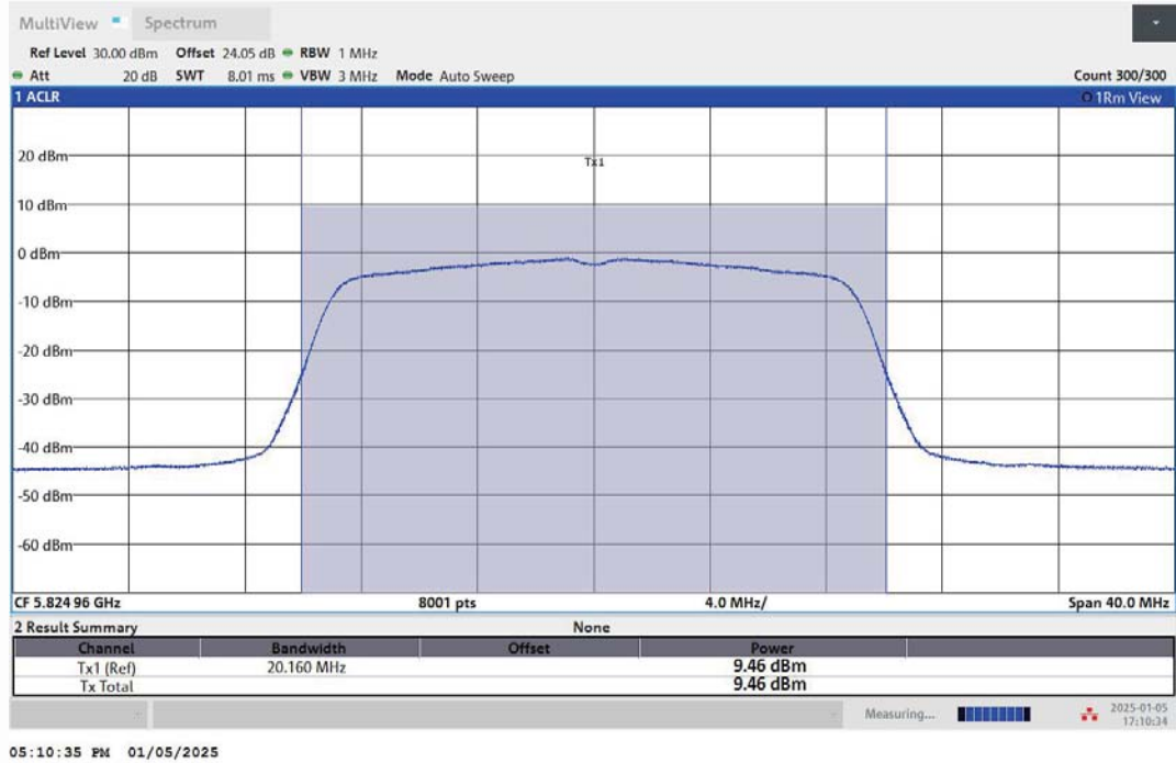
11AC20MIMO-Ant1-5825-PASS
