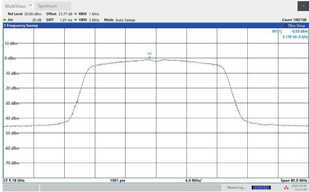
11N20MIMO-Ant1-5180-PASS
