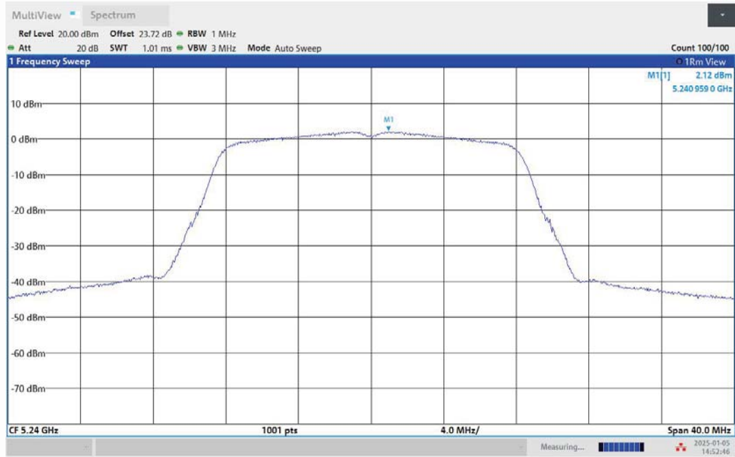
11A-Ant2-5240-PASS
