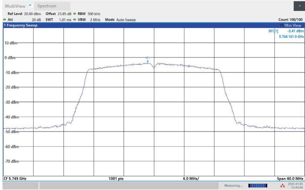
11N20MIMO-Ant1-5745-PASS
