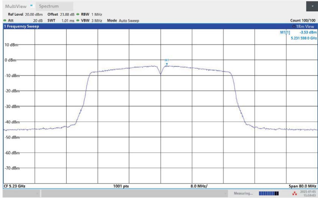
11N40MIMO-Ant1-5230-PASS
