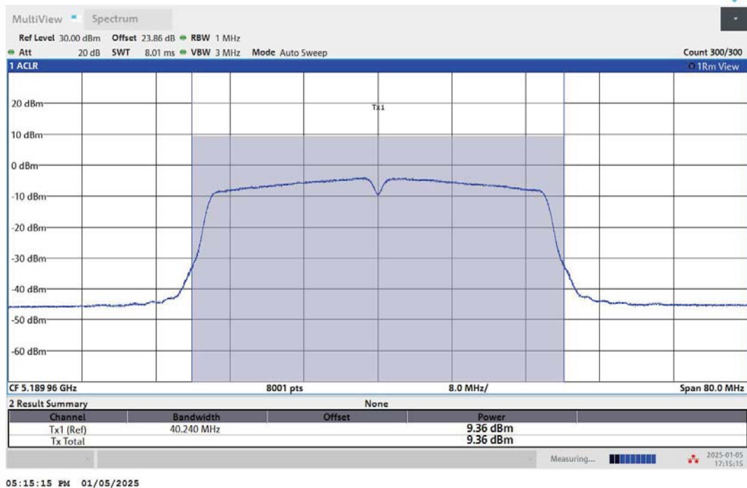
11AC40MIMO-Ant2-5190-PASS
