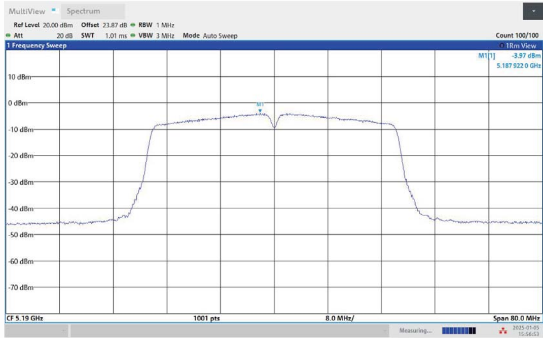
11N40MIMO-Ant2-5190-PASS
