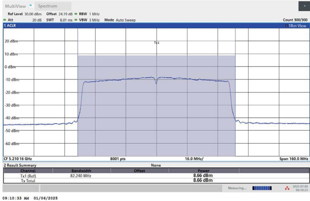
11AC80MIMO-Ant1-5210-PASS
