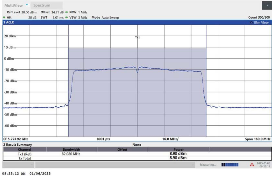
11AC80MIMO-Ant1-5775-PASS
