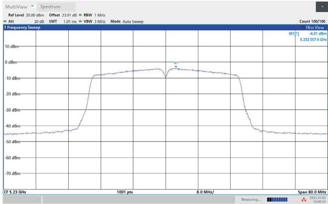
11N40MIMO-Ant2-5230-PASS
