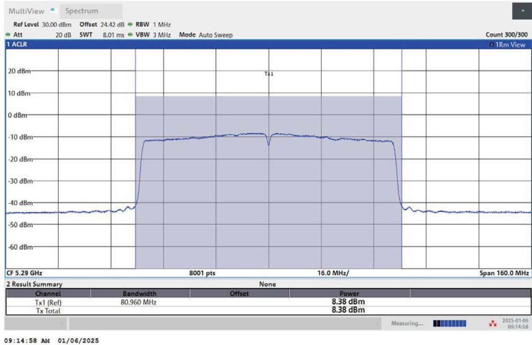
11AC80MIMO-Ant2-5290-PASS
