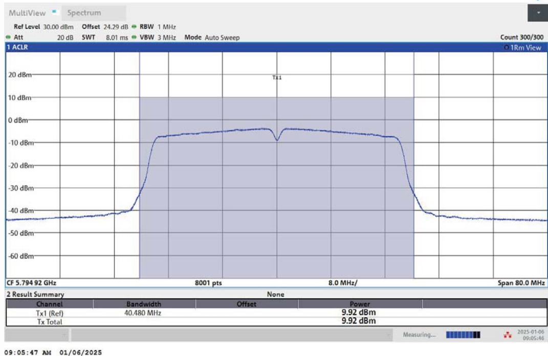
11AC40MIMO-Ant2-5795-PASS
