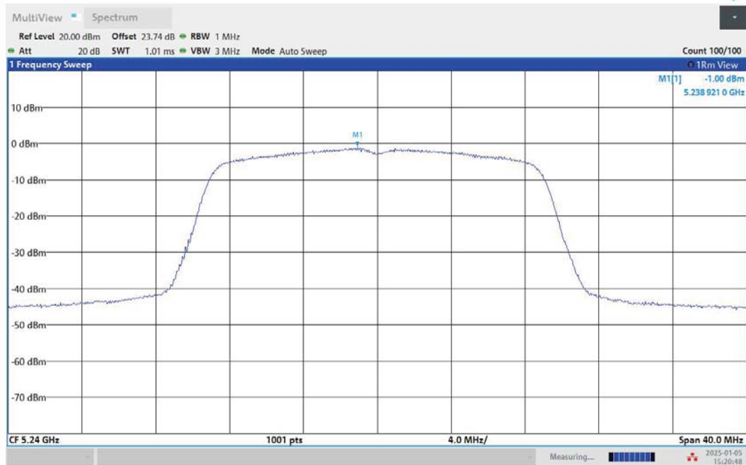
11N20MIMO-Ant2-5240-PASS
