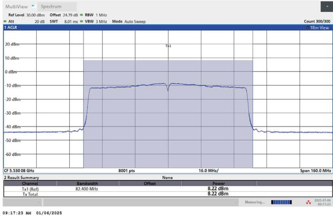
11AC80MIMO-Ant1-5530-PASS
