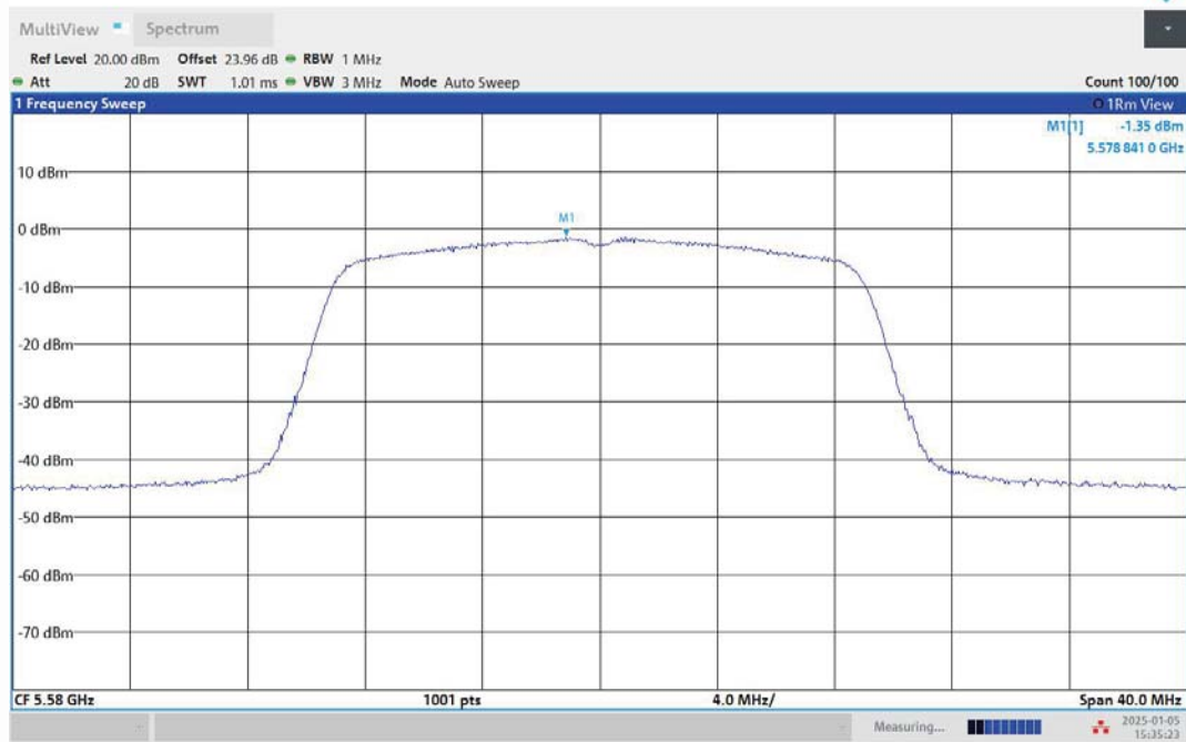
11N20MIMO-Ant1-5580-PASS
