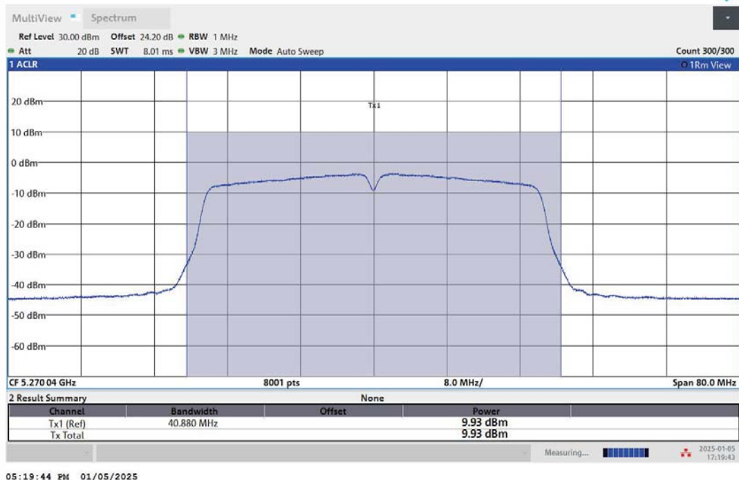
11AC40MIMO-Ant1-5270-PASS
