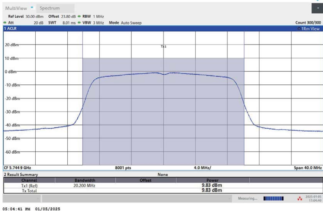
11AC20MIMO-Ant2-5745-PASS
