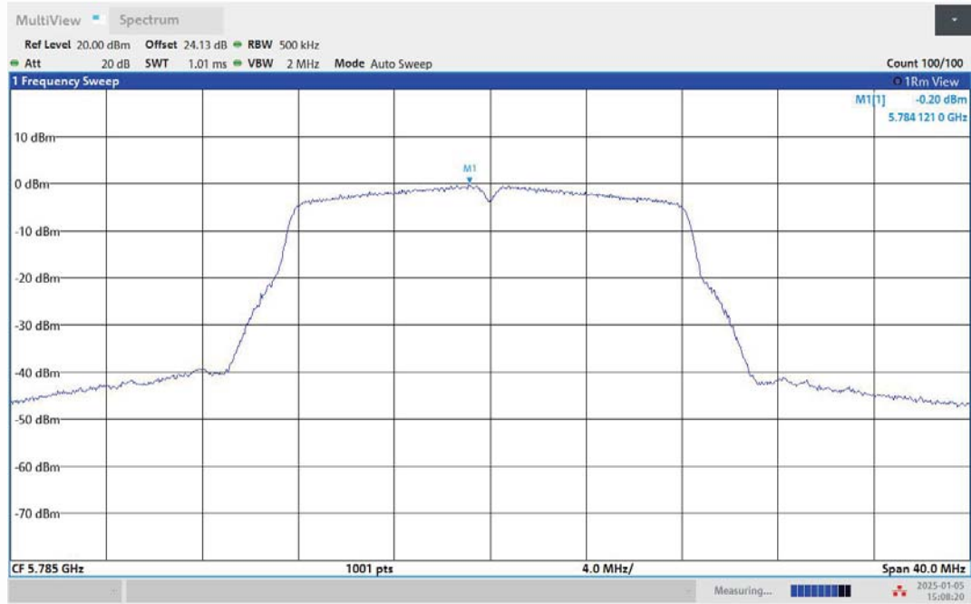
11A-Ant2-5785-PASS
