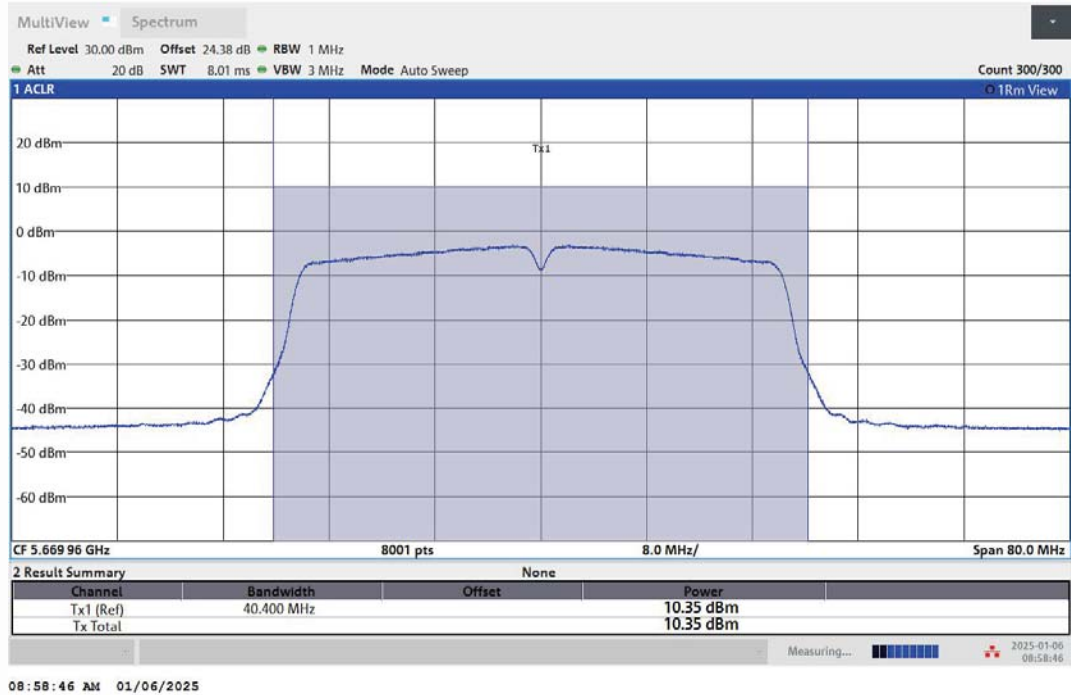
11AC40MIMO-Ant2-5670-PASS
