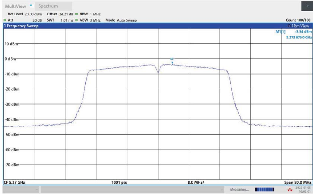
11N40MIMO-Ant1-5270-PASS
