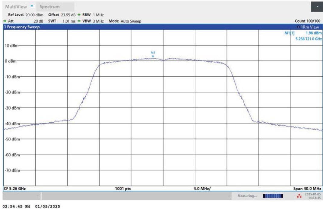
11A-Ant2-5260-PASS
