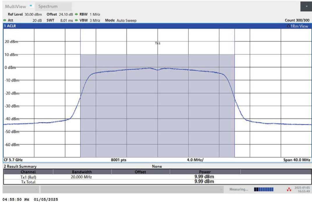
11AC20MIMO-Ant2-5700-PASS
