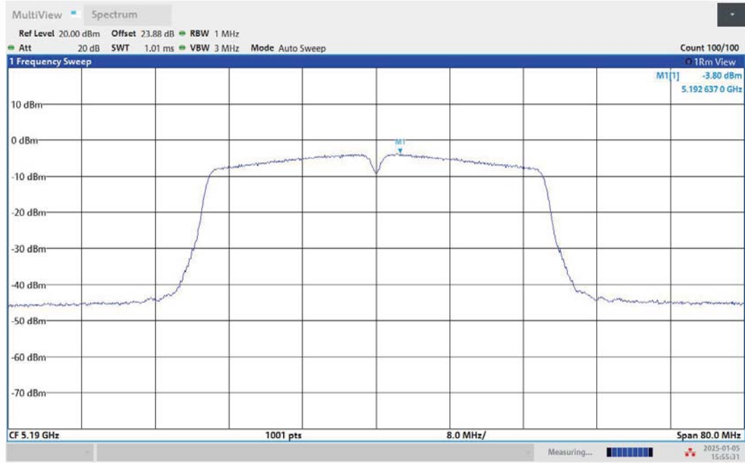
11N40MIMO-Ant1-5190-PASS
