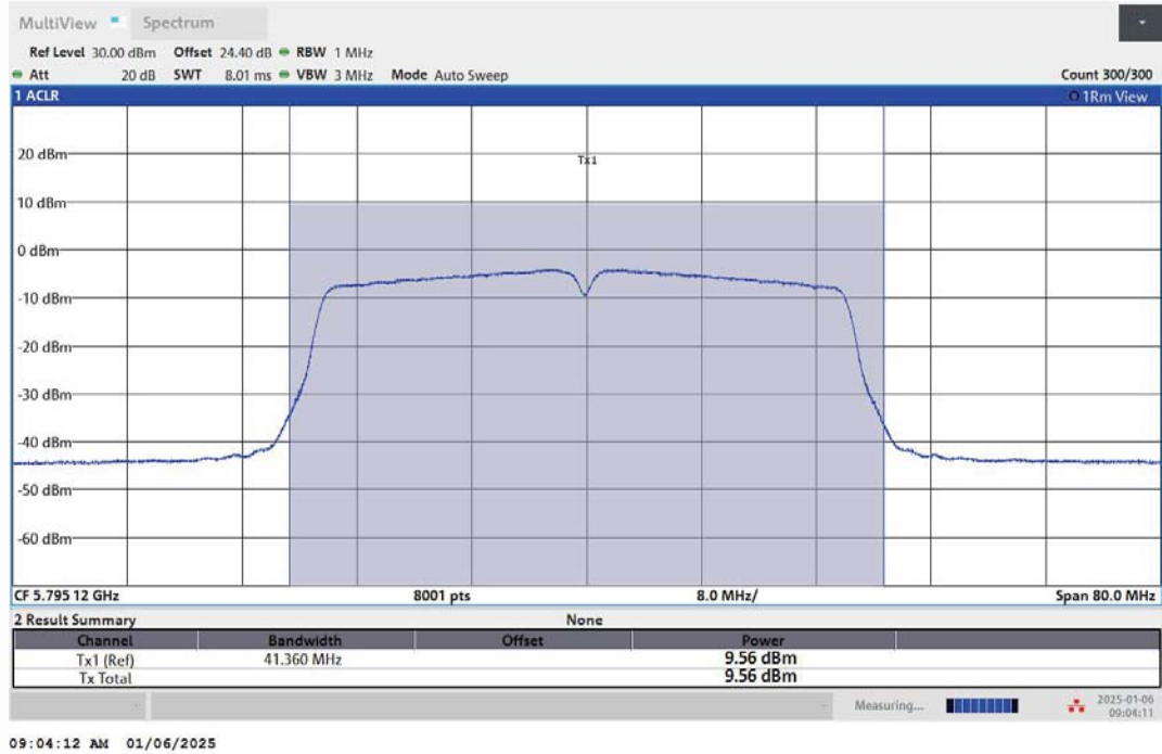
11AC40MIMO-Ant1-5795-PASS
