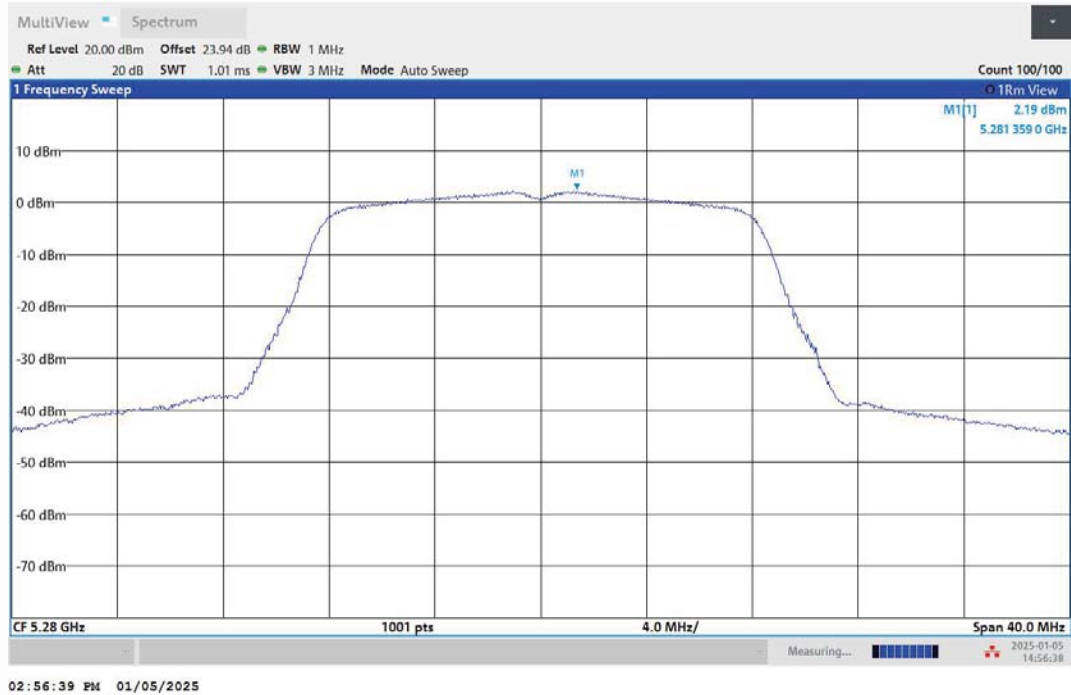
11A-Ant2-5280-PASS
