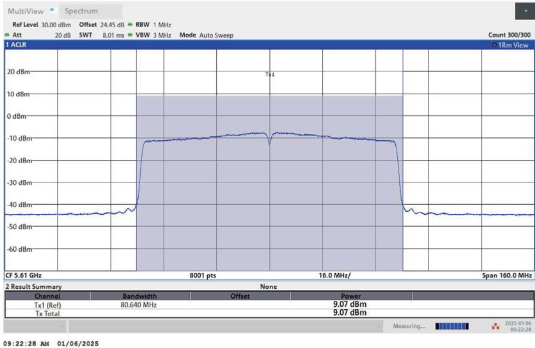
11AC80MIMO-Ant2-5610-PASS
