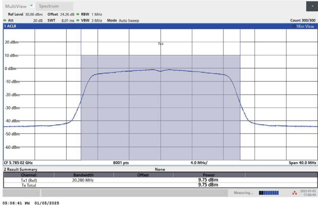
11AC20MIMO-Ant1-5785-PASS
