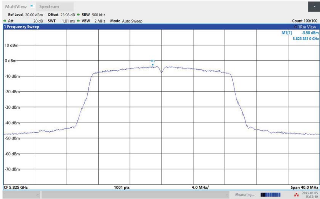
11N20MIMO-Ant2-5825-PASS
