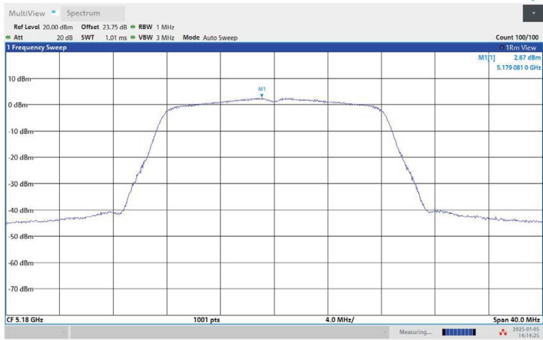
11A-Ant1-5180-PASS
