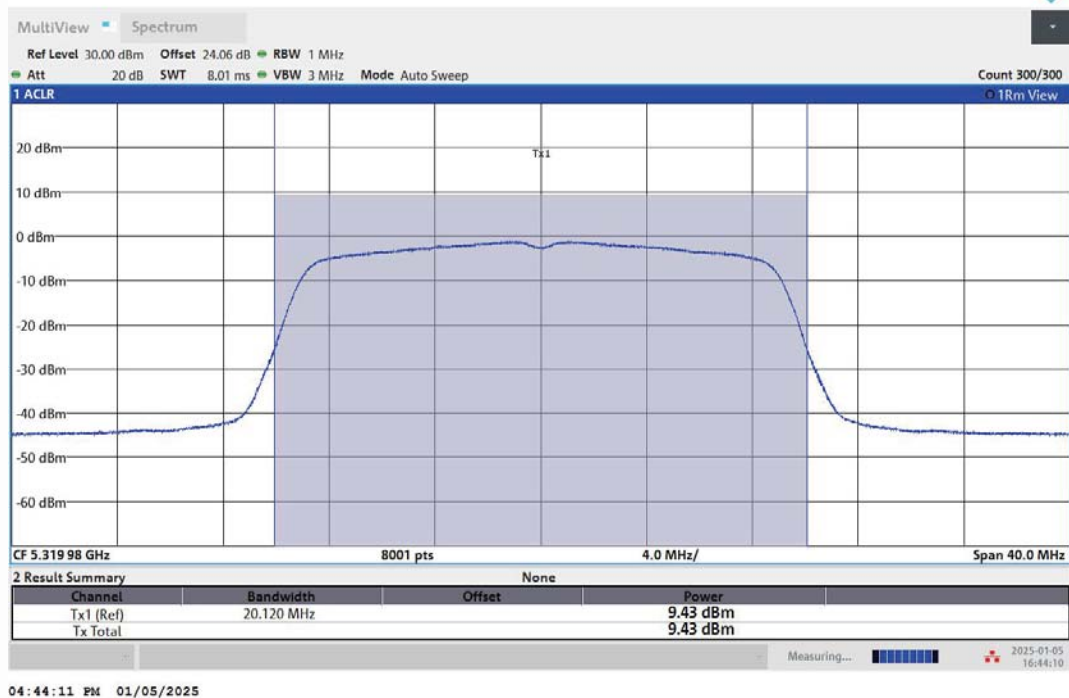
11AC20MIMO-Ant2-5320-PASS
