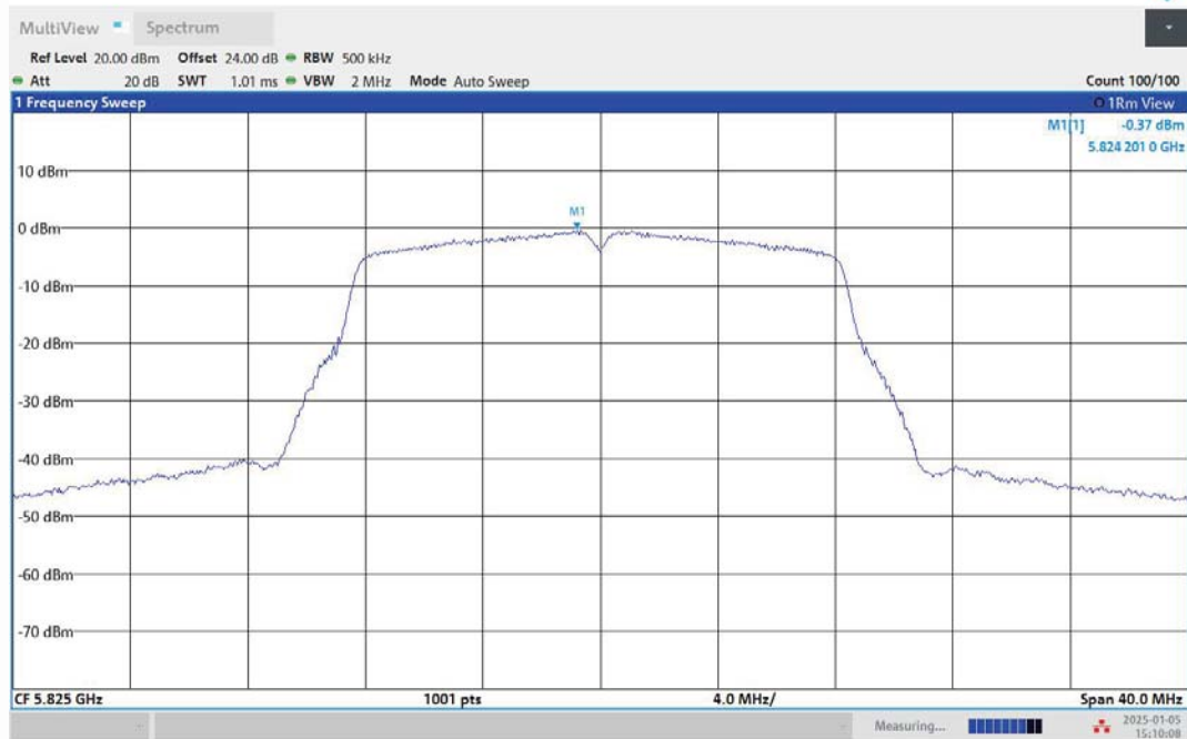
11A-Ant2-5825-PASS
