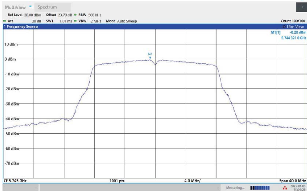
11A-Ant2-5745-PASS
