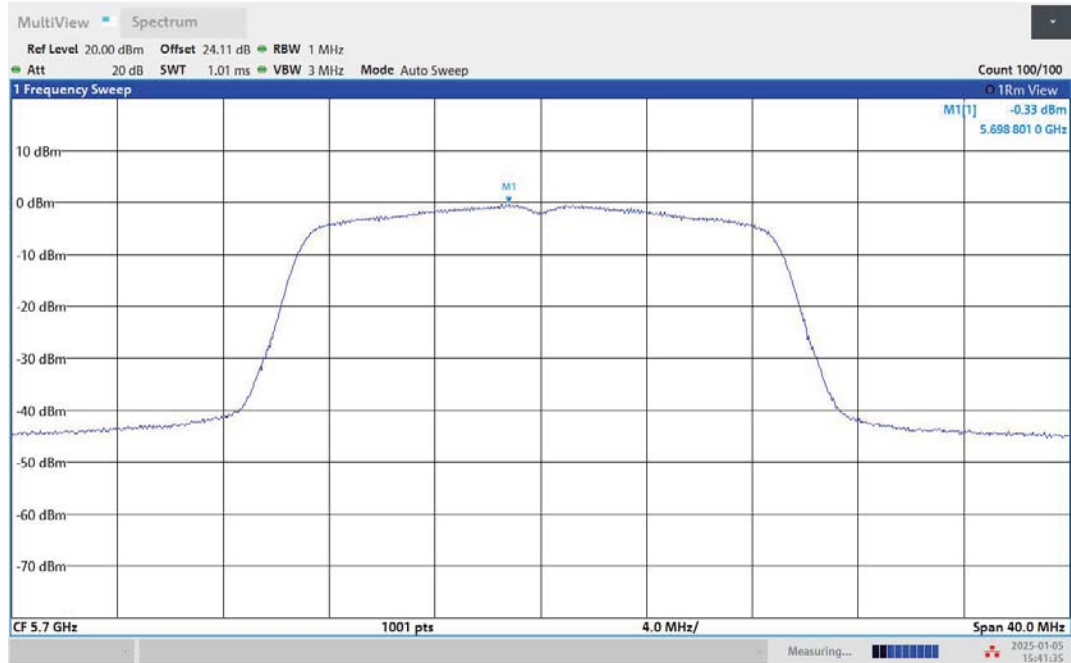
11N20MIMO-Ant2-5700-PASS
