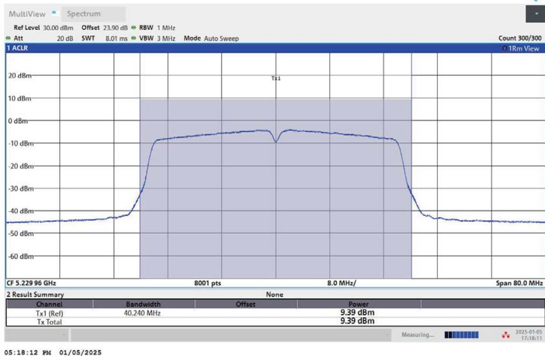
11AC40MIMO-Ant2-5230-PASS
