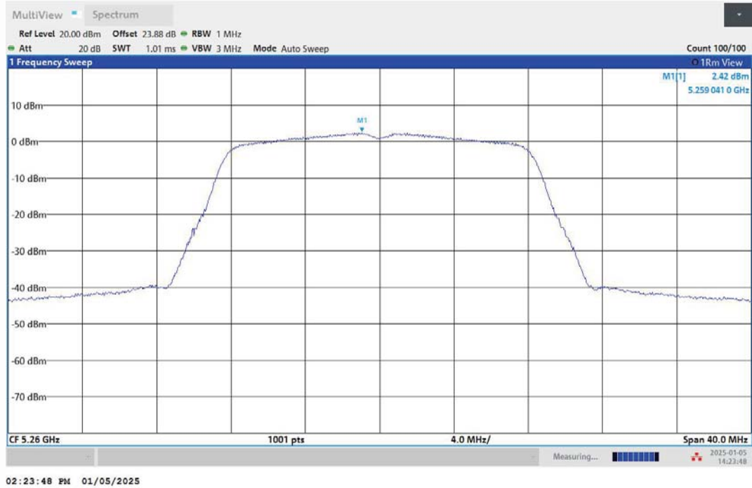
11A-Ant1-5260-PASS
