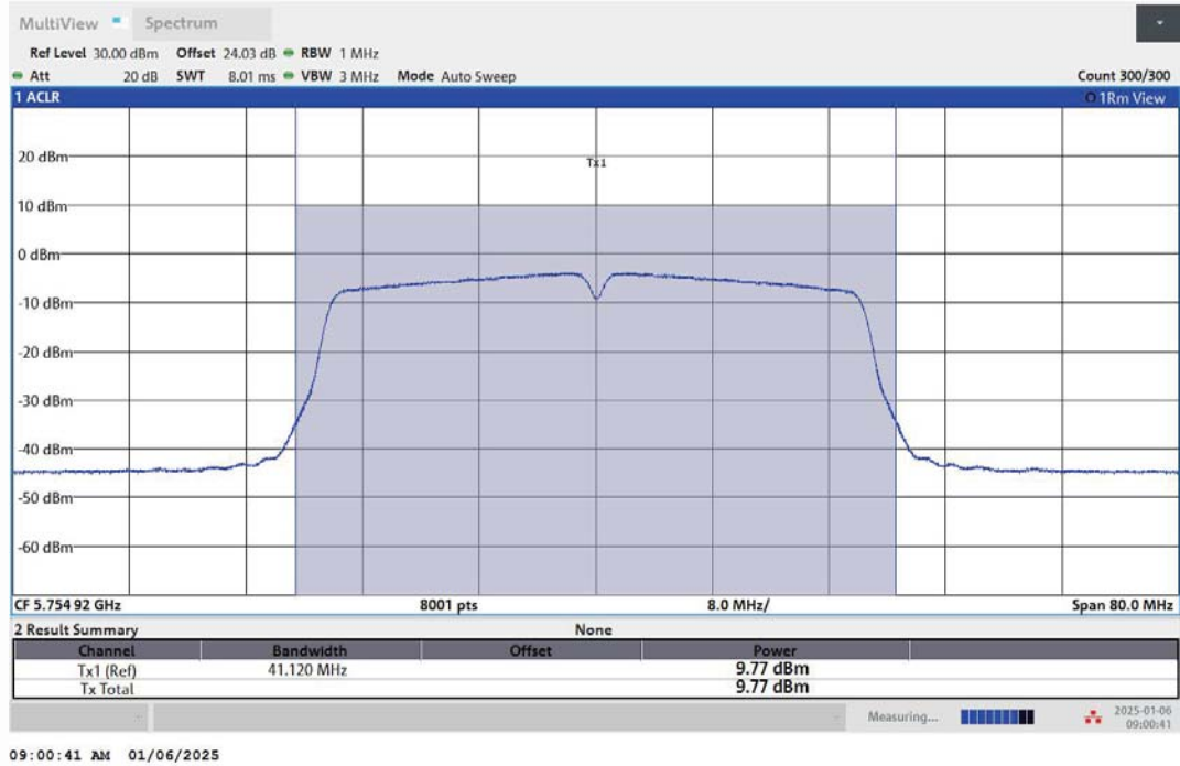
11AC40MIMO-Ant1-5755-PASS
