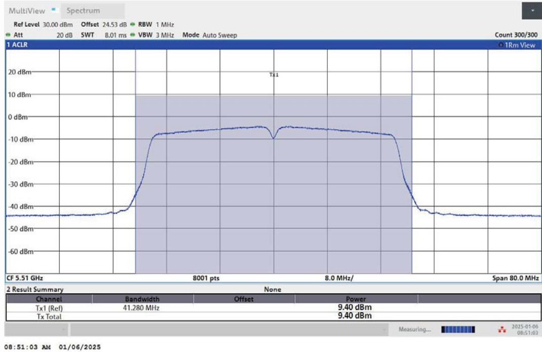
11AC40MIMO-Ant1-5510-PASS
