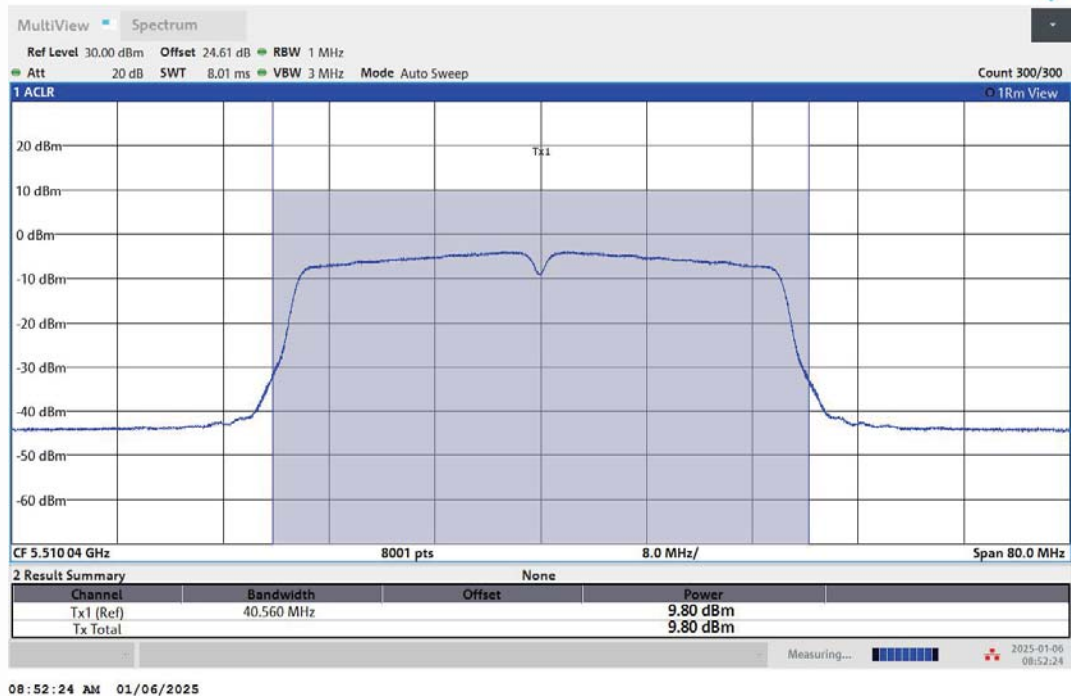
11AC40MIMO-Ant2-5510-PASS
