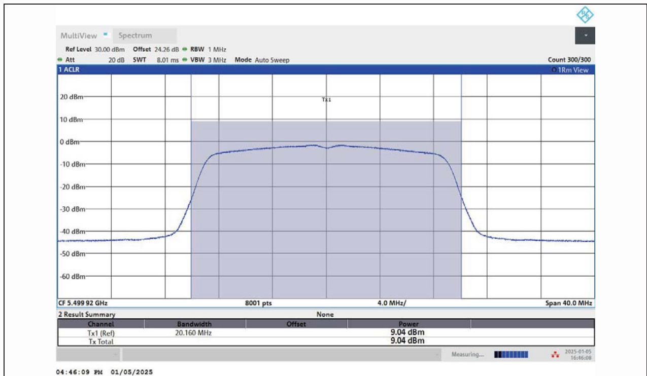
11AC20MIMO-Ant1-5500-PASS
