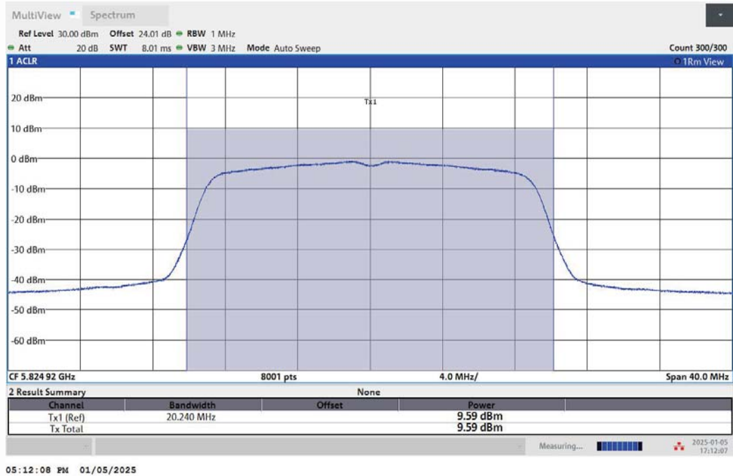
11AC20MIMO-Ant2-5825-PASS
