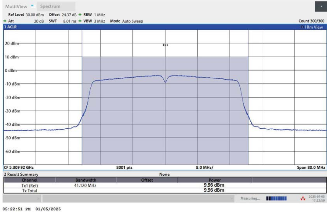
11AC40MIMO-Ant1-5310-PASS
