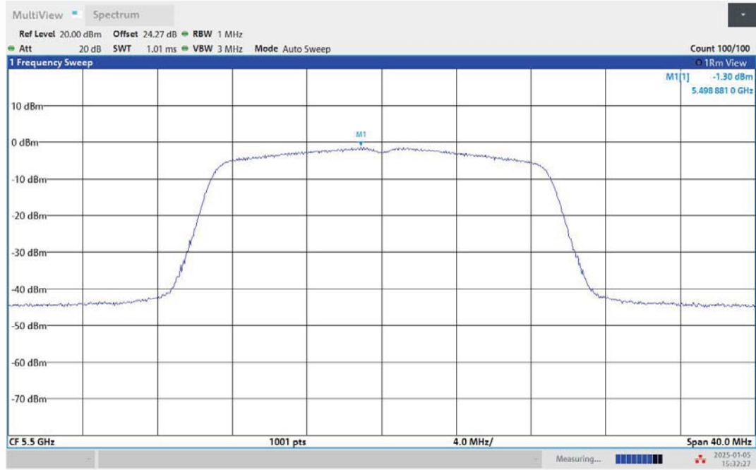
11N20MIMO-Ant1-5500-PASS
