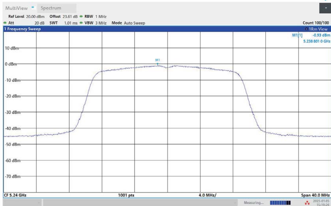
11N20MIMO-Ant1-5240-PASS
