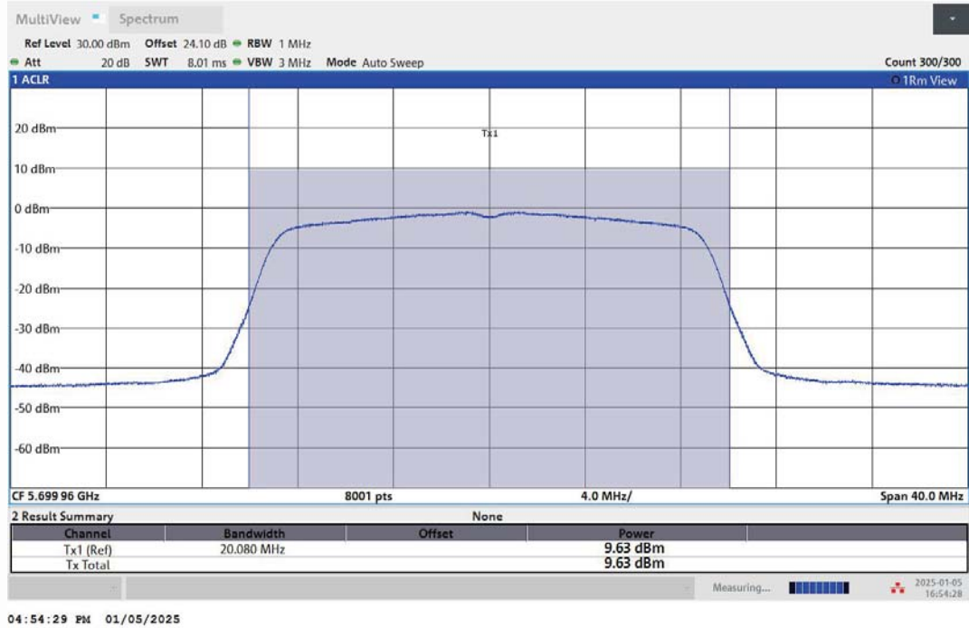
11AC20MIMO-Ant1-5700-PASS
