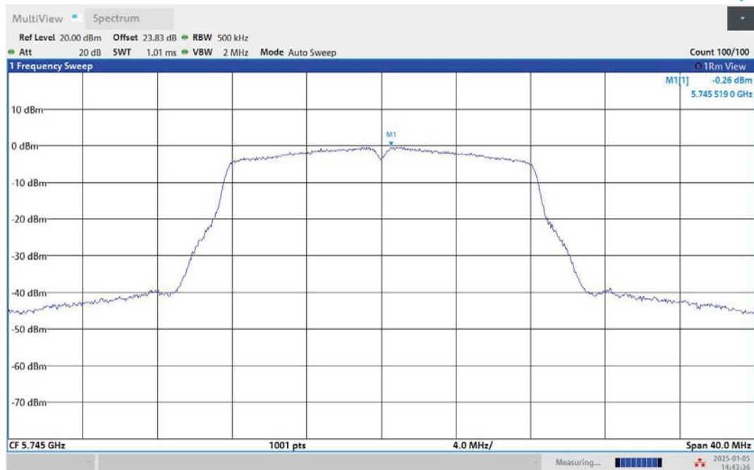
11A-Ant1-5745-PASS
