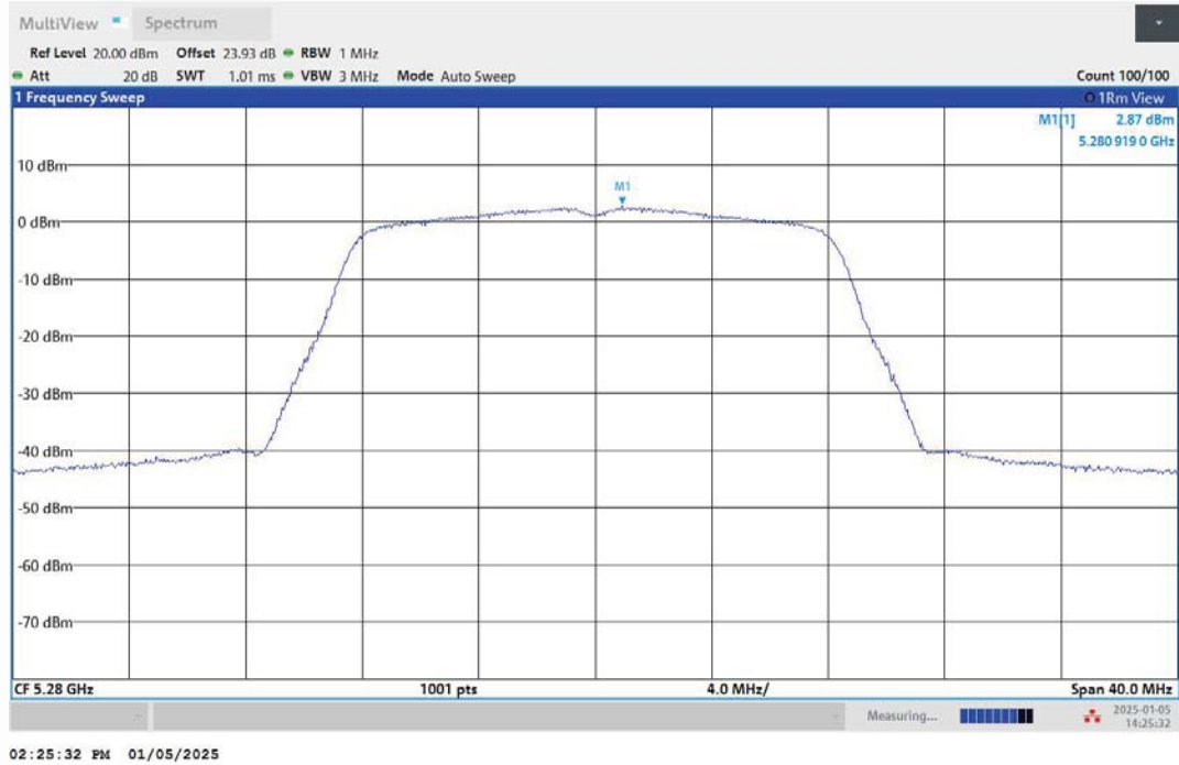
11A-Ant1-5280-PASS
