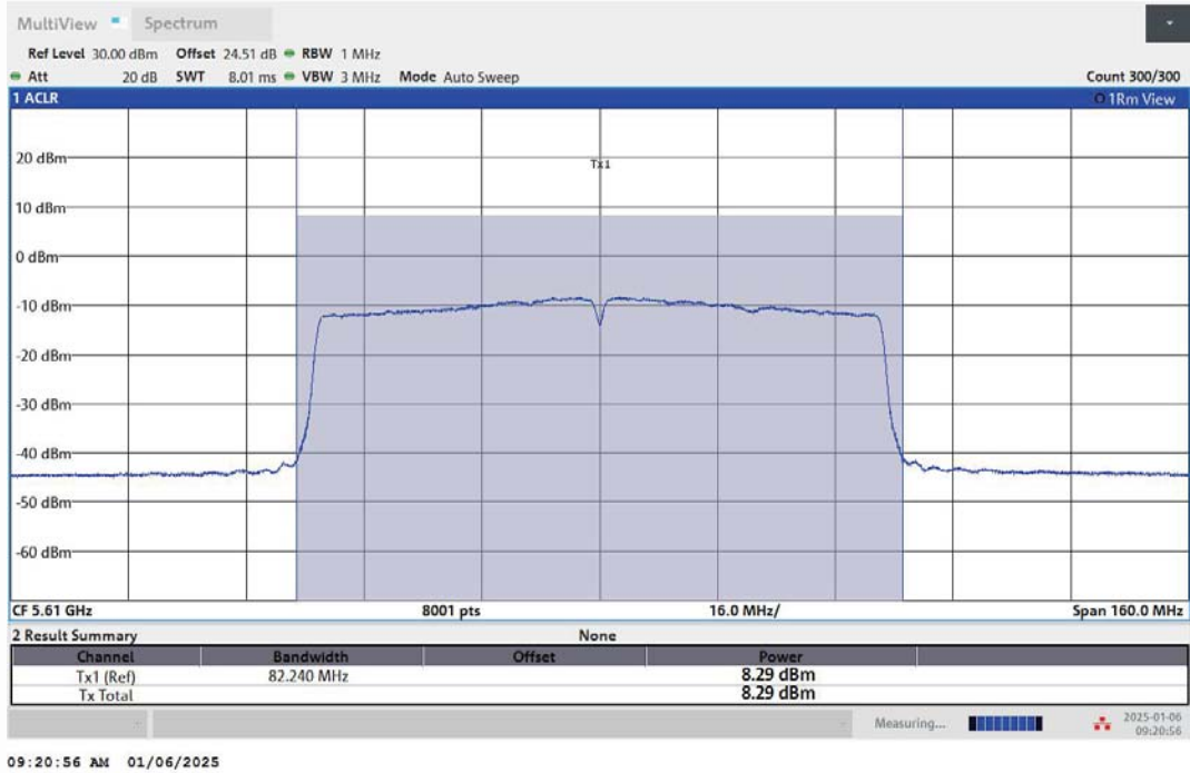
11AC80MIMO-Ant1-5610-PASS
