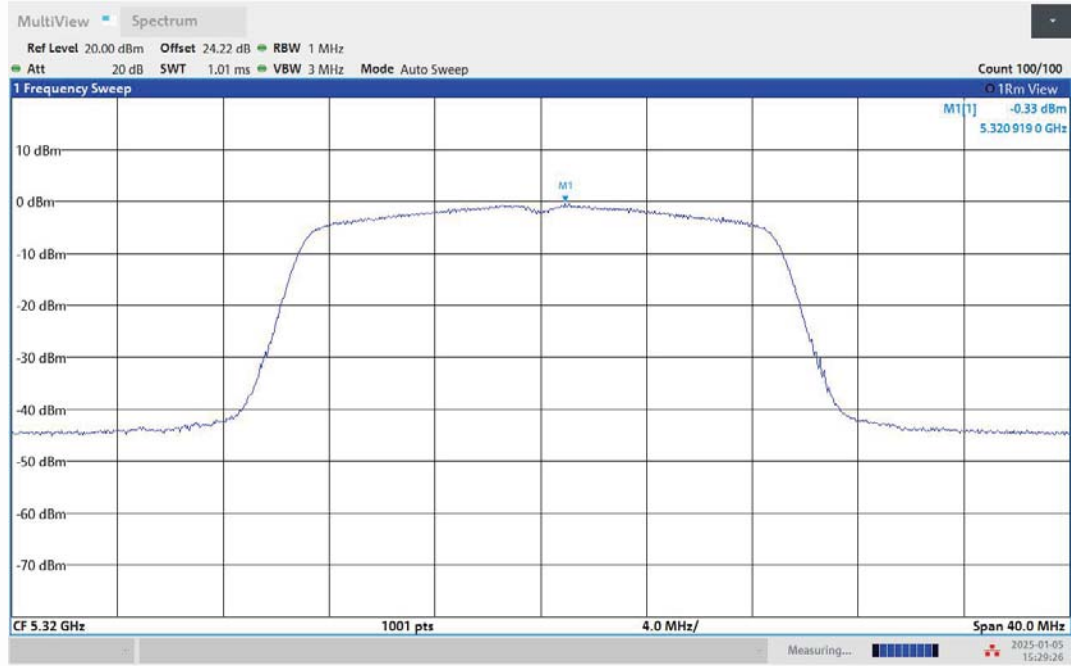
11N20MIMO-Ant1-5320-PASS
