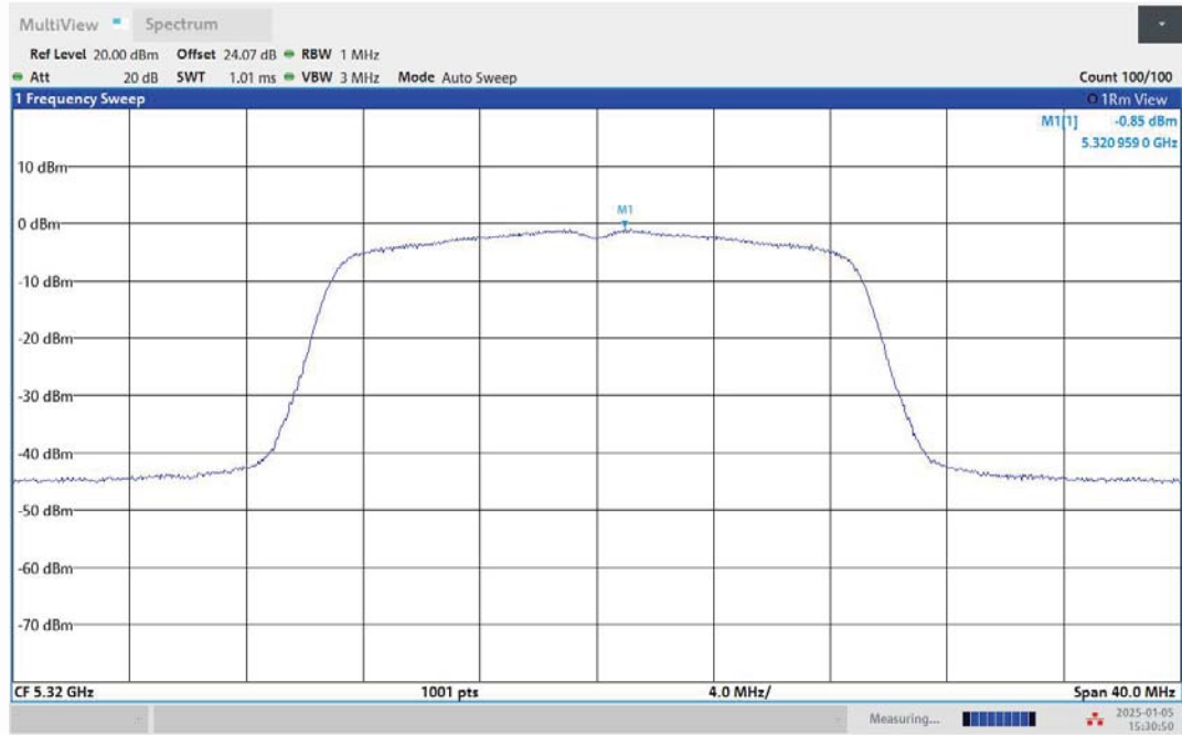
11N20MIMO-Ant2-5320-PASS
