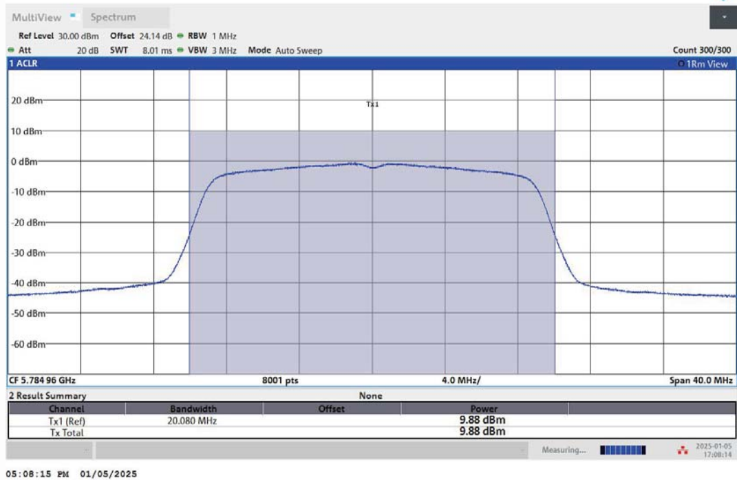
11AC20MIMO-Ant2-5785-PASS
