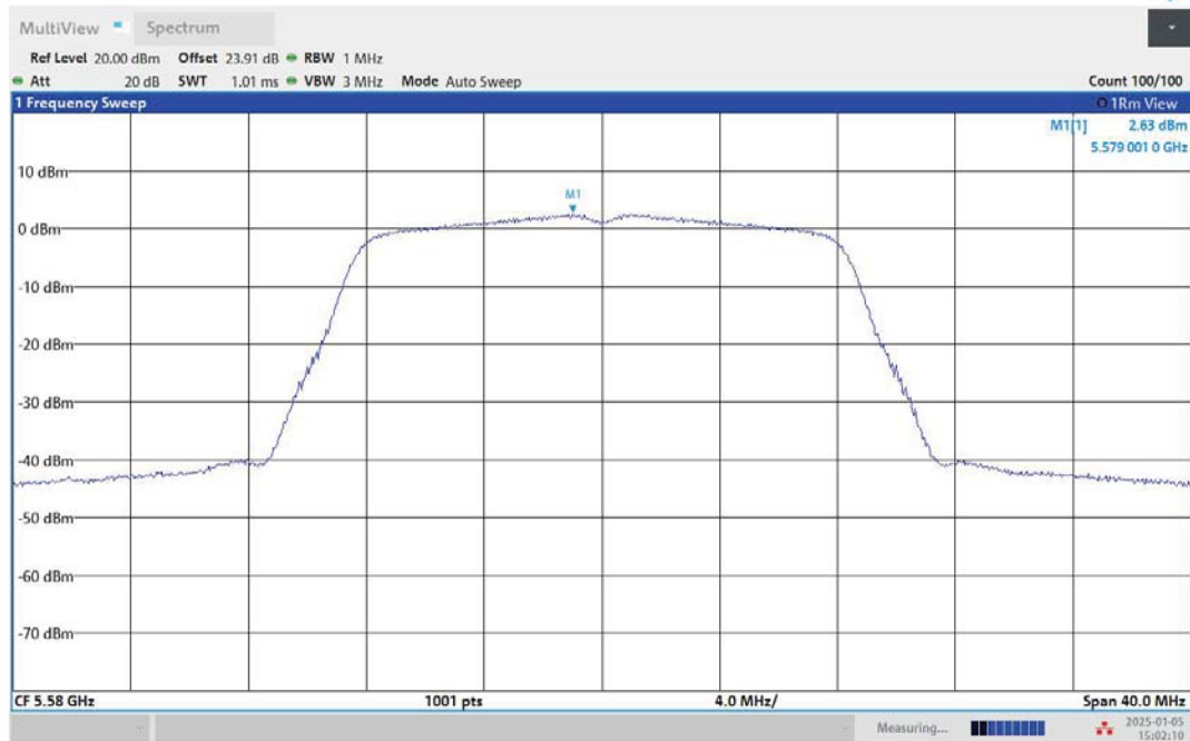
11A-Ant2-5580-PASS
