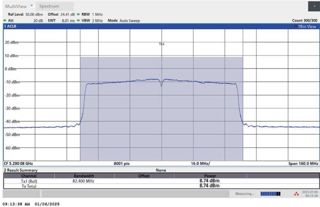
11AC80MIMO-Ant1-5290-PASS
