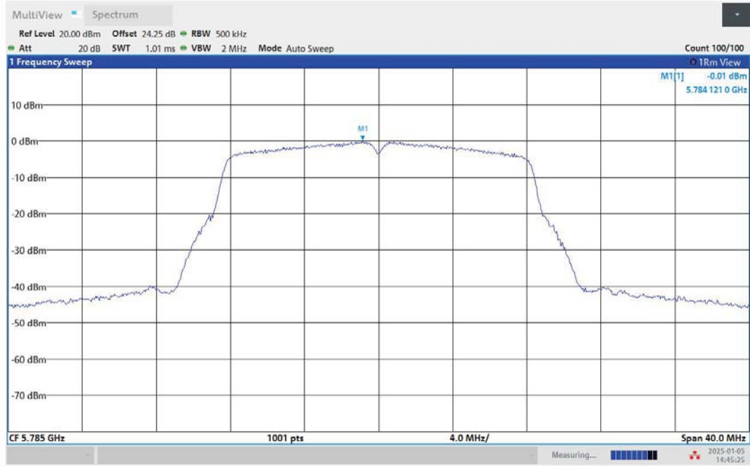
11A-Ant1-5785-PASS
