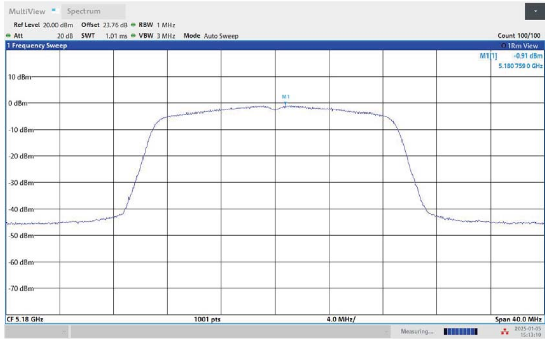
11N20MIMO-Ant2-5180-PASS
