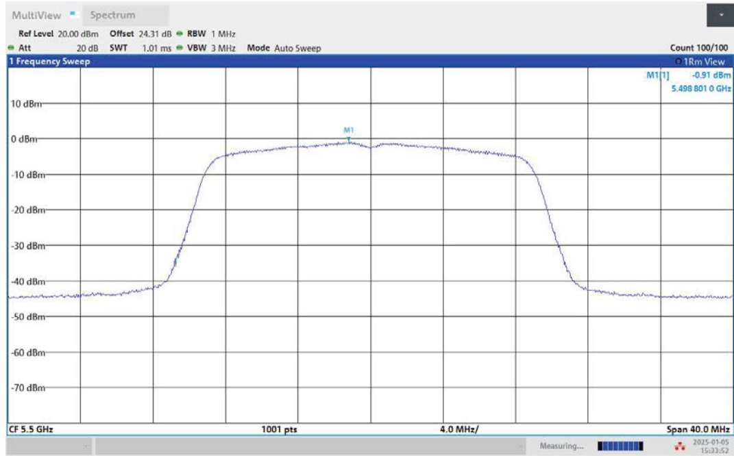
11N20MIMO-Ant2-5500-PASS
