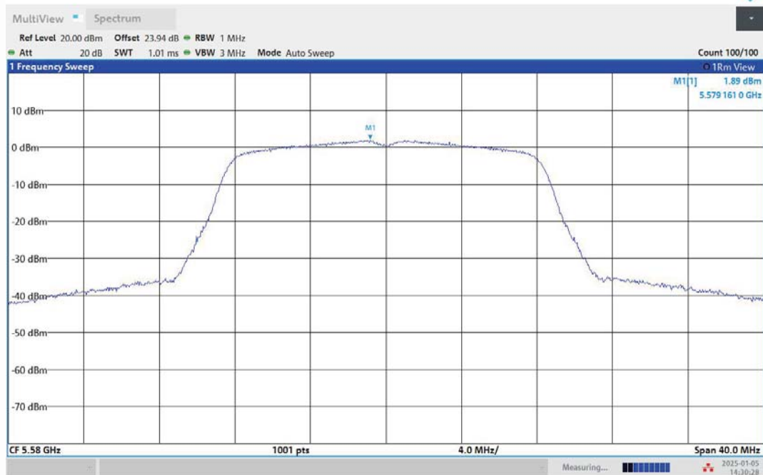
11A-Ant1-5580-PASS
