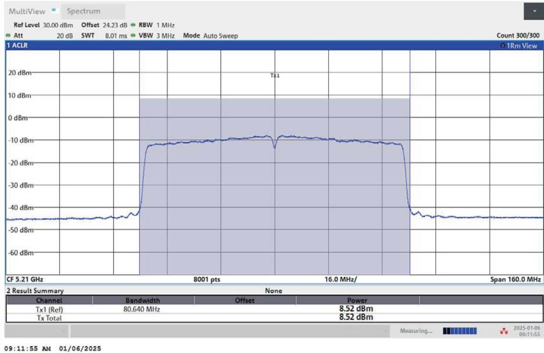
11AC80MIMO-Ant2-5210-PASS
