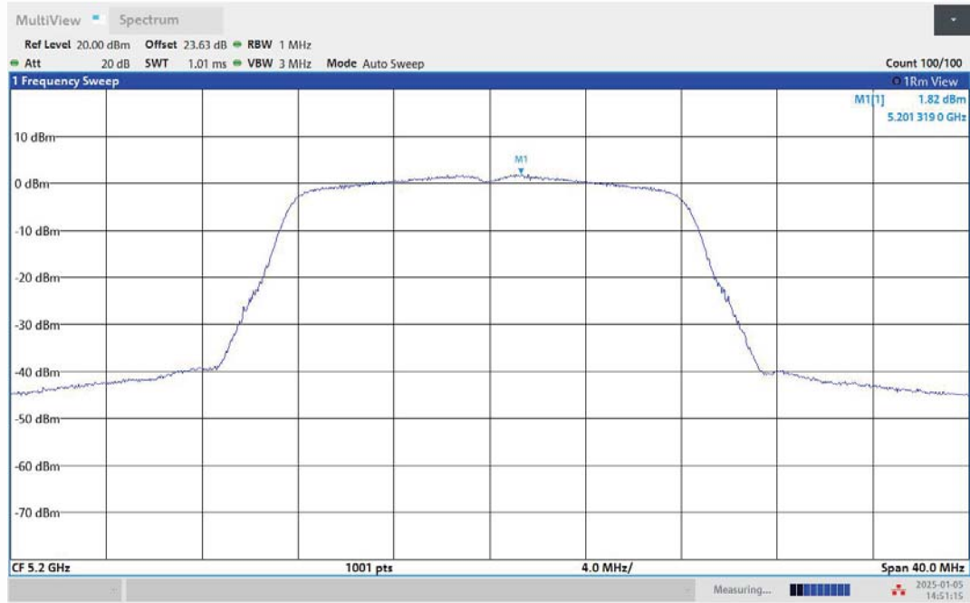
11A-Ant2-5200-PASS
