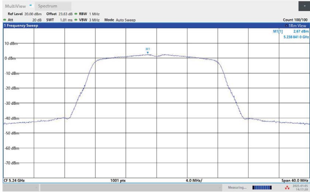
11A-Ant1-5240-PASS
