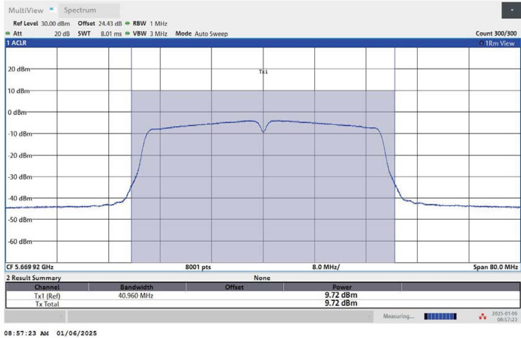
11AC40MIMO-Ant1-5670-PASS
