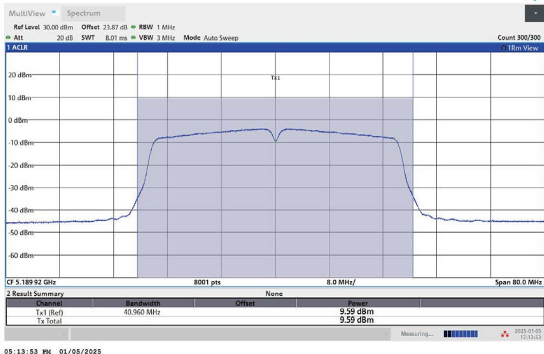
11AC40MIMO-Ant1-5190-PASS
