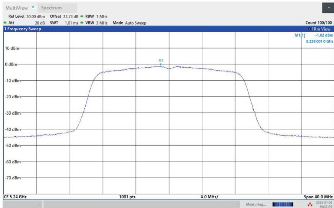
11AC20MIMO-Ant2-5240-PASS
