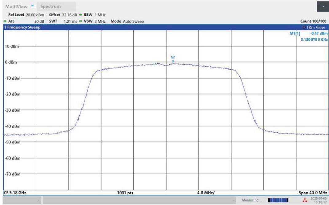
11AC20MIMO-Ant1-5180-PASS
