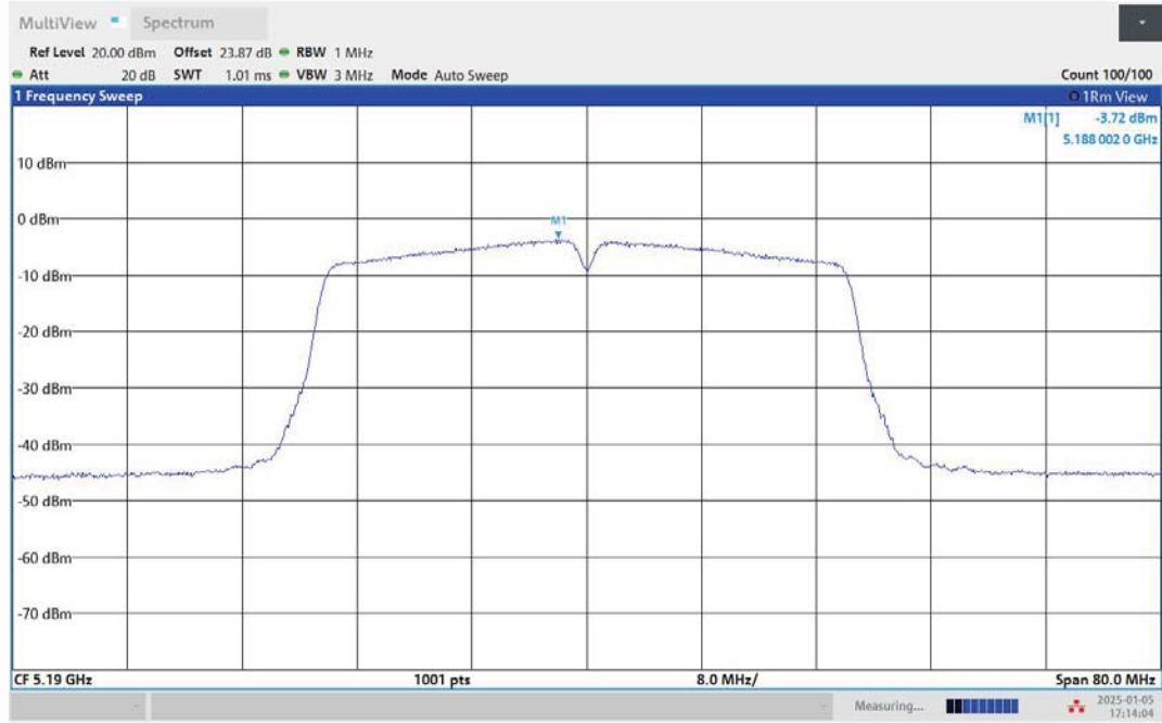
11AC40MIMO-Ant1-5190-PASS
