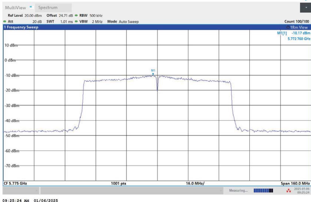
11AC80MIMO-Ant1-5775-PASS
