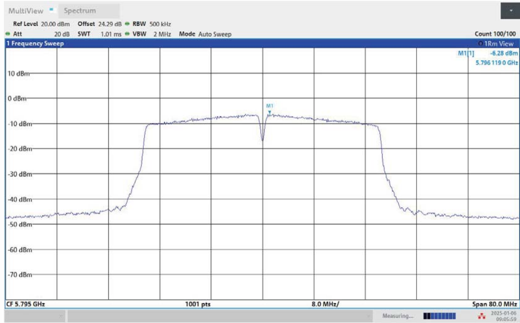
11AC40MIMO-Ant2-5795-PASS
