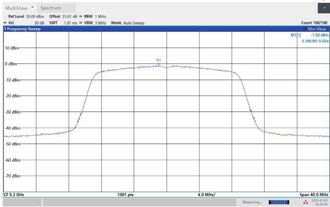
11AC20MIMO-Ant1-5200-PASS
