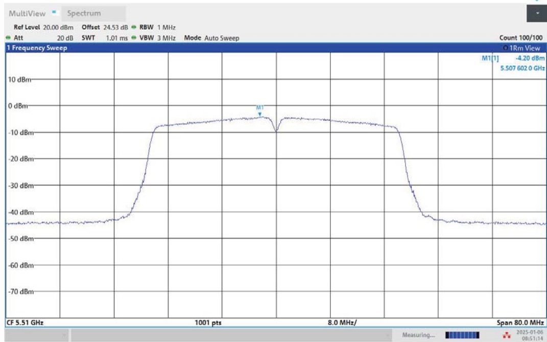
11AC40MIMO-Ant1-5510-PASS
