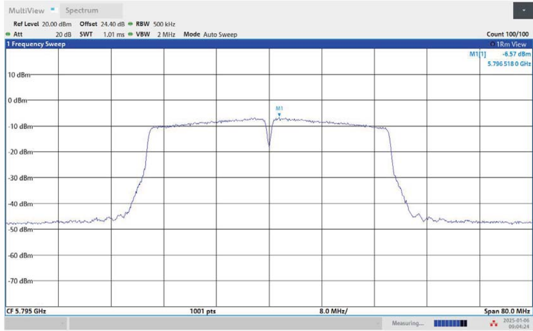
11AC40MIMO-Ant1-5795-PASS
