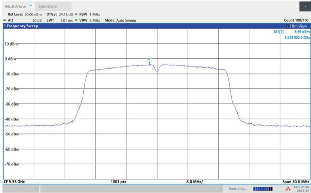
11AC40MIMO-Ant2-5550-PASS
