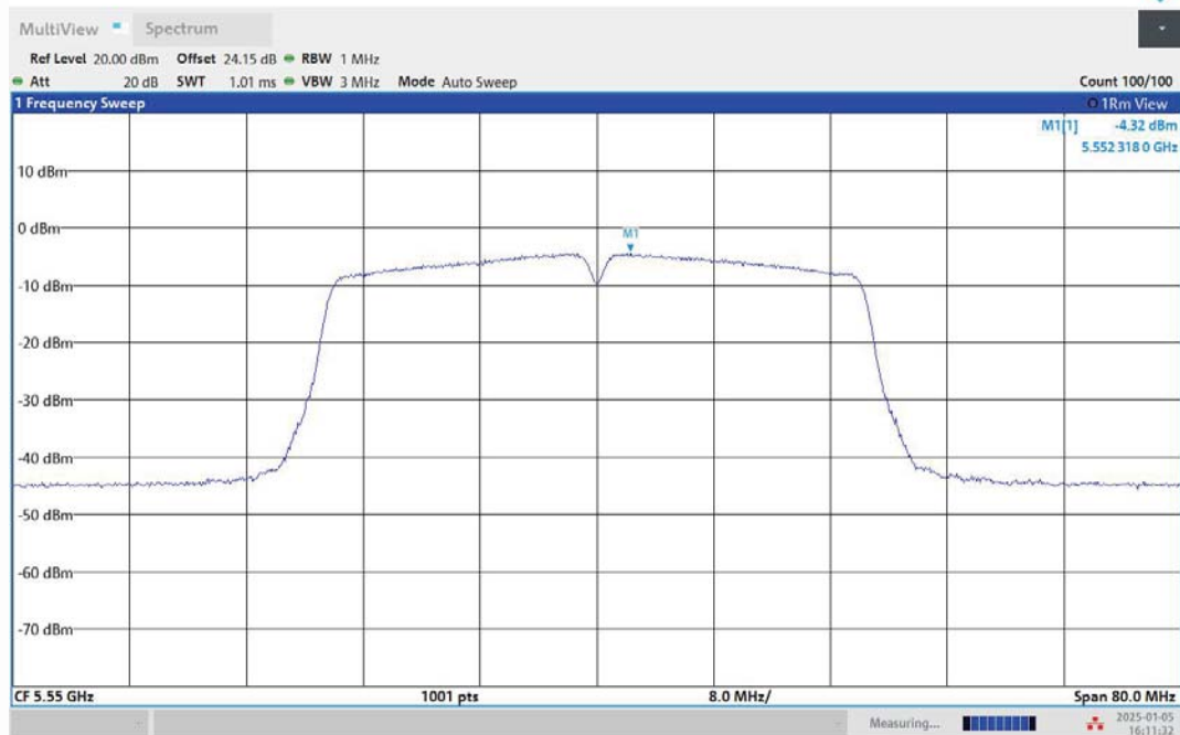
11N40MIMO-Ant1-5550-PASS
