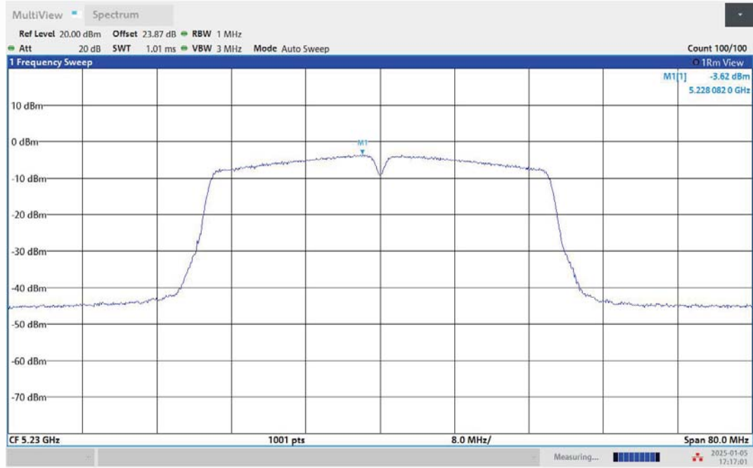
11AC40MIMO-Ant1-5230-PASS
