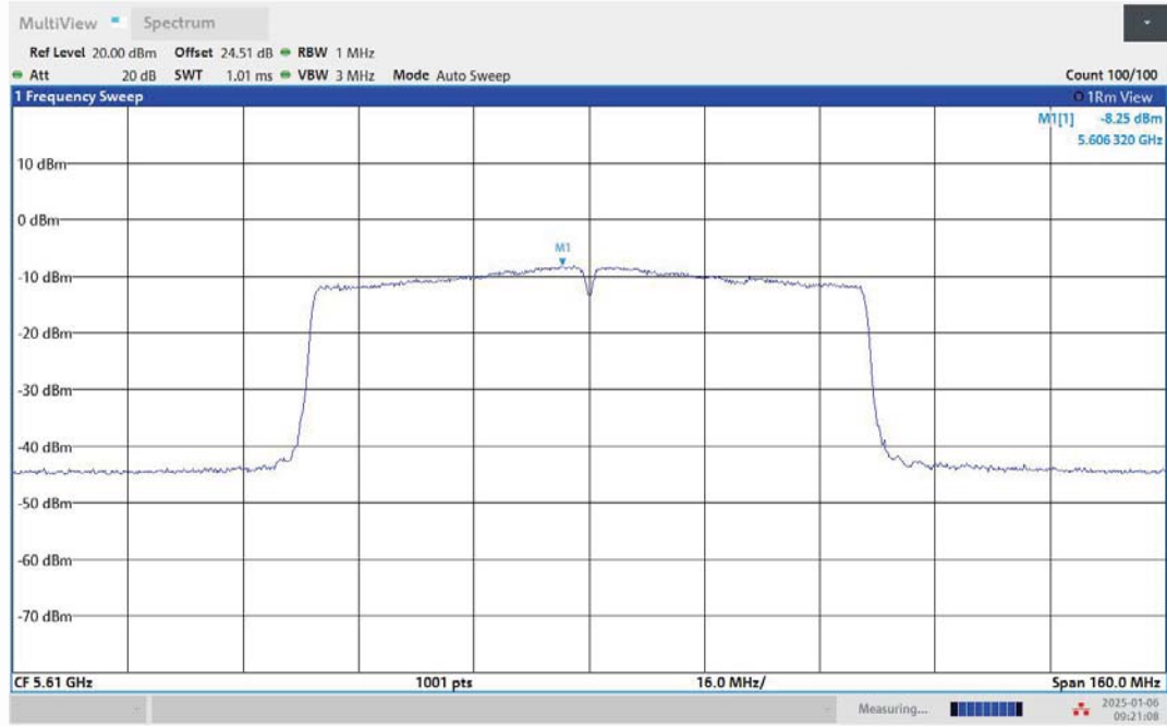
11AC80MIMO-Ant1-5610-PASS
