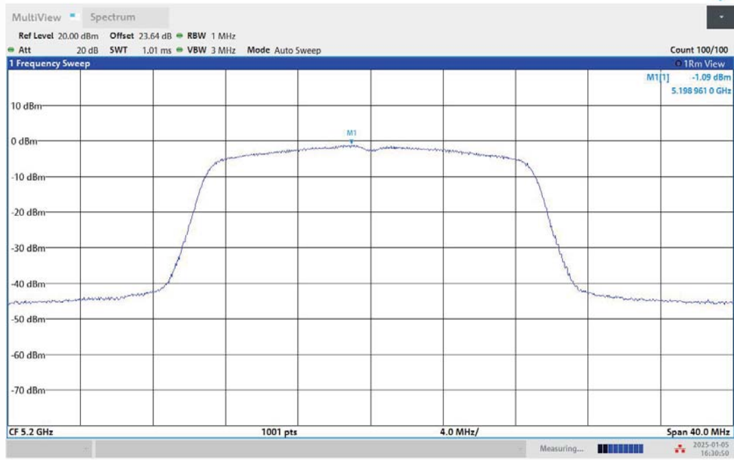
11AC20MIMO-Ant2-5200-PASS
