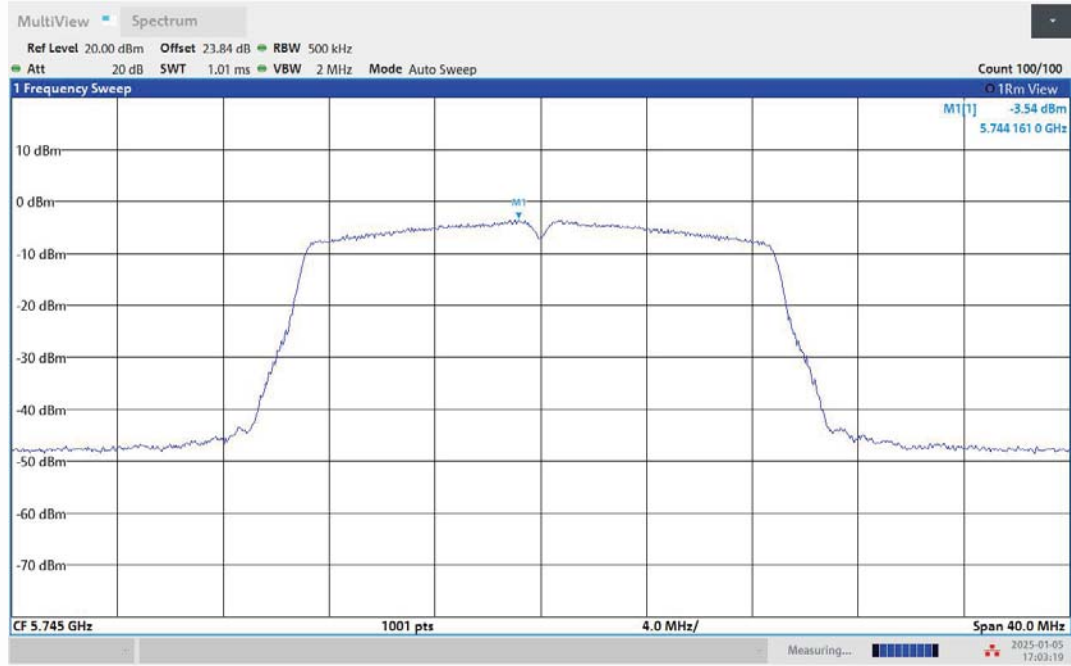
11AC20MIMO-Ant1-5745-PASS
