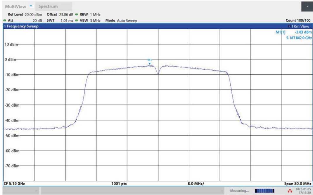
11AC40MIMO-Ant2-5190-PASS
