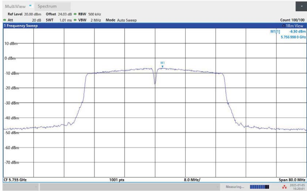
11N40MIMO-Ant2-5755-PASS
