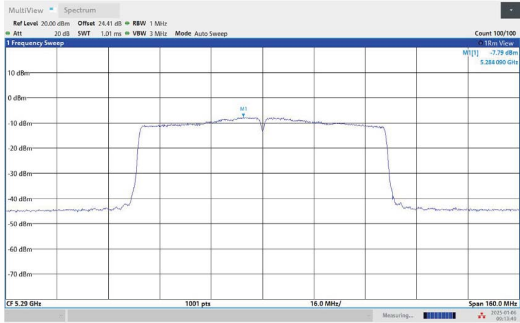
11AC80MIMO-Ant1-5290-PASS
