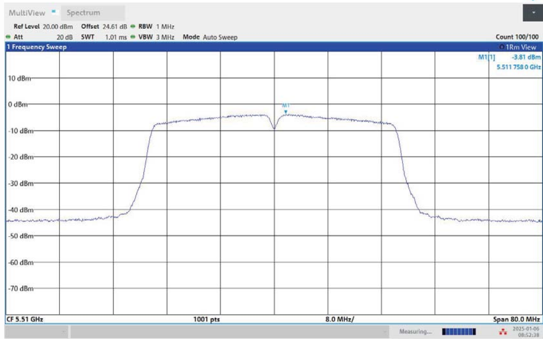
11AC40MIMO-Ant2-5510-PASS
