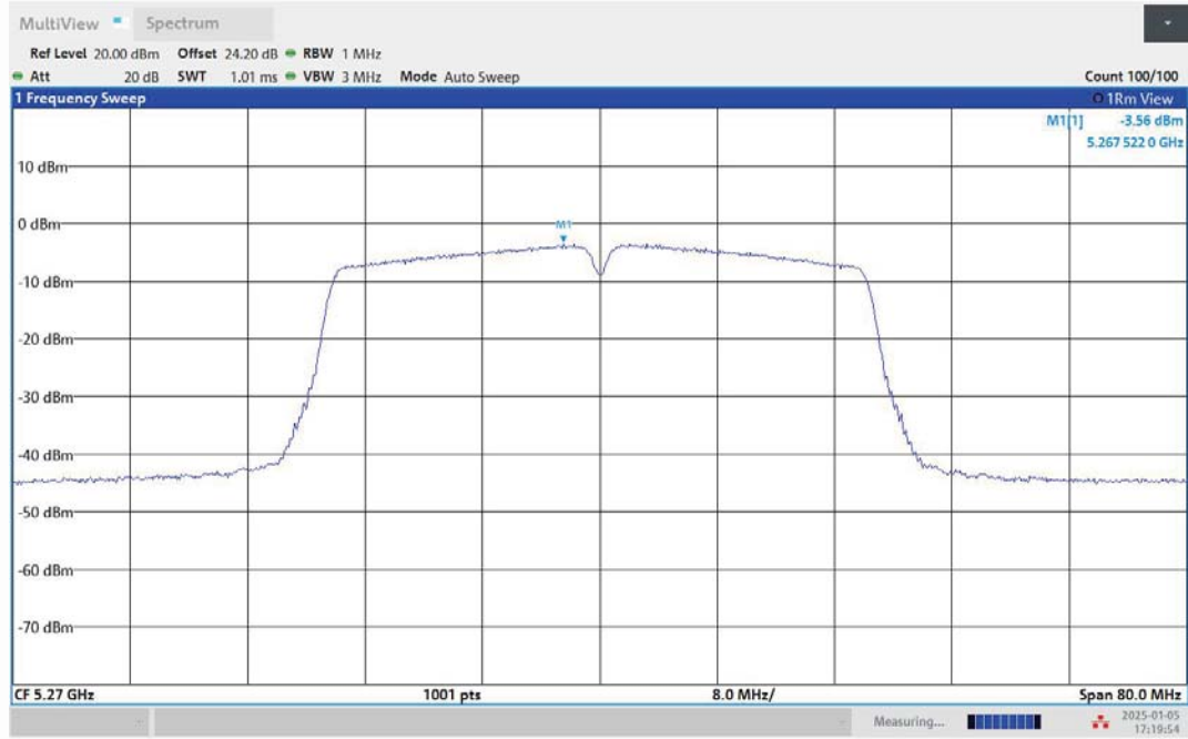
11AC40MIMO-Ant1-5270-PASS
