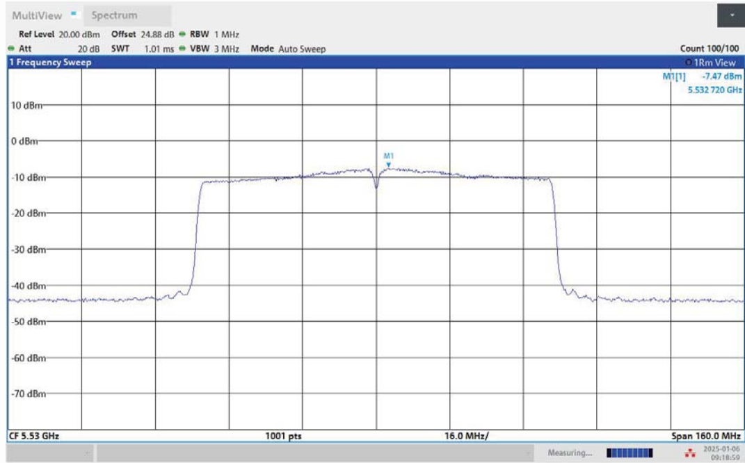
11AC80MIMO-Ant2-5530-PASS
