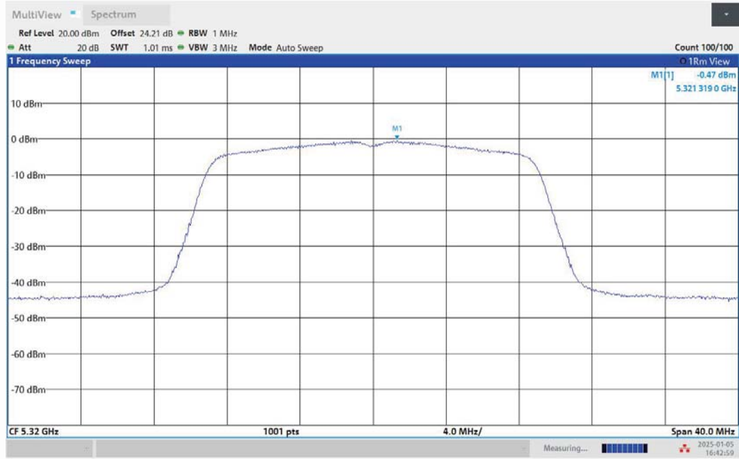
11AC20MIMO-Ant1-5320-PASS
