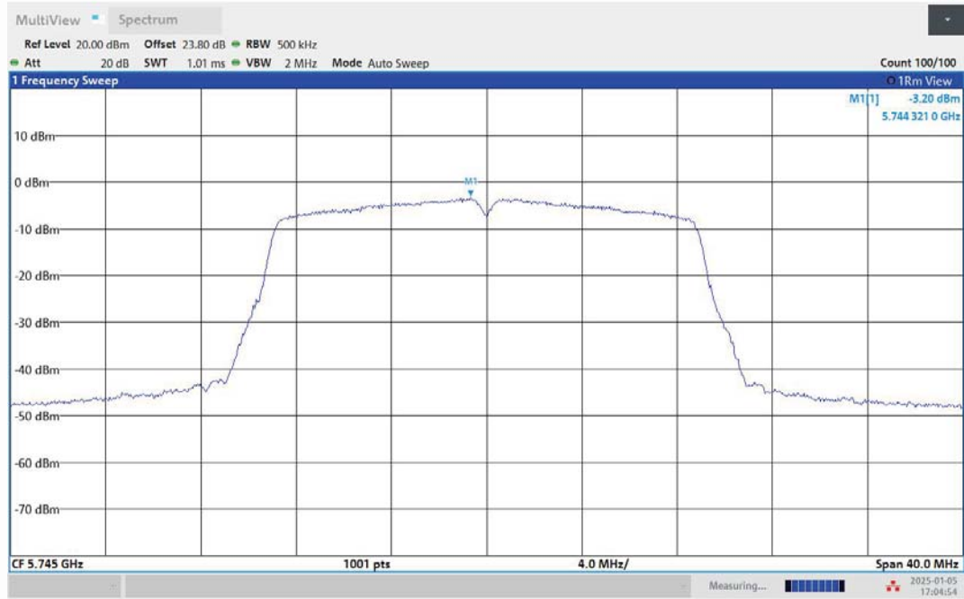
11AC20MIMO-Ant2-5745-PASS
