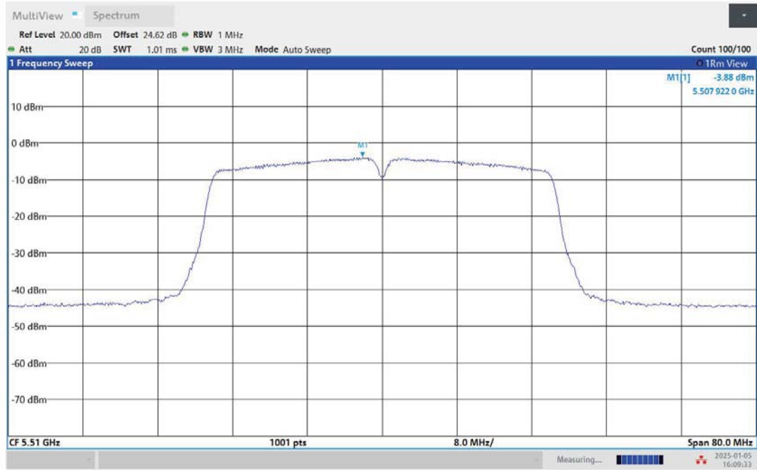
11N40MIMO-Ant2-5510-PASS
