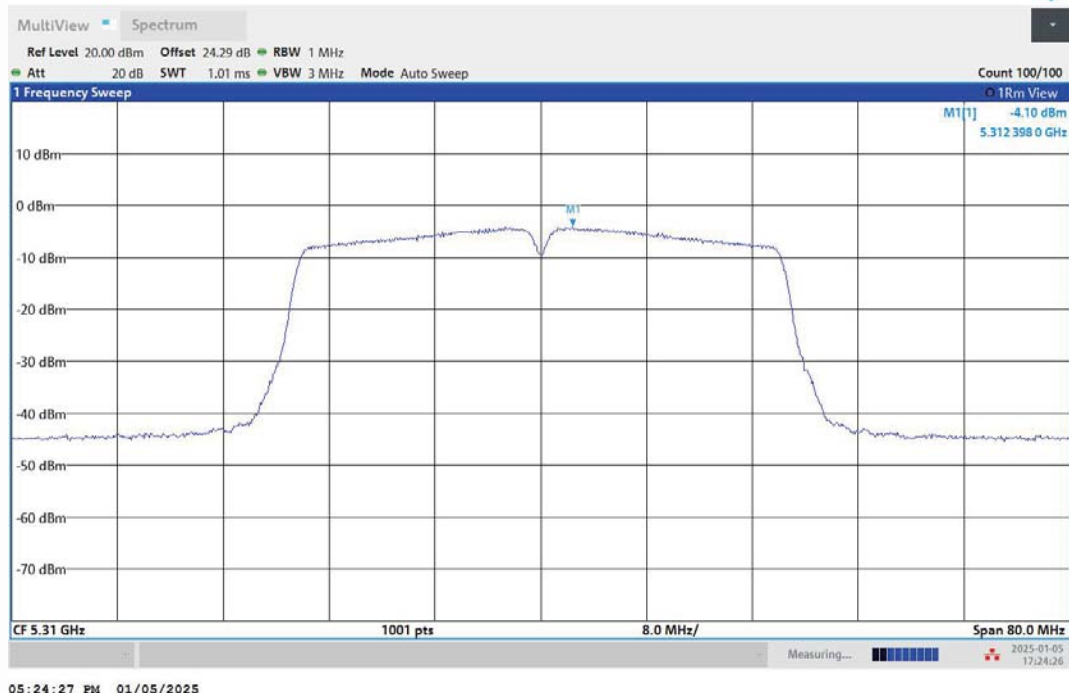
11AC40MIMO-Ant2-5310-PASS
