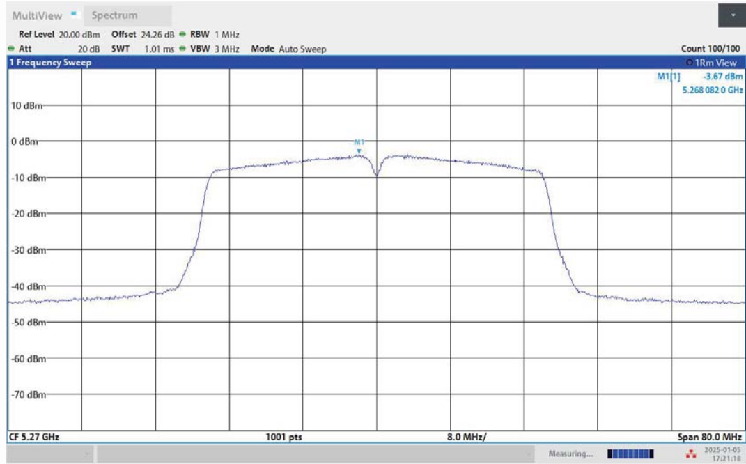
11AC40MIMO-Ant2-5270-PASS
