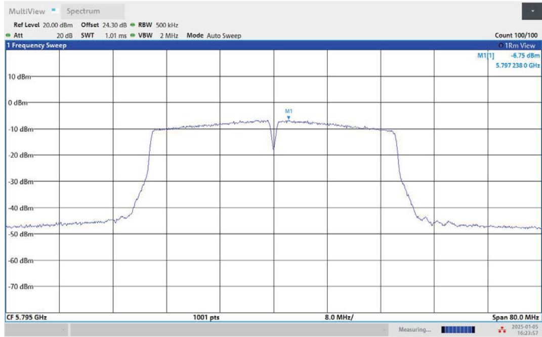
11N40MIMO-Ant2-5795-PASS
