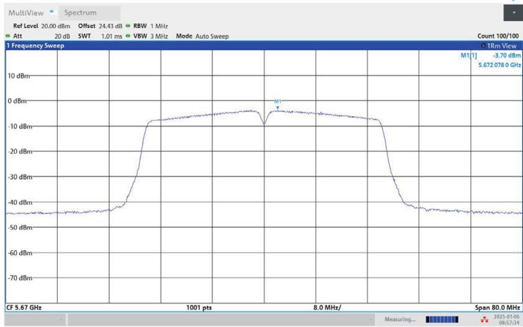
11AC40MIMO-Ant1-5670-PASS
