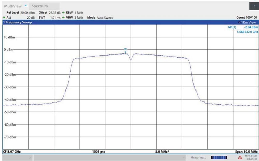
11AC40MIMO-Ant2-5670-PASS
