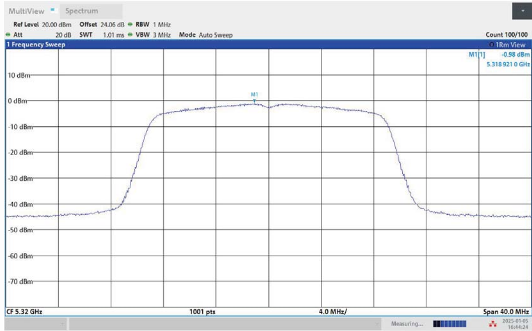
11AC20MIMO-Ant2-5320-PASS
