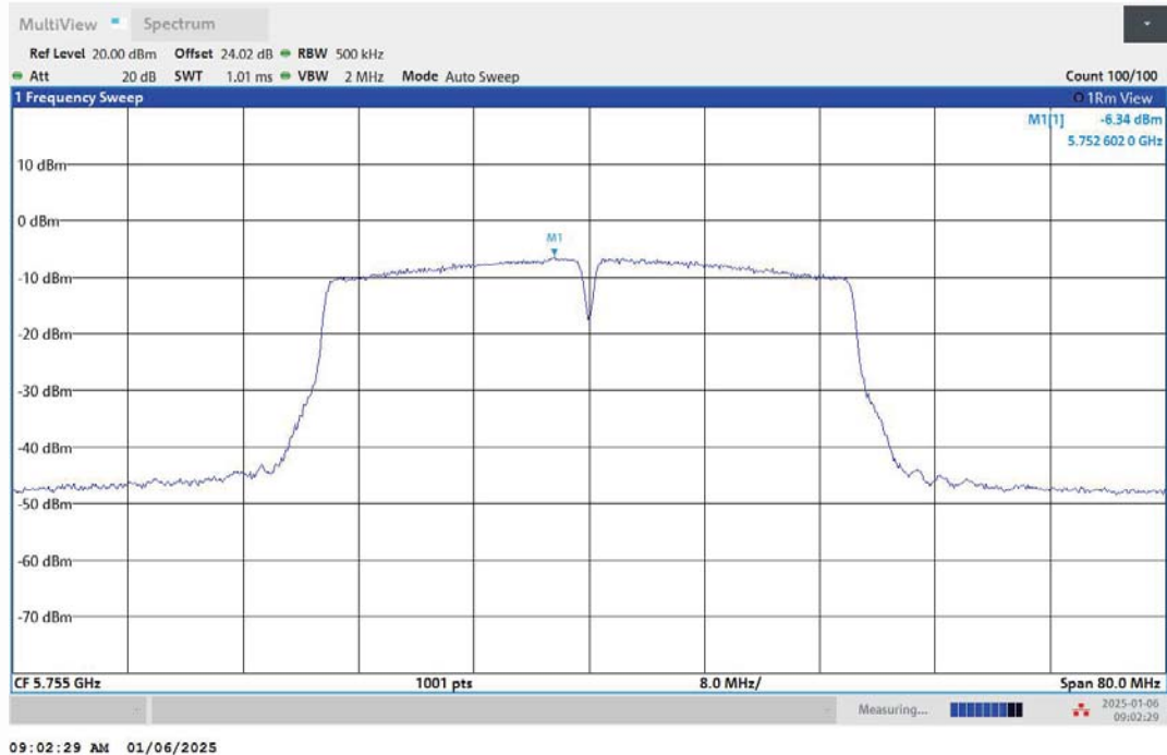
11AC40MIMO-Ant2-5755-PASS
