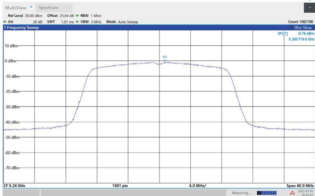
11AC20MIMO-Ant1-5240-PASS
