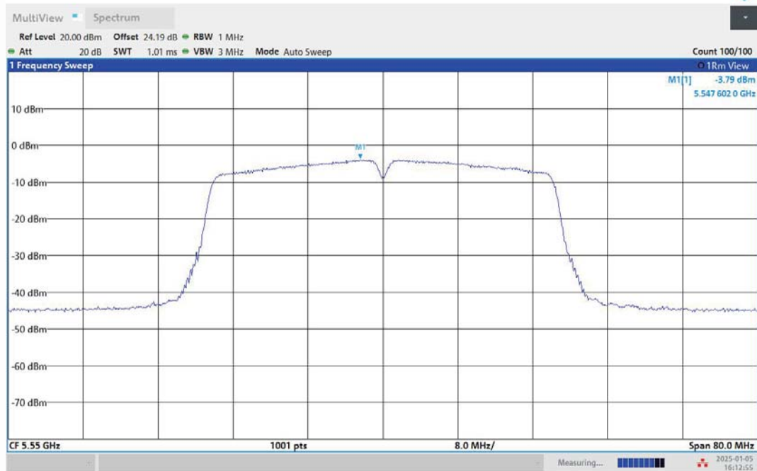
11N40MIMO-Ant2-5550-PASS
