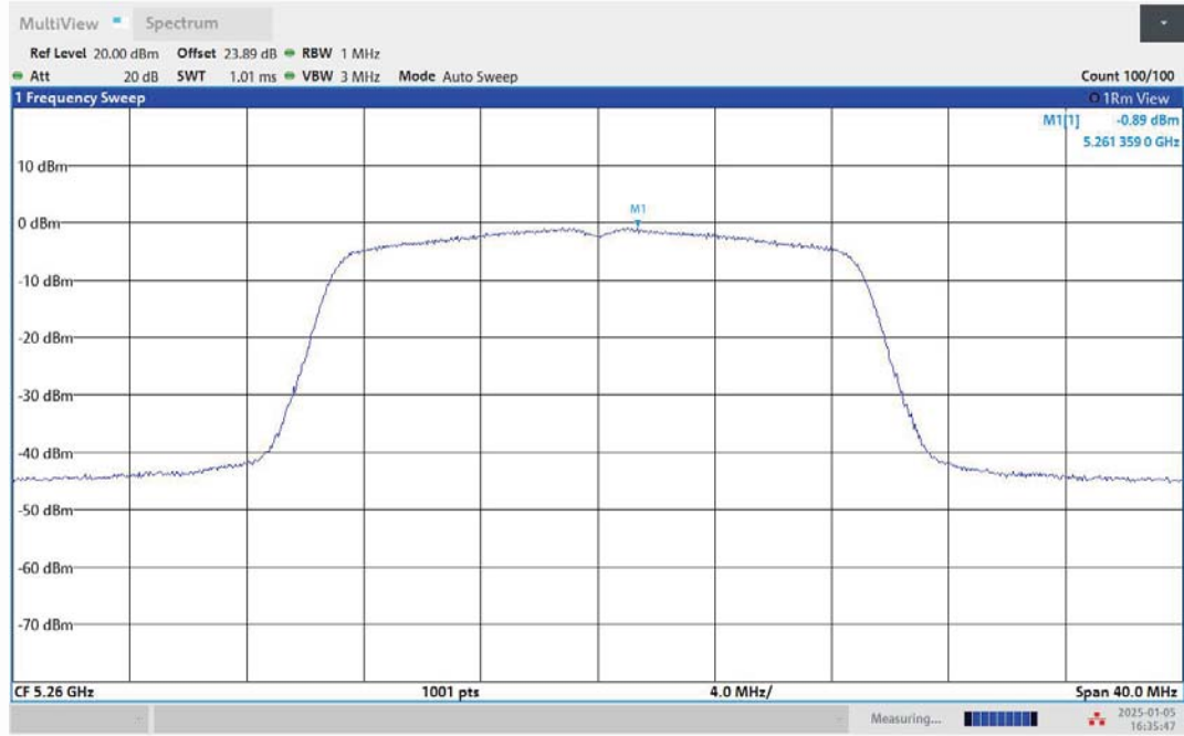
11AC20MIMO-Ant1-5260-PASS
