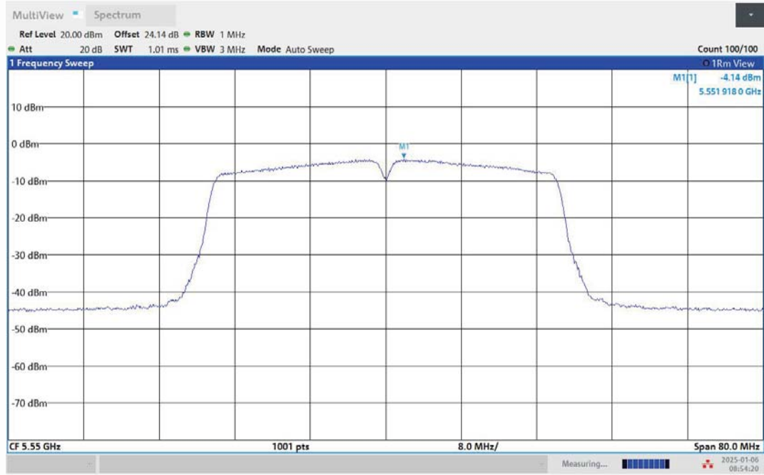
11AC40MIMO-Ant1-5550-PASS
