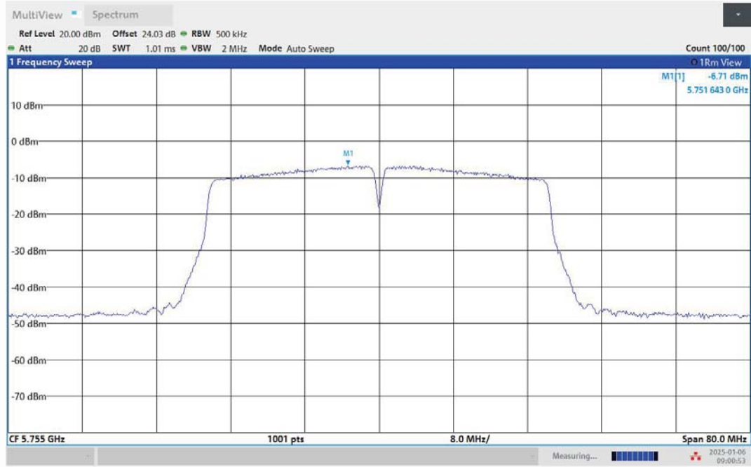
11AC40MIMO-Ant1-5755-PASS
