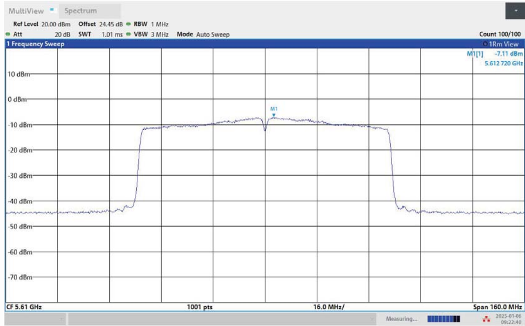
11AC80MIMO-Ant2-5610-PASS
