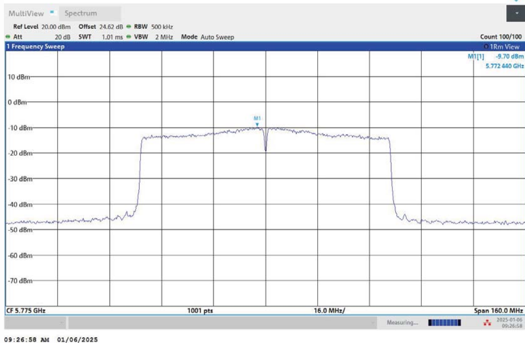
11AC80MIMO-Ant2-5775-PASS
