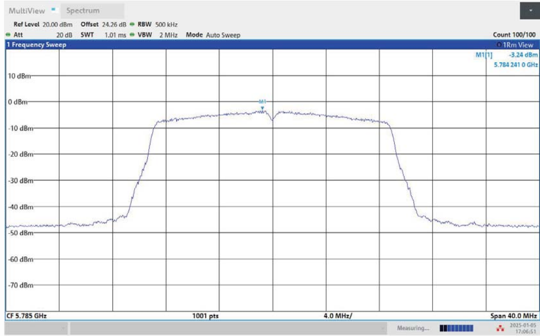
11AC20MIMO-Ant1-5785-PASS
