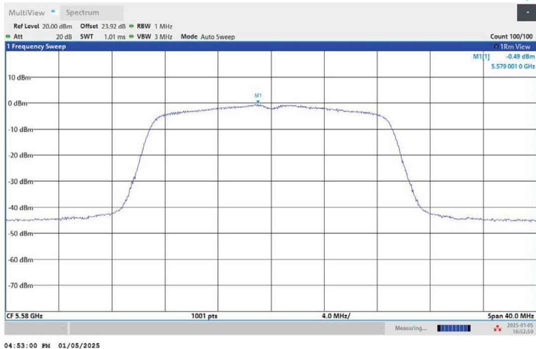
11AC20MIMO-Ant2-5580-PASS
