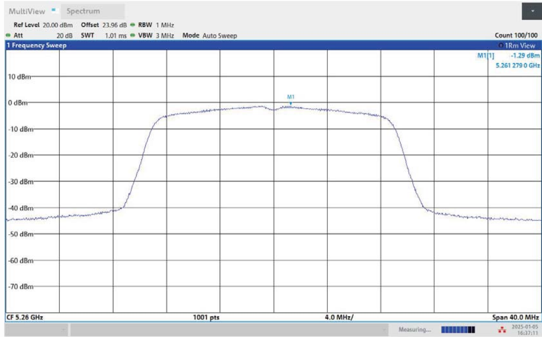
11AC20MIMO-Ant2-5260-PASS
