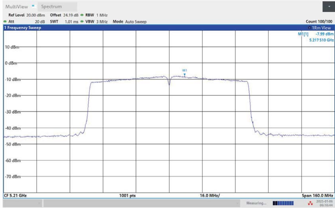
11AC80MIMO-Ant1-5210-PASS
