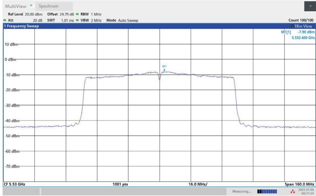
11AC80MIMO-Ant1-5530-PASS
