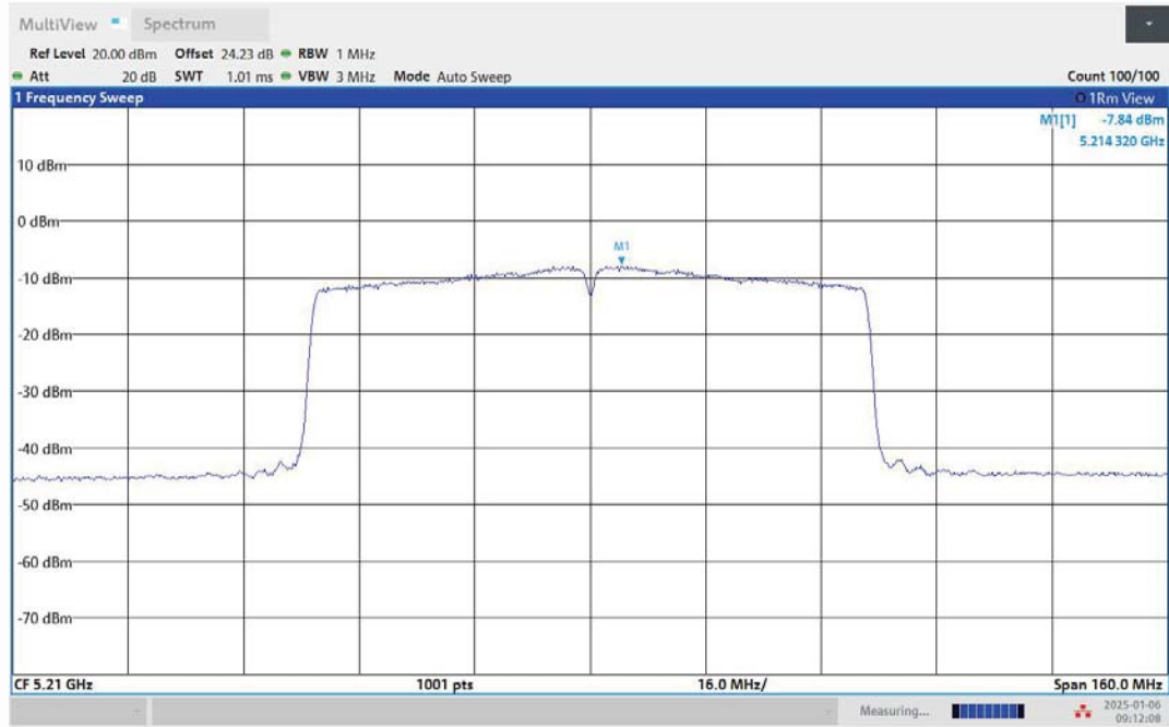
11AC80MIMO-Ant2-5210-PASS
