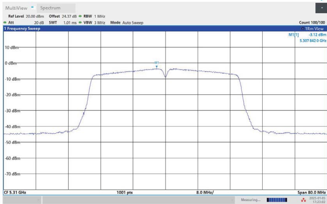
11AC40MIMO-Ant1-5310-PASS
