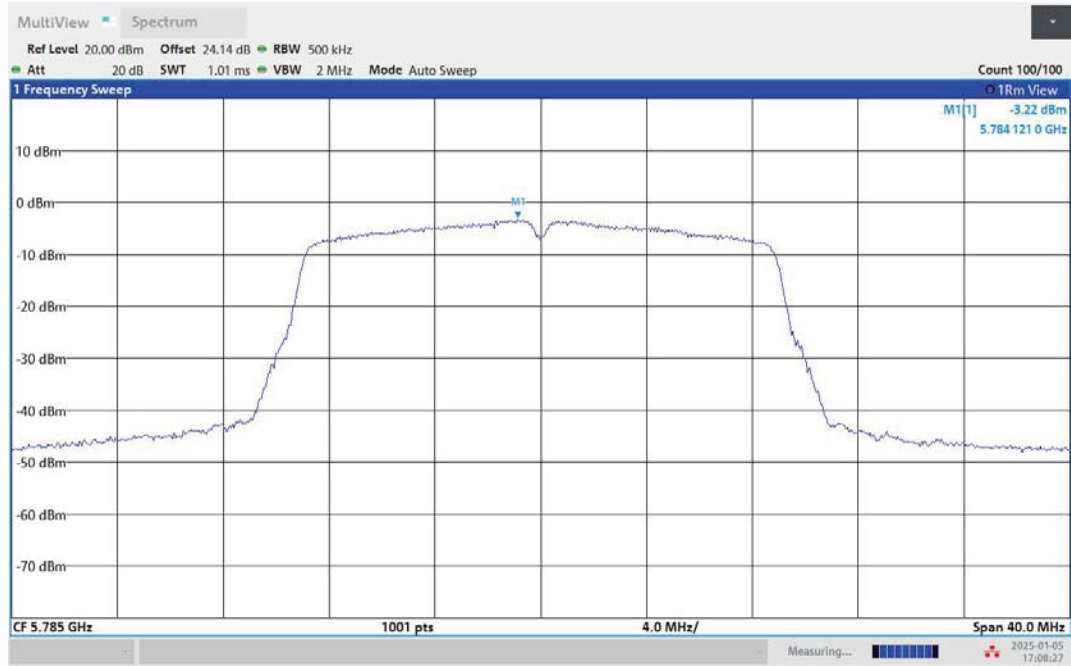
11AC20MIMO-Ant2-5785-PASS
