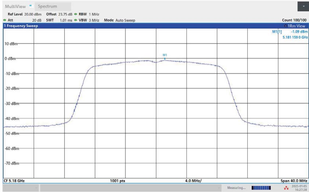
11AC20MIMO-Ant2-5180-PASS
