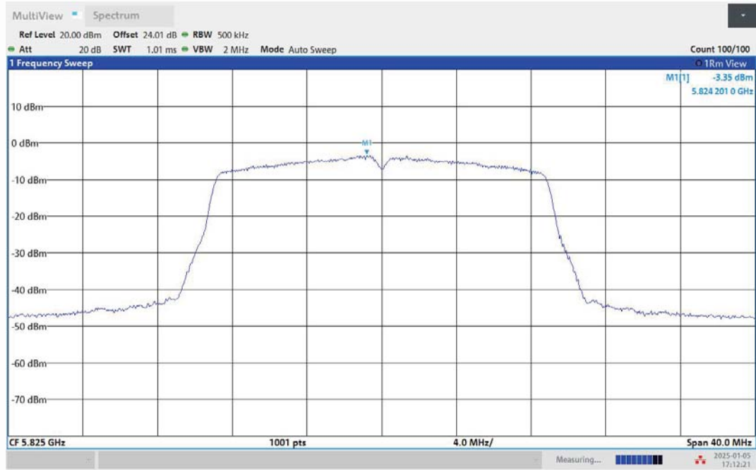
11AC20MIMO-Ant2-5825-PASS
