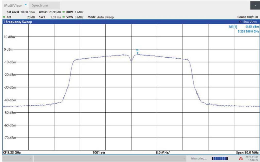
11AC40MIMO-Ant2-5230-PASS
