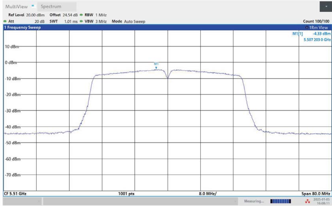
11N40MIMO-Ant1-5510-PASS
