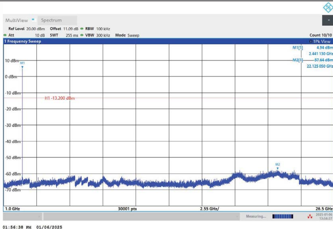
3DH5-Ant1-2441-1000~26500-PASS
