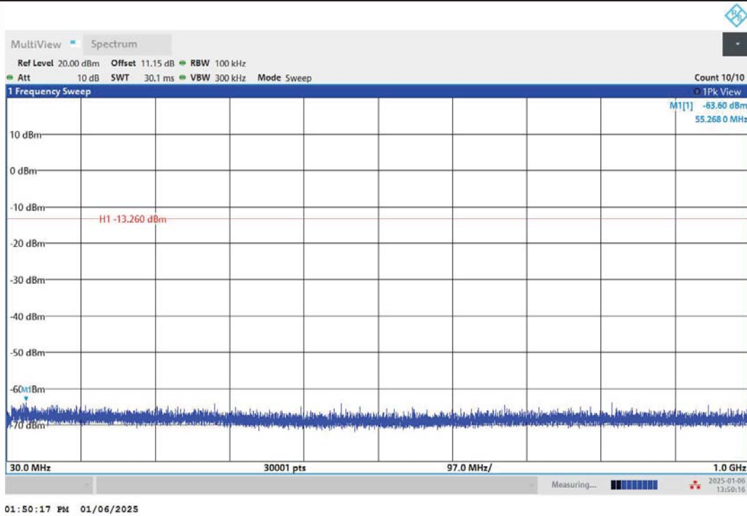
2DH5-Ant1-2480-30~1000-PASS
