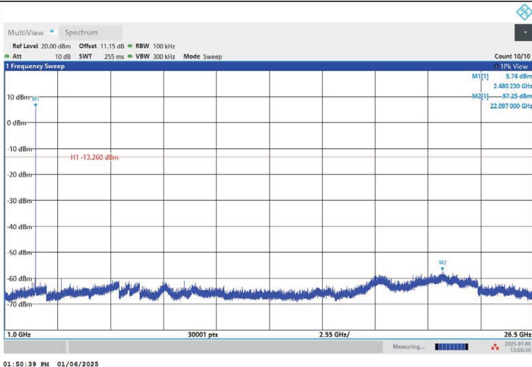
2DH5-Ant1-2480-1000~26500-PASS
