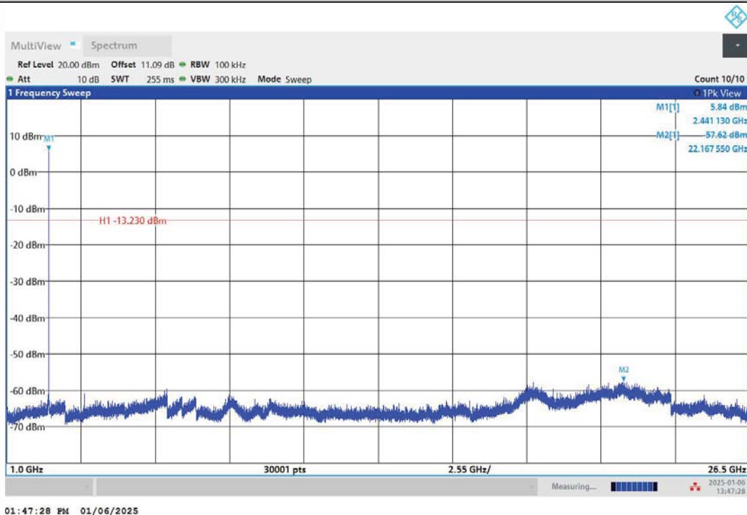
2DH5-Ant1-2441-1000~26500-PASS
