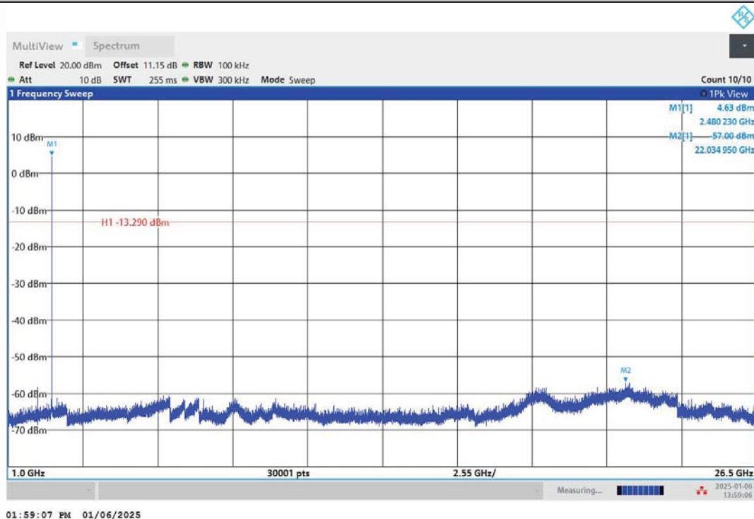
3DH5-Ant1-2480-1000~26500-PASS
