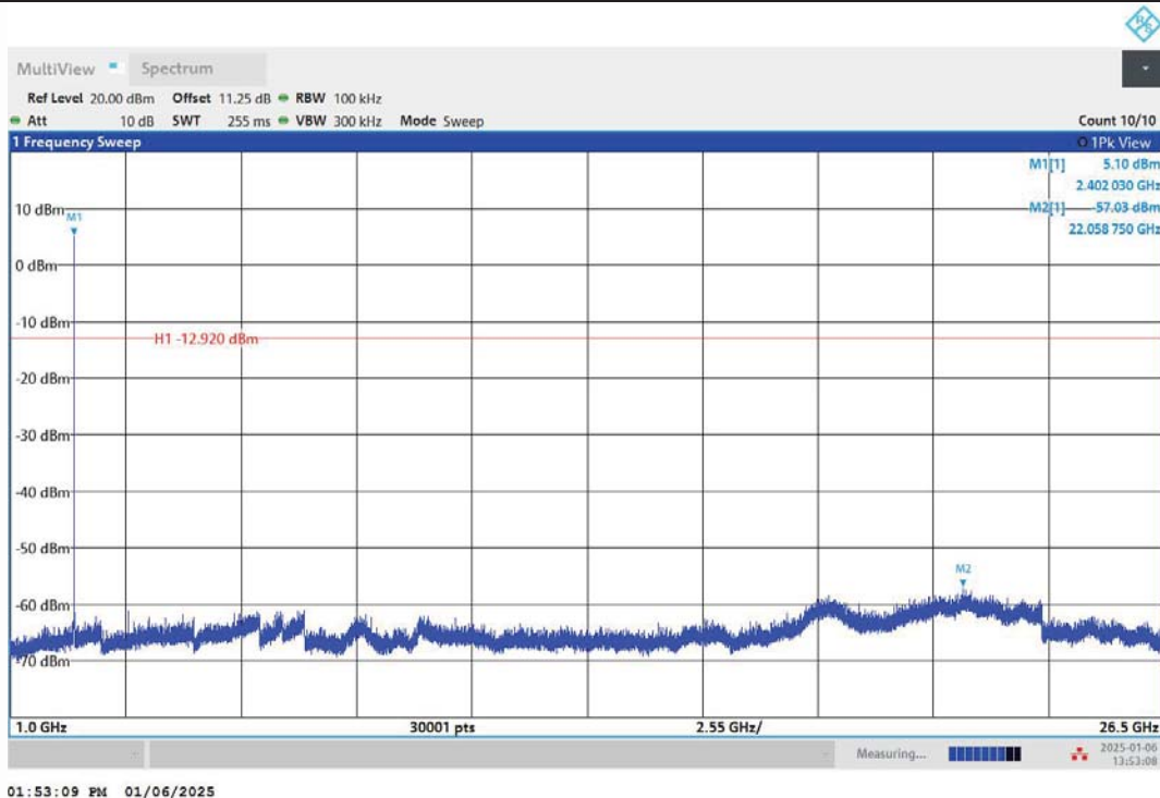
3DH5-Ant1-2402-1000~26500-PASS
