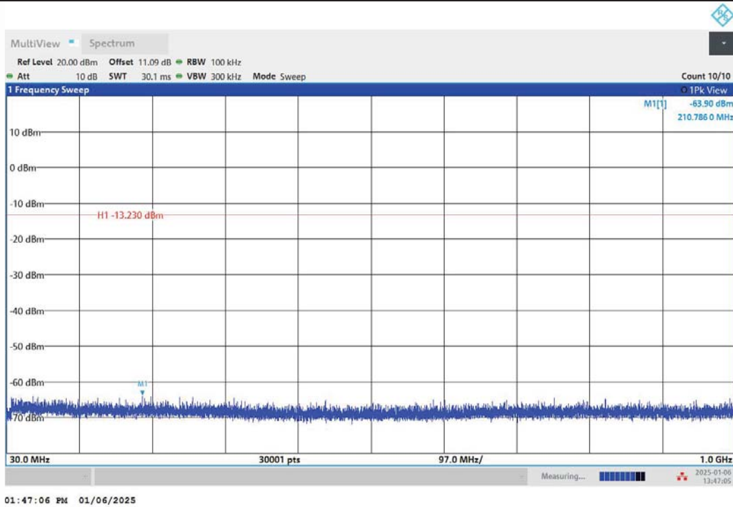
2DH5-Ant1-2441-30~1000-PASS
