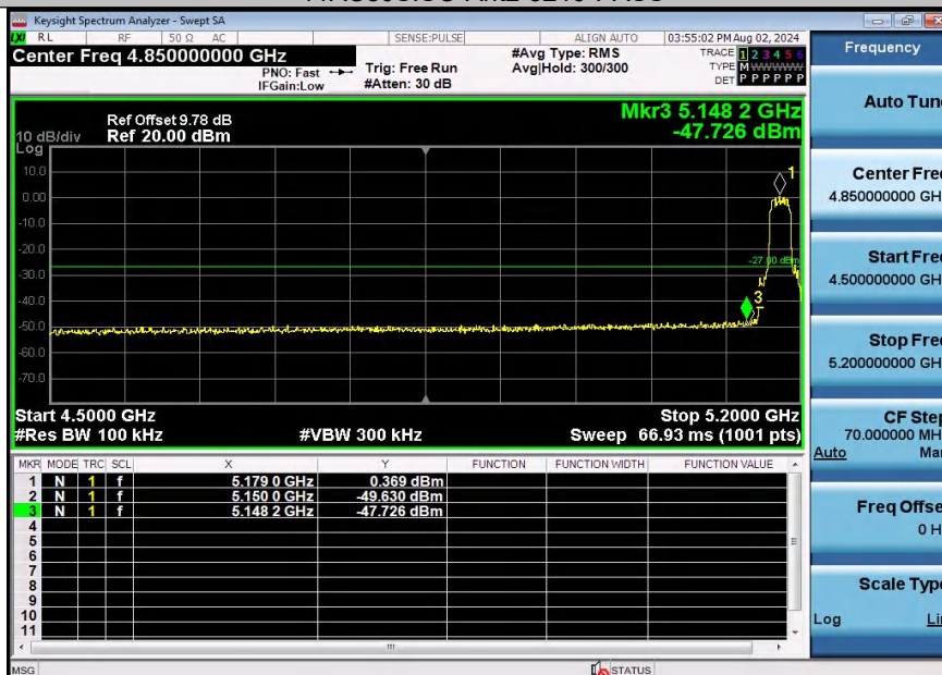
11AX20SISO-Ant2-5180-PASS
