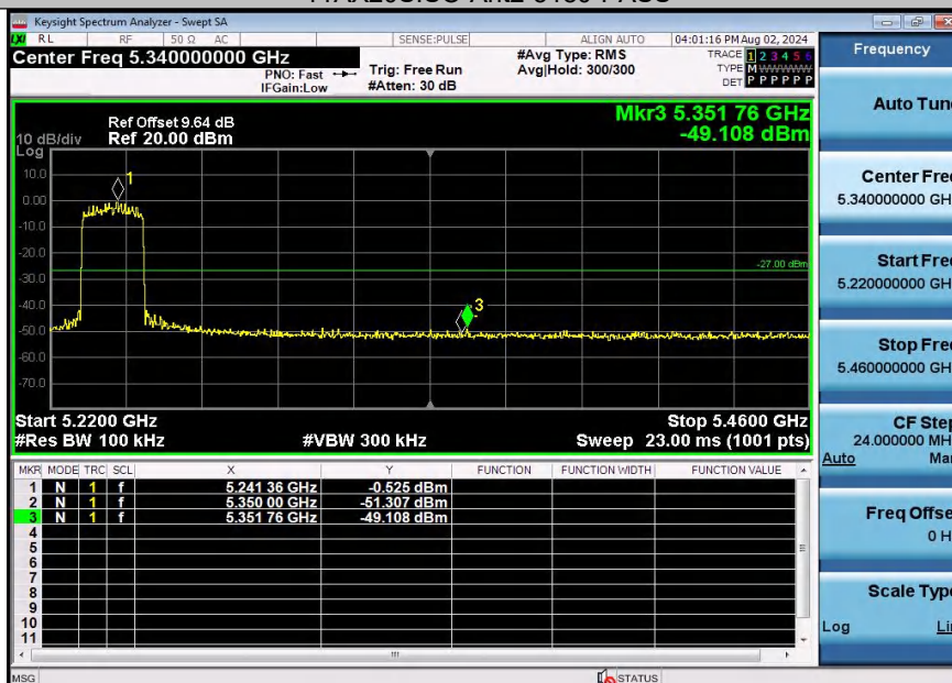
11AX20SISO-Ant2-5240-PASS
