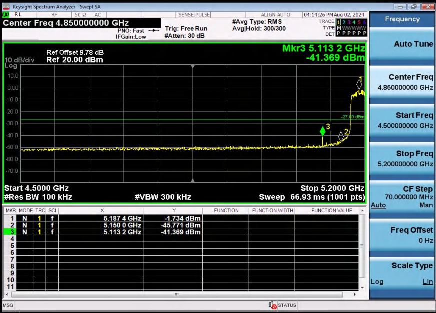
11AX40SISO-Ant2-5190-PASS
