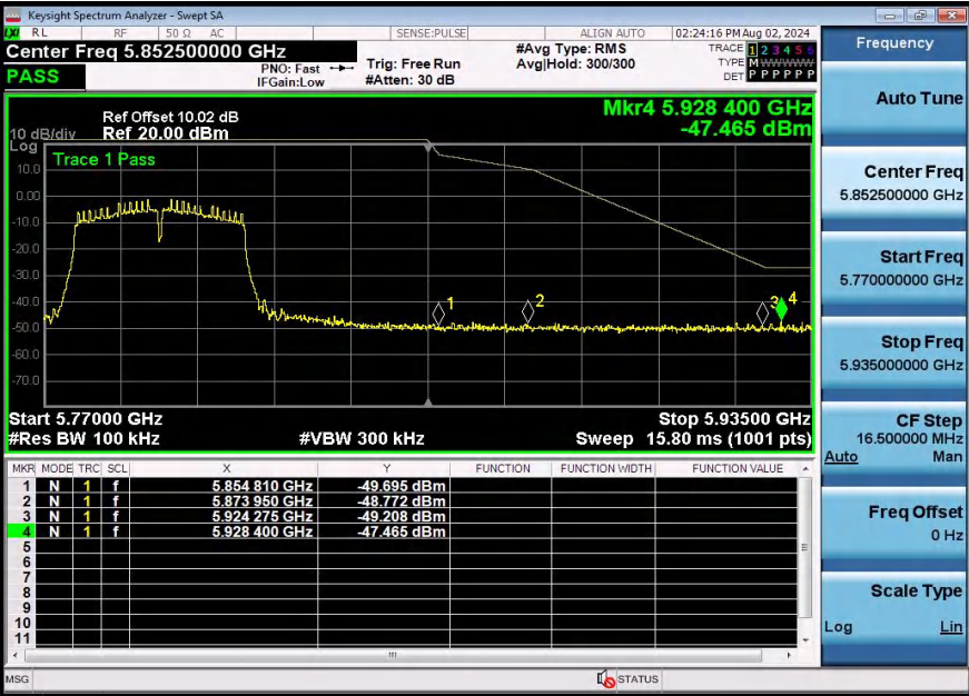
11N40SISO-Ant2-5795-PASS
