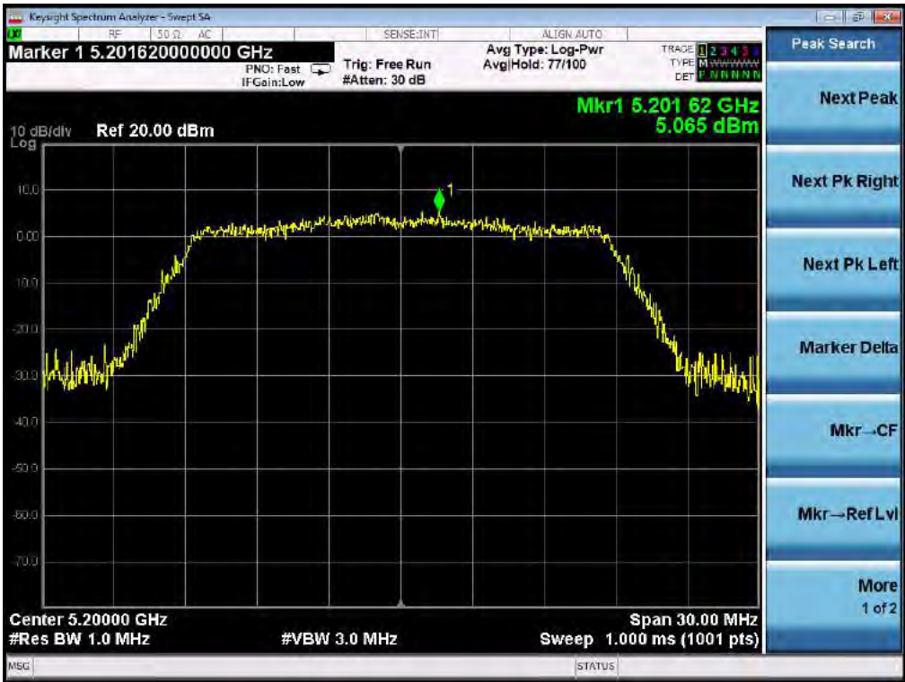
TEST PLOT OF SPECTRAL DENSITY FOR 5200MHz AT CHAIN 1
