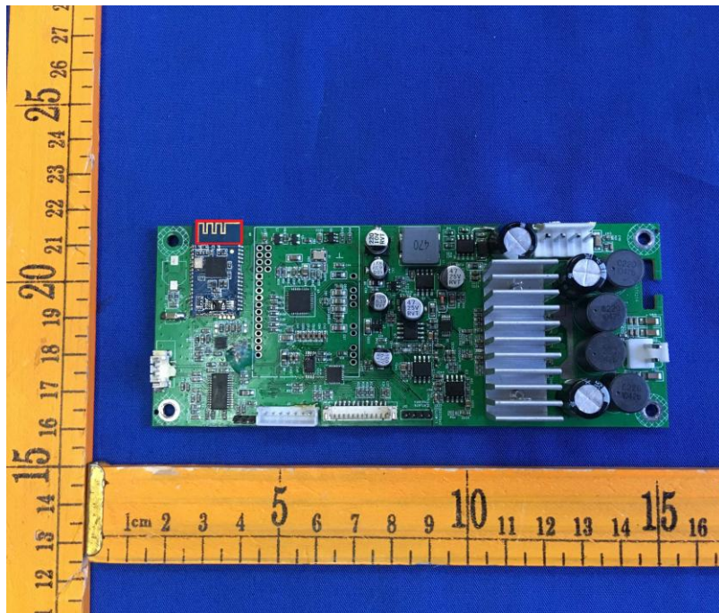
Antenna View
