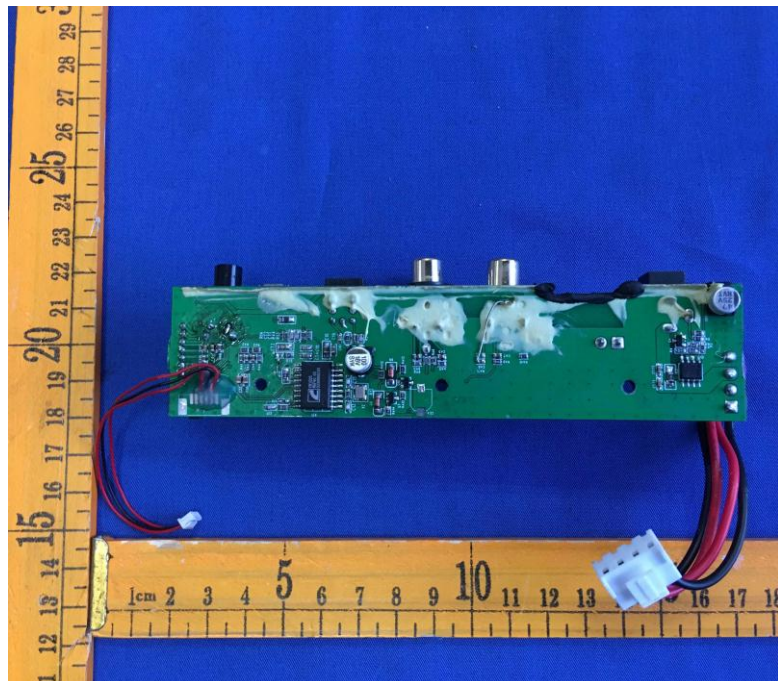
Small board – Rear View
