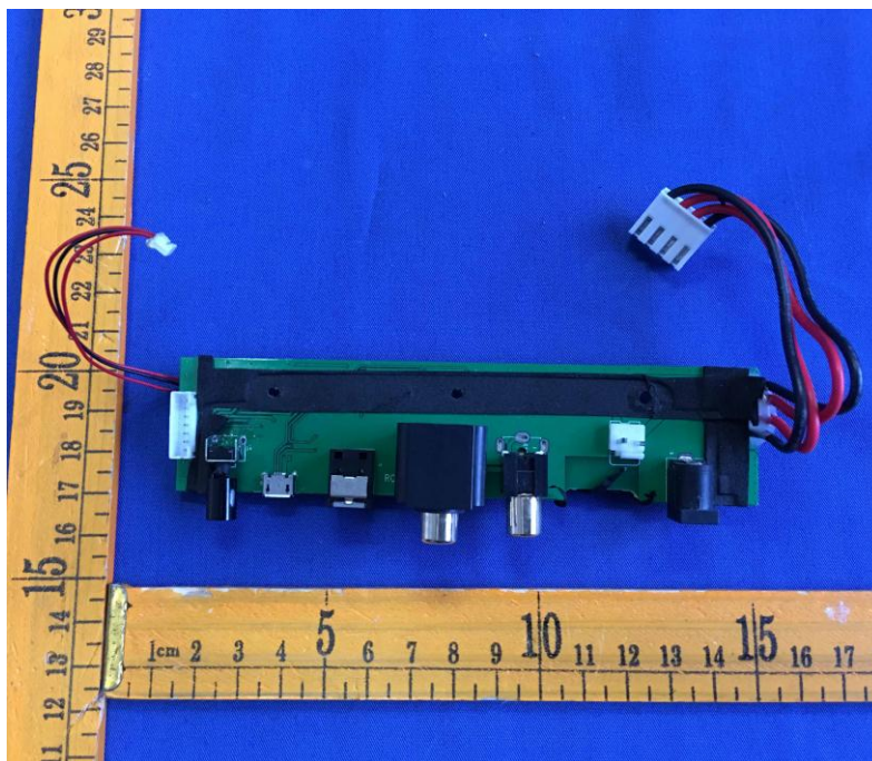
Small board – Front View
