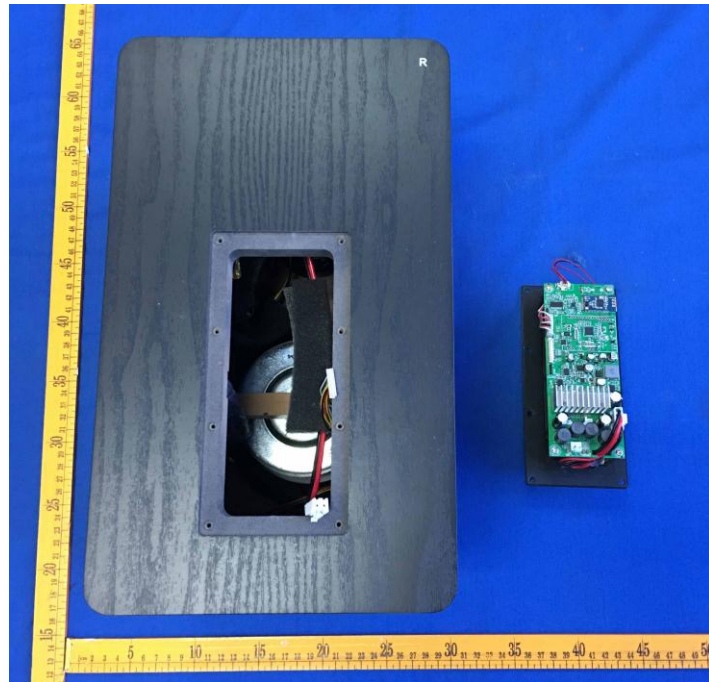
Cover Off View 1
