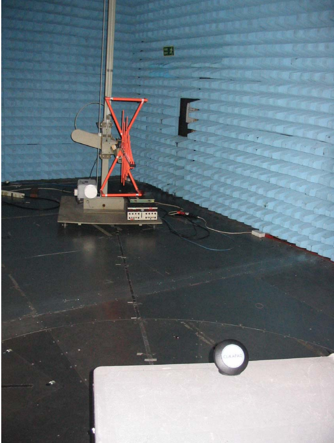
Radiated Emissions
