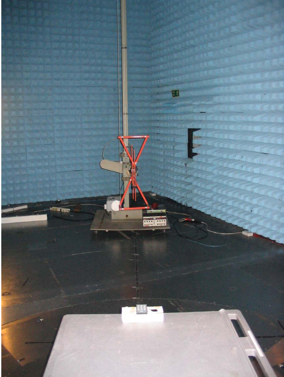
Radiated Emissions
