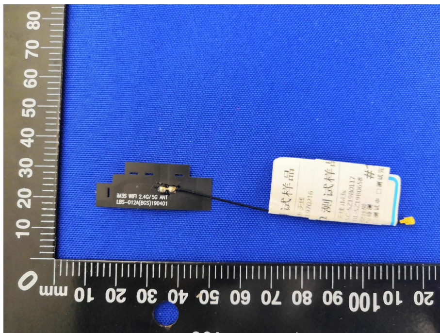
Antenna-iM3s
