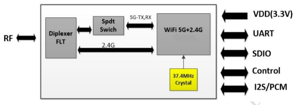
Figure 2 Block Diagram
