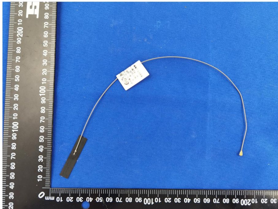
Antenna-iM3
