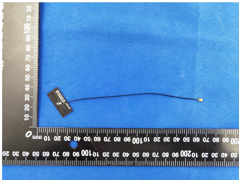
Antenna-iM50/iM60/iM70/iM80
