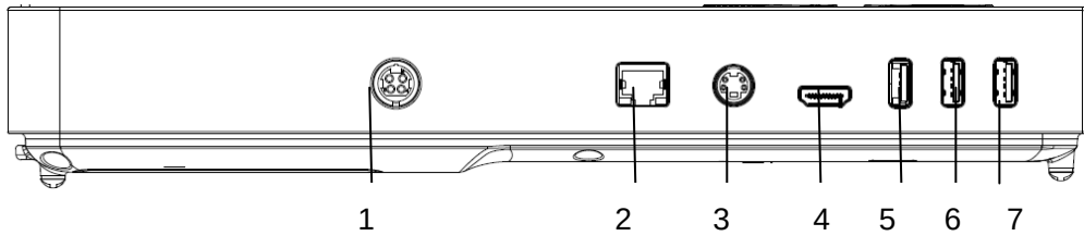
Figure 3-2 I/O ports
