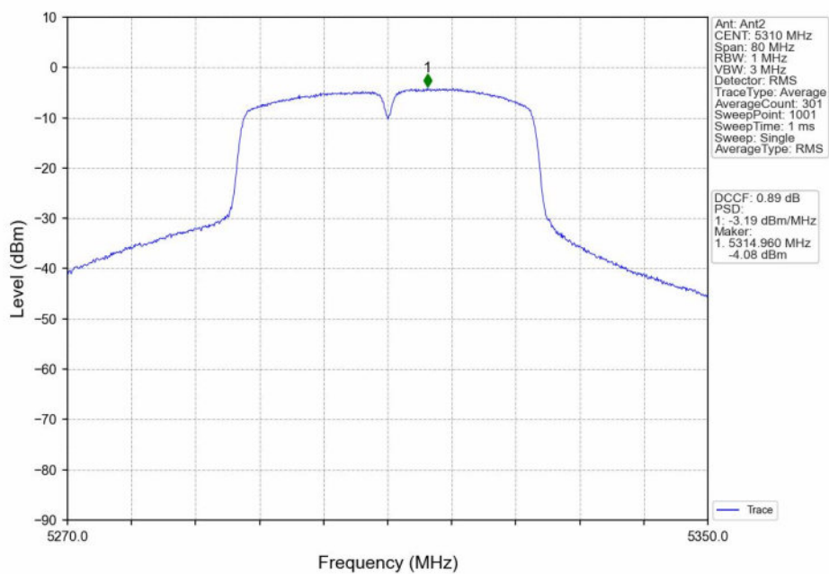
802.11ac(VHT40)_HCH_5310MHz_Ant2_NTNV
