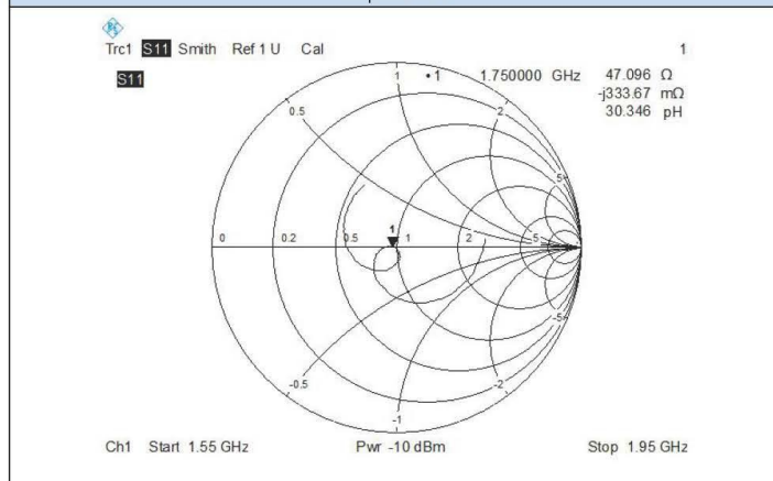
Impedance
