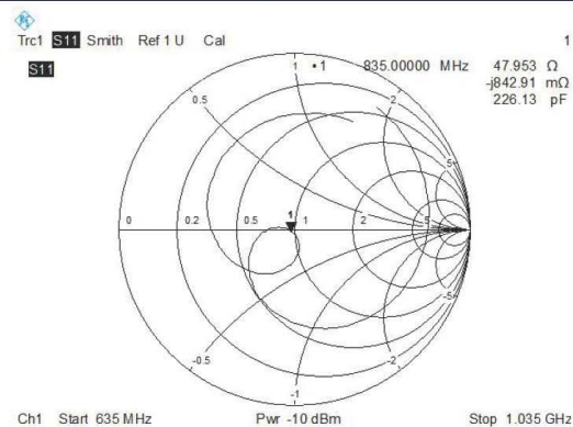
Impedance
