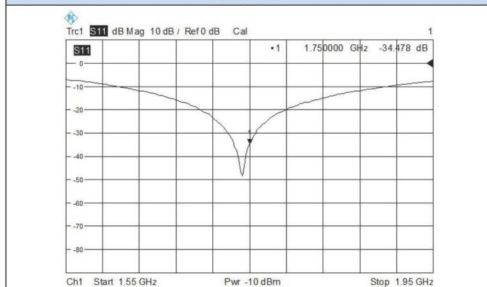
Return Loss
