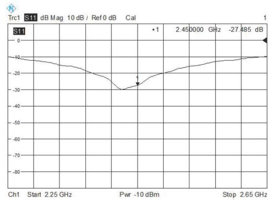
Return Loss
