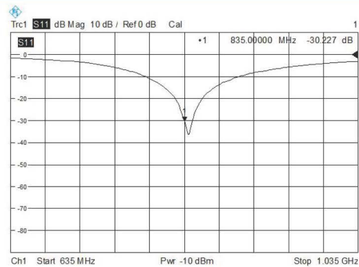
Return Loss
