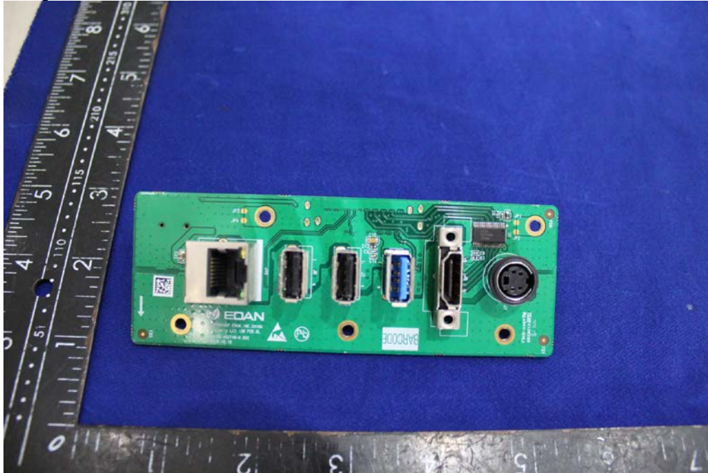
Solder Board-Component View 1
