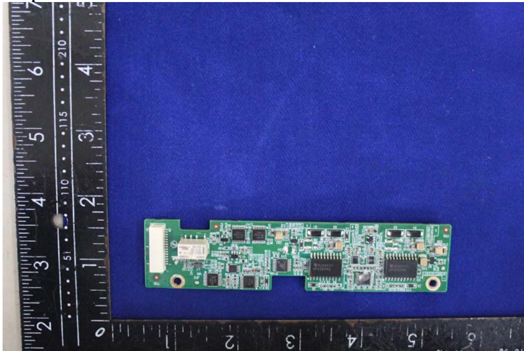
Solder Board-Component View 7
