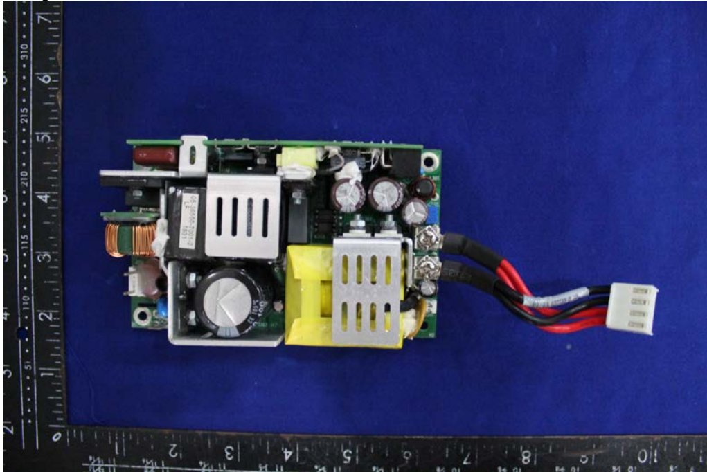
Solder Board-Component View 5
