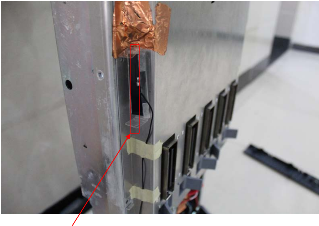
Antenna 1
