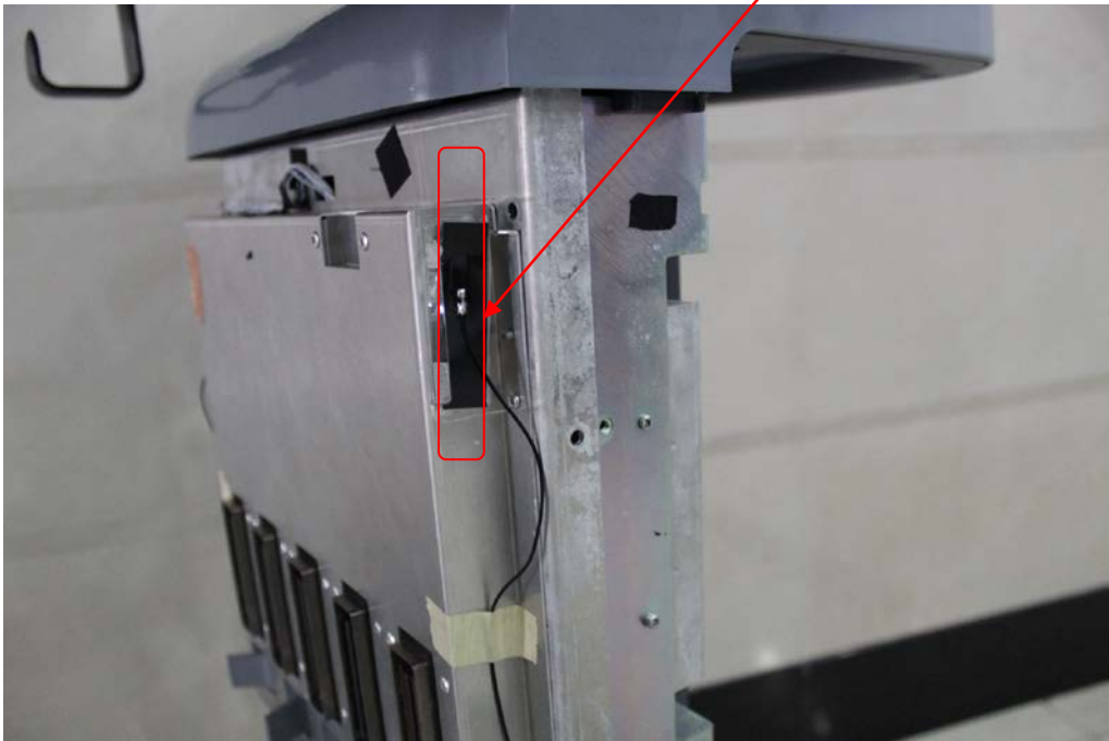
Antenna 2
