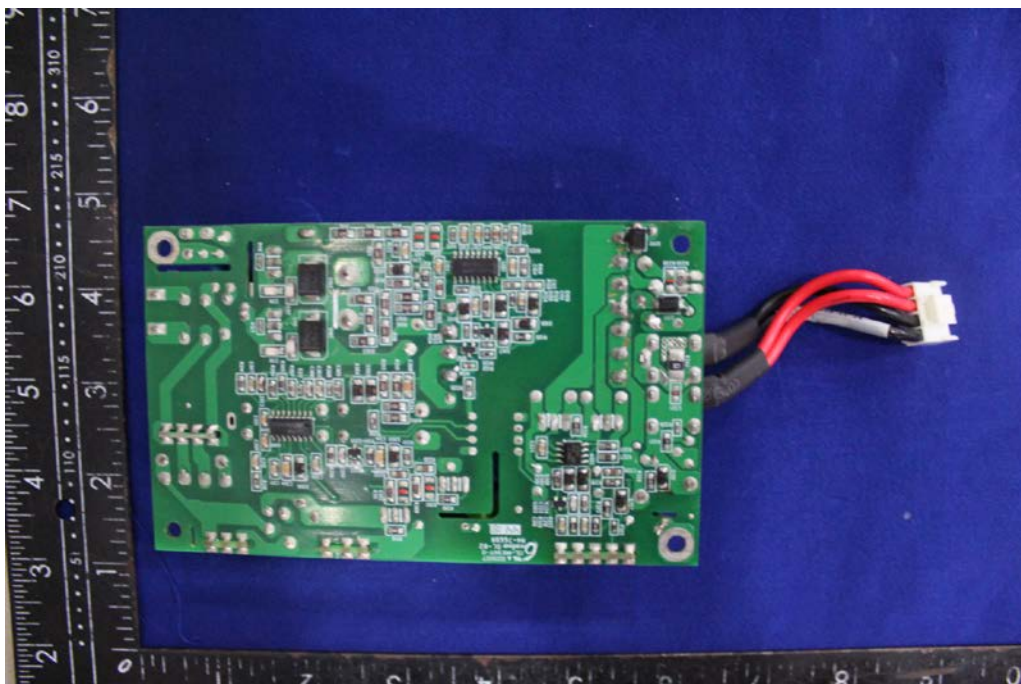
Solder Board-Component View 6
