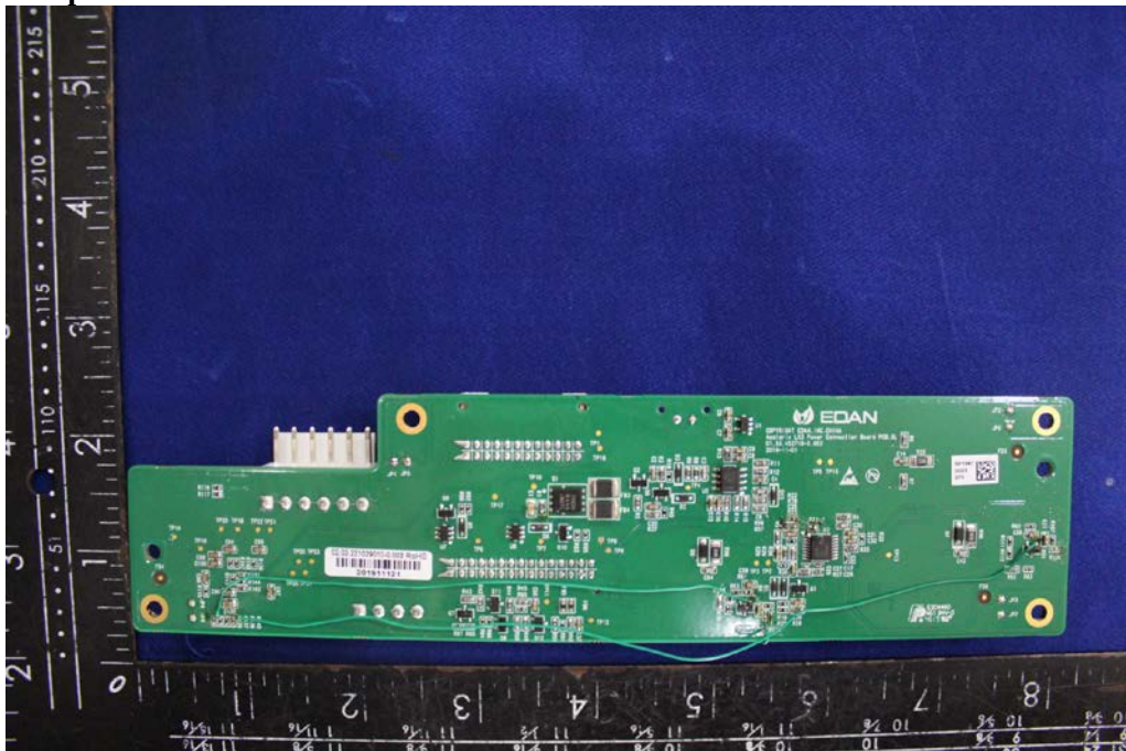
Solder Board-Component View 4
