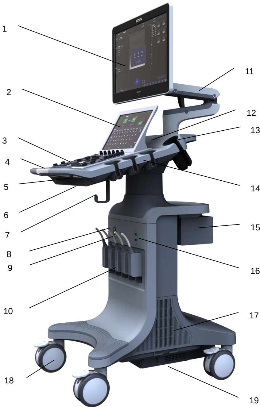
Figure 3-1 Main Unit
