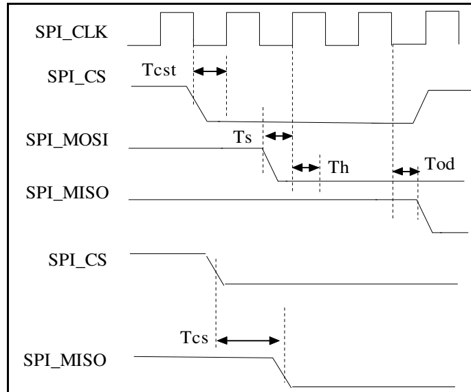
Figure 9: Interface Timings – SPI Interface Full-Speed Mode
