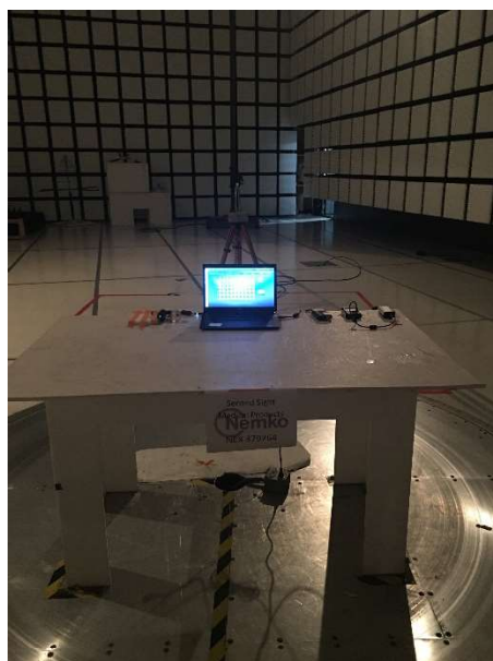
Figure 9.2.10 Radiated emissions 9 kHz-30 MHz (Test antenna at 90 deg, Back)
