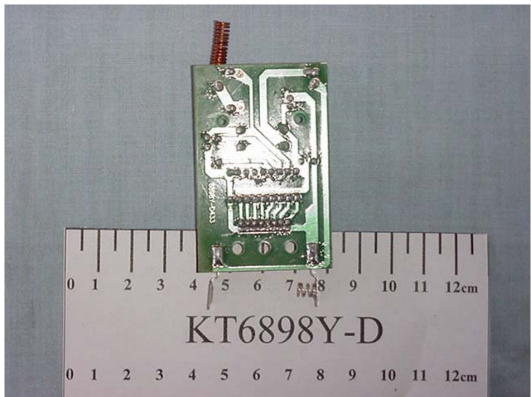
FIGURE 3 WIRELESS DOOR CHIME (M/N: KT6898Y-D) MAIN BOARD (SOLDERED SIDE)
