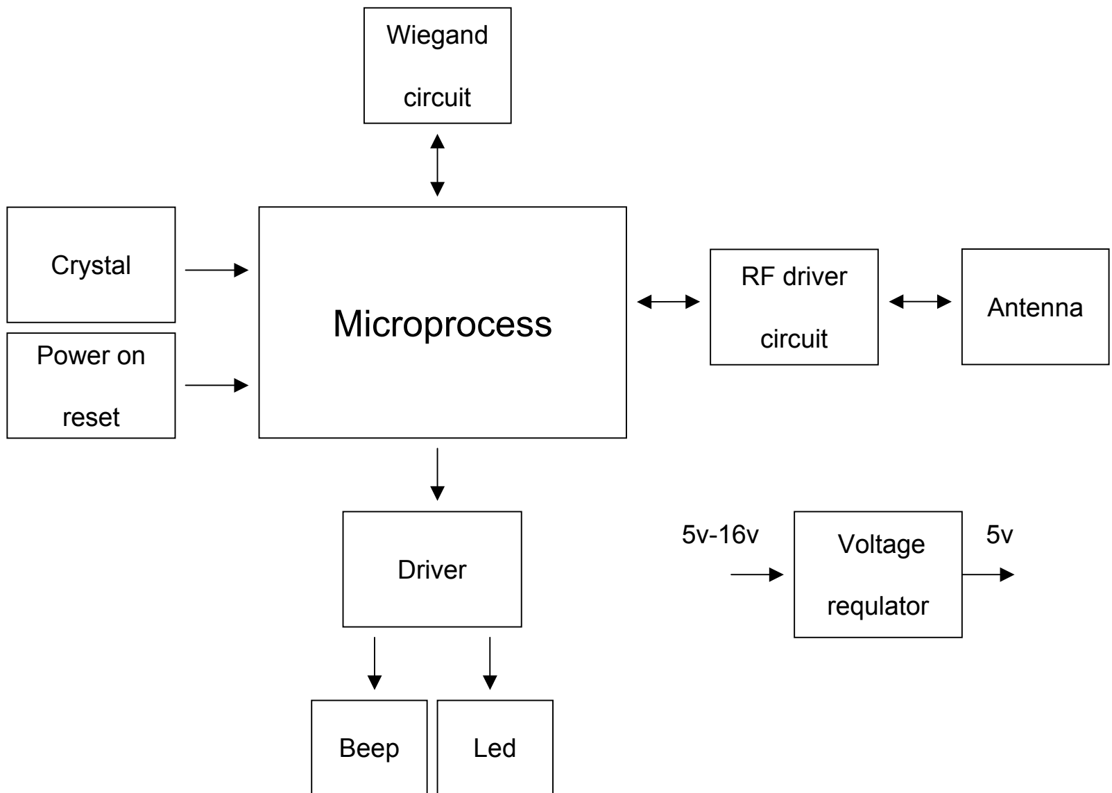
MINRD-1 BLOCK DIAGRAM
