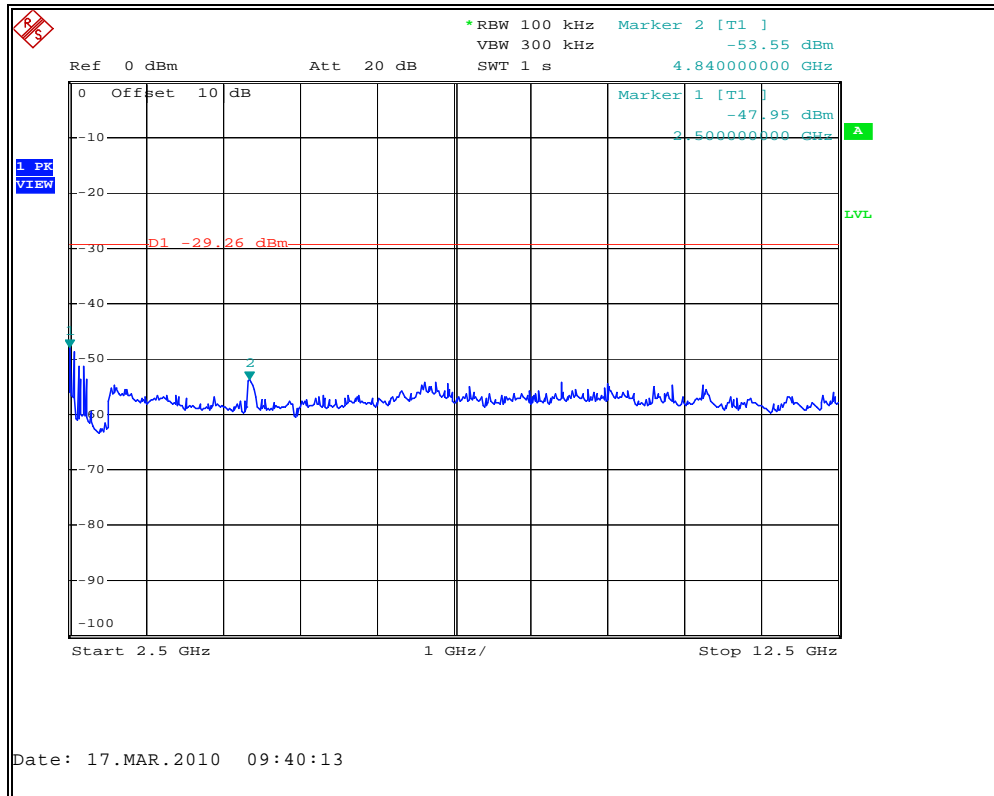
Figure 7.6.2.2-2: 2.5 GHz – 12.5 GHz
