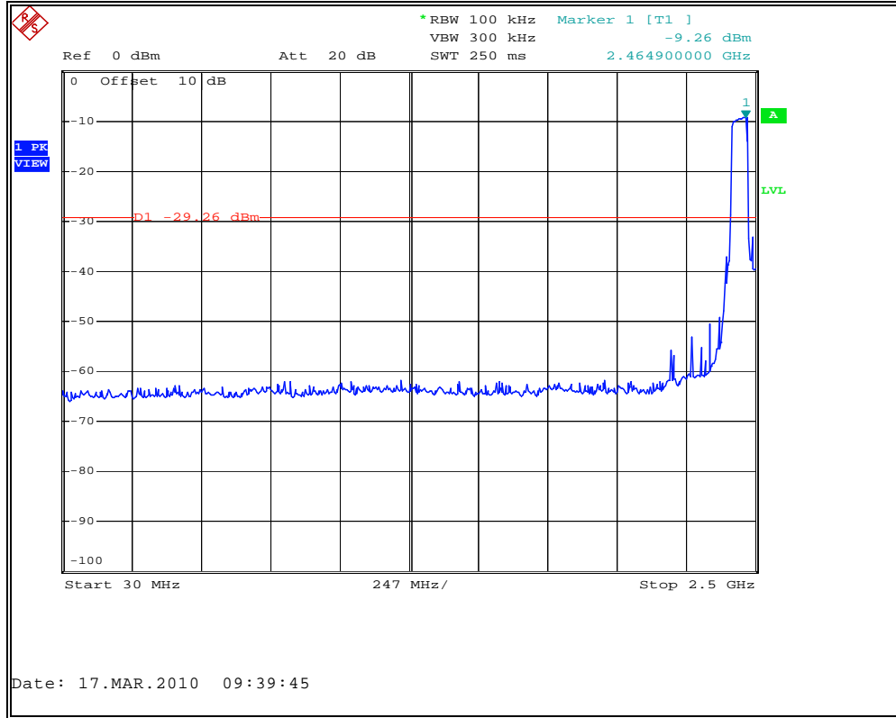
Figure 7.6.2.2-1: 30 MHz – 2.5 GHz
