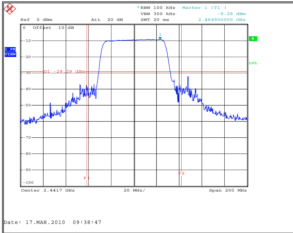
Figure 7.6.2.2-4: Band-edge (Conducted)
