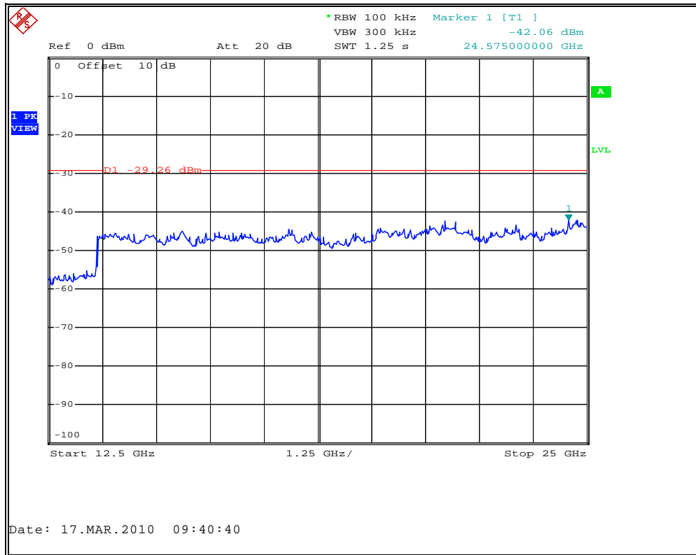
Figure 7.6.2.2-3: 12.5 GHz – 25 GHz
