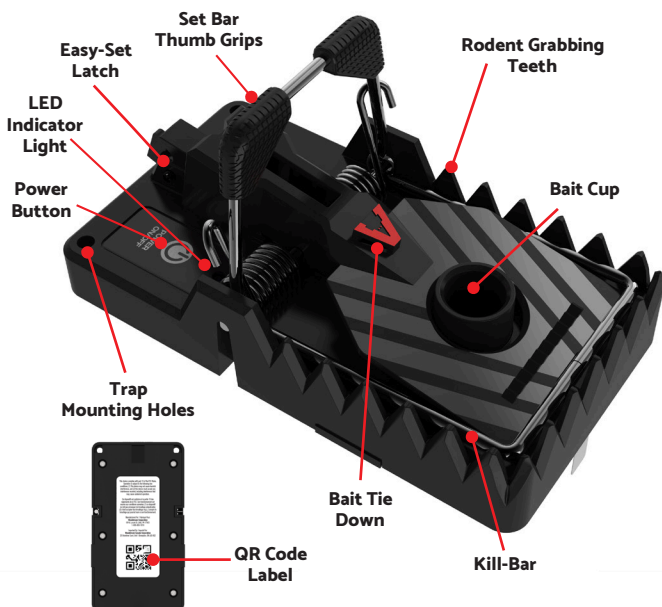
Victor® VLINK® Rat Trap Model: V430B
