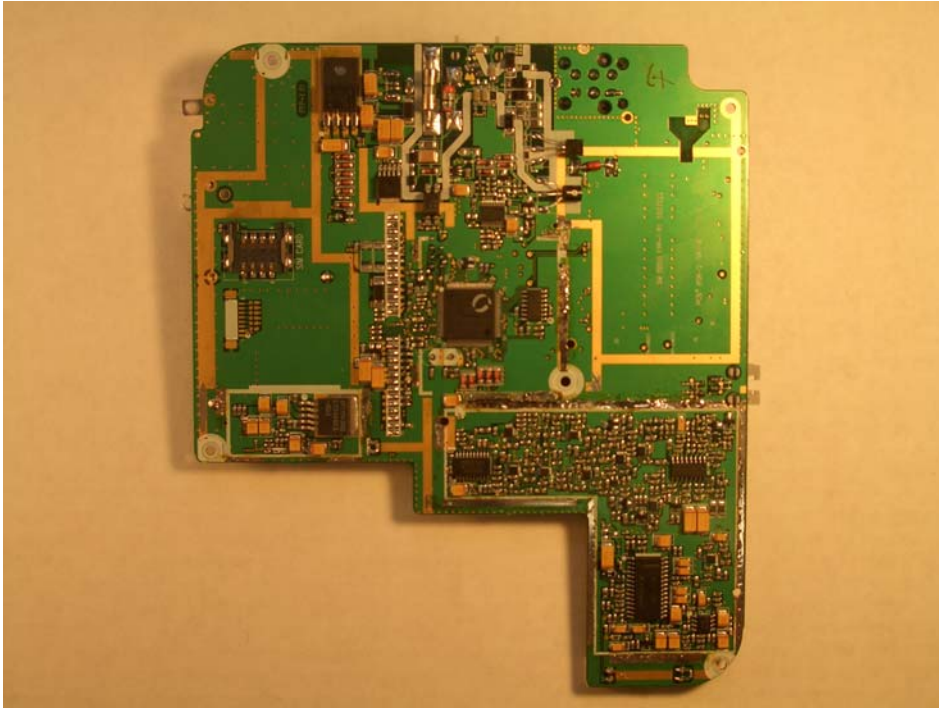
Base Component View without shielding
