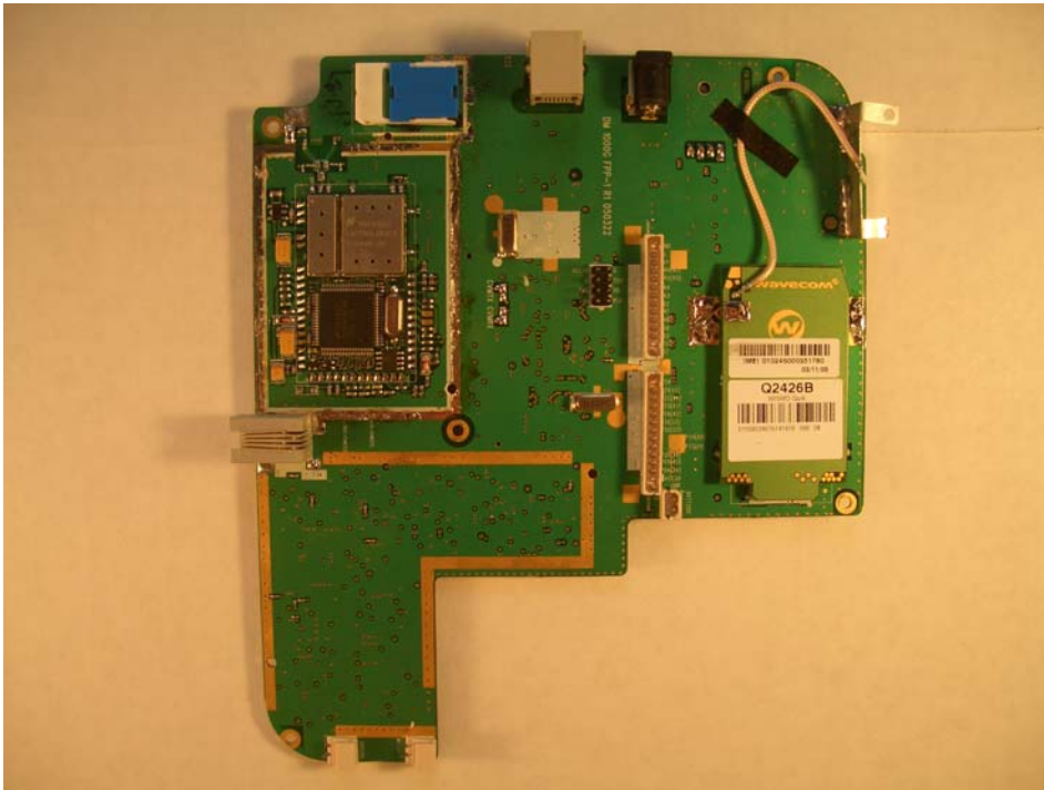
Base Solder View without Shielding
