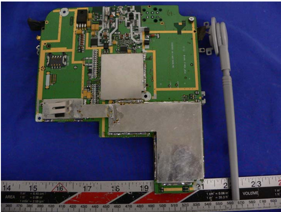
Base Component View with shielding
