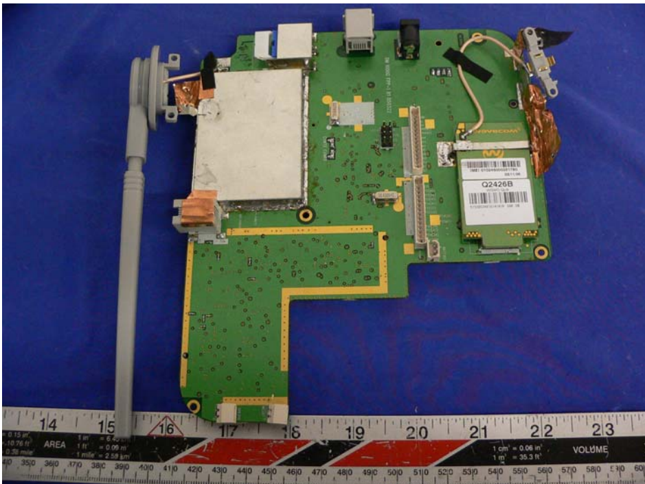
Base Solder View with Shielding
