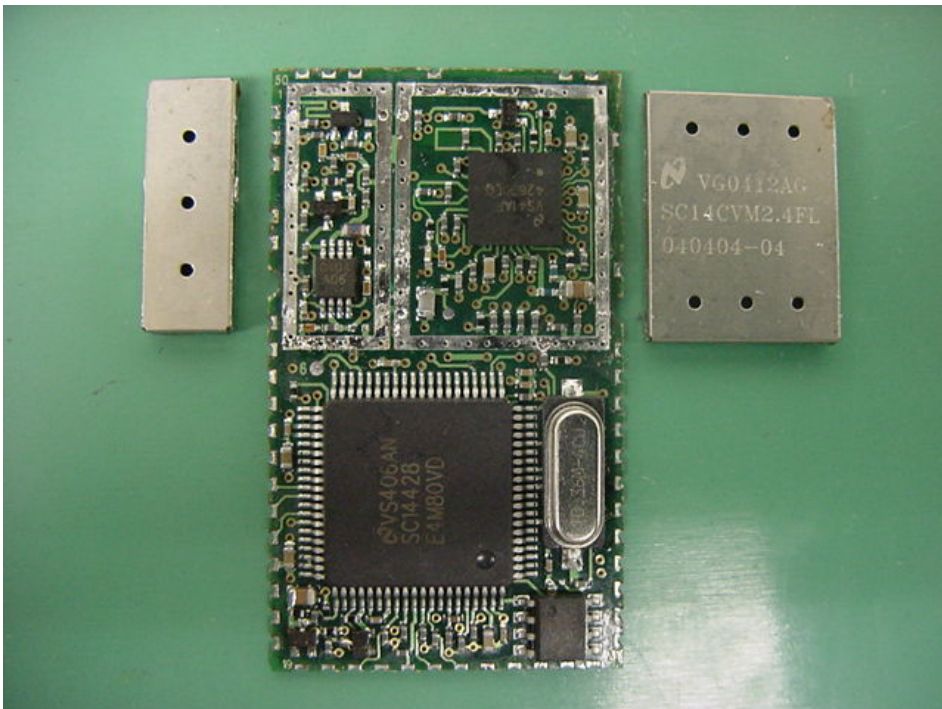
Transmitter Component View
