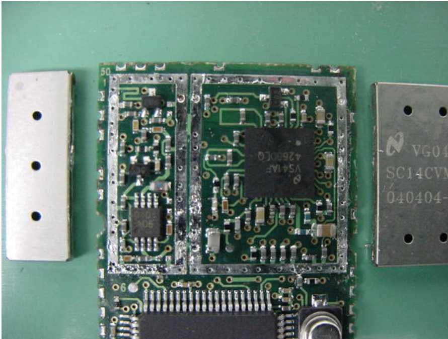
Base – Transmitter Close View 3
