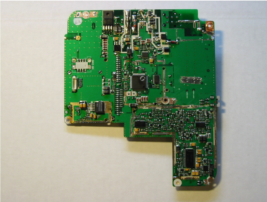
Base – Board Component Shield Cover Removed View
