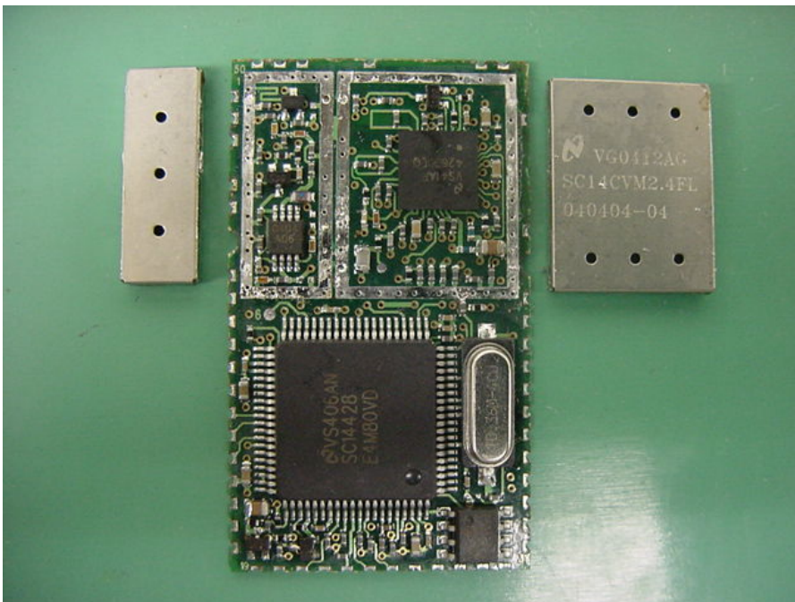
Base – Transmitter Close View 2
