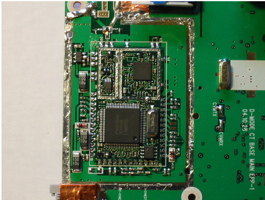
Base – Transmitter Close View 1
