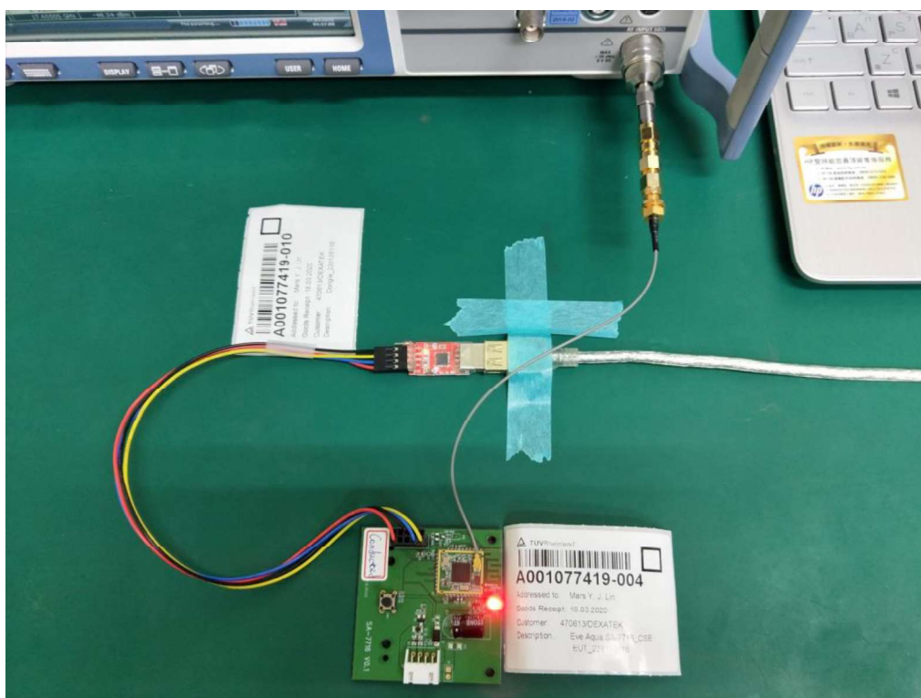
Photograph 8: Set-up for Conducted Testing (View 2)
