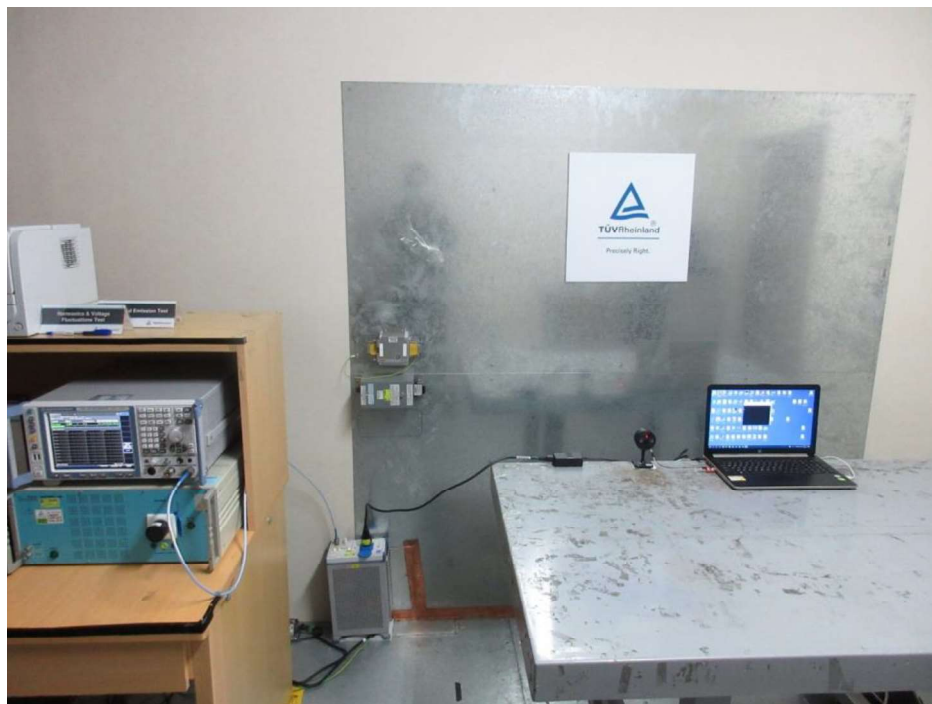
Photograph 8: Set-up for AC Mains (Front View)
