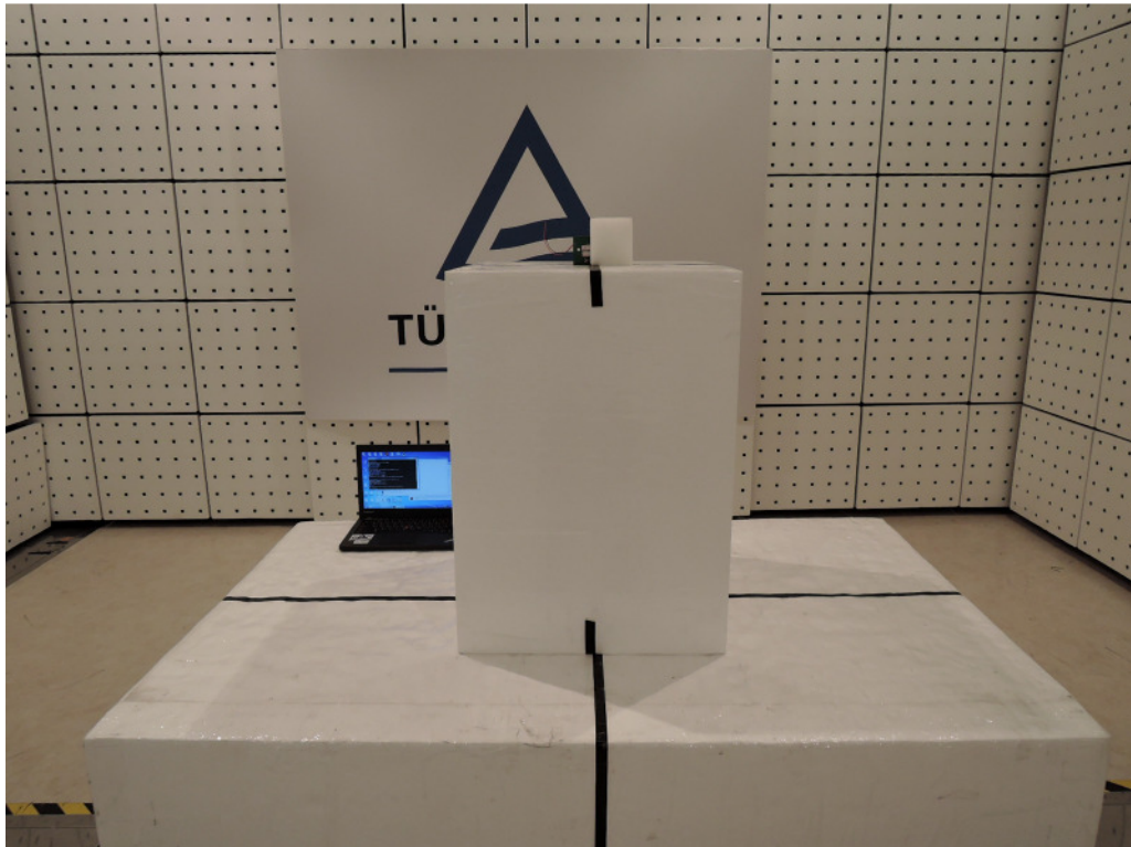
Photograph 1: Set-up for Fundamental and Spurious Emissions (Front View)
