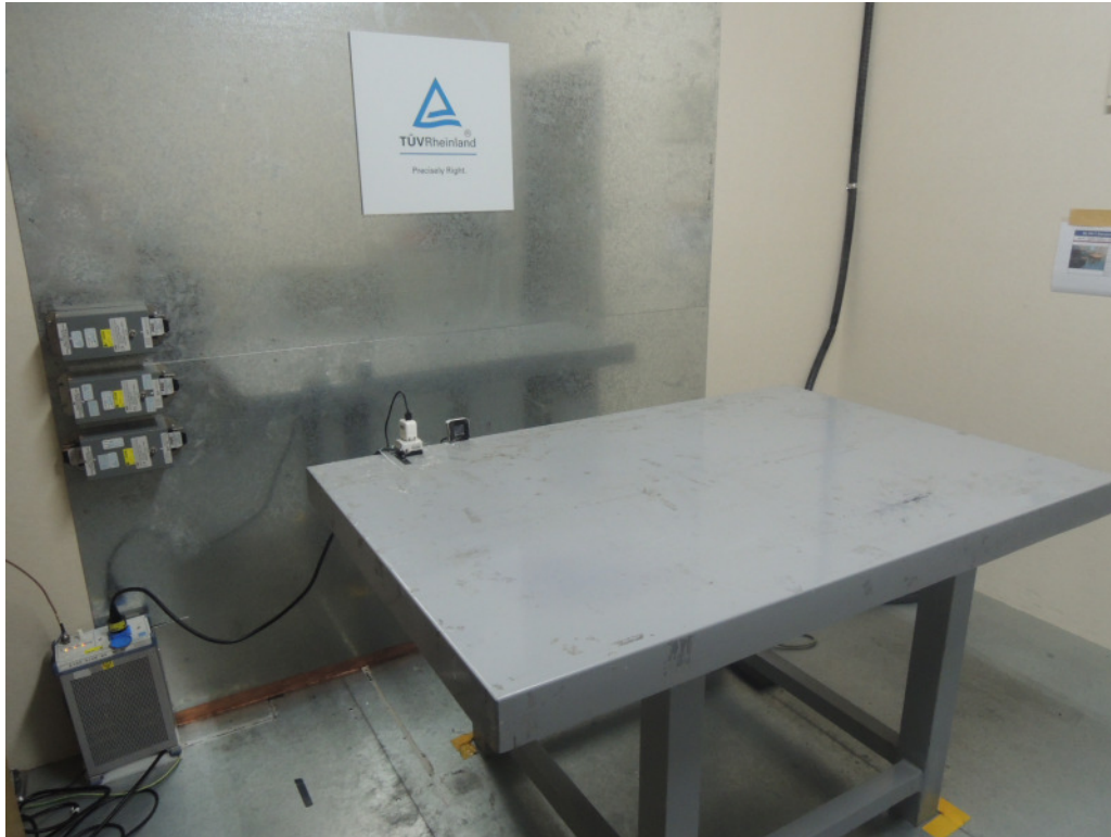
Photograph 7: Set-up for Mains Conducted testing (Back view)
