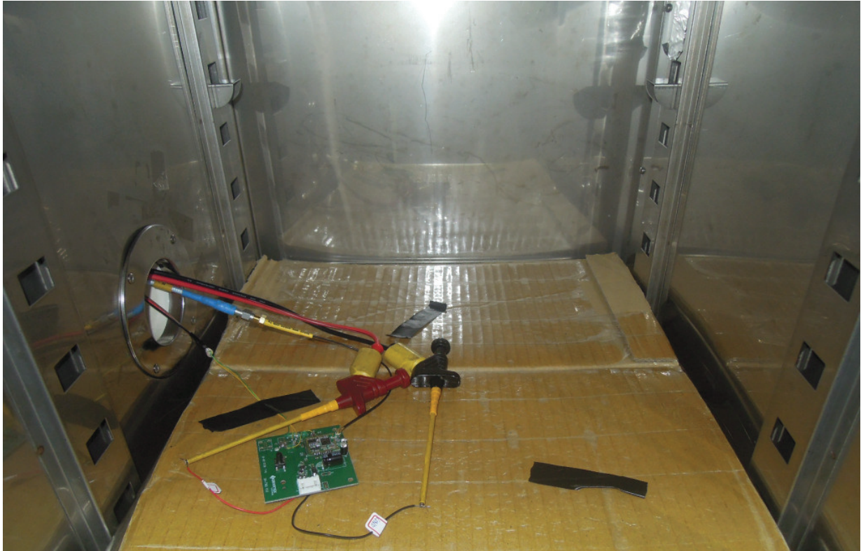
Photograph 6: Set-up for Conducted testing
