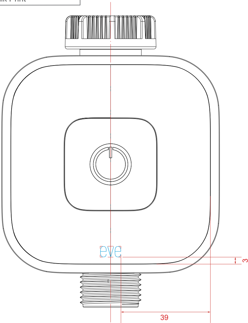
PRINTING DIMENSION
