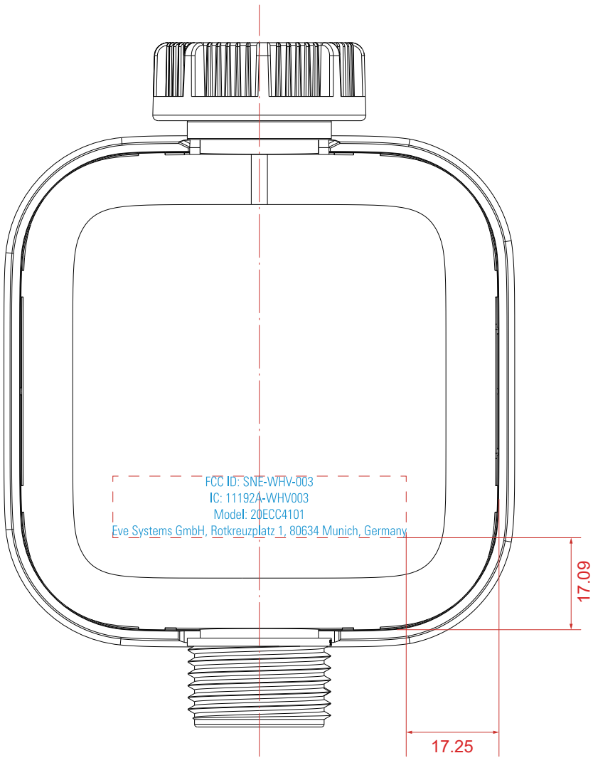
PRINTING DIMENSION
