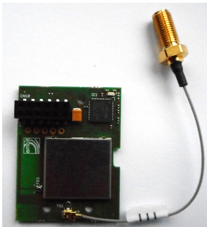
Radio board with connected antenna connector
