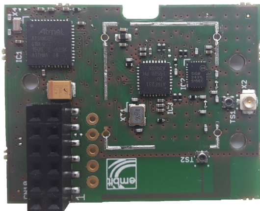
Radio board without RF shield
