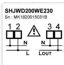
230V, connections
