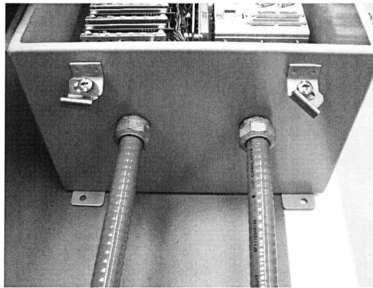
Figure 4 Modem cable and AC wiring
